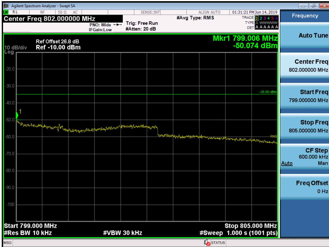
BAND 14 Upper Emission Mask (799 MHz ~805 MHz) Plot (5M BW Ch.23355 QPSK_RB25_0)-2
