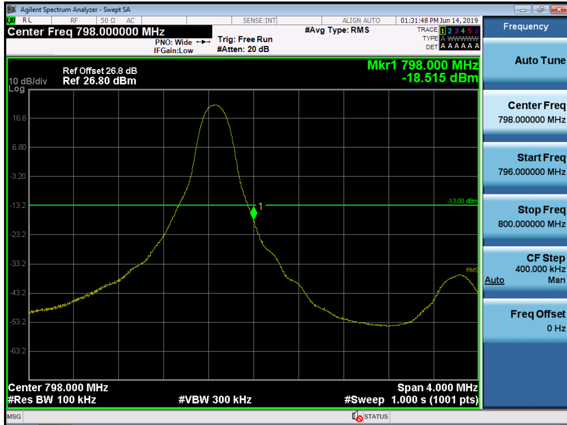
BAND 14 Upper Band Edge Plot (5M BW Ch.23355 QPSK_RB1_Offset 24)
