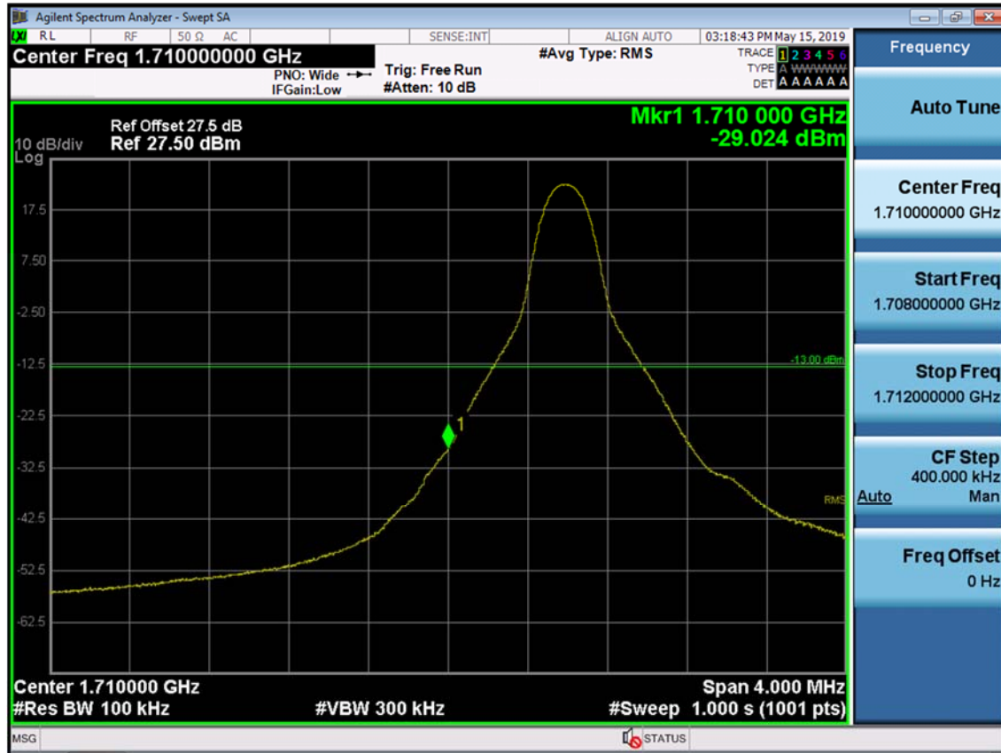
BAND 66/4. Lower Band Edge Plot (10M BW Ch.132022 QPSK RB 1, Offset 0) -1
