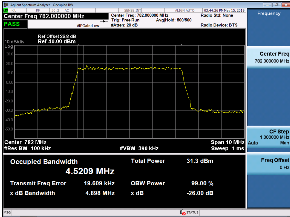
BAND 13. Occupied Bandwidth Plot (Ch.23230 QPSK RB 25) 5 MHz
