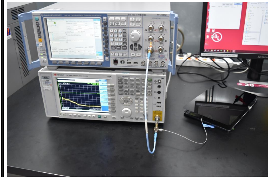
LICENSED BAND TEST PHOTO
