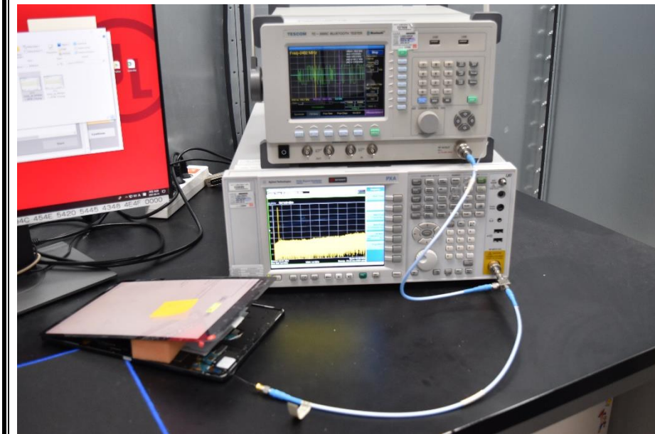
BLUETOOTH TEST PHOTO
