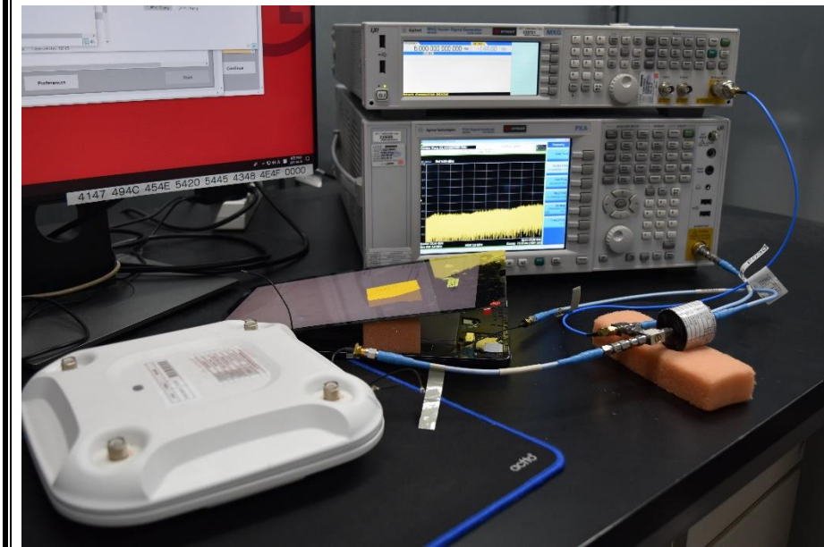
DFS TEST PHOTO
