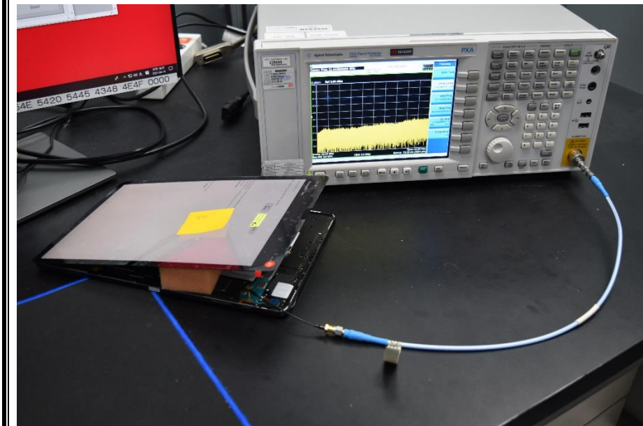
CONDUCTED TEST PHOTO
