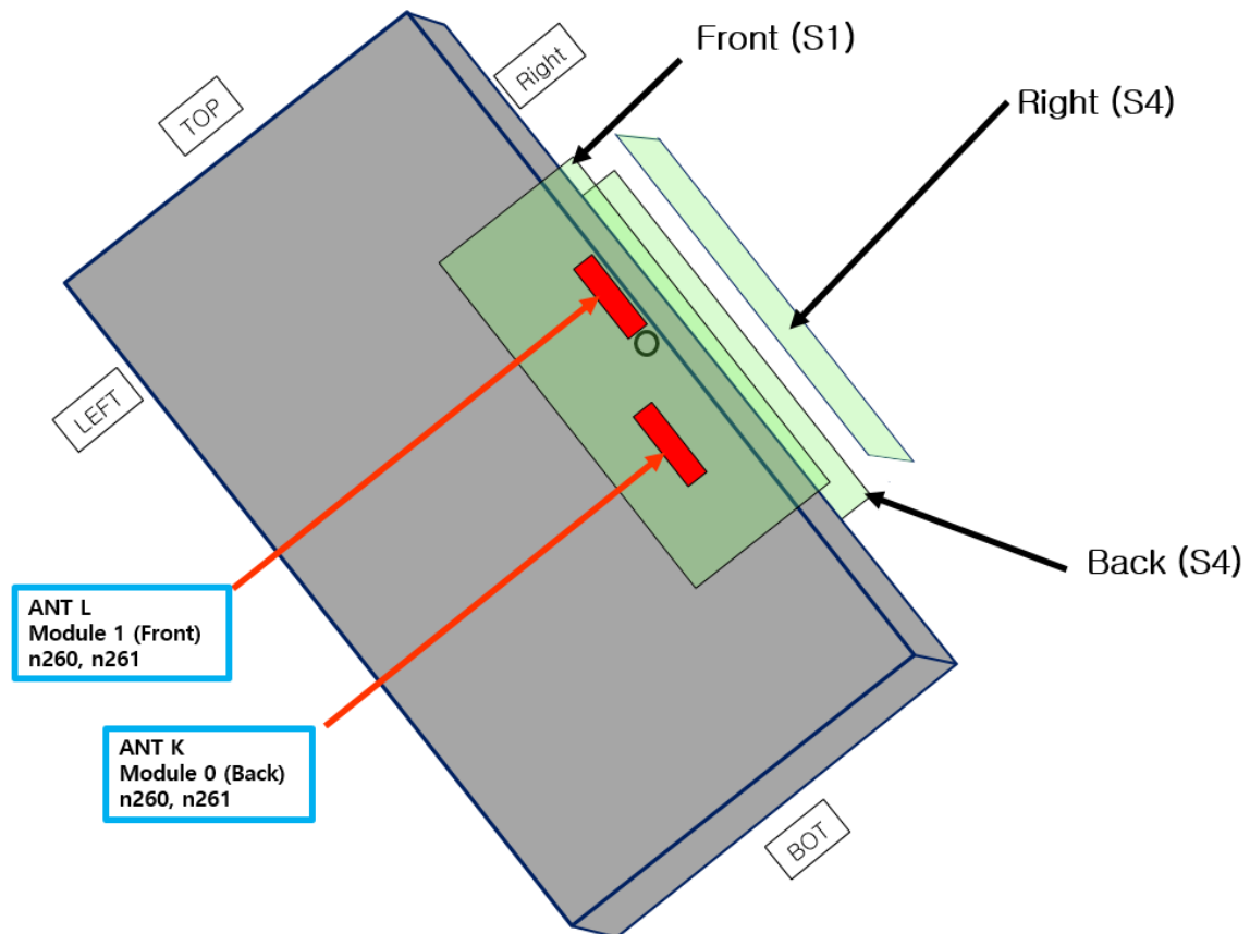
(a) ANT K L Front view
