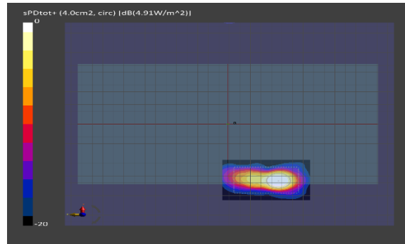
(b) Measurement Front view
