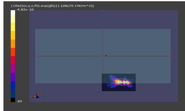
(b) Measurement Front view
