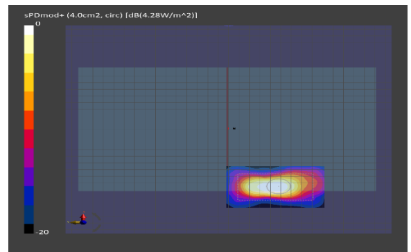
(b) Measurement Front view
