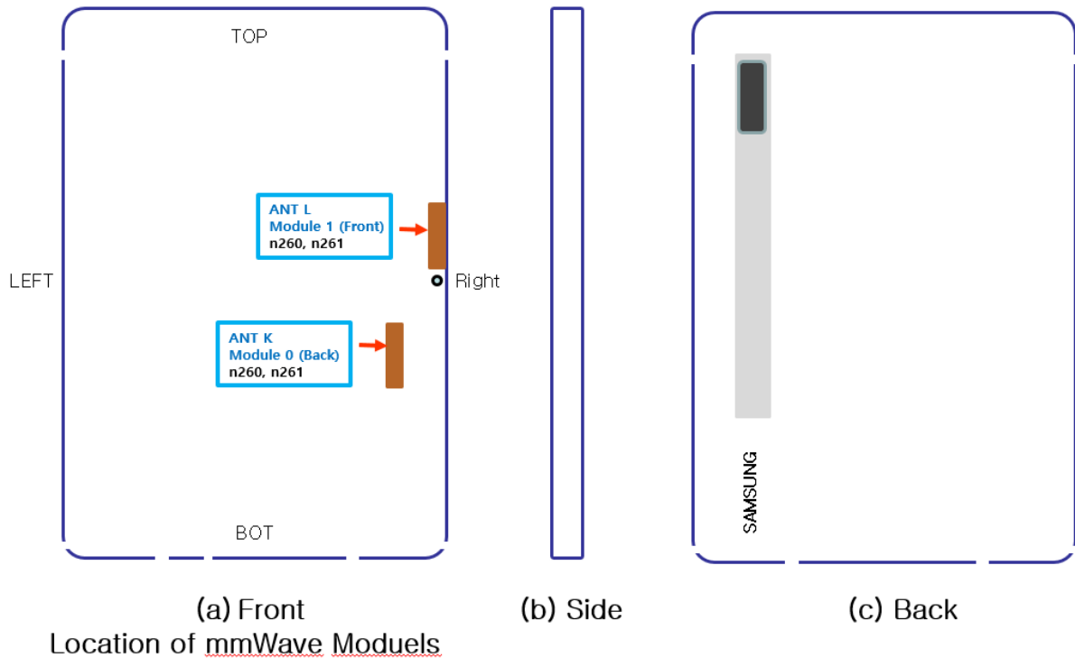
Figure 3 Simulation model which is mounted two mmWave antenna modules
