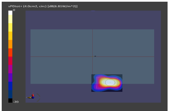
(b) Measurement Front view
