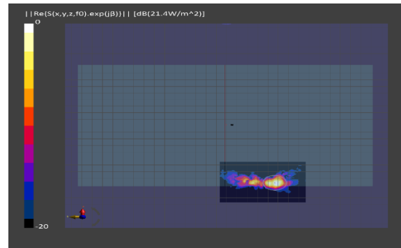
(b) Measurement Front view
