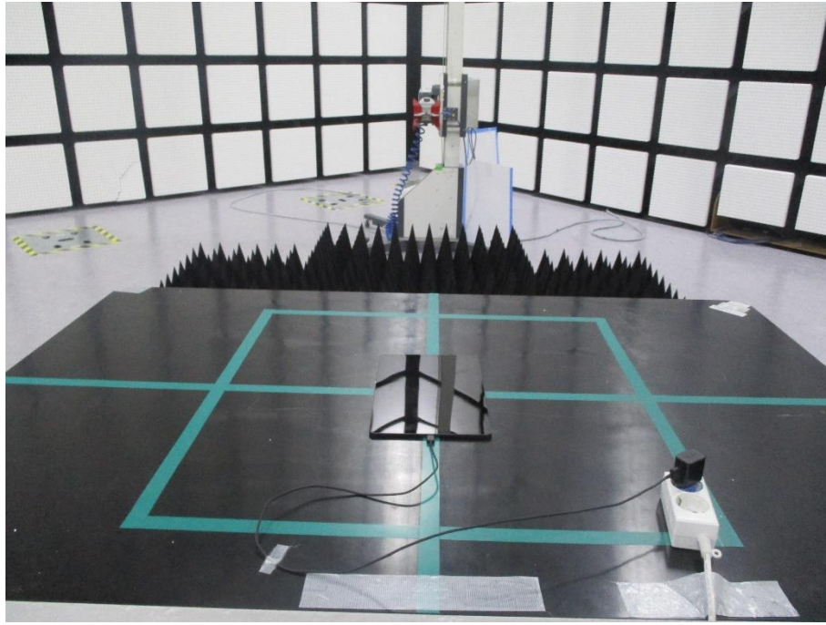
ABOVE 1 GHz FRONT TEST PHOTO (CXX)
