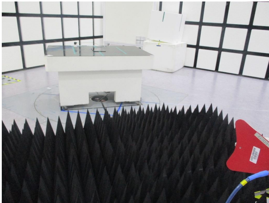
ABOVE 1 GHz REAR TEST PHOTO (CXX)
