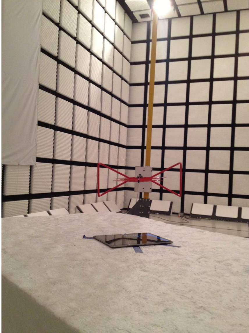
RADIATED BACK PHOTO (BELOW 1 GHz)
