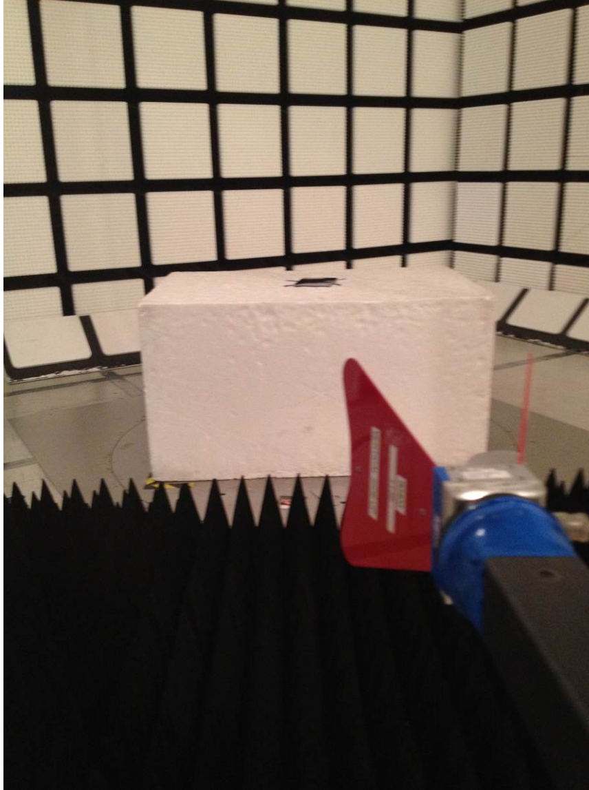
RADIATED FRONT PHOTO (ABOVE 1 GHz)
