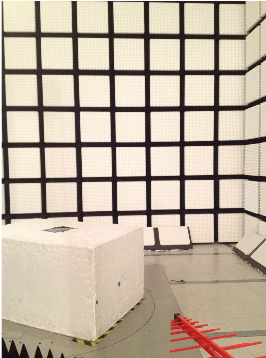
RADIATED FRONT PHOTO (BELOW 1 GHz)
