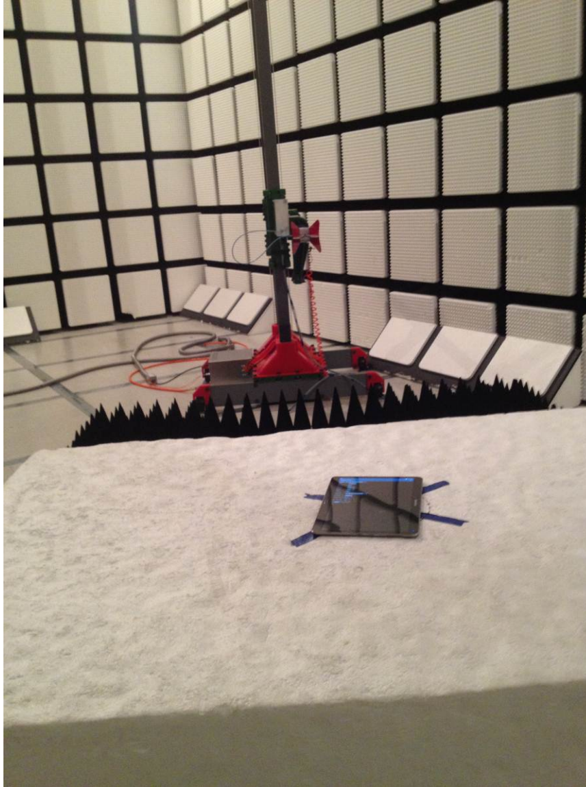
RADIATED BACK PHOTO (ABOVE 1 GHz)
