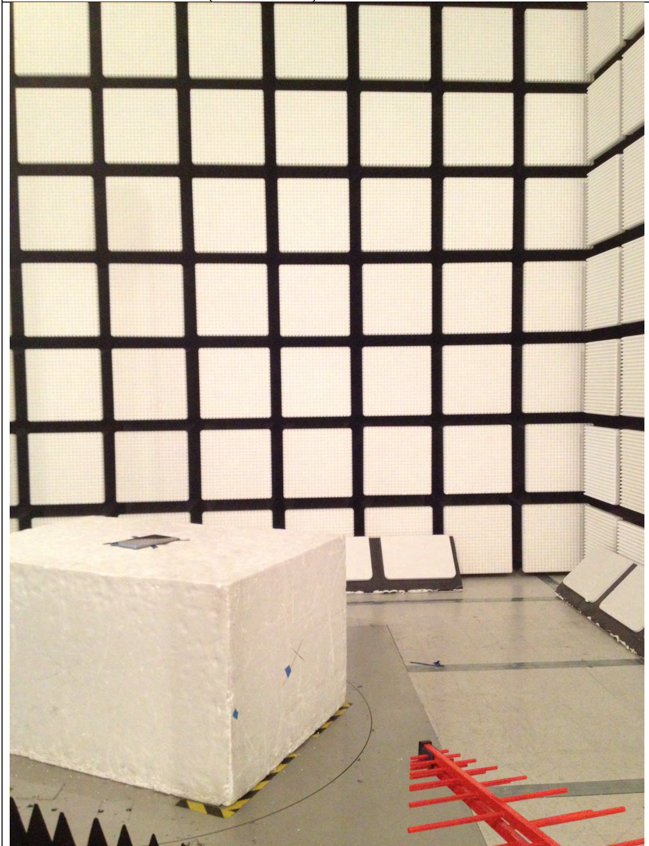
RADIATED FRONT=PHOTO (BELOW 1 GHz)
