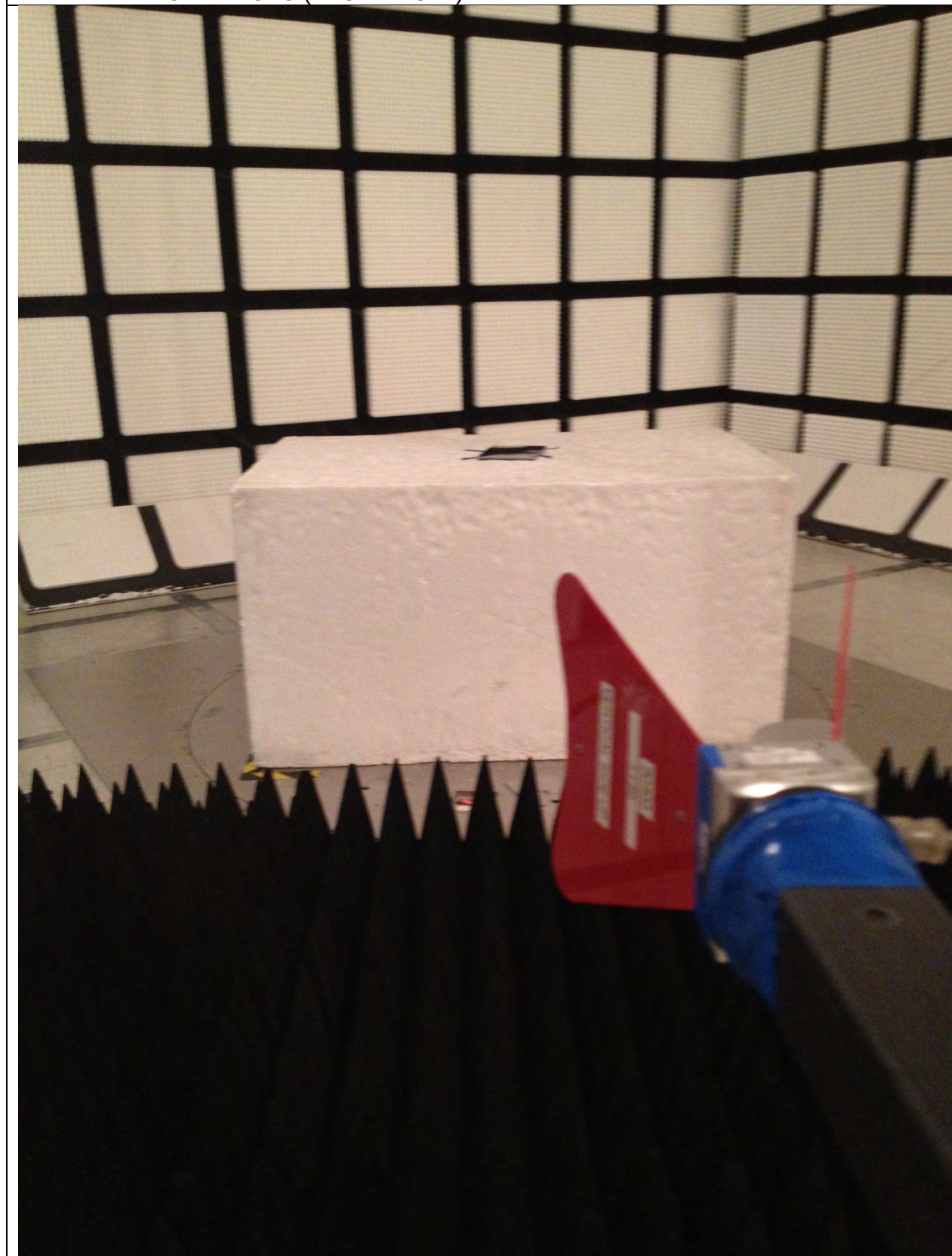
RADIATED FRONT PHOTO (ABOVE 1 GHz)
