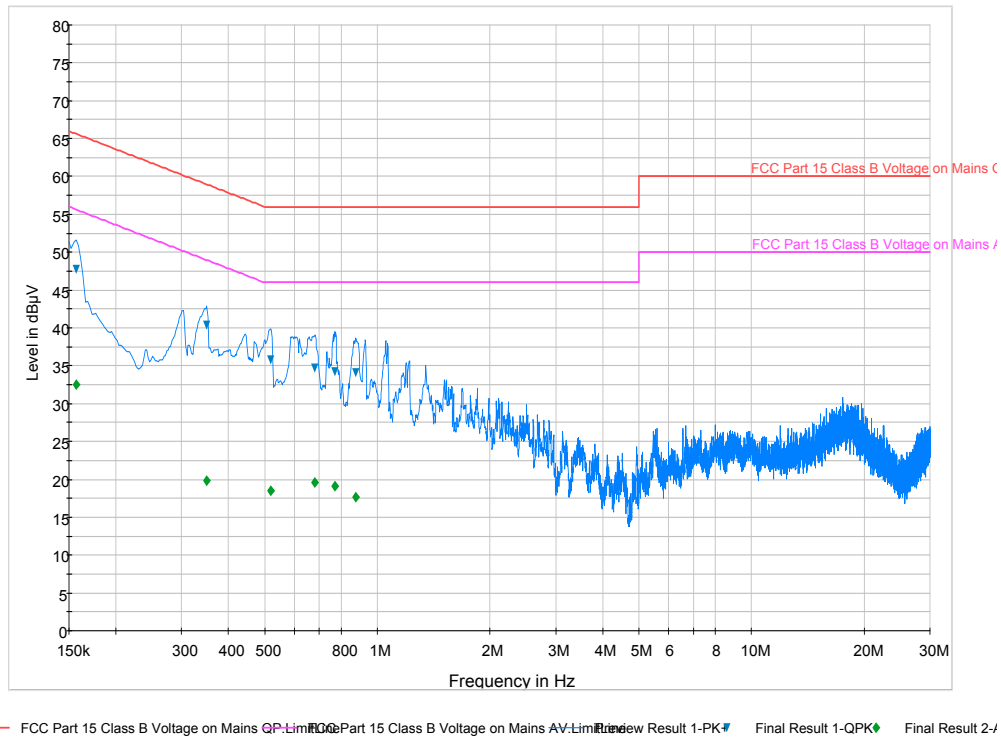
Plot 7-2. Line Conducted Plot (LN)
