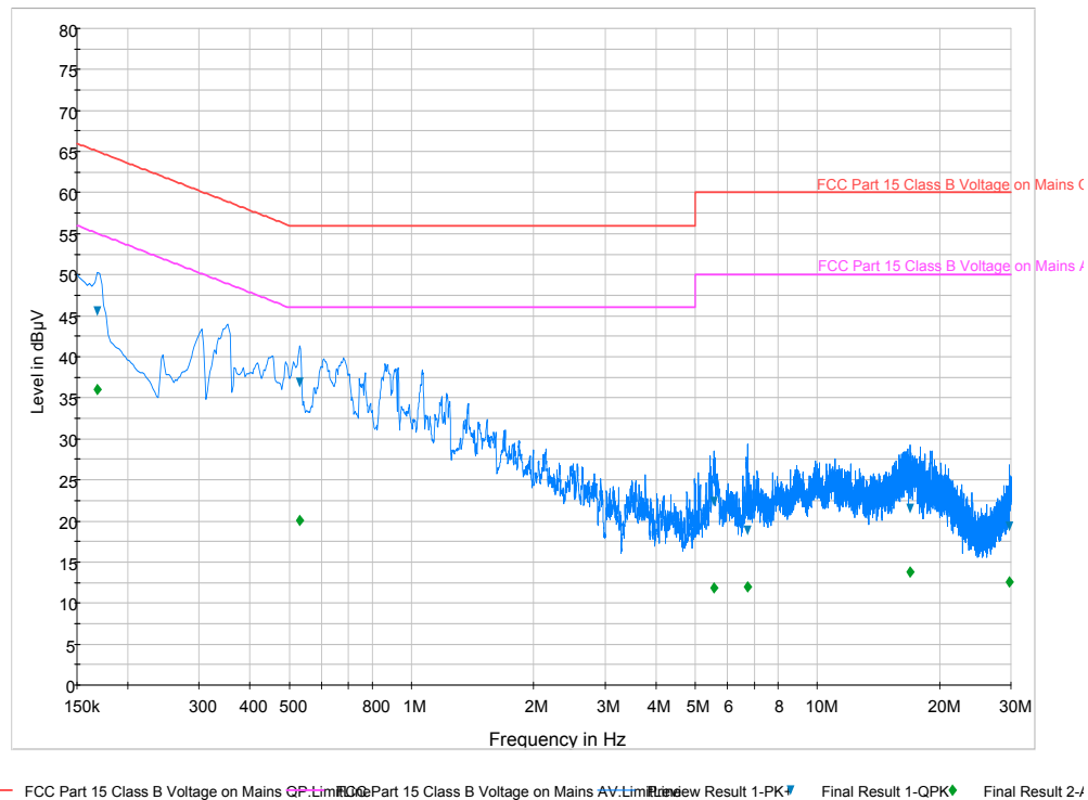
Plot 7-1. Line Conducted Plot (L1)
