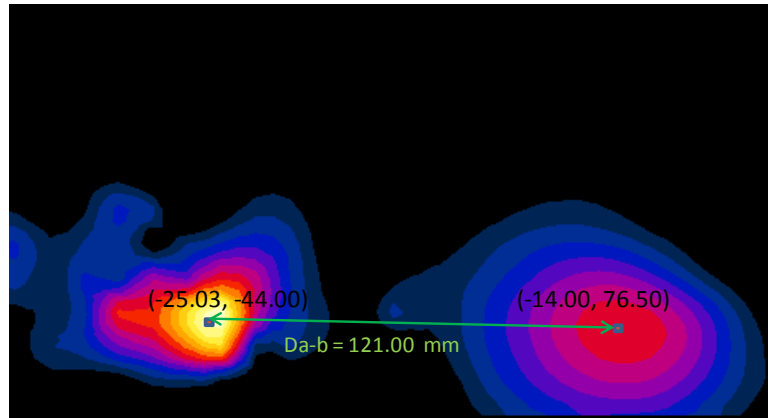
Figure 11-25 Peak SAR Locations of 5 GHz WLAN Ant. 2 and UMTS 1900 at 20 mm
