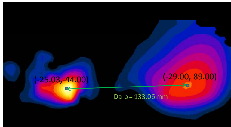
Figure 11-19 Peak SAR Locations of 5 GHz WLAN Ant. 2 and LTE Band 5 at 0 mm
