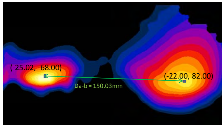
Figure 11-12 Peak SAR Locations of 5 GHz WLAN Ant. 1 and UMTS 850 at 0 mm
