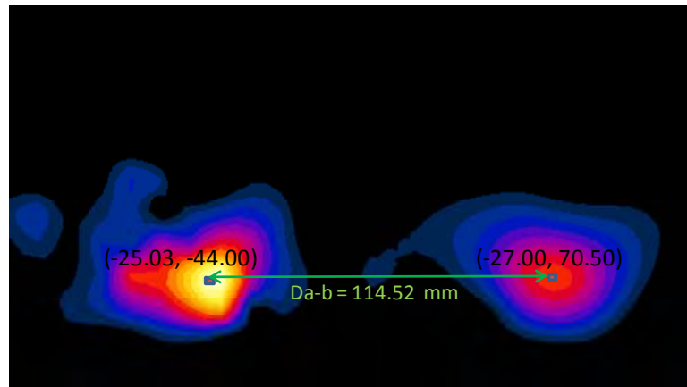
Figure 11-21 Peak SAR Locations of 5 GHz WLAN Ant. 2 and LTE Band 2 at 0 mm
