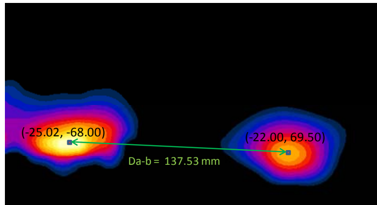
Figure 11-15 Peak SAR Locations of 5 GHz WLAN Ant. 1 and LTE Band 4 at 0 mm
