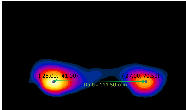
Figure 11-11 Peak SAR Locations of 2.4 GHz WLAN Ant. 2 and LTE Band 2 at 0 mm
