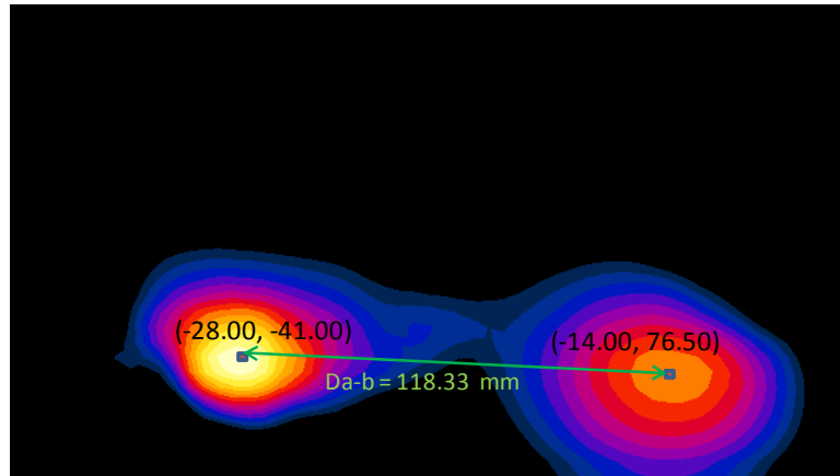
Figure 11-23 Peak SAR Locations of 2.4 GHz WLAN Ant. 2 and UMTS 1900 at 20 mm
