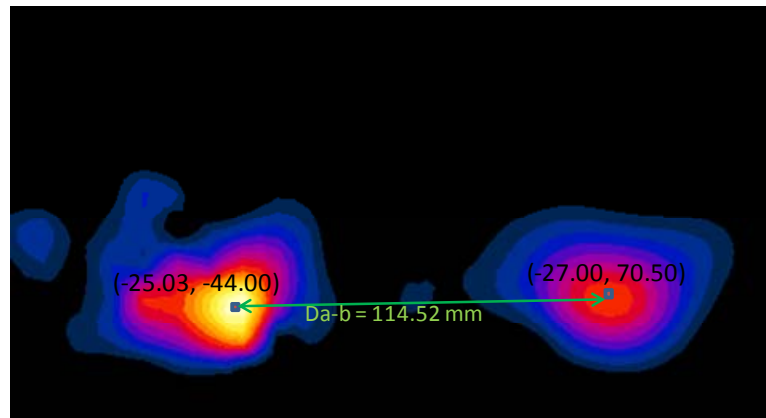
Figure 11-17 Peak SAR Locations of 5 GHz WLAN Ant. 2 and UMTS 1900 at 0 mm
