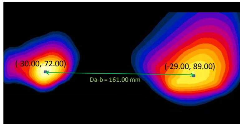
Figure 11-3 Peak SAR Locations of 2.4 GHz WLAN Ant. 1 and LTE Band 5 at 0 mm
