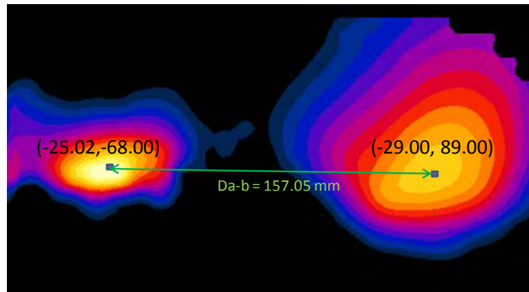
Figure 11-14 Peak SAR Locations of 5 GHz WLAN Ant. 1 and LTE Band 5 at 0 mm
