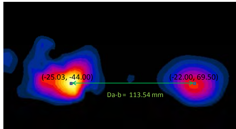
Figure 11-20 Peak SAR Locations of 5 GHz WLAN Ant. 2 and LTE Band 4 at 0 mm
