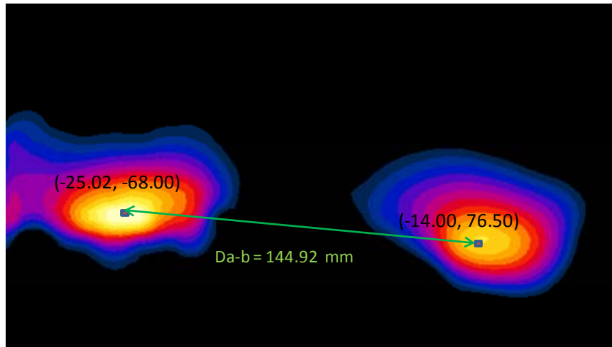
Figure 11-24 Peak SAR Locations of 5 GHz WLAN Ant. 1 and UMTS 1900 at 20 mm
