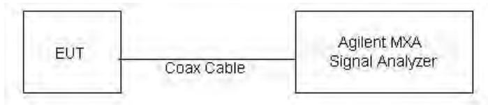
Figure 8-4 Power Measurement Setup for Bandwidths > 50 MHz
