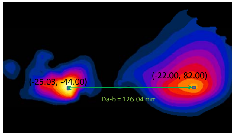
Figure 11-16 Peak SAR Locations of 5 GHz WLAN Ant. 2 and UMTS 850 at 0 mm
