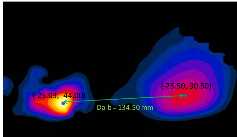
Figure 11-18 Peak SAR Locations of 5 GHz WLAN Ant. 2 and LTE Band 17 at 0 mm
