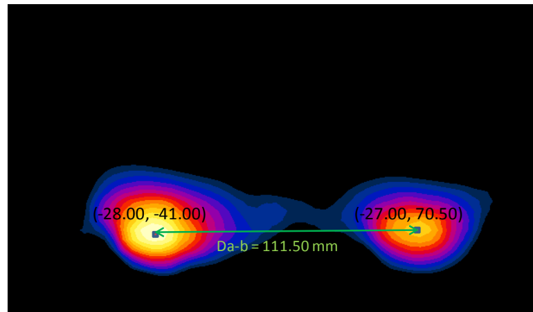
Figure 11-7 Peak SAR Locations of 2.4 GHz WLAN Ant. 2 and UMTS 1900 at 0 mm
