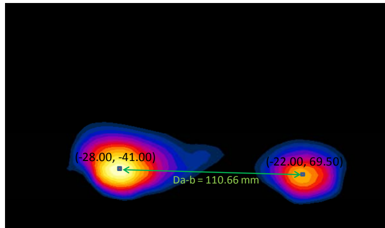
Figure 11-10 Peak SAR Locations of 2.4 GHz WLAN Ant. 2 and LTE Band 4 at 0 mm
