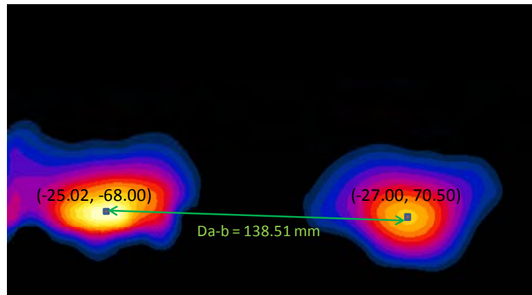
Figure 11-13 Peak SAR Locations of 5 GHz WLAN Ant. 1 and UMTS 1900 at 0 mm
