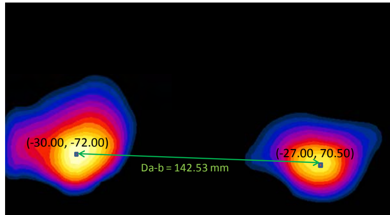
Figure 11-2 Peak SAR Locations of 2.4 GHz WLAN Ant. 1 and UMTS 1900 at 0 mm
