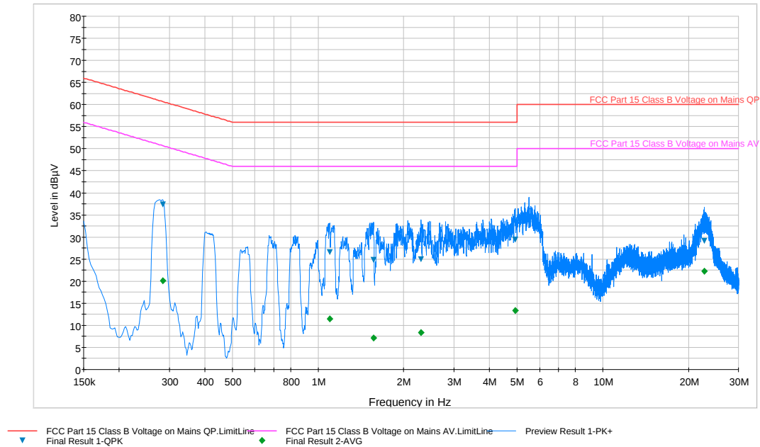
Plot 6-193. Line Conducted Plot with 802.11a UNII Band 2A (L1)
