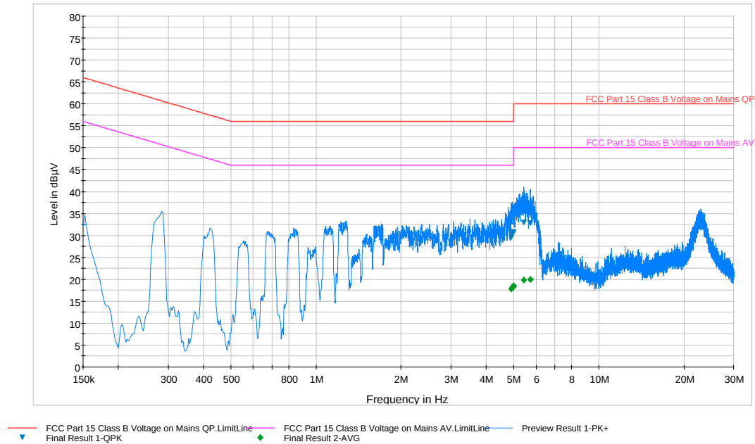
Plot 6-194. Line Conducted Plot with 802.11a UNII Band 2A (N)
