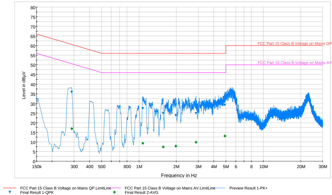
Plot 6-195. Line Conducted Plot with 802.11a UNII Band 2C (L1)
