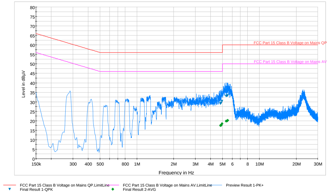
Plot 6-196. Line Conducted Plot with 802.11a UNII Band 2C (N)
