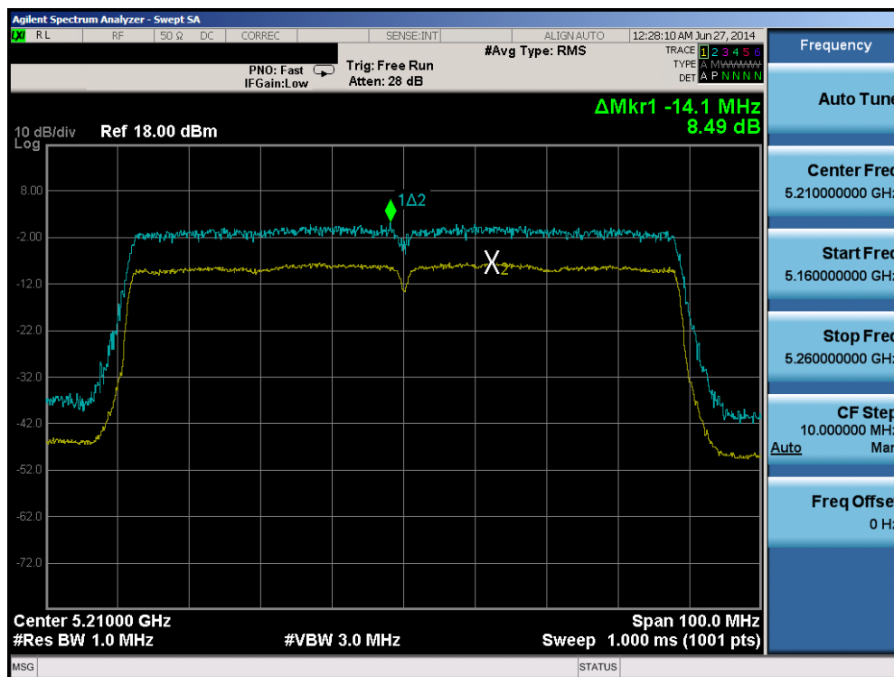
Plot 6-124. Peak Excursion Ratio Plot (80MHz BW 802.11ac (UNII Band 1) – Ch. 42)
