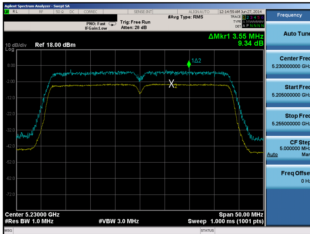
Plot 6-123. Peak Excursion Ratio Plot (40MHz BW 802.11n (UNII Band 1) – Ch. 46)
