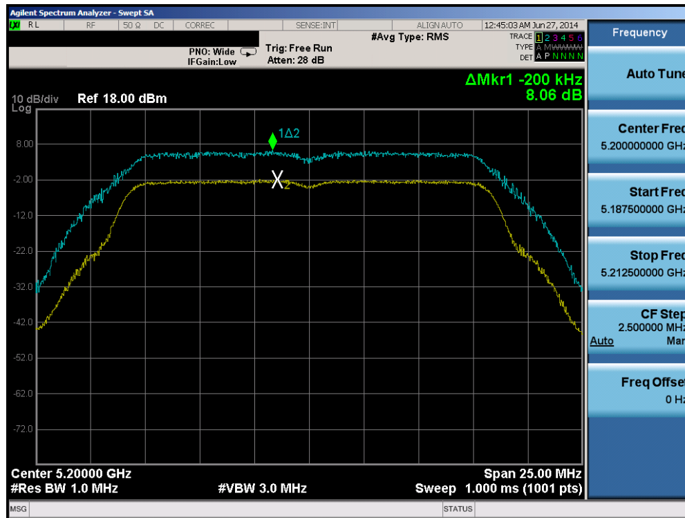
Plot 6-127. Peak Excursion Ratio Plot (802.11a (UNII Band 1) – Ch. 40)
