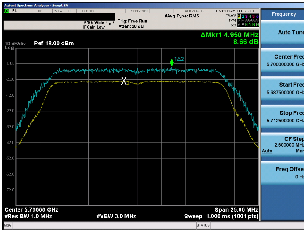
Plot 6-130. Peak Excursion Ratio Plot (20MHz BW 802.11n (UNII Band 2C) – Ch. 140)
