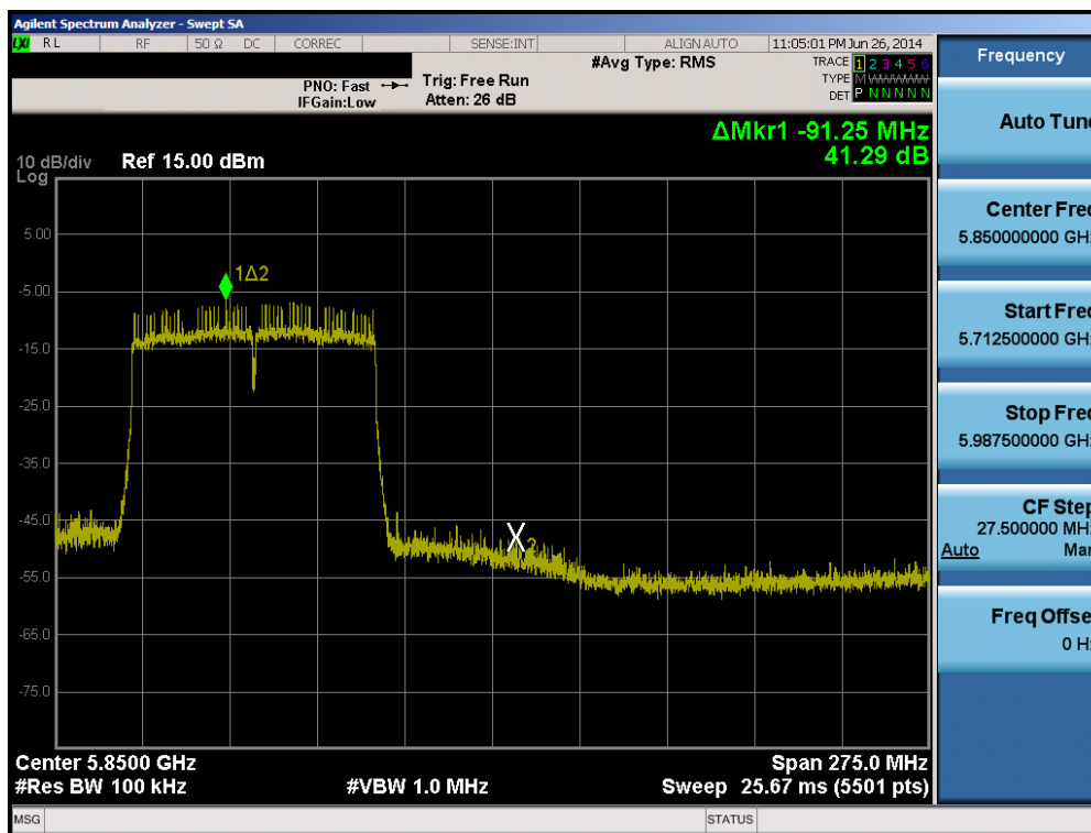
Plot 6-86. Band Edge Plot (80MHz BW 802.11ac (5.8GHz) – Ch. 155)
