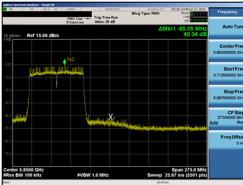
Plot 6-100. Band Edge Plot (80MHz BW 802.11ac (5.8GHz) – Ch. 155)
