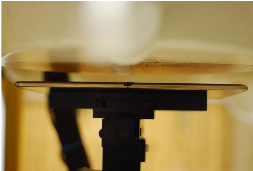
SAR Test Setup Photo 2: Back at 2.1 cm
