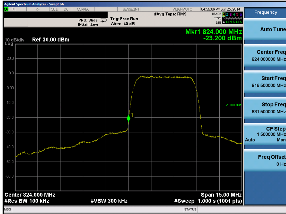
Plot 6-22. Band Edge Plot (Cellular WCDMA Mode – Ch. 4132)
