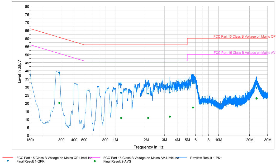
Plot 6-6. Line-Conducted Test Plot (L1)
