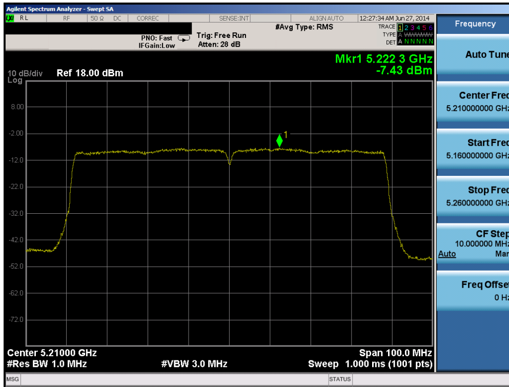
Plot 6-75. Peak Power Spectral Density Plot (80MHz BW 802.11ac (UNII Band 1) – Ch. 42)
