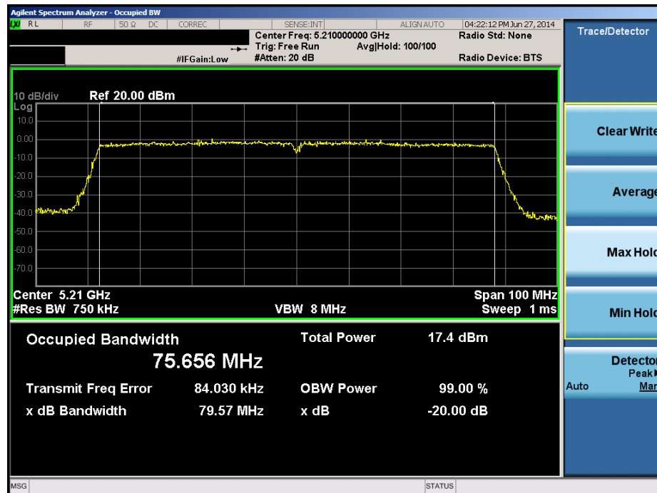
Plot 6-66. 20dB Bandwidth Plot (80MHz BW 802.11a/c (UNII Band 1) – Ch. 42)
