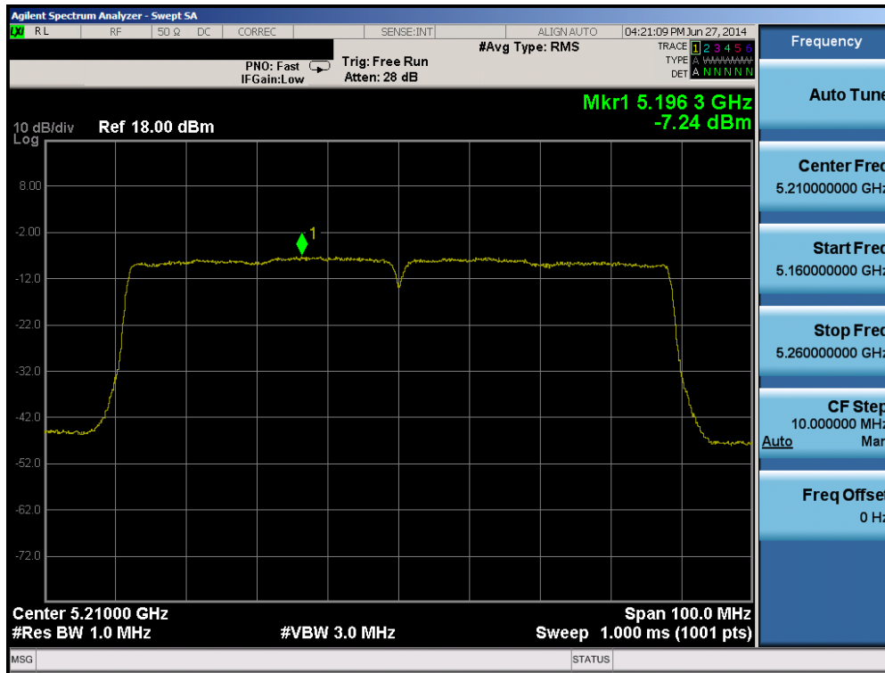
Plot 6-103. Peak Power Spectral Density Plot (80MHz BW 802.11ac (UNII Band 1) – Ch. 42)
