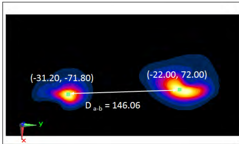
Figure 11-1 Peak SAR Locations for Body Back Side at 0 mm UMTS 850 MHz and 2.4 GHz WLAN Antenna 1
