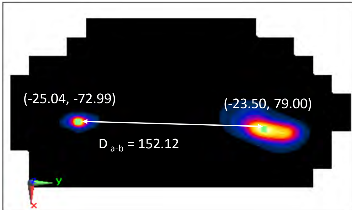
Figure 11-8 Peak SAR Locations for Body Back Side at 0 mm LTE Band 2 and 5 GHz WLAN Antenna 1
