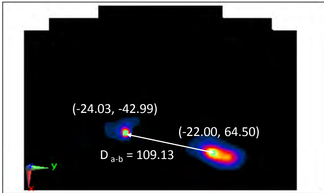
Figure 11-10 Peak SAR Locations for Body Back Side at 0 mm LTE Band 4 and 5 GHz WLAN Antenna 2
