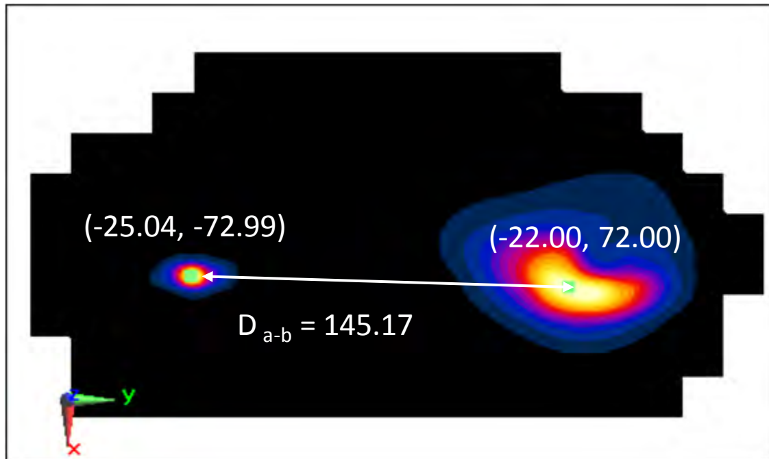
Figure 11-6 Peak SAR Locations for Body Back Side at 0 mm UMTS 850 MHz and 5 GHz WLAN Antenna 1
