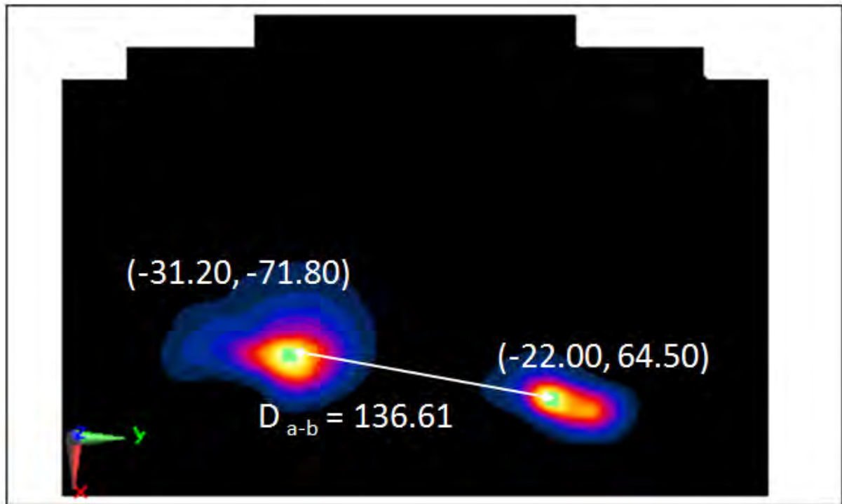
Figure 11-2 Peak SAR Locations for Body Back Side at 0 mm LTE B4 and 2.4 GHz WLAN Antenna 1
