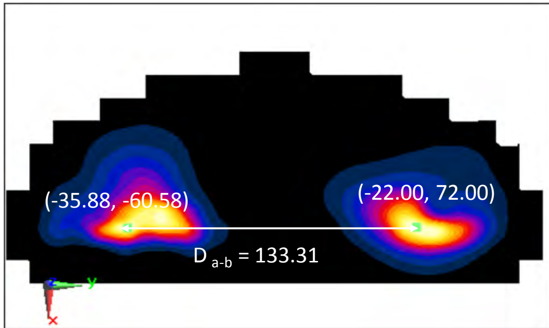
Figure 11-3 Peak SAR Locations for Body Back Side at 0 mm UMTS 850 MHz and 2.4 GHz WLAN MIMO
