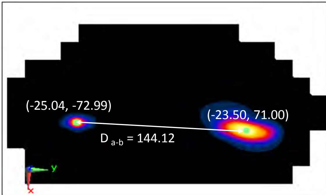
Figure 11-5 Peak SAR Locations for Body Back Side at 0 mm GPRS 1900 MHz and 5 GHz WLAN Antenna 1
