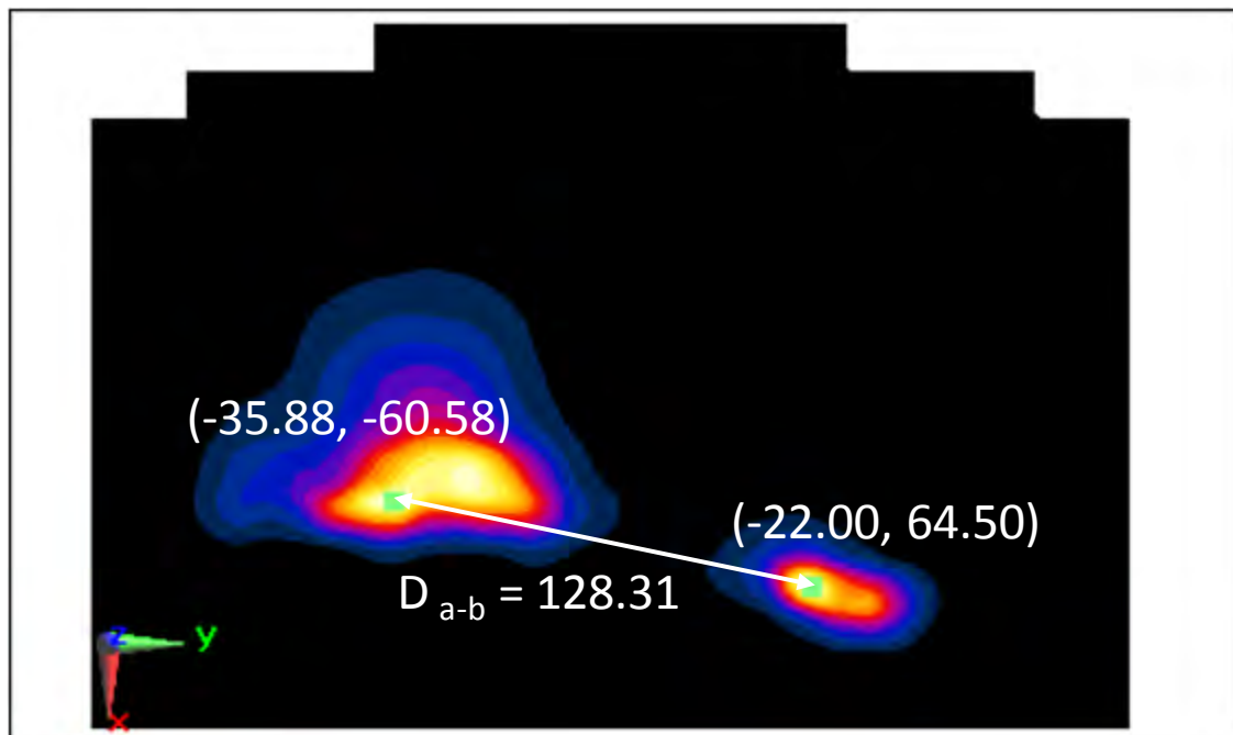
Figure 11-4 Peak SAR Locations for Body Back Side at 0 mm LTE Band 4 and 2.4 GHz WLAN MIMO
