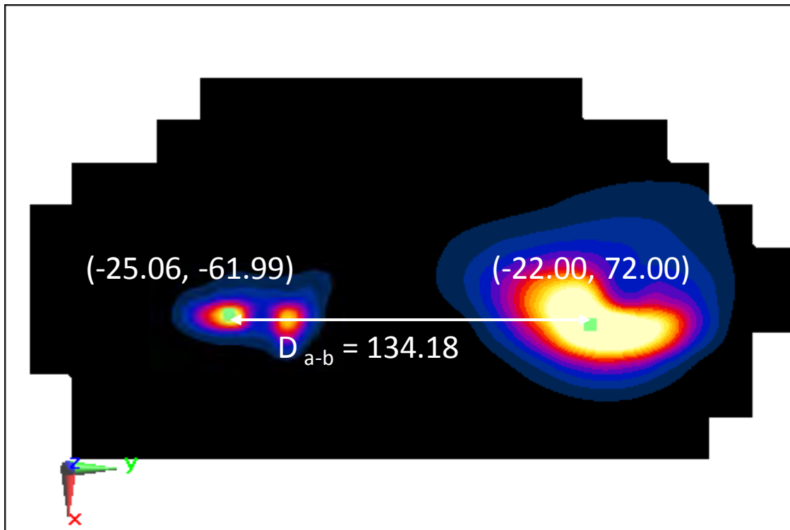
Figure 11-11 Peak SAR Locations for Body Back Side at 0 mm UMTS 850 MHz and 5 GHz WLAN MIMO
