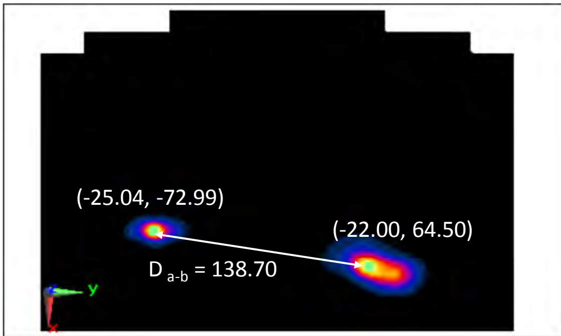
Figure 11-7 Peak SAR Locations for Body Back Side at 0 mm LTE Band 4 and 5 GHz WLAN Antenna 1
