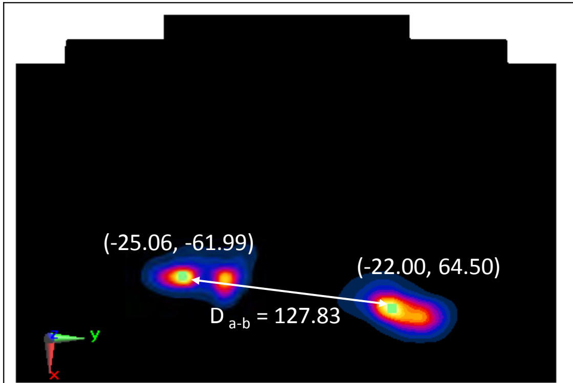
Figure 11-12 Peak SAR Locations for Body Back Side at 0 mm LTE Band 4 and 5 GHz WLAN MIMO
