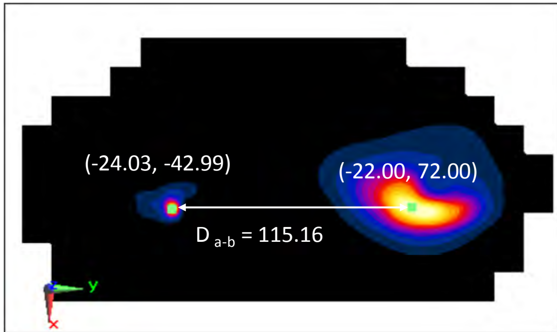
Figure 11-9 Peak SAR Locations for Body Back Side at 0 mm UMTS 850 MHz and 5 GHz WLAN Antenna 2
