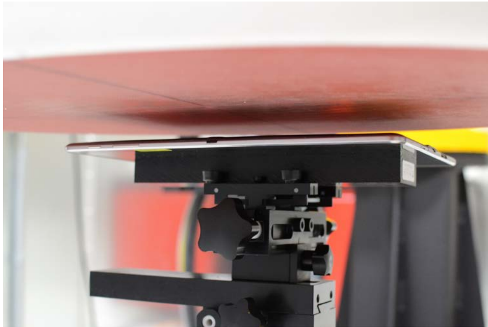
SAR Test Setup Photo 2: Back Side at 20 mm
