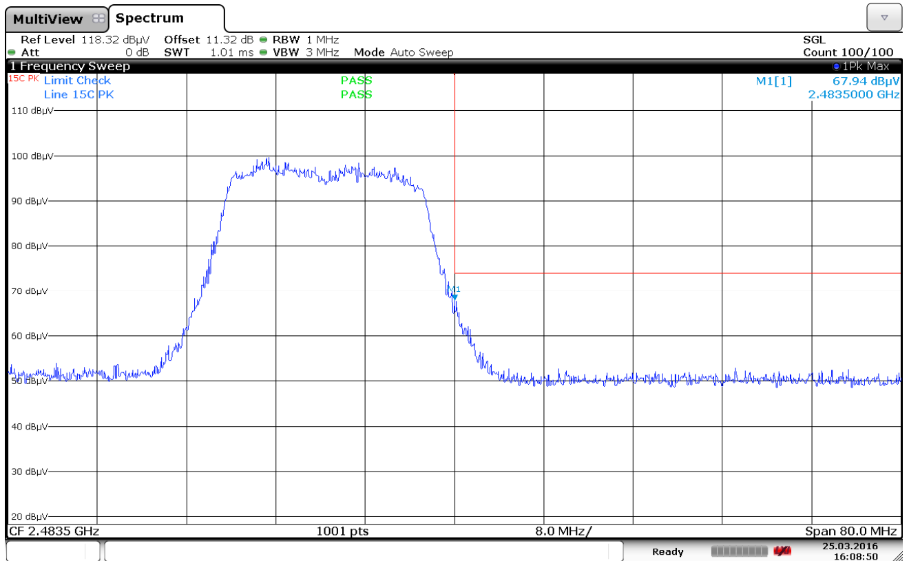
Plot 7-106. Radiated Restricted Upper Band Edge Measurement (Peak)
