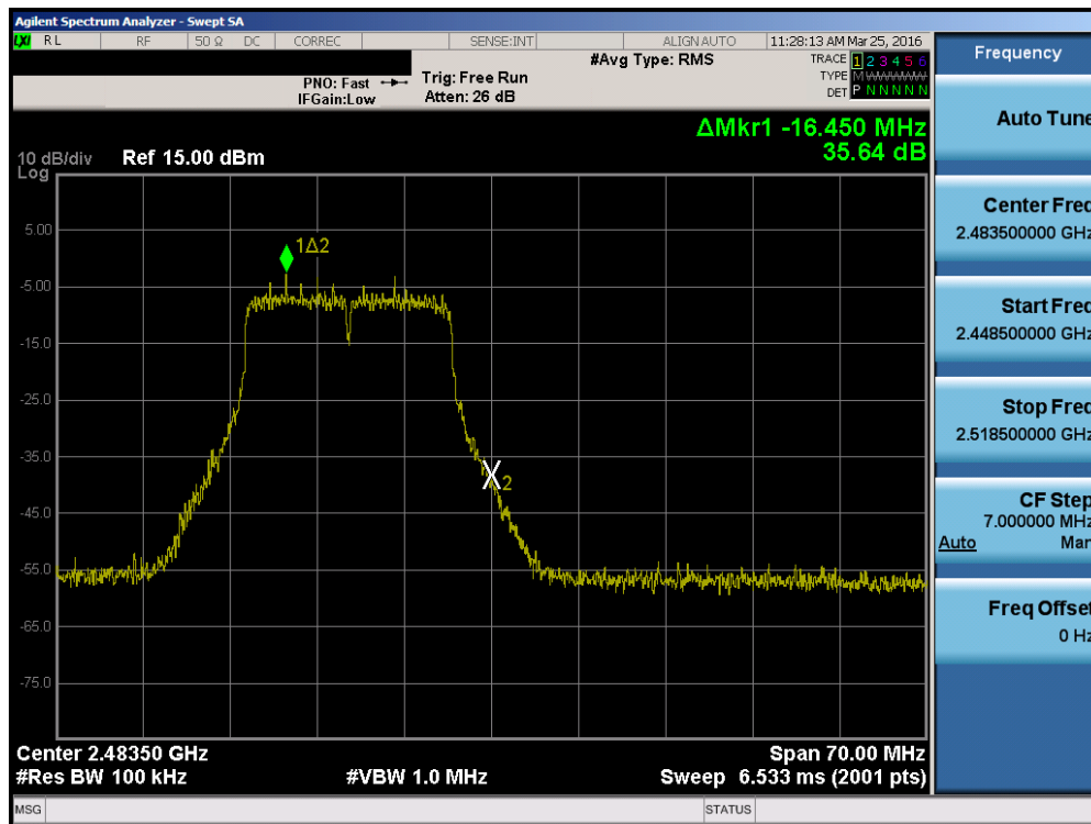
Plot 7-51. Band Edge Plot (802.11g – Ch. 13)
