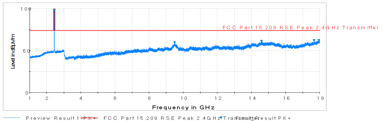
Plot 7-77. Radiated Spurious Plot above 1GHz (802.11b – Ch. 6, Ant. Pol. H)
