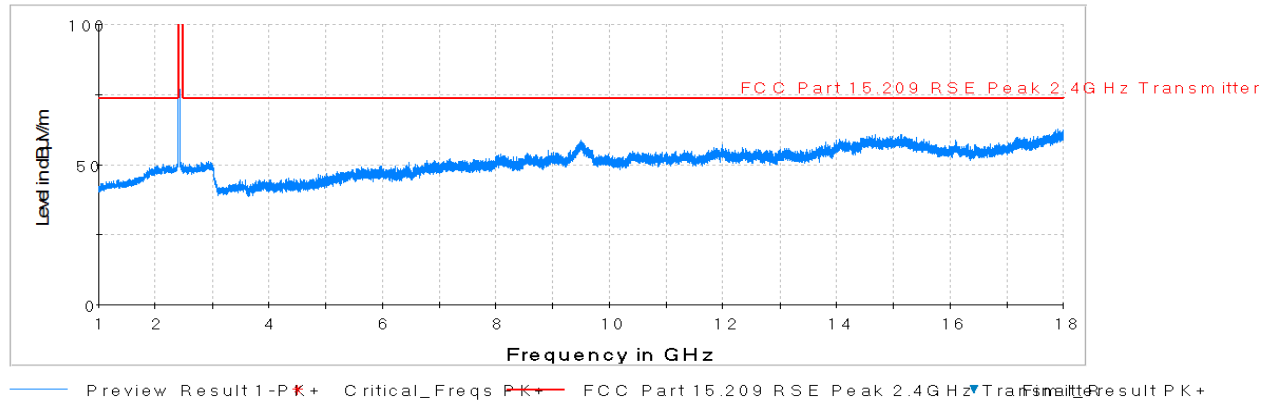
Plot 7-67. Radiated Spurious Plot above 1GHz (802.11b – Ch. 1, Ant. Pol. H)
