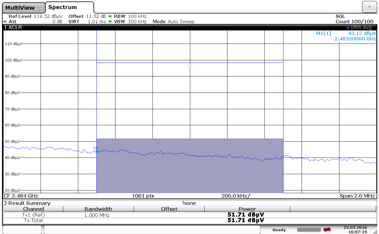
Plot 7-105. Radiated Restricted Upper Band Edge Measurement (Average)
