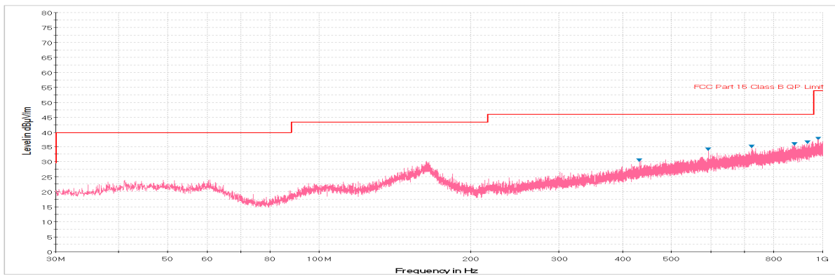
Plot 7-108. Radiated Spurious Plot below 1GHz (Pol. V)
