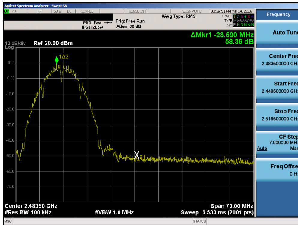
Plot 7-47. Band Edge Plot (802.11b – Ch. 11)
