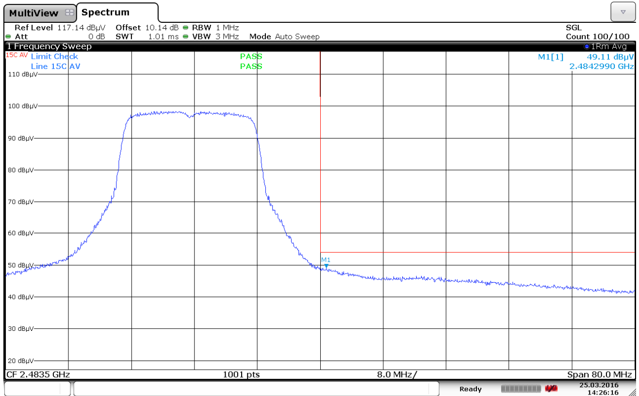
Plot 7-87. Radiated Restricted Upper Band Edge Measurement (Average)
