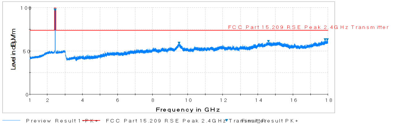
Plot 7-78. Radiated Spurious Plot above 1GHz (802.11b – Ch. 6, Ant. Pol. V)
