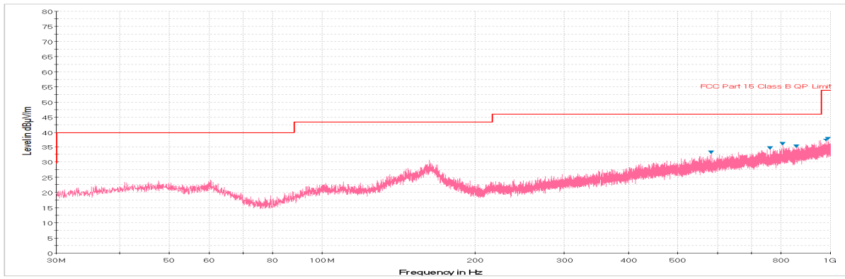
Plot 7-110. Radiated Spurious Plot below 1GHz (Pol. V)
