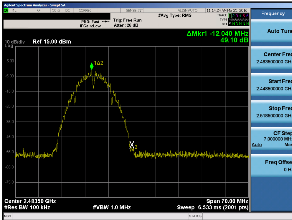
Plot 7-39. Band Edge Plot (802.11b – Ch. 13)
