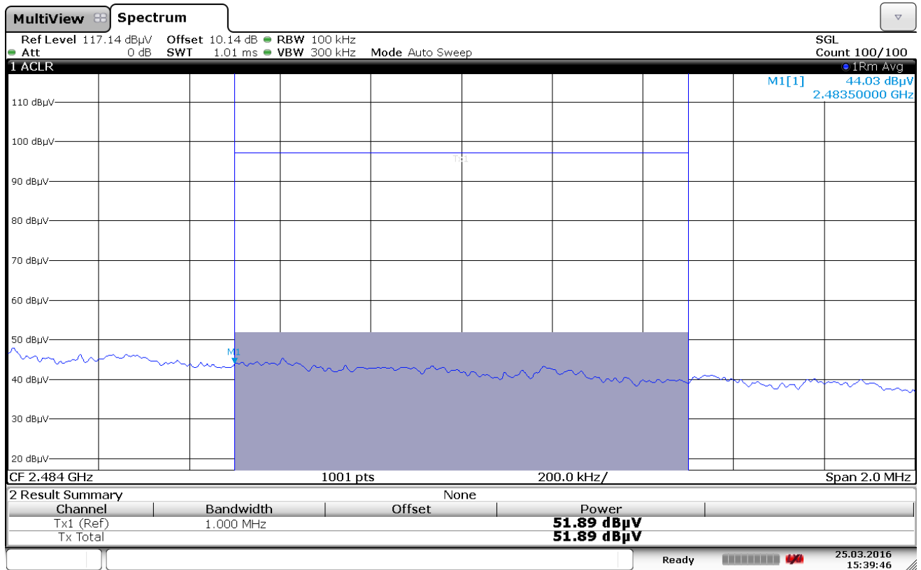
Plot 7-97. Radiated Restricted Upper Band Edge Measurement (Average)
