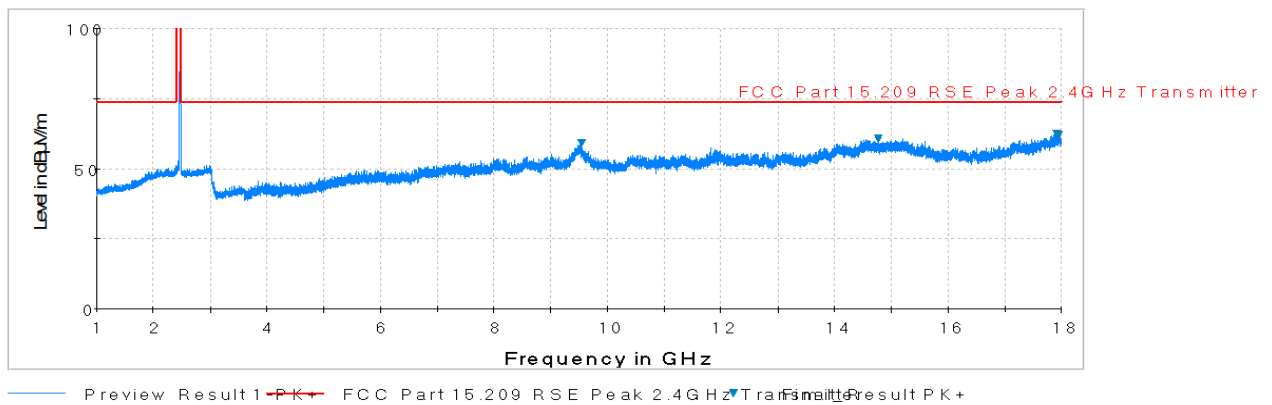
Plot 7-71. Radiated Spurious Plot above 1GHz (802.11b – Ch. 11, Ant. Pol. H)
