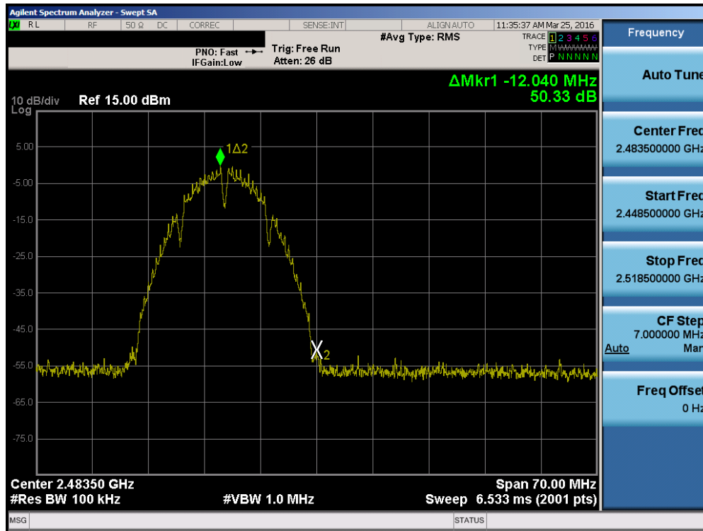
Plot 7-48. Band Edge Plot (802.11b – Ch. 13)
