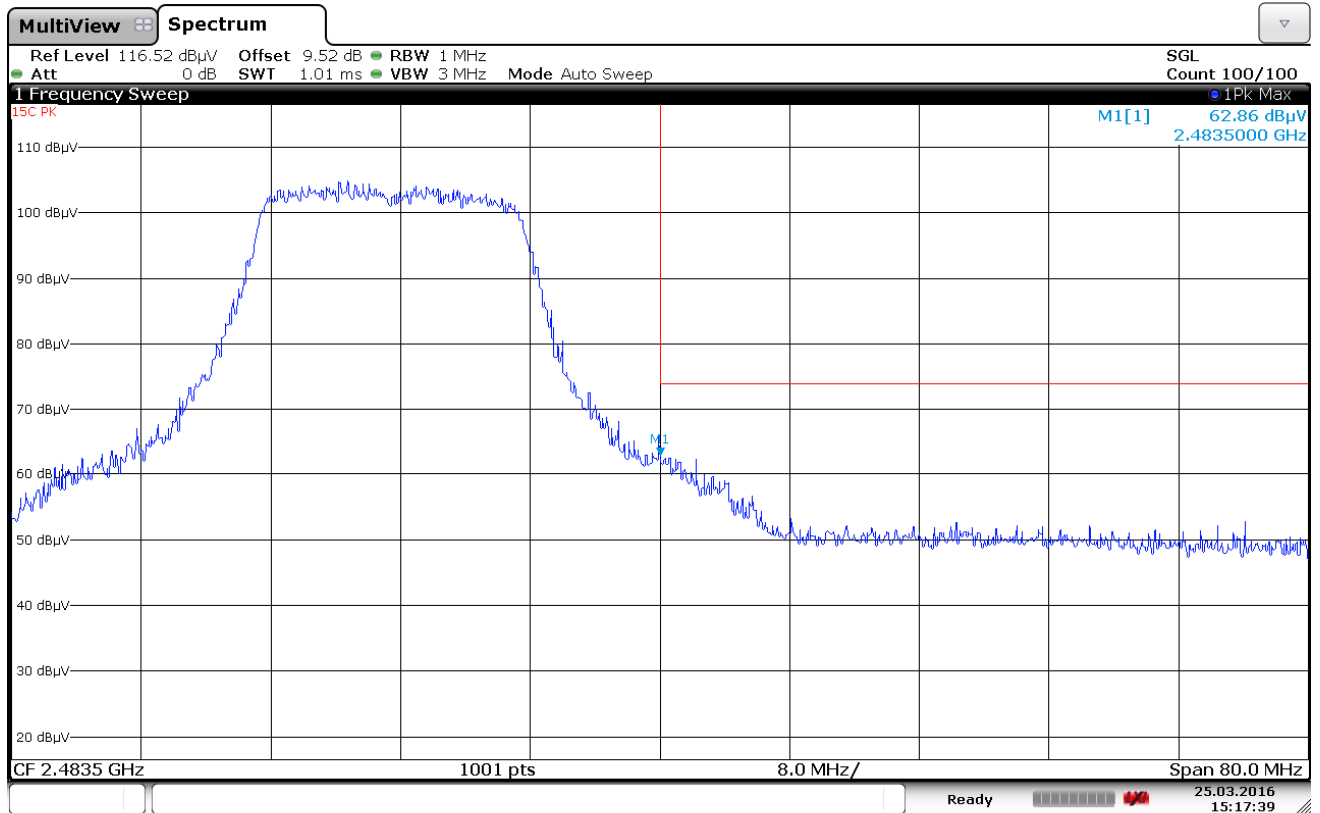
Plot 7-96. Radiated Restricted Upper Band Edge Measurement (Peak)
