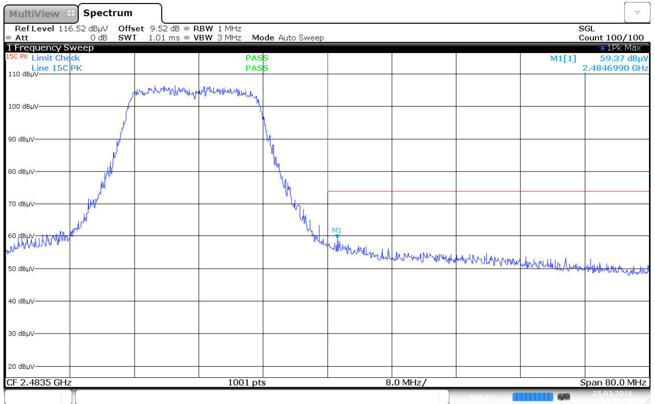
Plot 7-88. Radiated Restricted Upper Band Edge Measurement (Peak)
