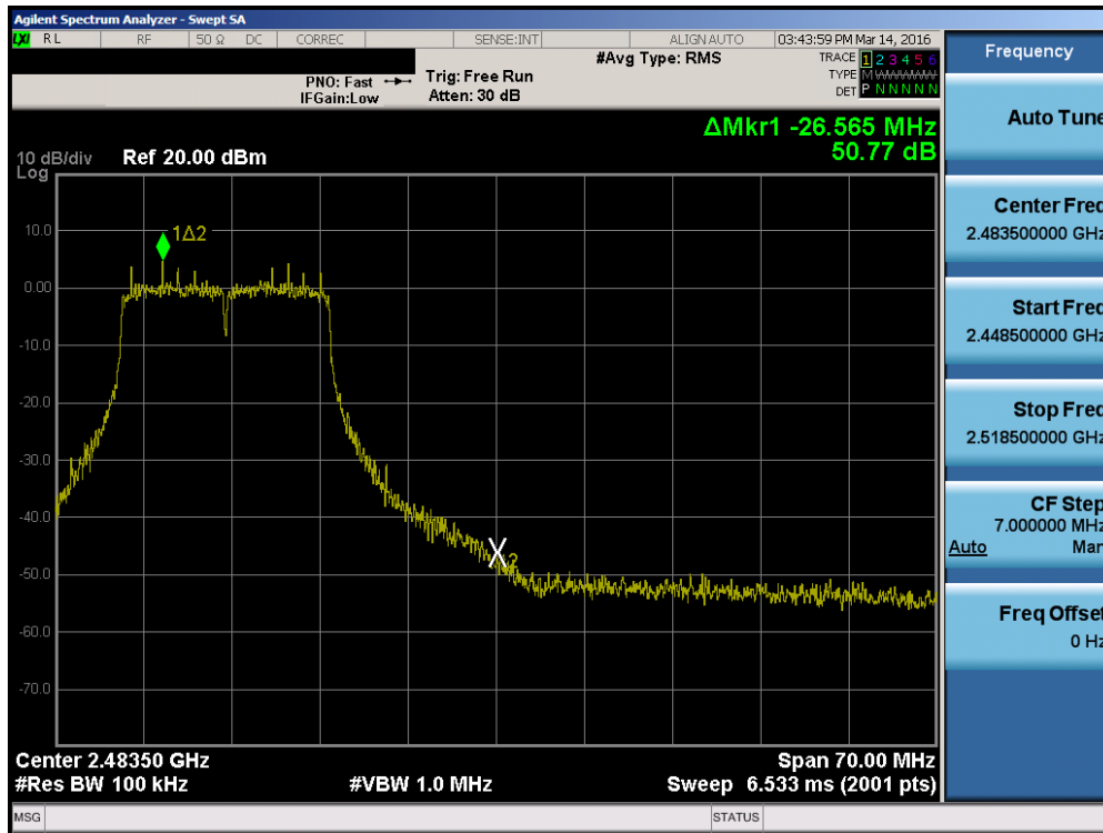
Plot 7-50. Band Edge Plot (802.11g – Ch. 11)
