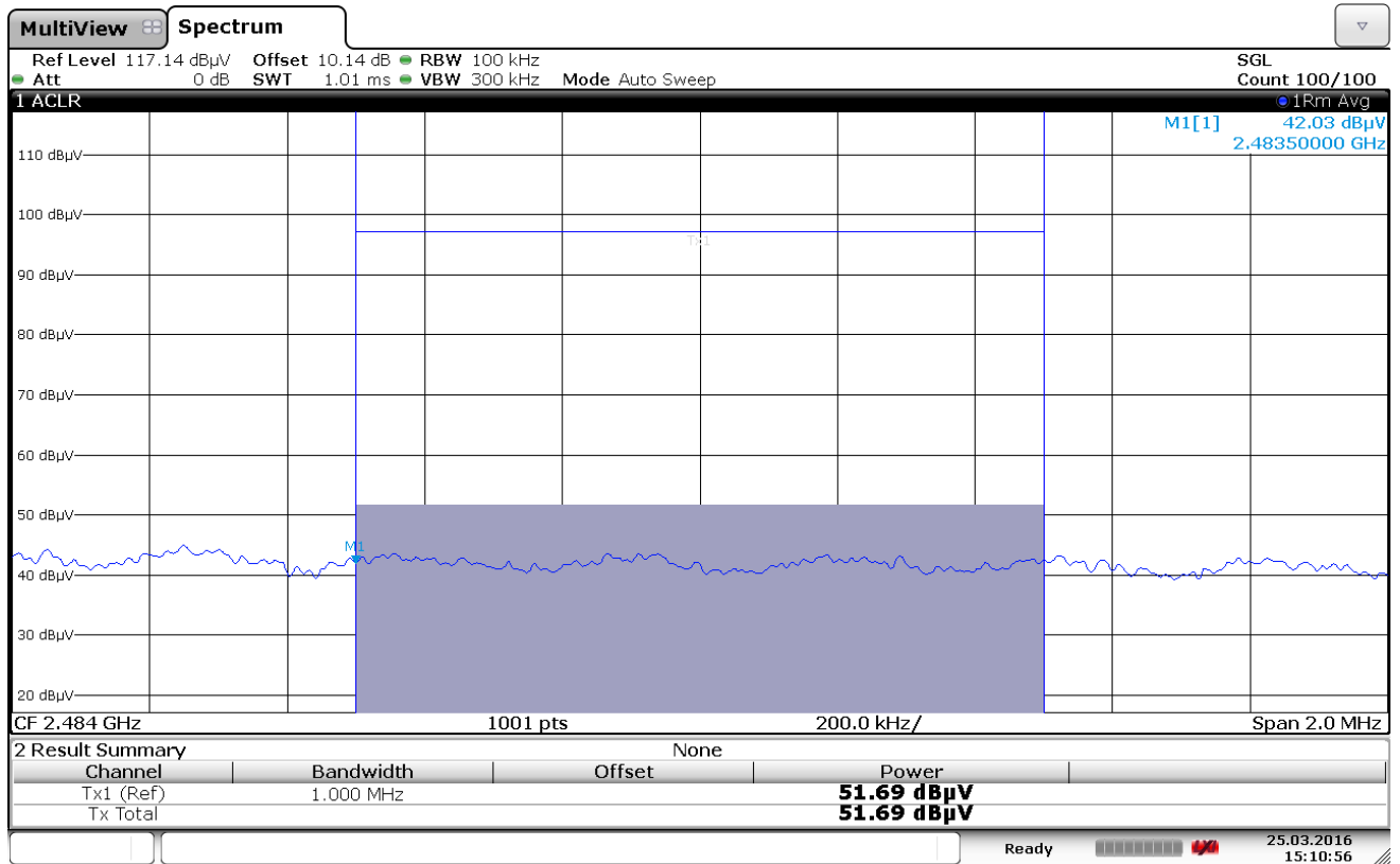
Plot 7-95. Radiated Restricted Upper Band Edge Measurement (Average)
