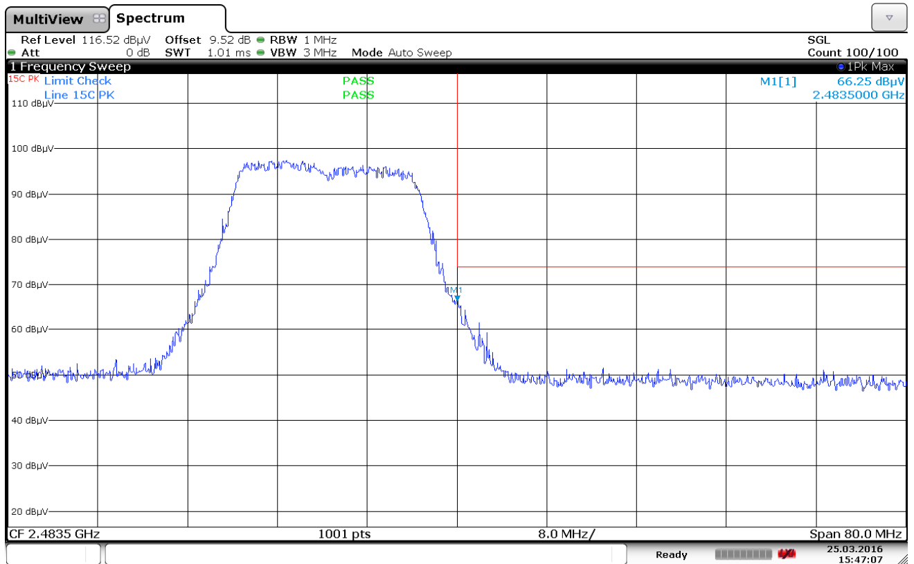
Plot 7-98. Radiated Restricted Upper Band Edge Measurement (Peak)
