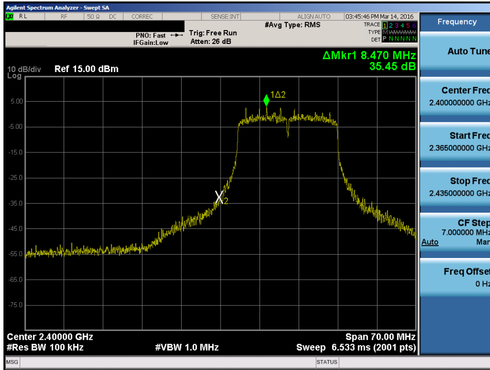
Plot 7-52. Band Edge Plot (802.11n (2.4GHz) – Ch. 1)
