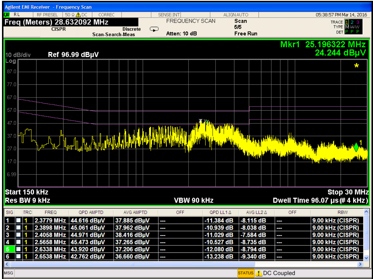
Plot 7-111. Line Conducted Plot with 802.11b (L1)
