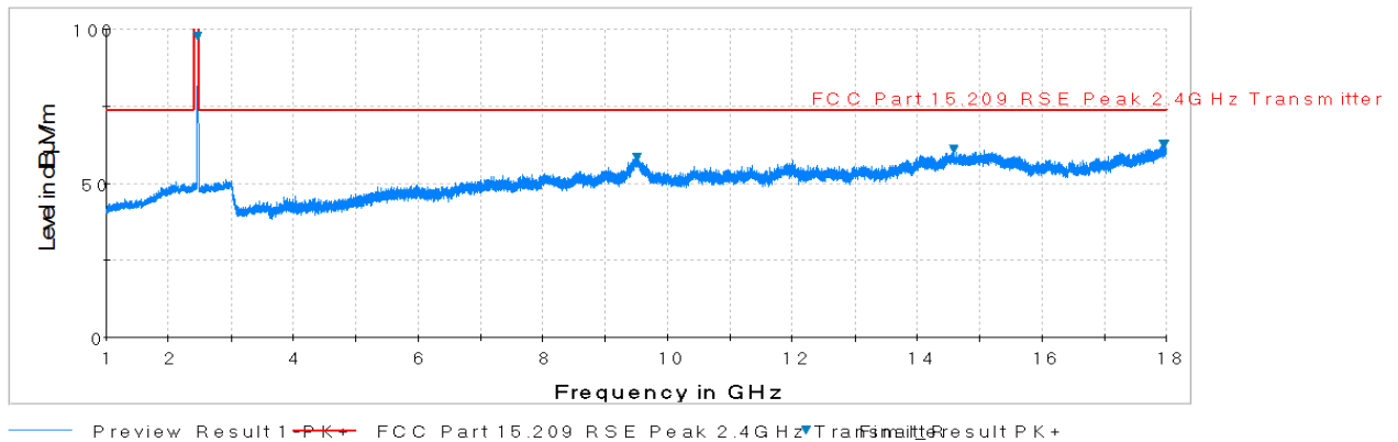
Plot 7-80. Radiated Spurious Plot above 1GHz (802.11b – Ch. 11, Ant. Pol. V)
