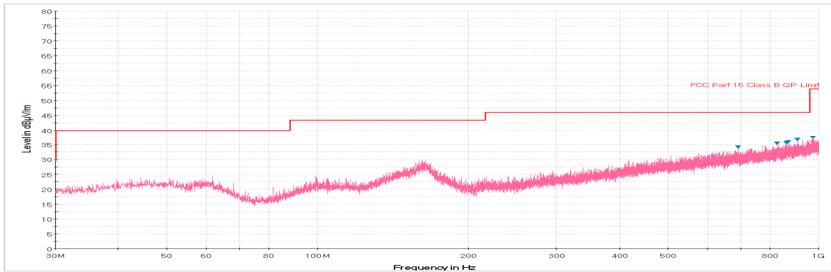
Plot 7-107. Radiated Spurious Plot below 1GHz (Pol. H)
