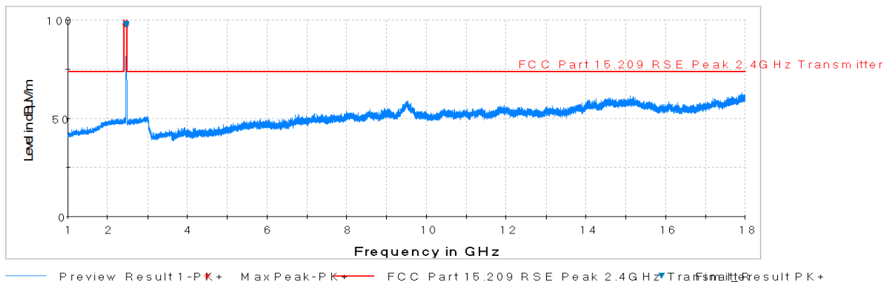
Plot 7-79. Radiated Spurious Plot above 1GHz (802.11b – Ch. 11, Ant. Pol. H)
