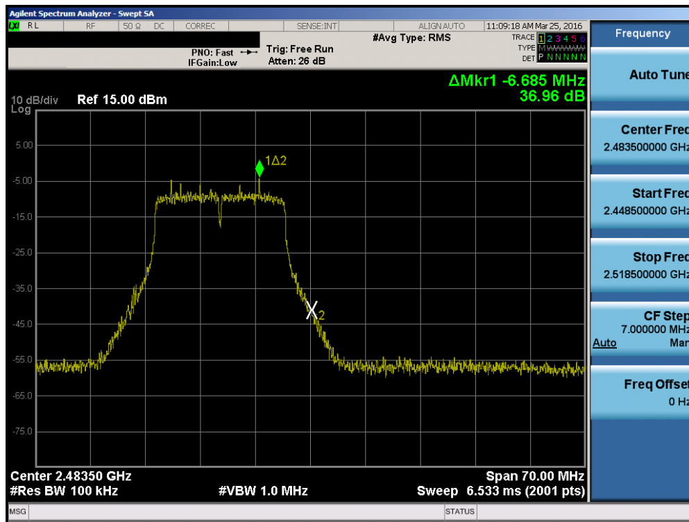
Plot 7-42. Band Edge Plot (802.11g – Ch. 13)
