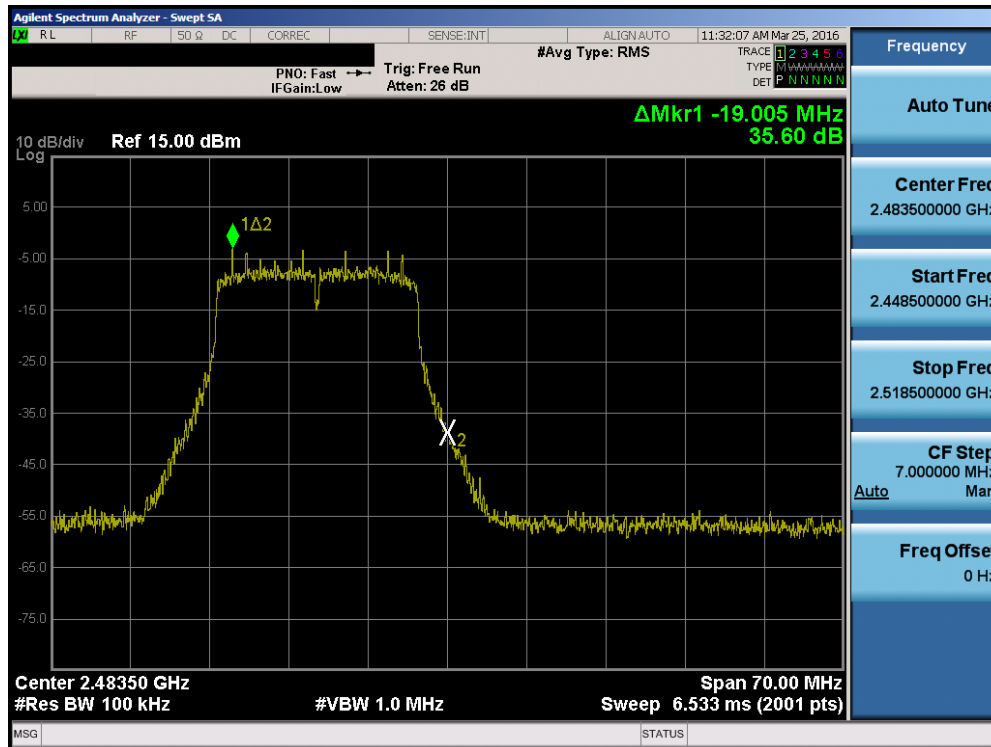
Plot 7-54. Band Edge Plot (802.11n (2.4GHz) – Ch. 13)
