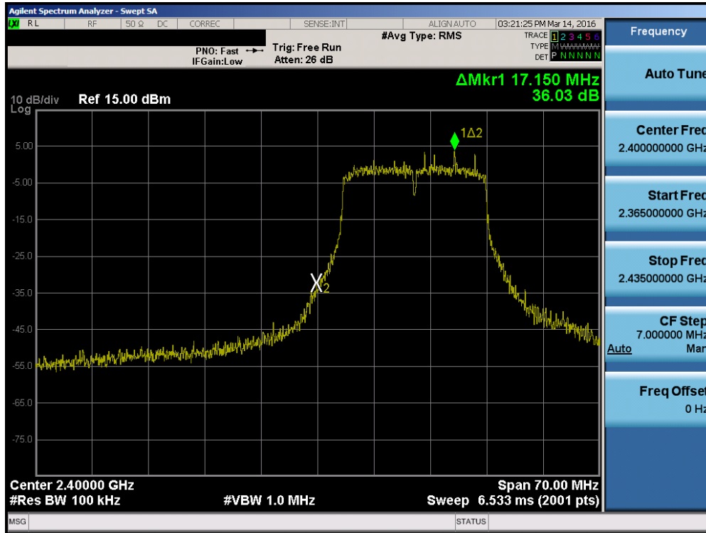
Plot 7-43. Band Edge Plot (802.11n (2.4GHz) – Ch. 1)
