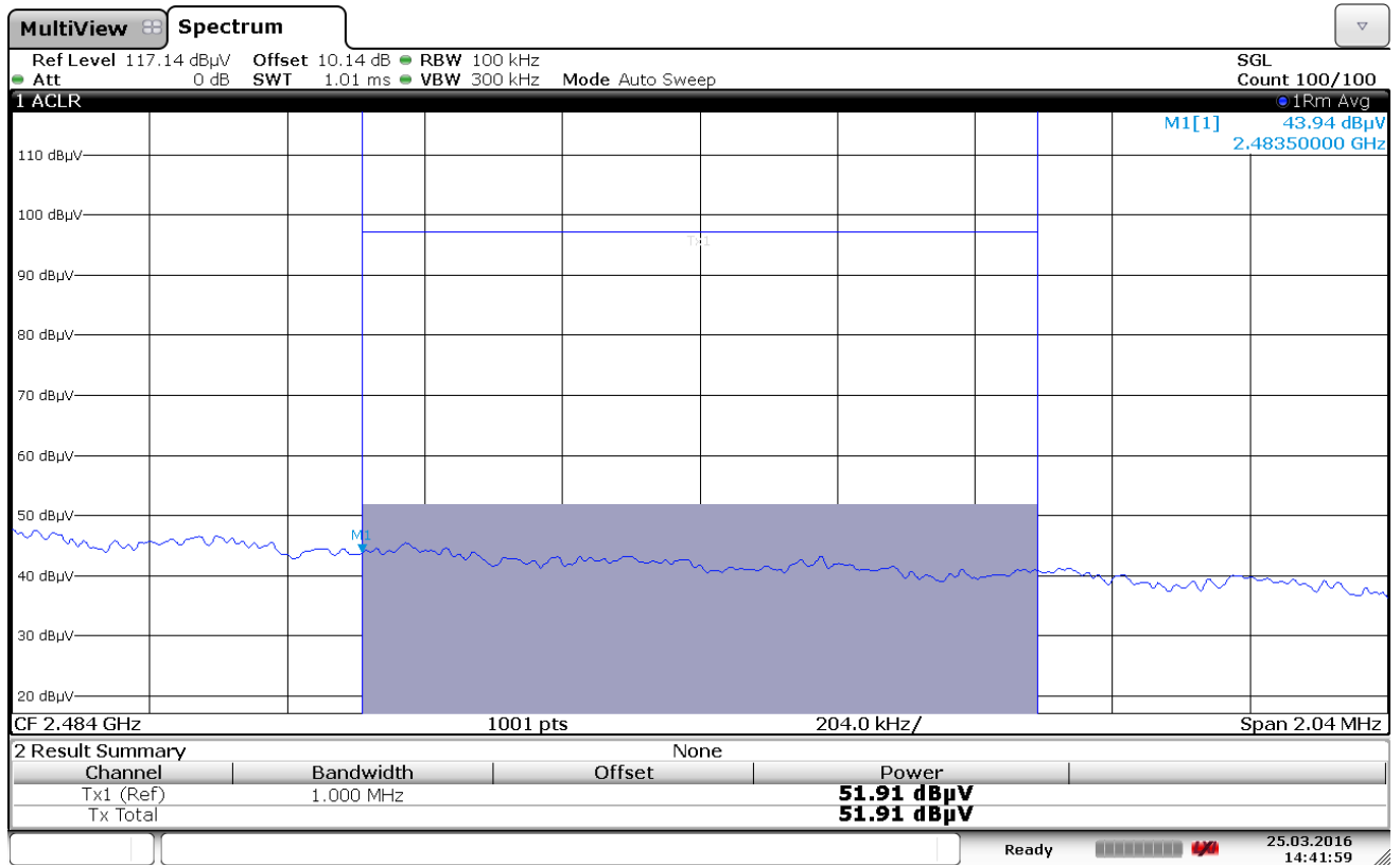
Plot 7-89. Radiated Restricted Upper Band Edge Measurement (Average)
