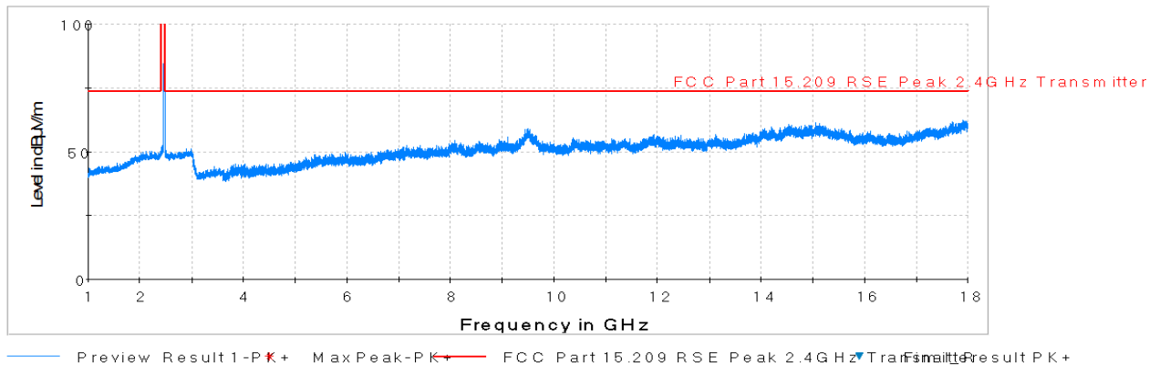
Plot 7-72. Radiated Spurious Plot above 1GHz (802.11b – Ch. 11, Ant. Pol. V)
