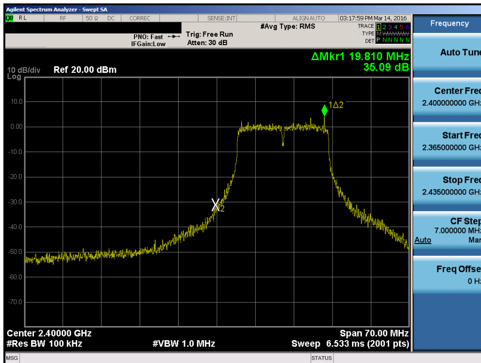
Plot 7-40. Band Edge Plot (802.11g– Ch. 1)
