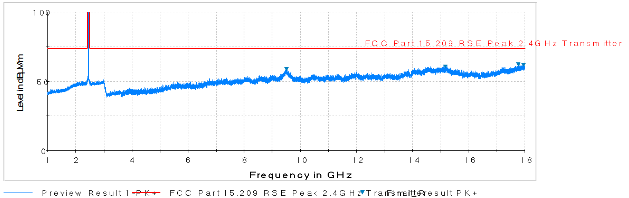
Plot 7-70. Radiated Spurious Plot above 1GHz (802.11b – Ch. 6, Ant. Pol. V)
