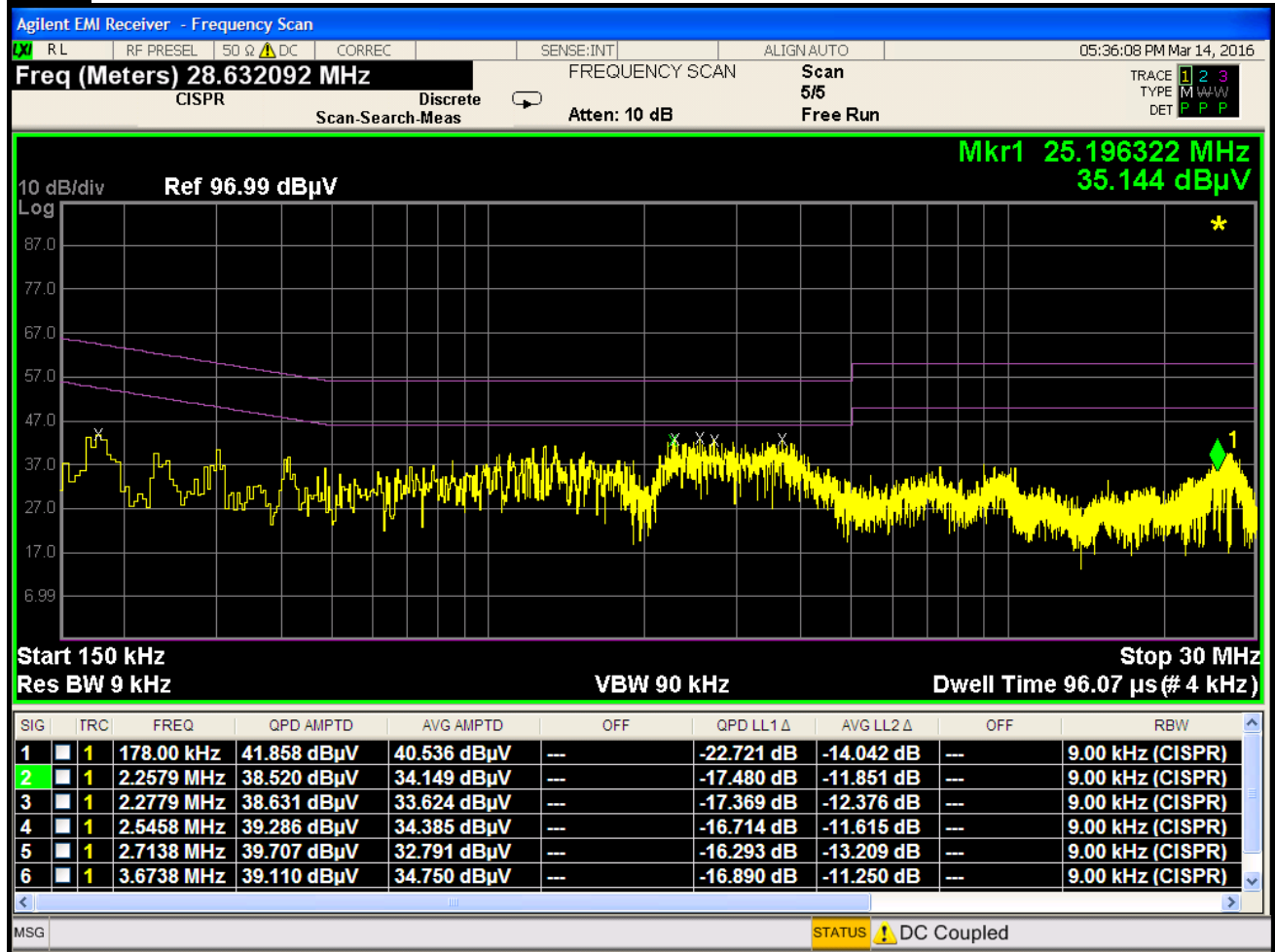
Plot 7-112. Line Conducted Plot with 802.11b (N)
