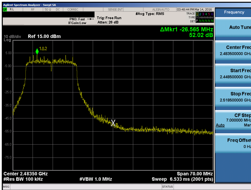
Plot 7-53. Band Edge Plot (802.11n (2.4GHz) – Ch. 11)
