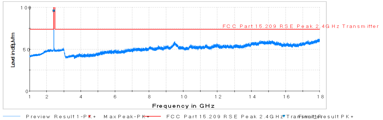
Plot 7-75. Radiated Spurious Plot above 1GHz (802.11b – Ch. 1, Ant. Pol. H)
