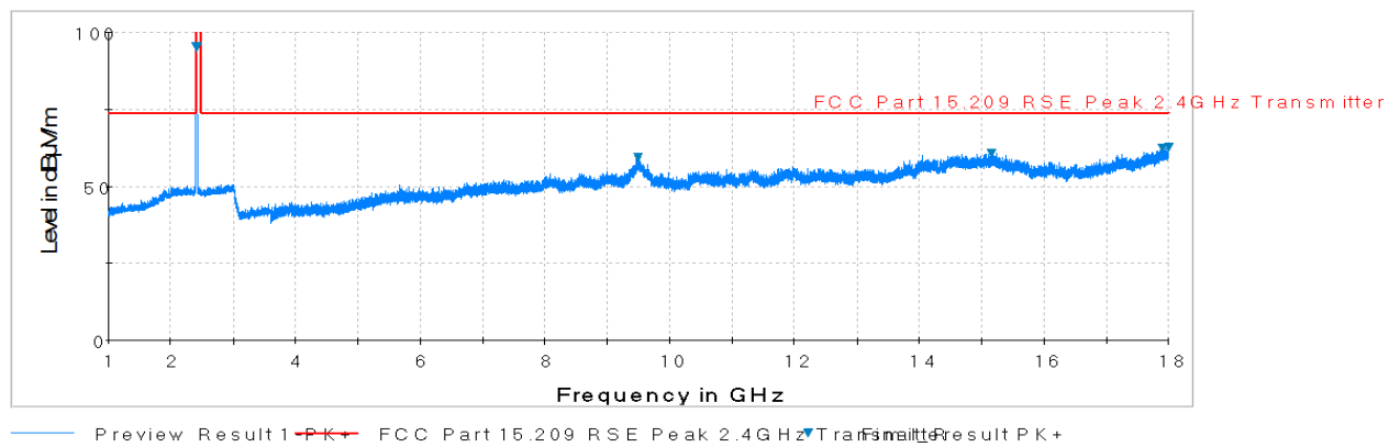
Plot 7-76. Radiated Spurious Plot above 1GHz (802.11b – Ch. 1, Ant. Pol. V)
