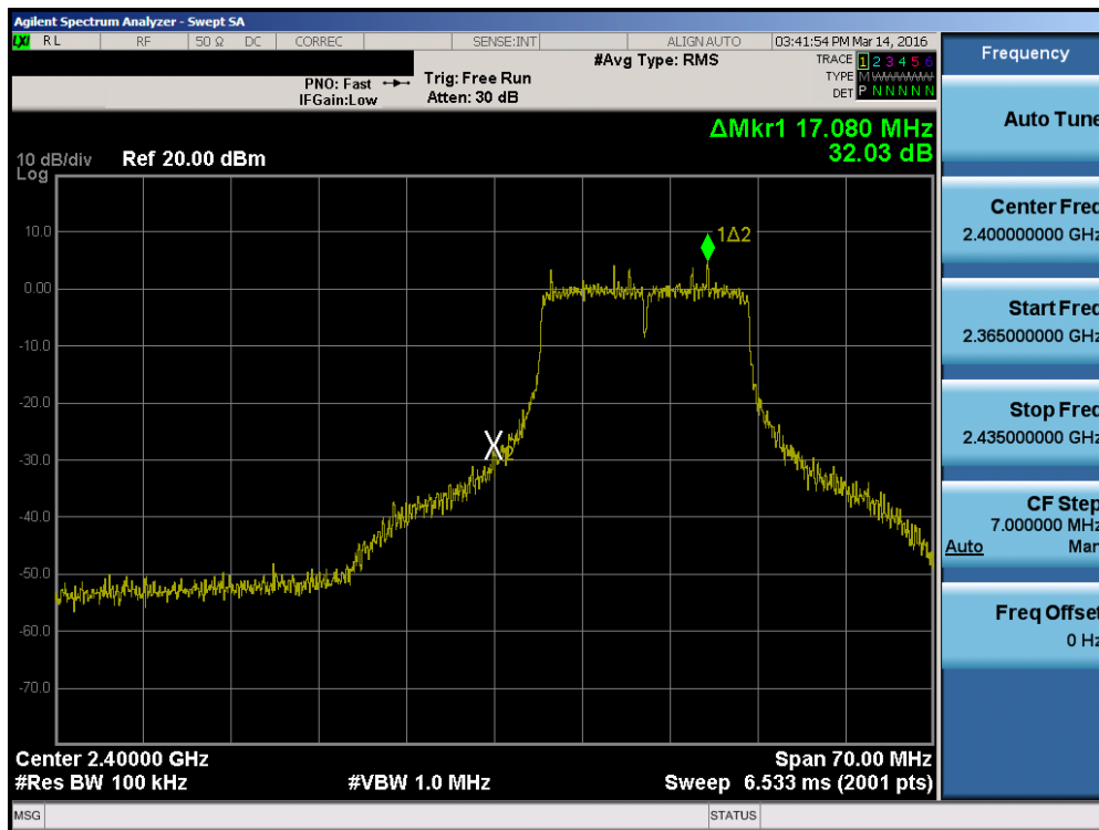
Plot 7-49. Band Edge Plot (802.11g– Ch. 1)
