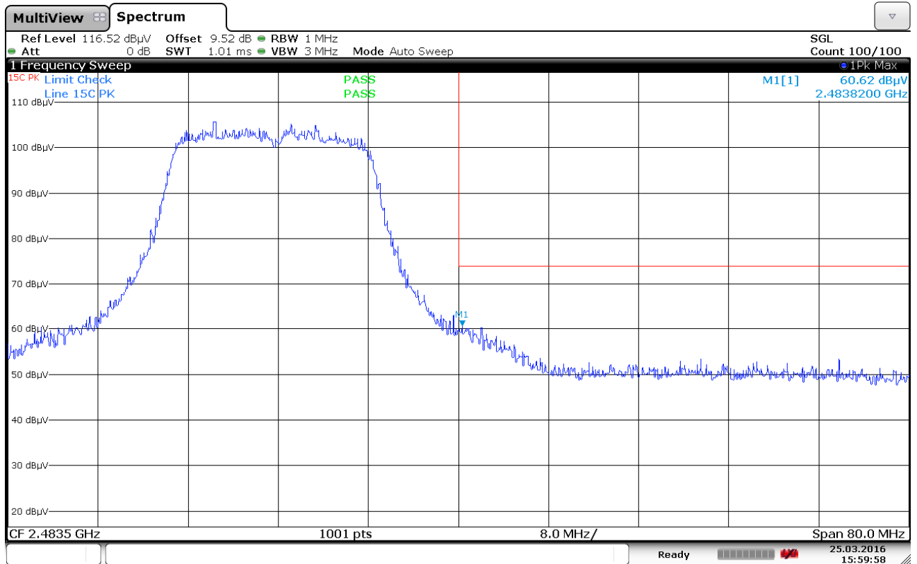
Plot 7-104. Radiated Restricted Upper Band Edge Measurement (Peak)
