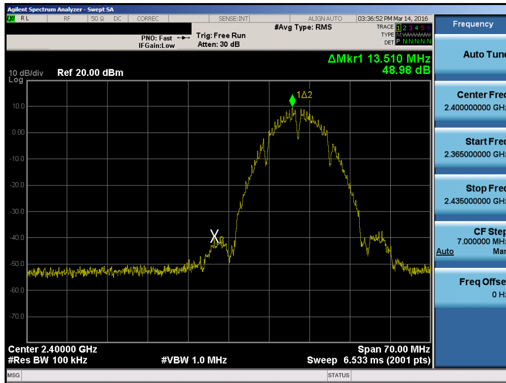
Plot 7-46. Band Edge Plot (802.11b – Ch. 1)
