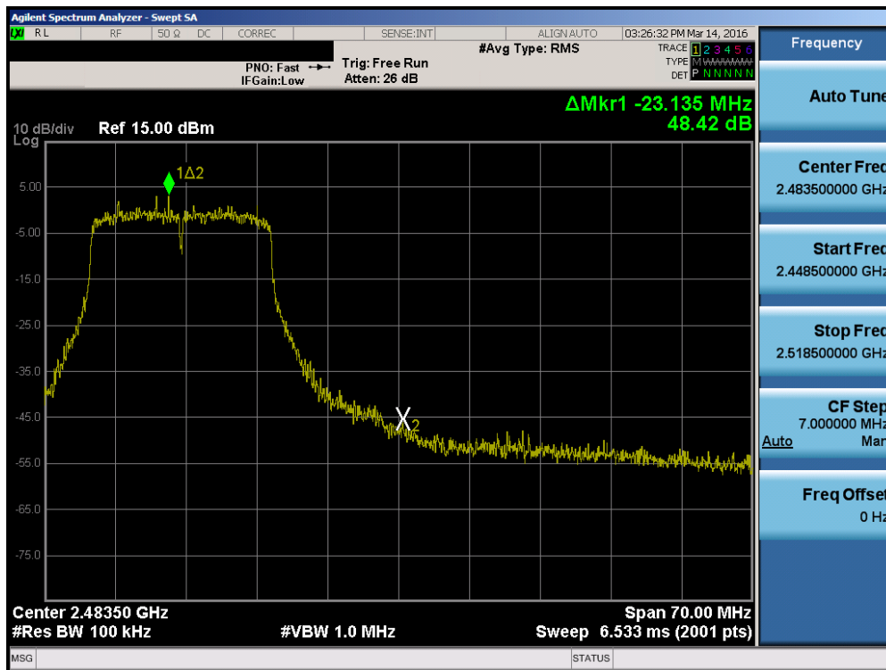
Plot 7-44. Band Edge Plot (802.11n (2.4GHz) – Ch. 11)
