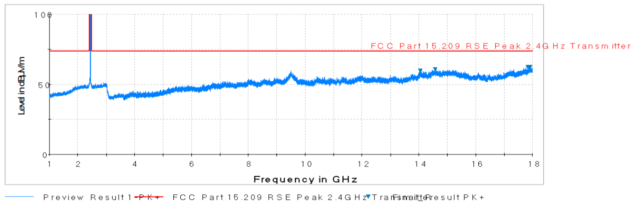
Plot 7-69. Radiated Spurious Plot above 1GHz (802.11b – Ch. 6, Ant. Pol. H)
