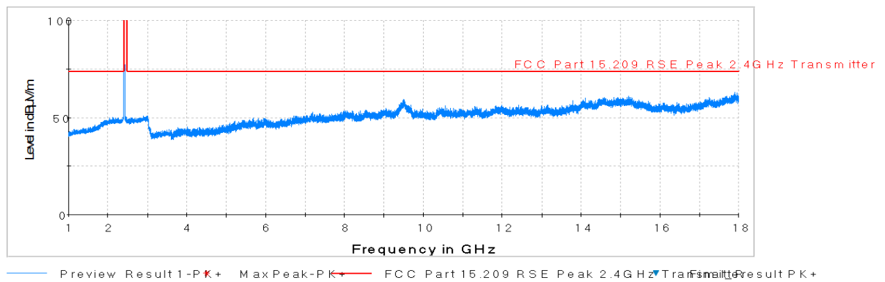
Plot 7-68. Radiated Spurious Plot above 1GHz (802.11b – Ch. 1, Ant. Pol. V)
