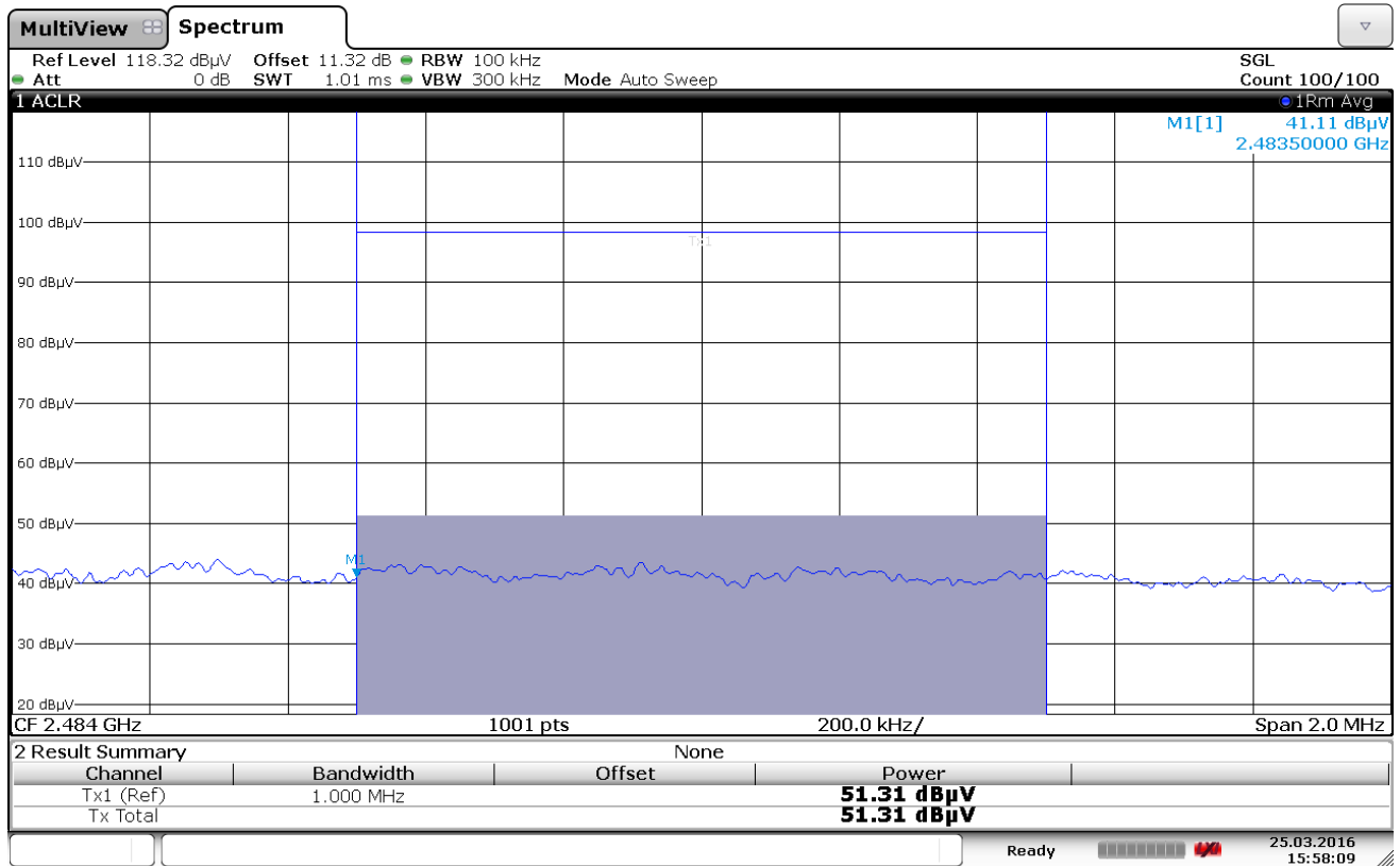
Plot 7-103. Radiated Restricted Upper Band Edge Measurement (Average)
