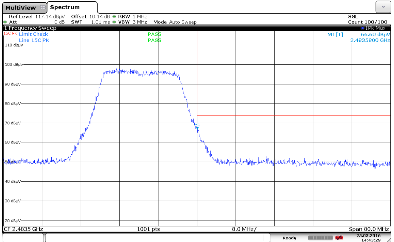
Plot 7-90. Radiated Restricted Upper Band Edge Measurement (Peak)
