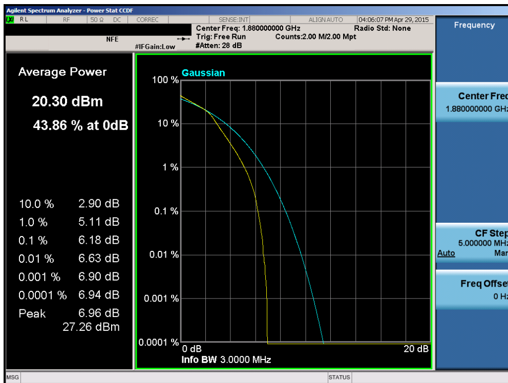
Plot 6-173. PAR Plot (Band 2 – 3.0MHz 16-QAM – RB Size 15)
