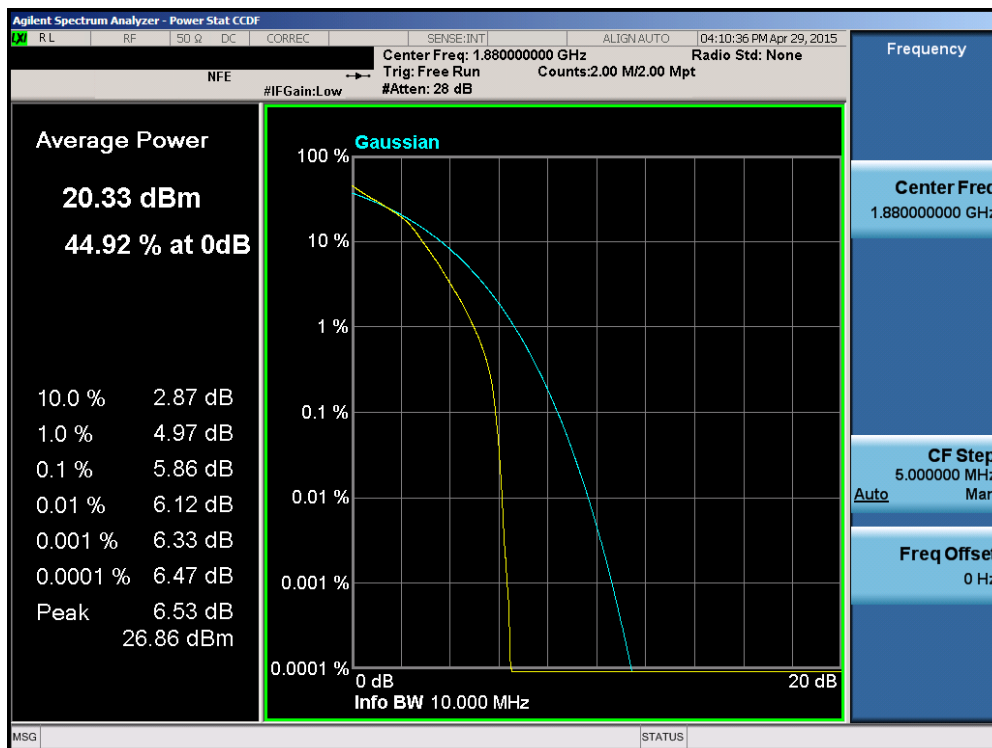
Plot 6-177. PAR Plot (Band 2 – 10.0MHz 16-QAM – RB Size 50)
