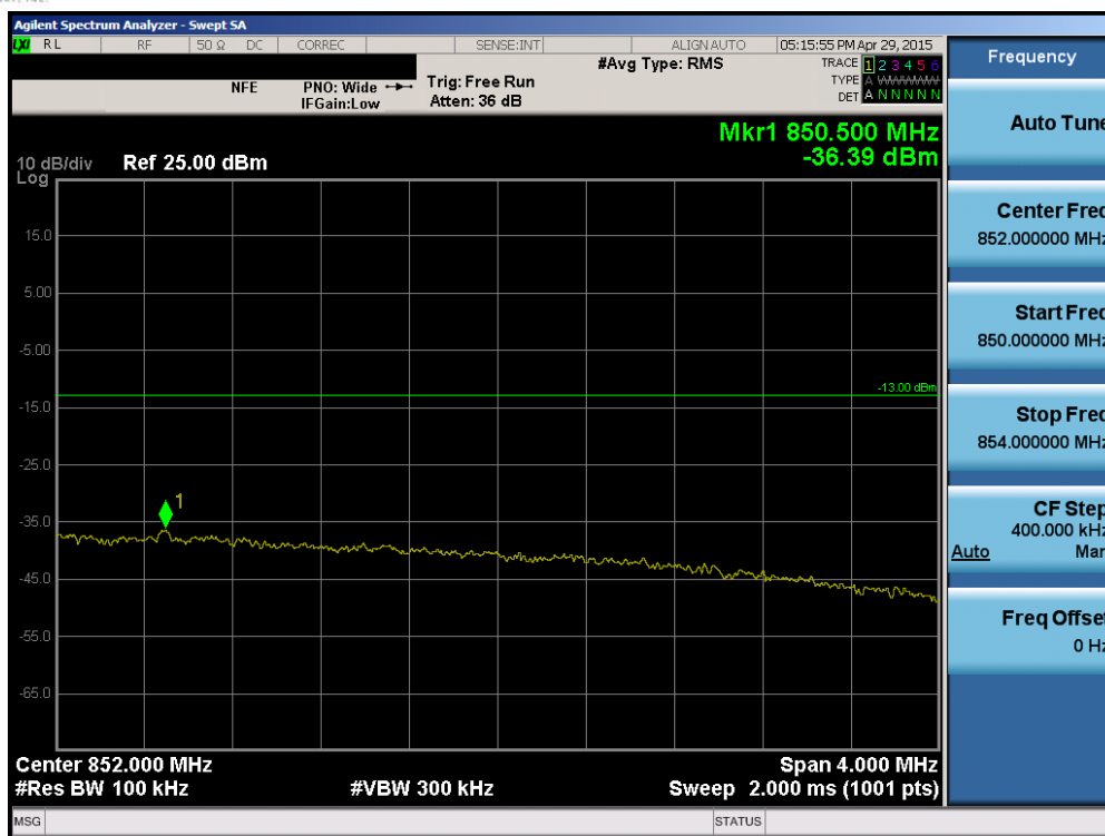
Plot 6-113. Upper Extended Band Edge Plot (Band 5 – 10.0MHz QPSK – RB Size 50)
