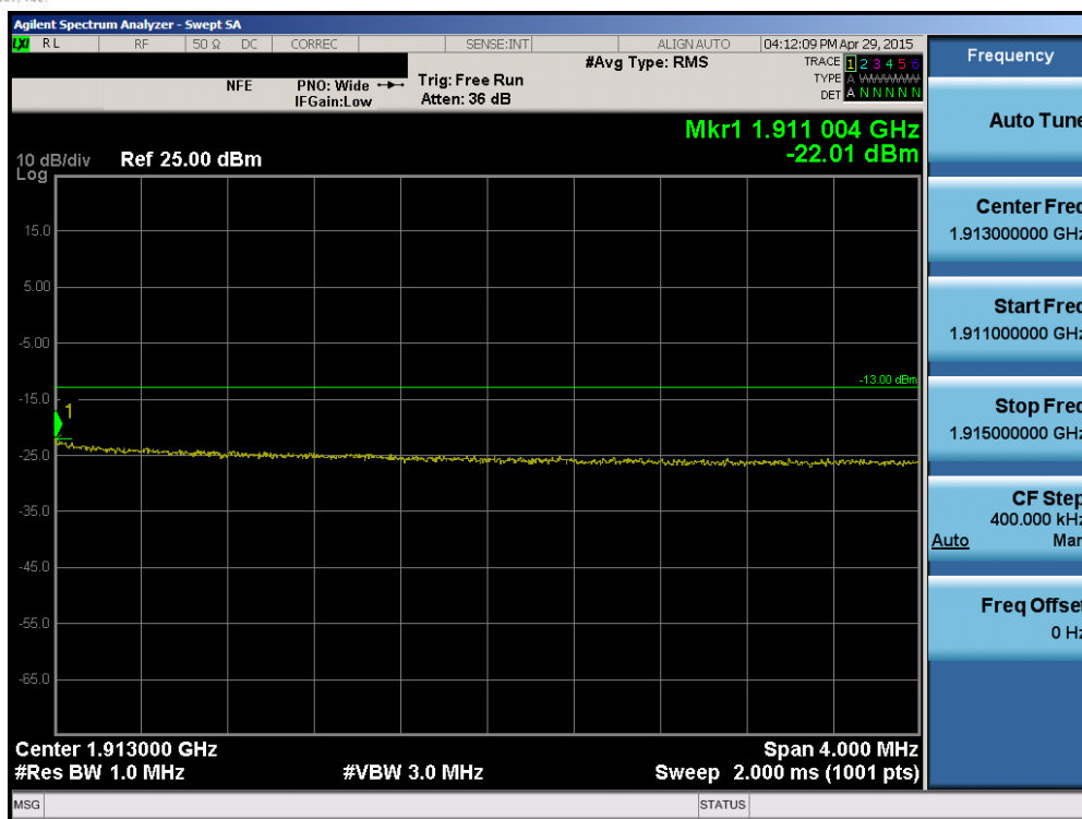
Plot 6-153. Upper Extended Band Edge Plot (Band 2 – 10.0MHz QPSK – RB Size 50)
