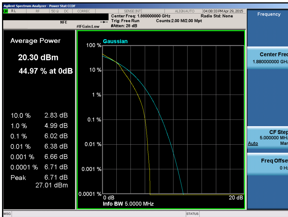
Plot 6-175. PAR Plot (Band 2 – 5.0MHz 16-QAM – RB Size 25)
