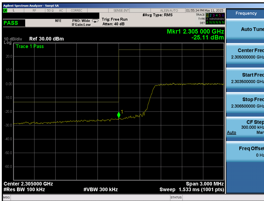
Plot 6-166. Lower Band Edge Plot (Band 30 – 10.0MHz QPSK – RB Size 50)
