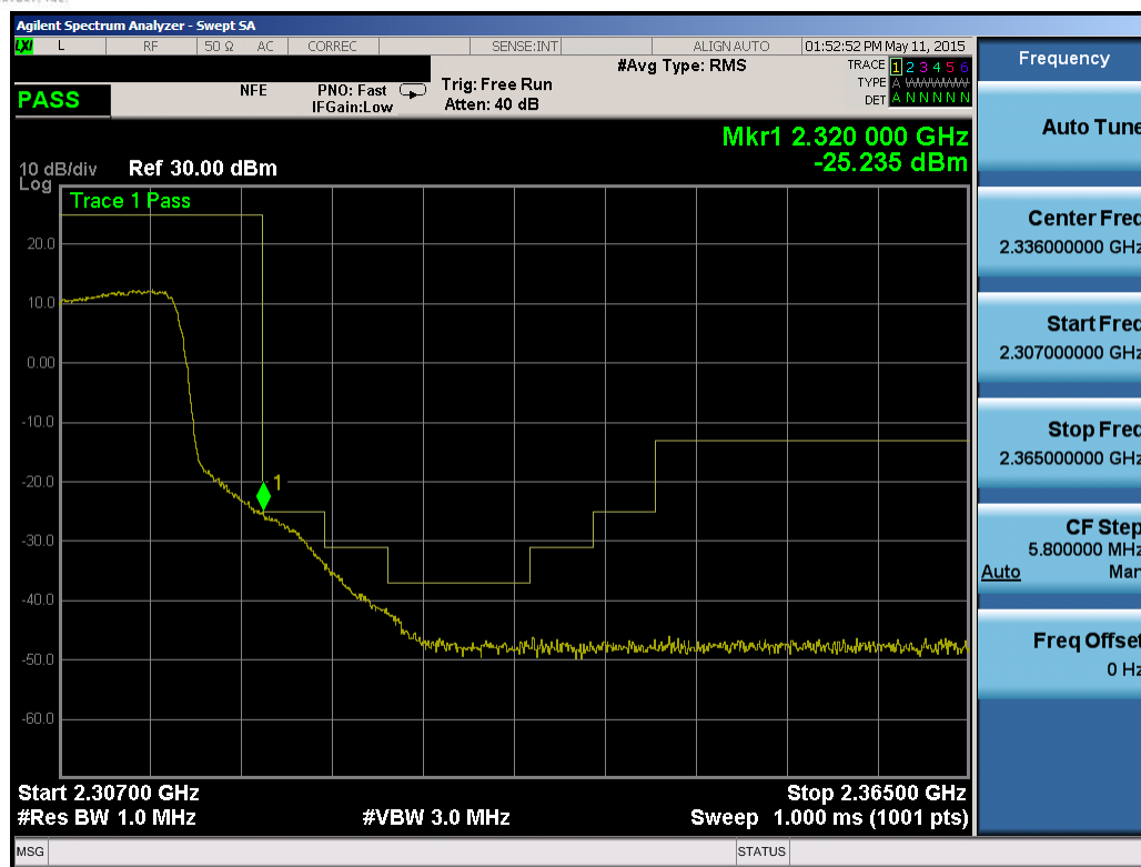
Plot 6-169. Upper Extended Band Edge Plot (Band 30 – 10.0MHz QPSK – RB Size 50)
