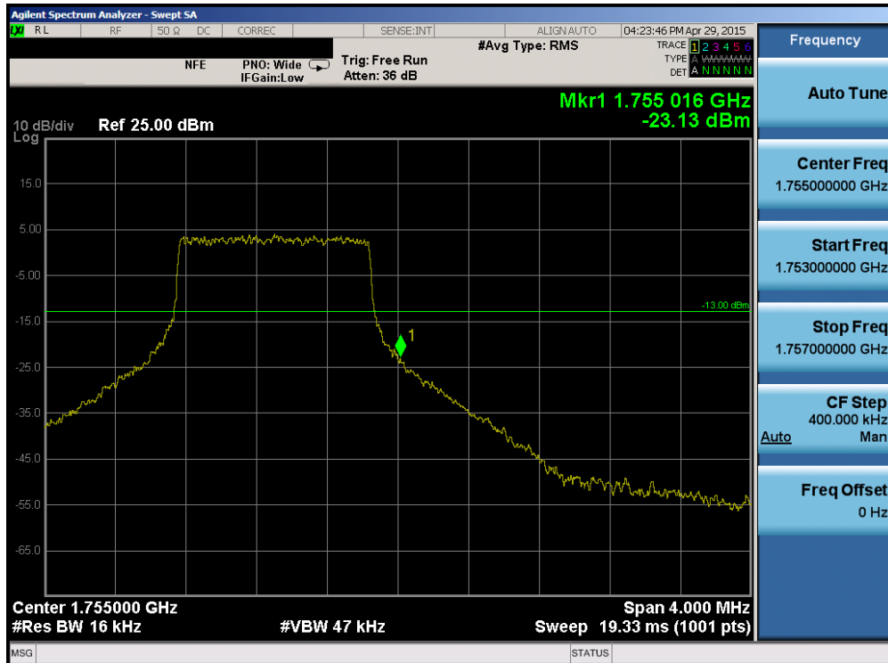
Plot 6-116. Upper Band Edge Plot (Band 4 – 1.4MHz QPSK – RB Size 6)
