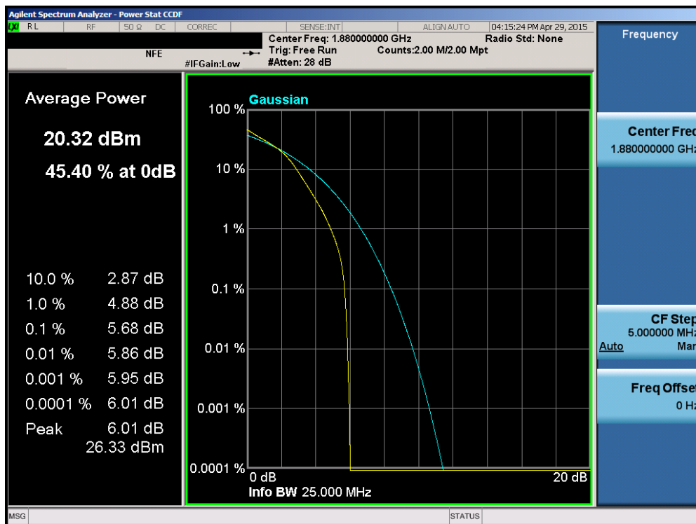
Plot 6-181. PAR Plot (Band 2 – 20.0MHz 16-QAM – RB Size 100)
