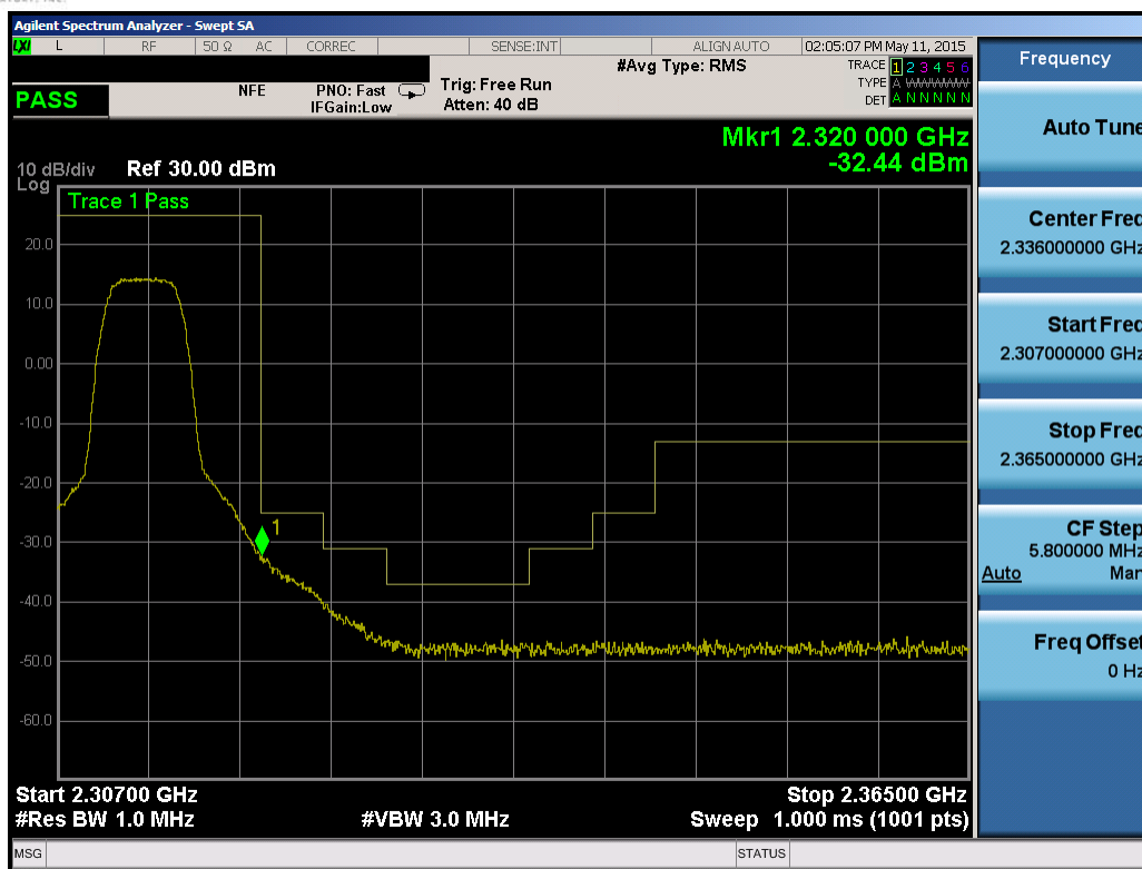
Plot 6-165. Upper Extended Band Edge Plot (Band 30 – 5.0MHz QPSK – RB Size 25)
