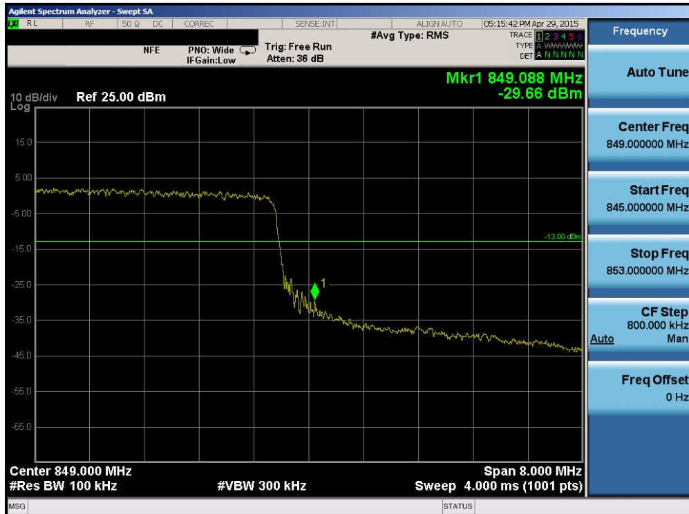
Plot 6-112. Upper Band Edge Plot (Band 5 – 10.0MHz QPSK – RB Size 50)
