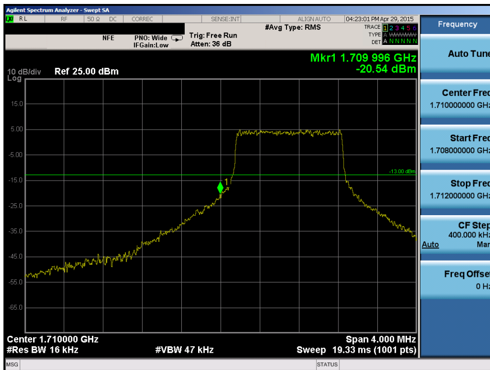
Plot 6-114. Lower Band Edge Plot (Band 4 – 1.4MHz QPSK – RB Size 6)
