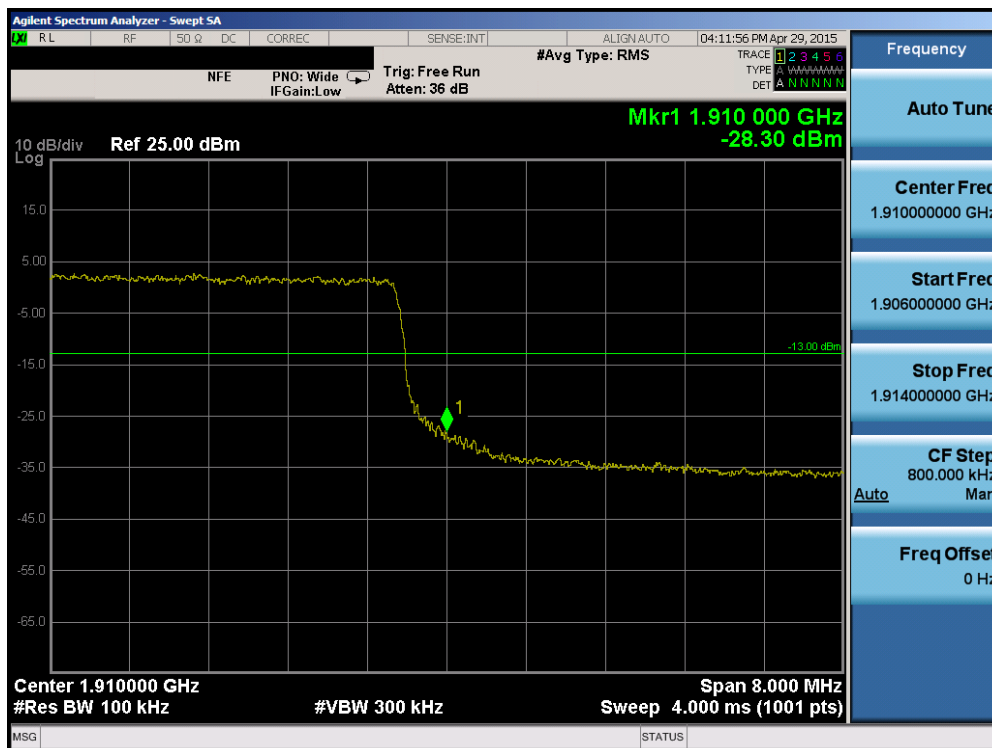
Plot 6-152. Upper Band Edge Plot (Band 2 – 10.0MHz QPSK – RB Size 50)
