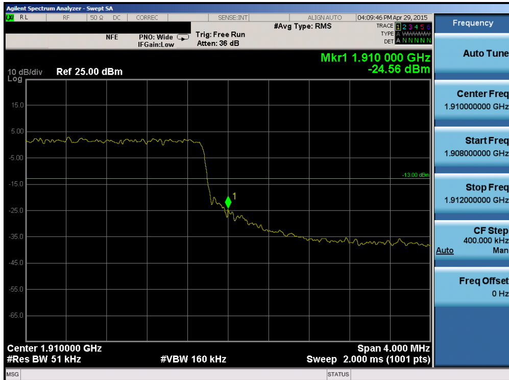
Plot 6-148. Upper Band Edge Plot (Band 2 – 5.0MHz QPSK – RB Size 25)
