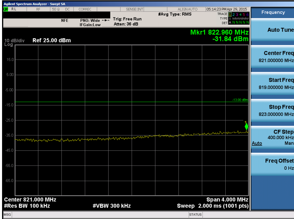
Plot 6-111. Lower Extended Band Edge Plot (Band 5 – 10.0MHz QPSK – RB Size 50)
