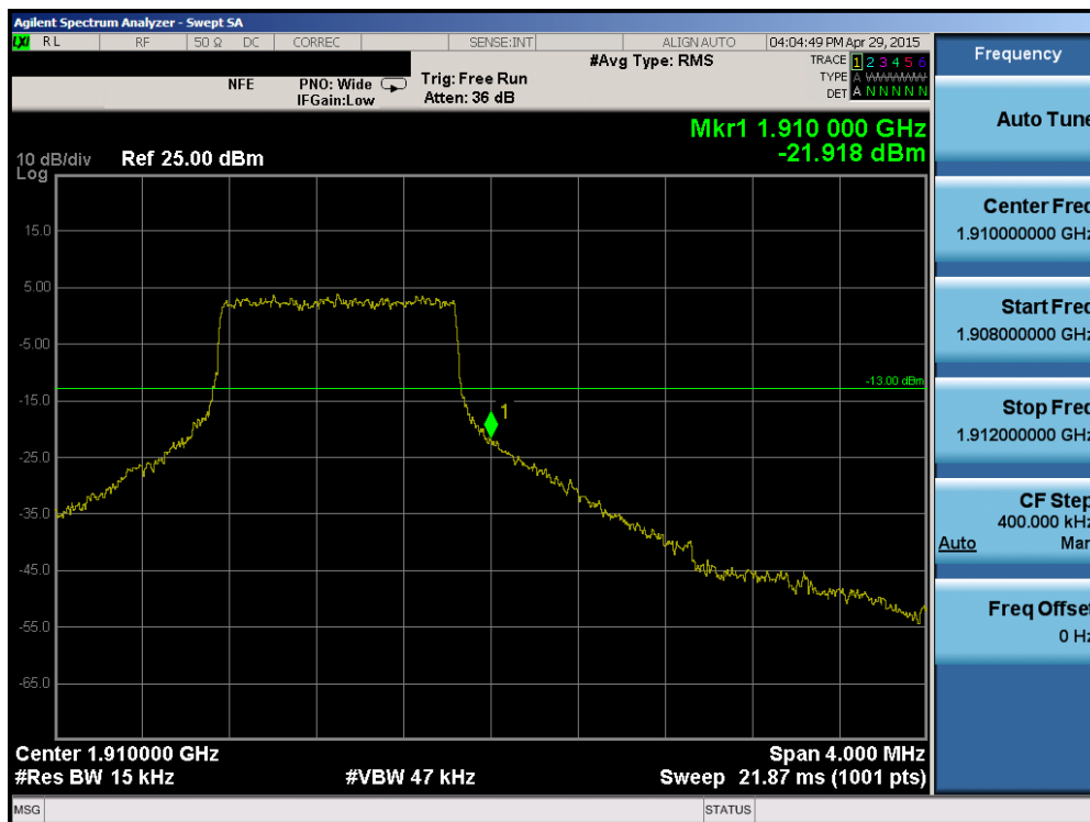
Plot 6-140. Upper Band Edge Plot (Band 2 – 1.4MHz QPSK – RB Size 6)
