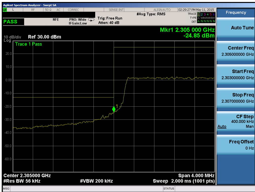
Plot 6-162. Lower Band Edge Plot (Band 30 – 5.0MHz QPSK – RB Size 25)
