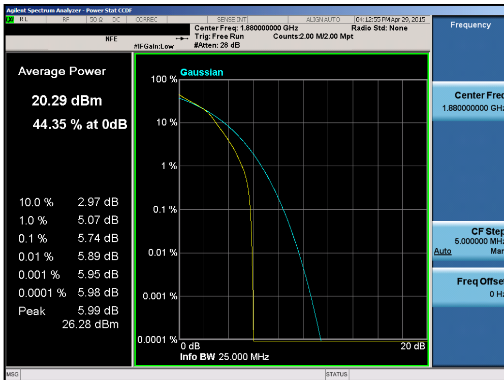
Plot 6-179. PAR Plot (Band 2 – 15.0MHz 16-QAM – RB Size 75)
