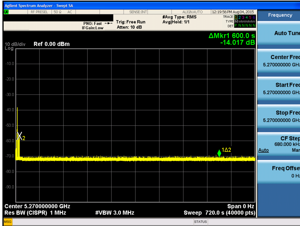
Figure 5-7. Band 2A Non-occupancy Period - Monitoring live spectrum
