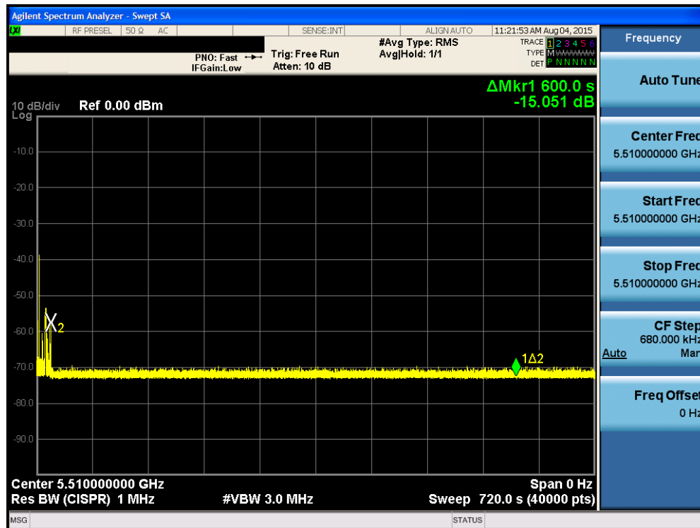
Figure 5-8. Band 2C Non-occupancy Period - Monitoring live spectrum
