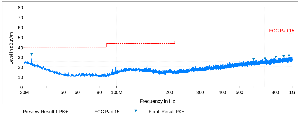
Plot 6-53. Radiated Spurious Plot below 1GHz (Pol. V)
