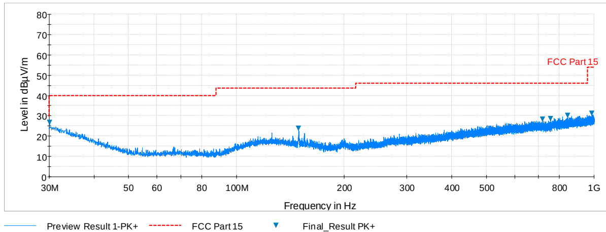
Plot 6-52. Radiated Spurious Plot below 1GHz (Pol. H)
