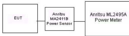
Figure 8-2 Power Measurement Setup for Bandwidths < 50 MHz
