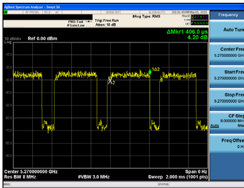
Figure 5-1. Band 2A Pulse Width
