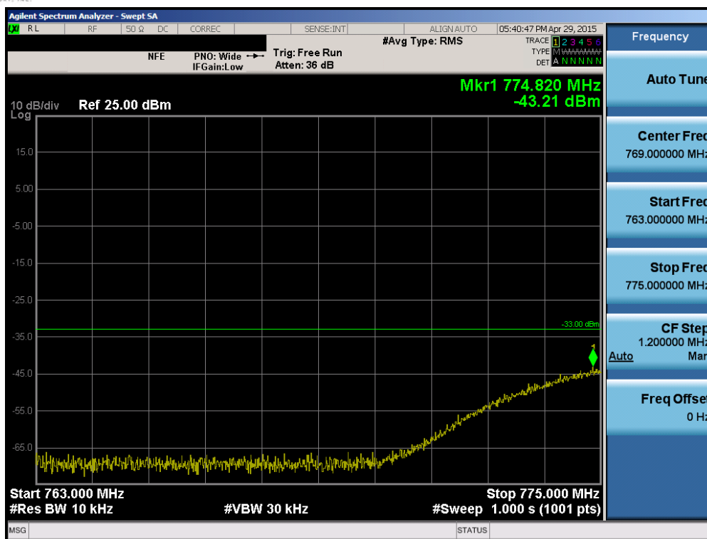
Plot 6-109. Lower Emission Mask Edge Plot (Band 13 - 10.0MHz QPSK - RB Size 50)
