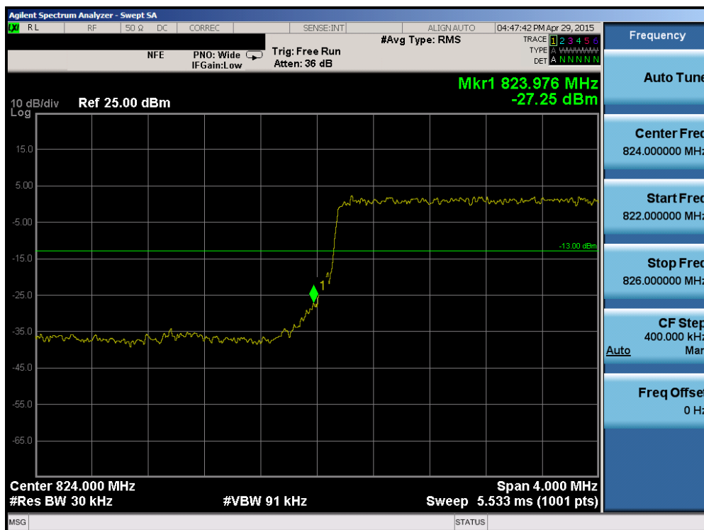
Plot 6-116. Lower Band Edge Plot (Band 5 - 3.0MHz QPSK - RB Size 15)
