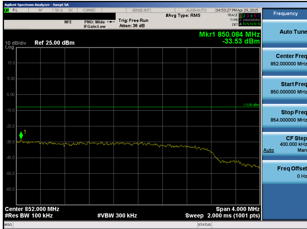
Plot 6-123. Upper Extended Band Edge Plot (Band 5 – 5.0MHz QPSK – RB Size 25)
