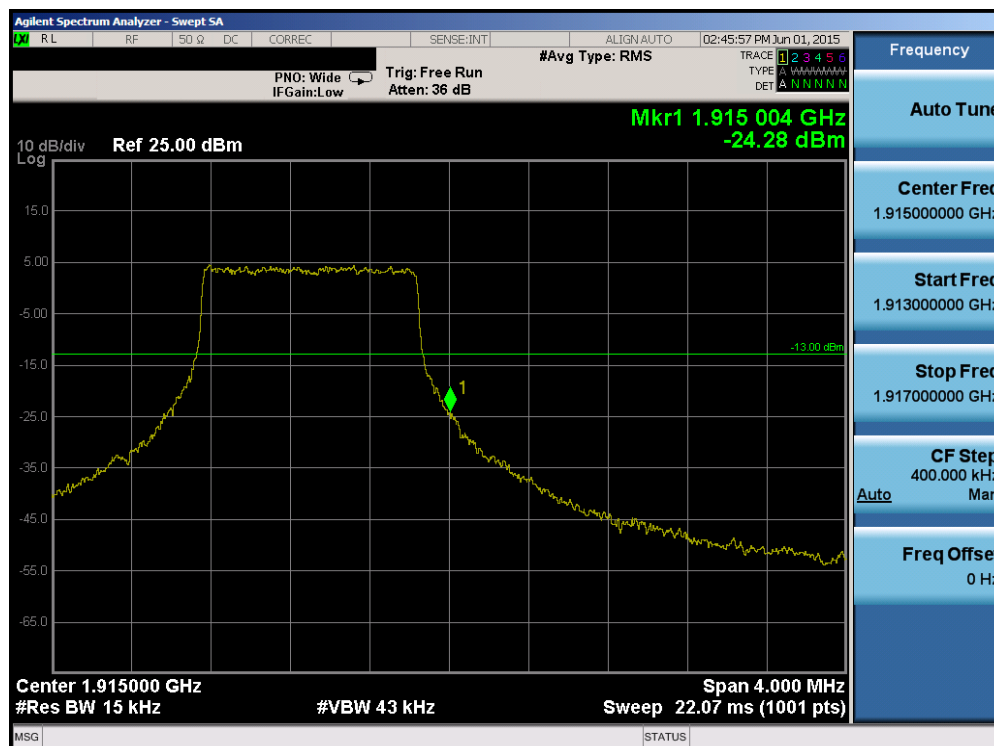
Plot 6-152. Upper Band Edge Plot (Band 25 - 1.4MHz QPSK - RB Size 6)
