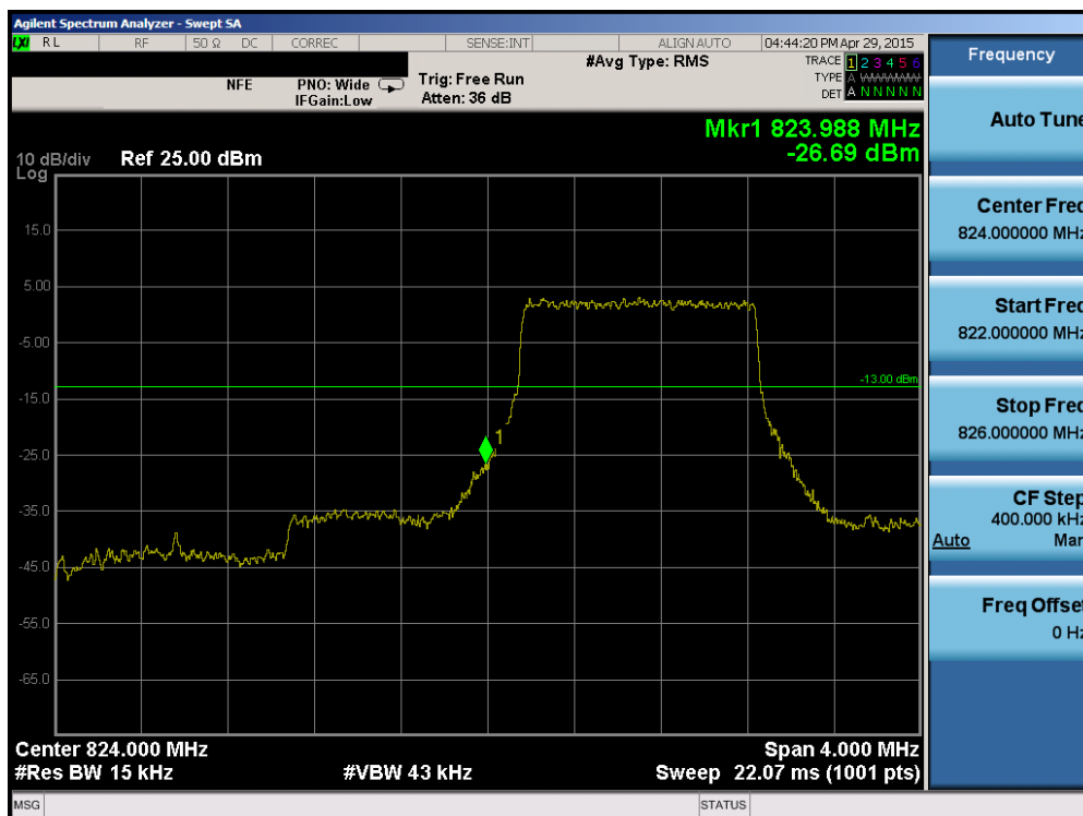
Plot 6-112. Lower Band Edge Plot (Band 5 – 1.4MHz QPSK – RB Size 6)
