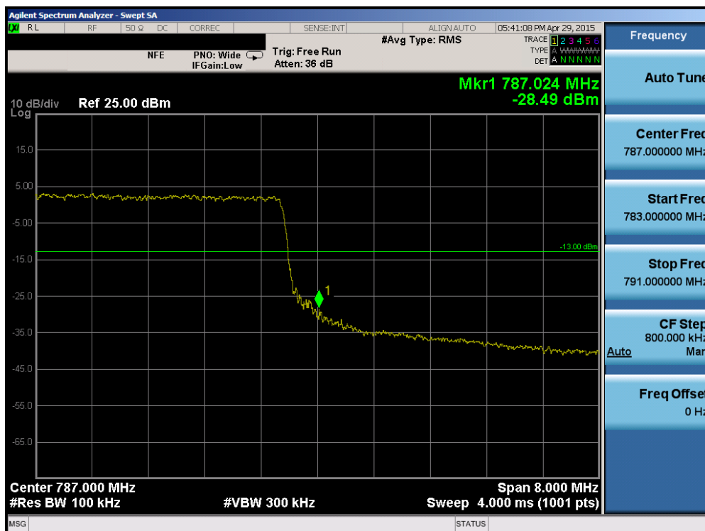
Plot 6-110. Upper Band Edge Plot (Band 13 - 10.0MHz QPSK - RB Size 50)
