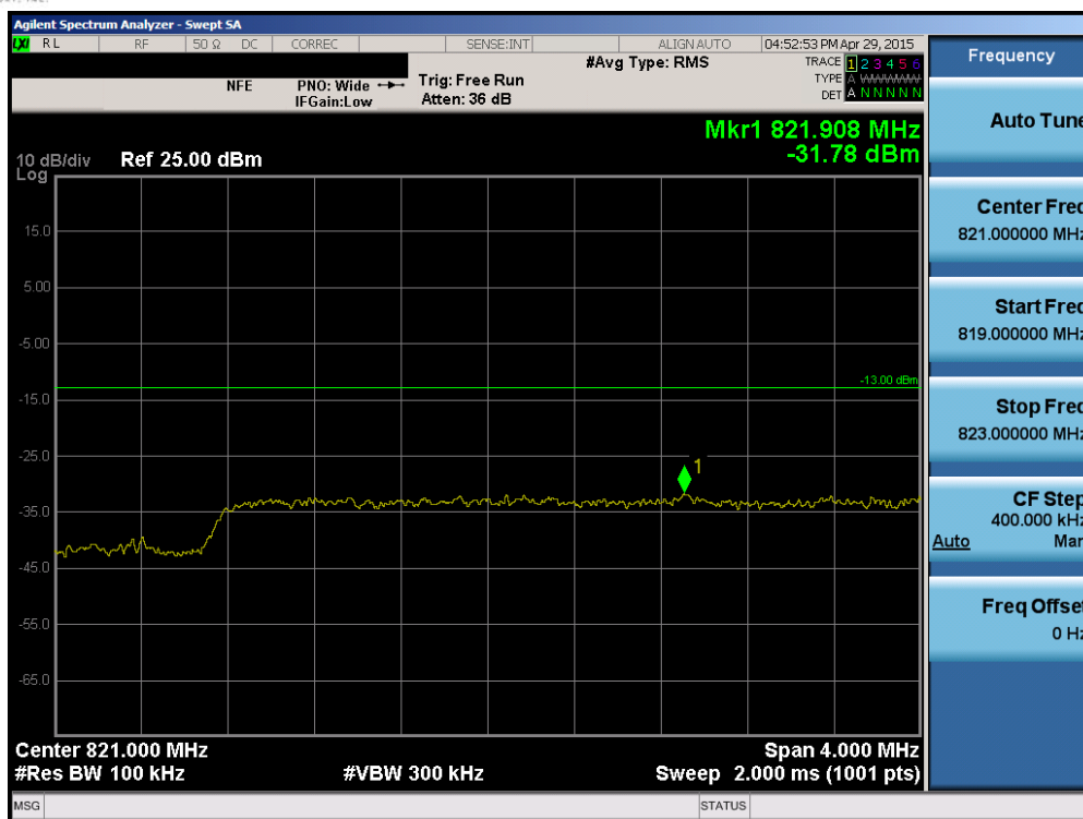
Plot 6-121. Lower Extended Band Edge Plot (Band 5 - 5.0MHz QPSK - RB Size 25)
