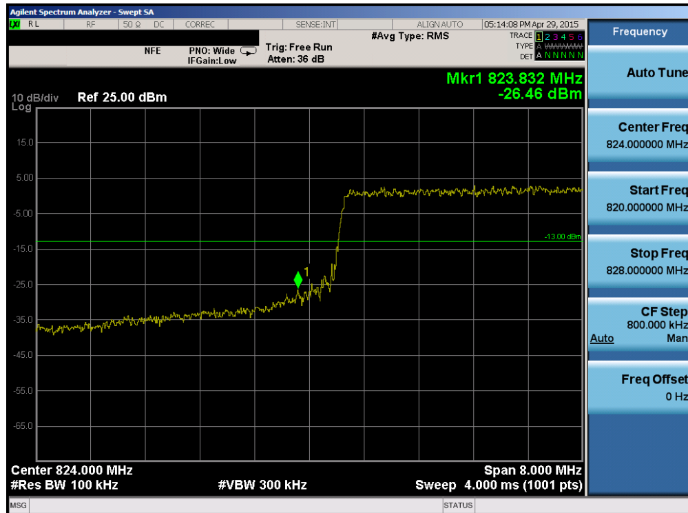
Plot 6-124. Lower Band Edge Plot (Band 5 – 10.0MHz QPSK – RB Size 50)
