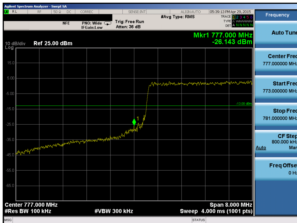
Plot 6-108. Lower Band Edge Plot (Band 13 – 10.0MHz QPSK – RB Size 50)
