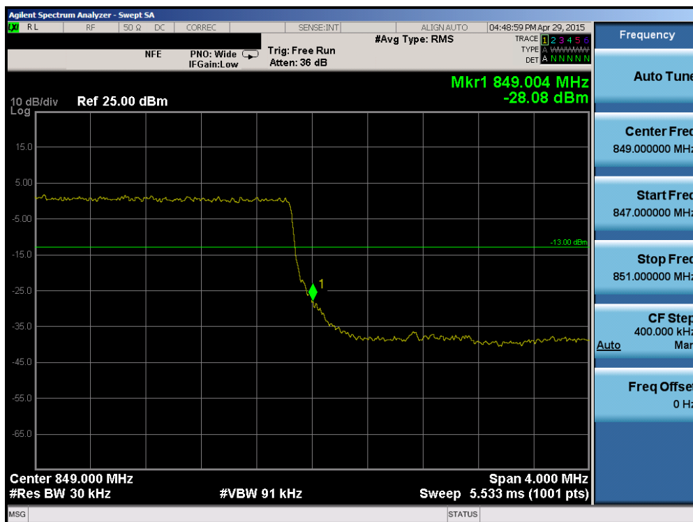
Plot 6-118. Upper Band Edge Plot (Band 5 – 3.0MHz QPSK – RB Size 15)
