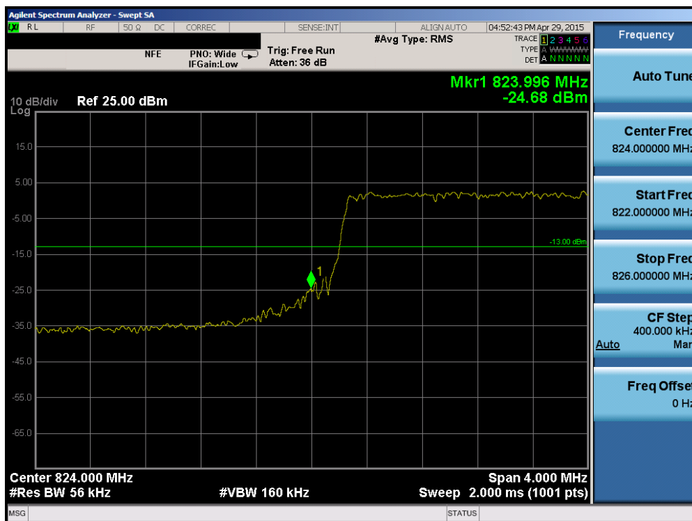
Plot 6-120. Lower Band Edge Plot (Band 5 – 5.0MHz QPSK – RB Size 25)
