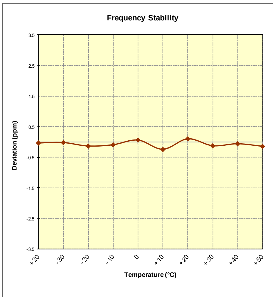
Figure 6-11. Frequency Stability Graph (Band 25)
