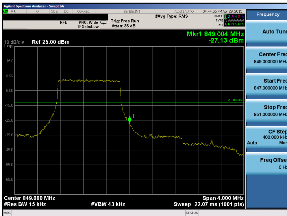
Plot 6-114. Upper Band Edge Plot (Band 5 – 1.4MHz QPSK – RB Size 6)
