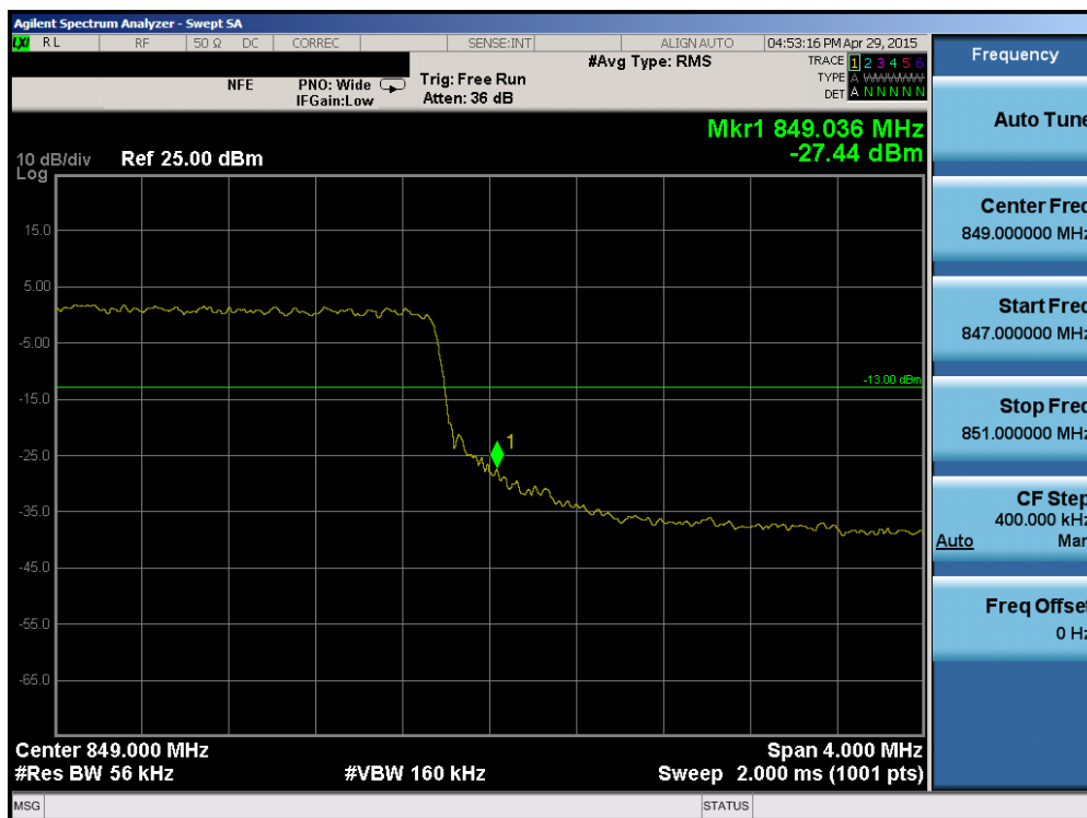
Plot 6-122. Upper Band Edge Plot (Band 5 - 5.0MHz QPSK - RB Size 25)
