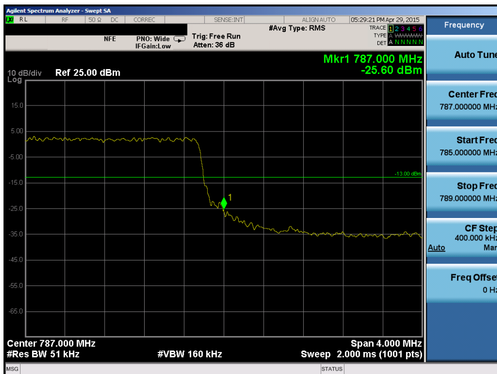
Plot 6-106. Upper Band Edge Plot (Band 13 – 5.0MHz QPSK – RB Size 25)
