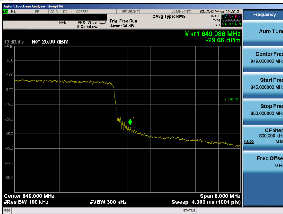
Plot 6-125. Upper Band Edge Plot (Band 5 – 10.0MHz QPSK – RB Size 50)
