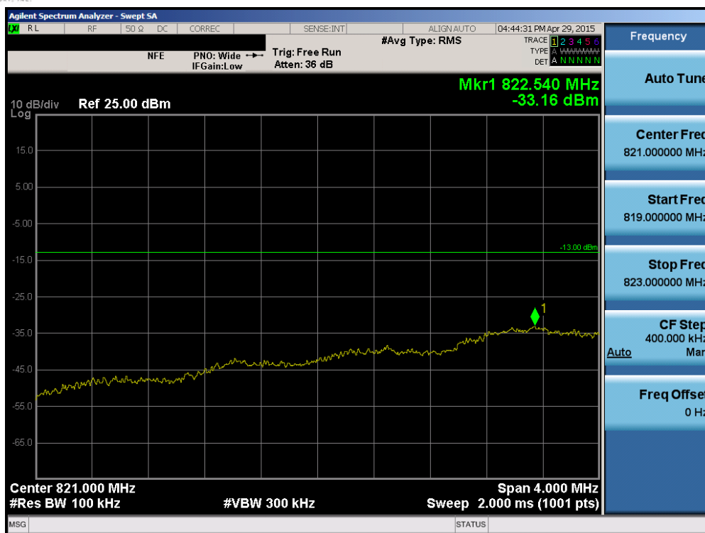
Plot 6-113. Lower Extended Band Edge Plot (Band 5 – 1.4MHz QPSK – RB Size 6)
