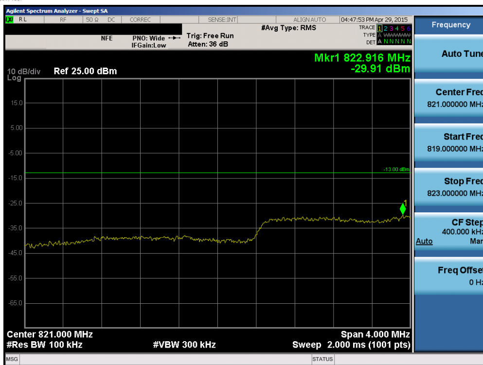
Plot 6-117. Lower Extended Band Edge Plot (Band 5 – 3.0MHz QPSK – RB Size 15)
