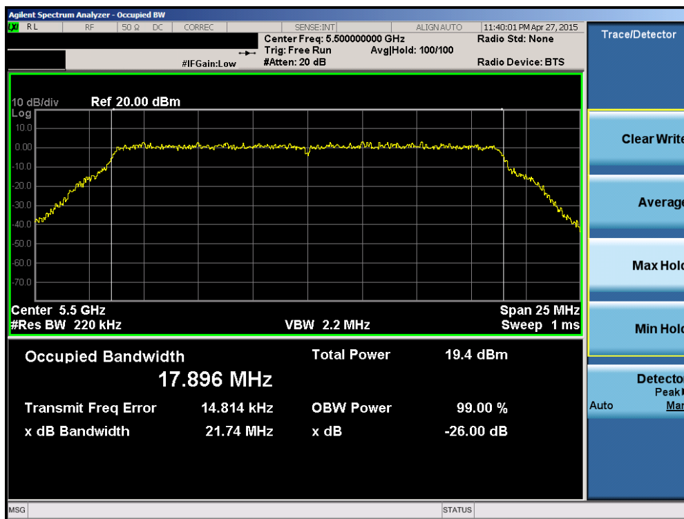
Plot 6-51. 26dB Bandwidth Plot (20MHz BW 802.11n (UNII Band 2C) – Ch. 100)
