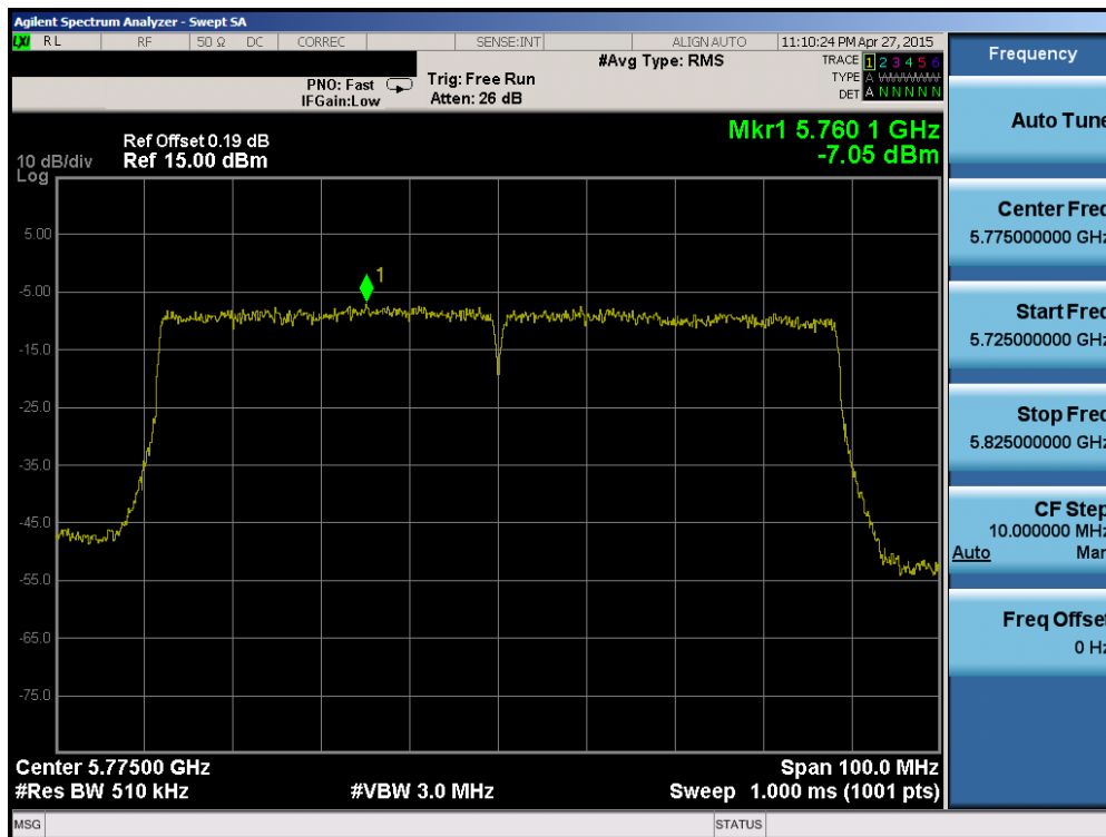
Plot 6-114. Power Spectral Density Plot (80MHz BW 802.11a/n/ac (UNII Band 3) – Ch. 155)
