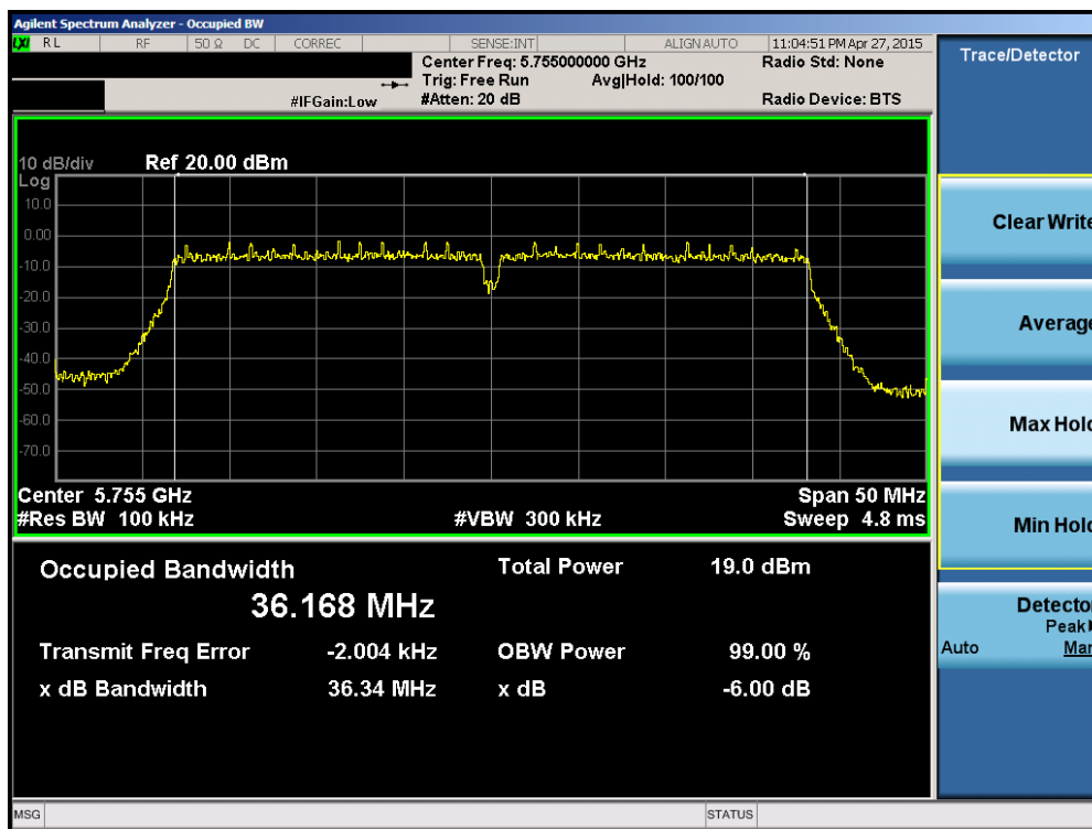
Plot 6-65. 6dB Bandwidth Plot (40MHz BW 802.11n (UNII Band 3) – Ch. 151)
