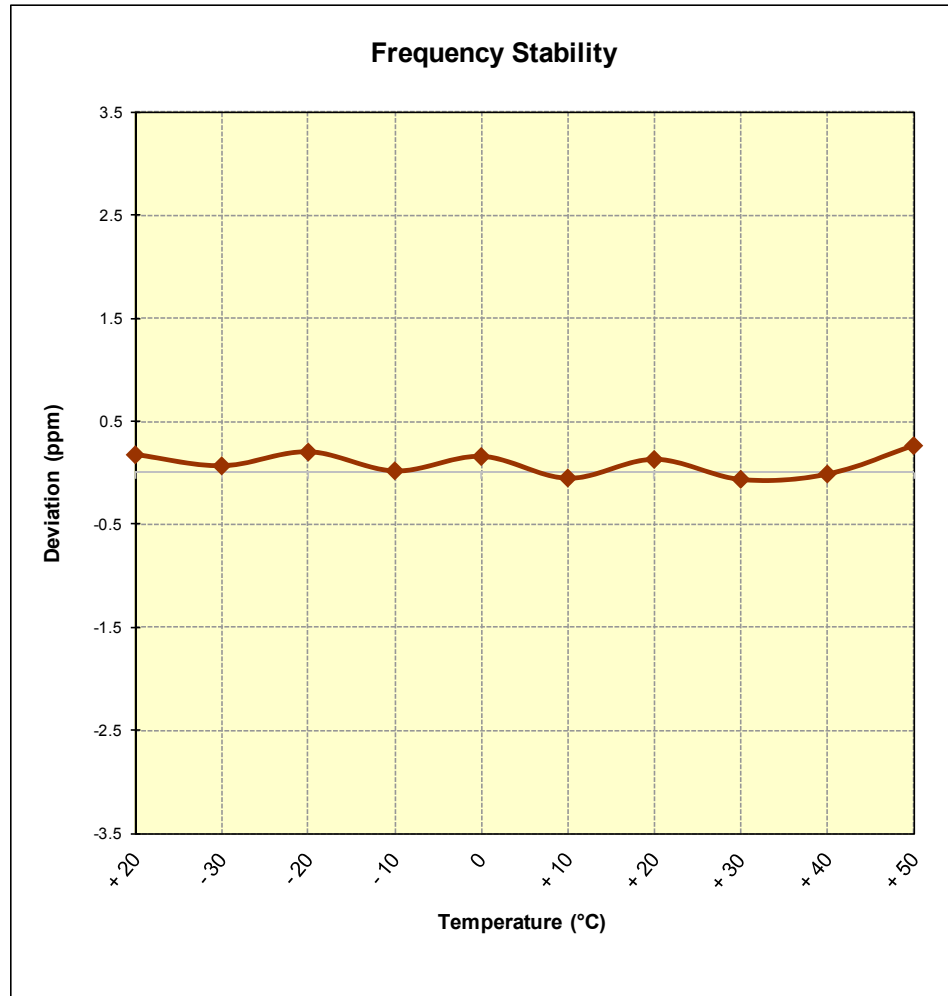
Figure 6-8. Frequency Stability Graph (AWS WCDMA Mode – Ch. 1412)
