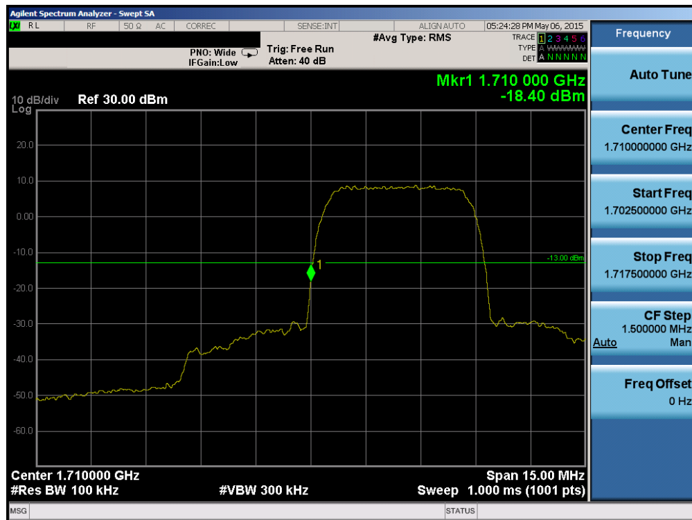
Plot 6-34. Band Edge Plot (AWS WCDMA Mode – Ch. 1312)
