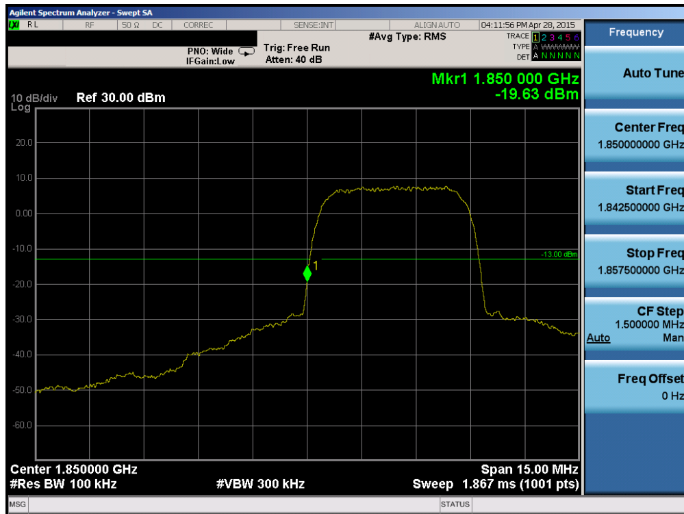
Plot 6-38. Band Edge Plot (PCS WCDMA Mode – Ch. 9262)
