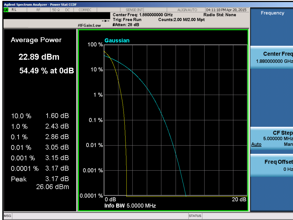
Plot 6-42. Peak-Average Ratio Plot (PCS WCDMA Mode – Ch. 9400)
