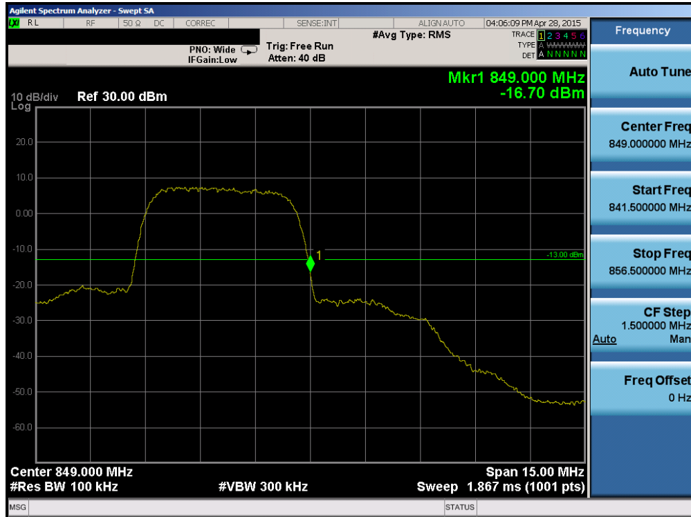
Plot 6-33. Band Edge Plot (Cellular WCDMA Mode – Ch. 4233)
