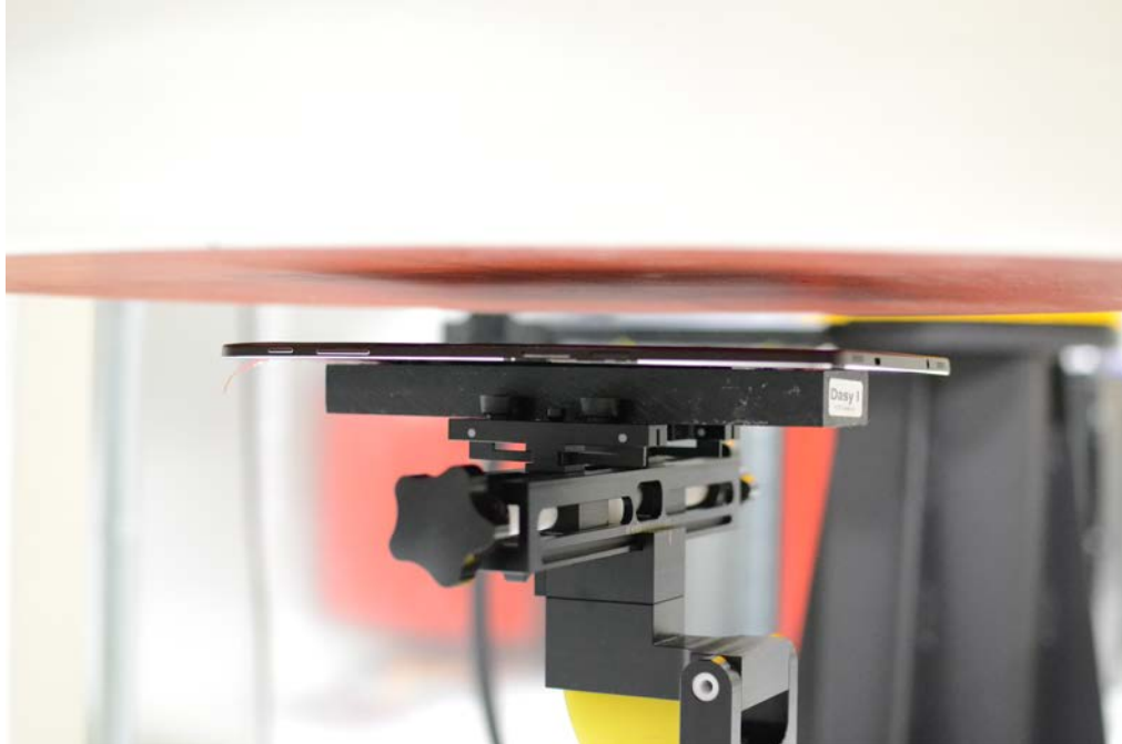
SAR Test Setup Photo 3: Back Side at 2.4 cm
