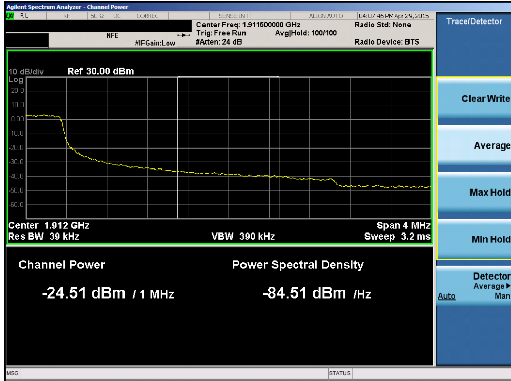
Plot 6-126. Upper Extended Band Edge Plot (Band 2 – 3.0MHz QPSK – RB Size 15)
