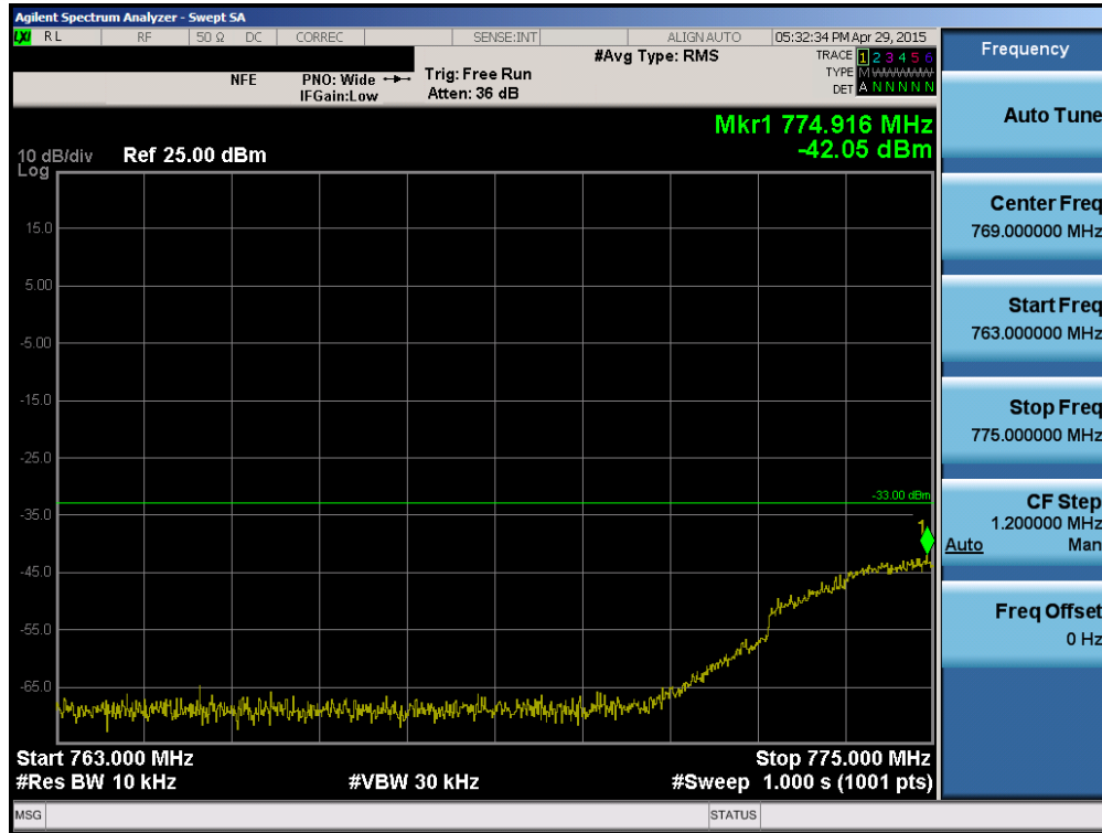
Plot 6-74. Lower Emission Mask Edge Plot (Band 13 – 5.0MHz QPSK – RB Size 25)
