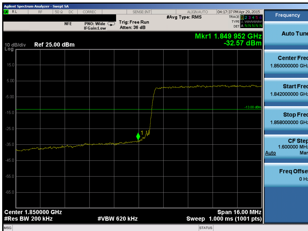
Plot 6-139. Lower Band Edge Plot (Band 2 – 20.0MHz QPSK – RB Size 100)
