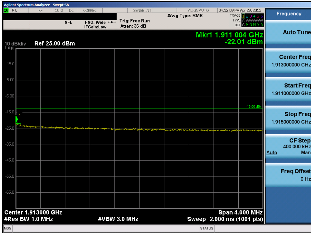
Plot 6-134. Upper Extended Band Edge Plot (Band 2 – 10.0MHz QPSK – RB Size 50)
