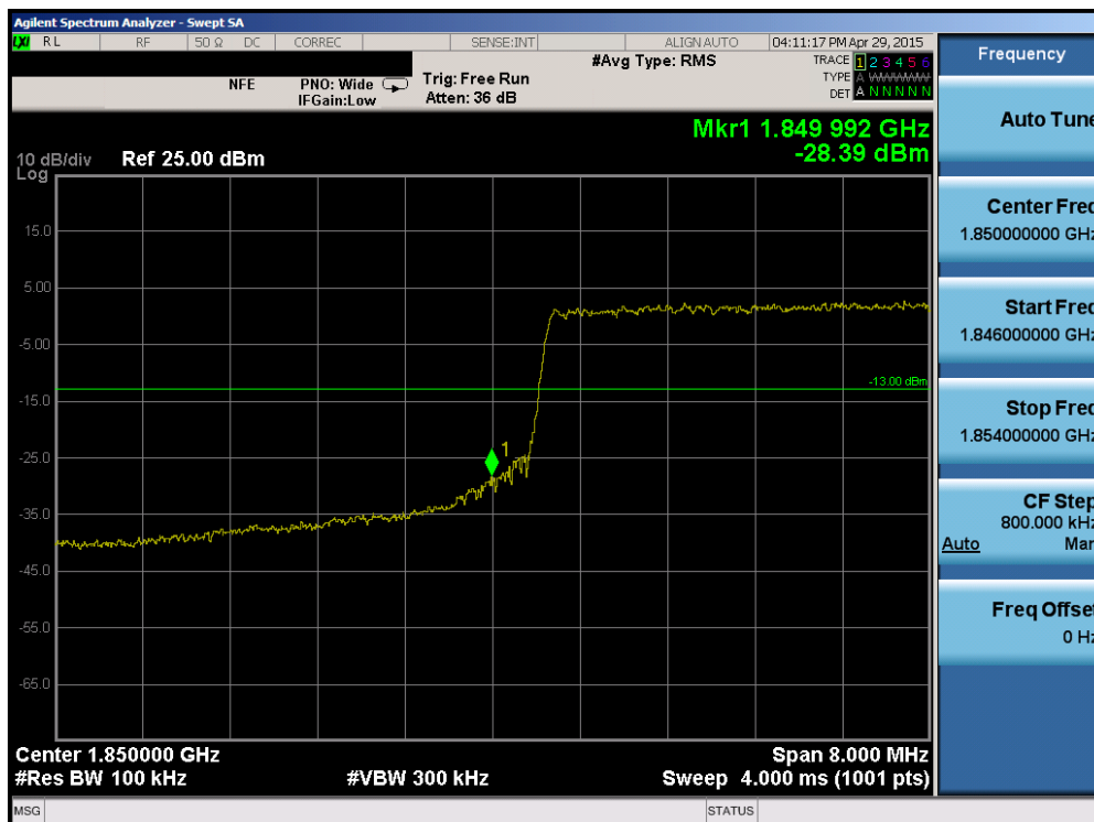
Plot 6-131. Lower Band Edge Plot (Band 2 – 10.0MHz QPSK – RB Size 50)
