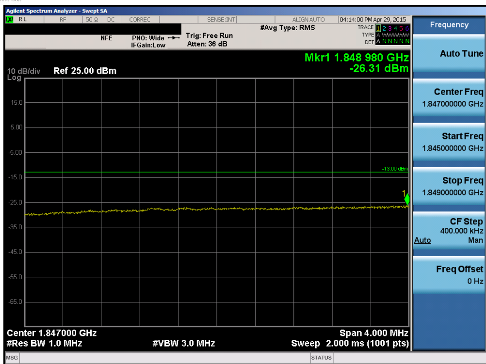
Plot 6-136. Lower Extended Band Edge Plot (Band 2 – 15.0MHz QPSK – RB Size 75)
