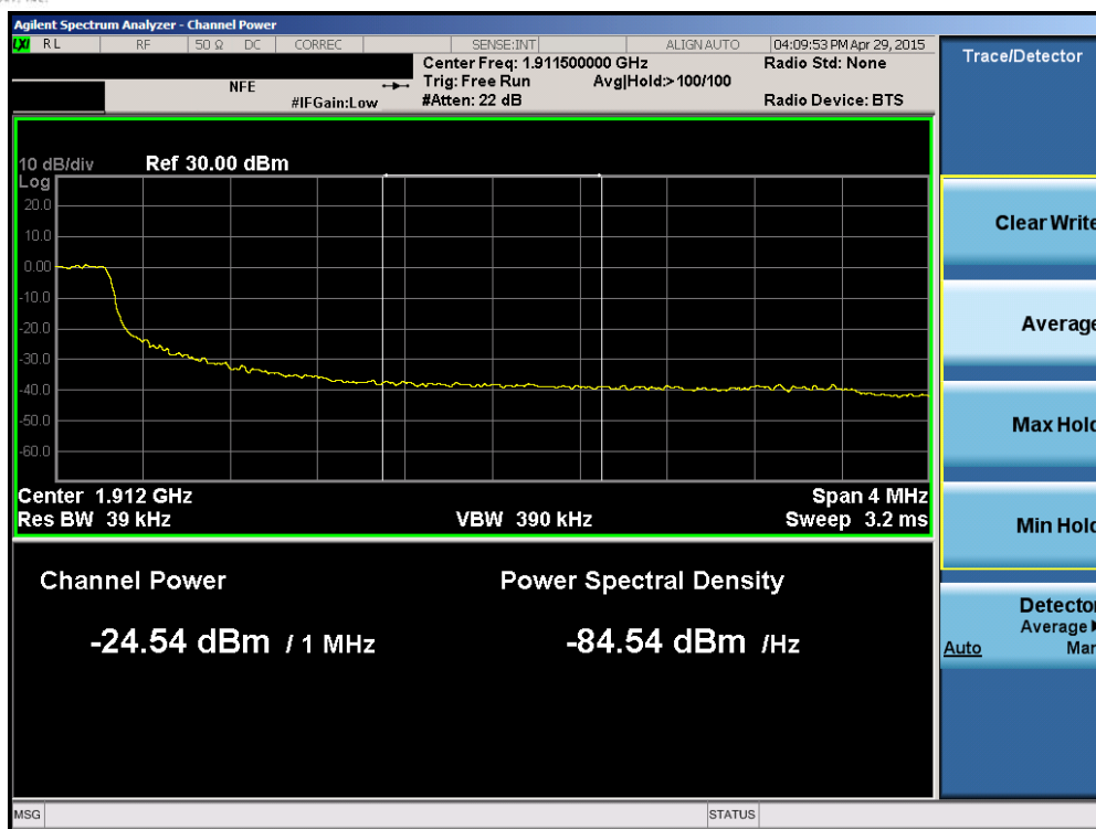
Plot 6-130. Upper Extended Band Edge Plot (Band 2 – 5.0MHz QPSK – RB Size 25)
