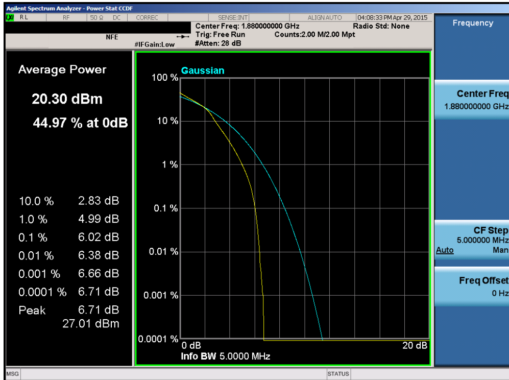
Plot 6-148. PAR Plot (Band 2 – 5.0MHz 16-QAM – RB Size 25)
