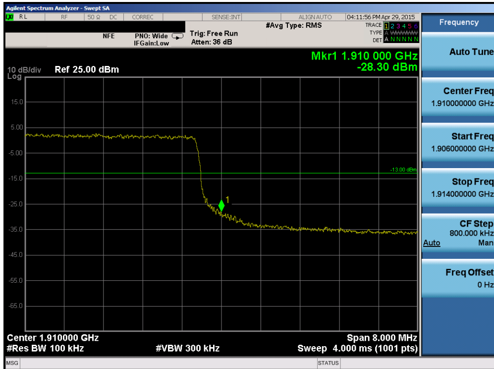
Plot 6-133. Upper Band Edge Plot (Band 2 – 10.0MHz QPSK – RB Size 50)
