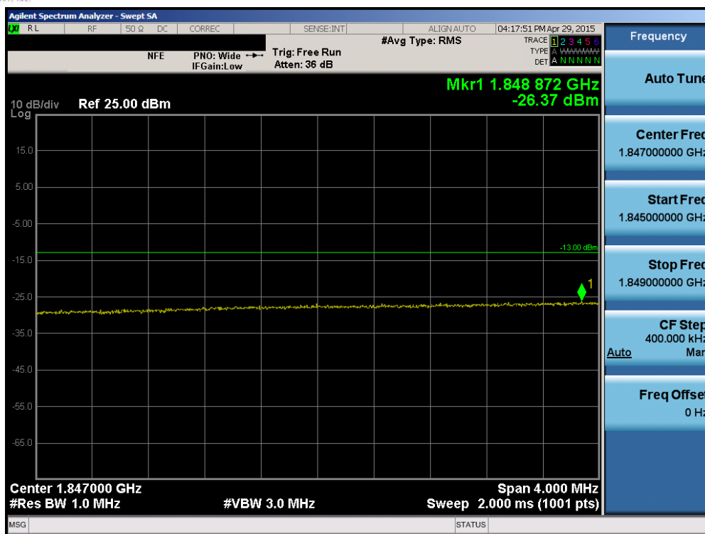
Plot 6-140. Lower Extended Band Edge Plot (Band 2 – 20.0MHz QPSK – RB Size 100)
