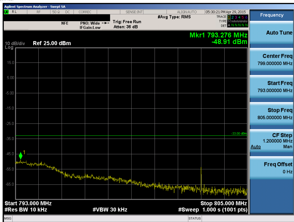
Plot 6-76. Upper Emission Mask Edge Plot (Band 13 – 5.0MHz QPSK – RB Size 25)
