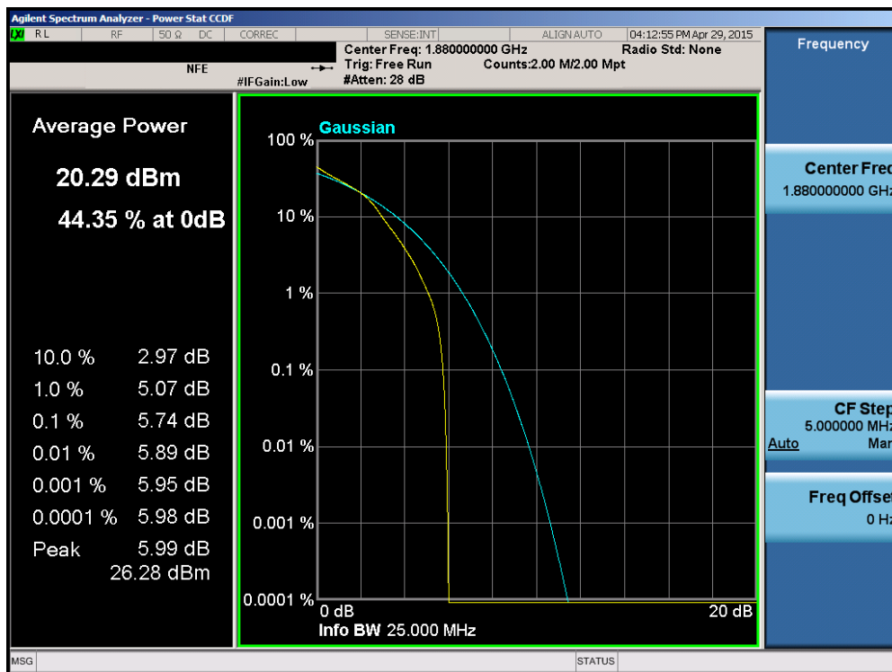
Plot 6-152. PAR Plot (Band 2 – 15.0MHz 16-QAM – RB Size 75)
