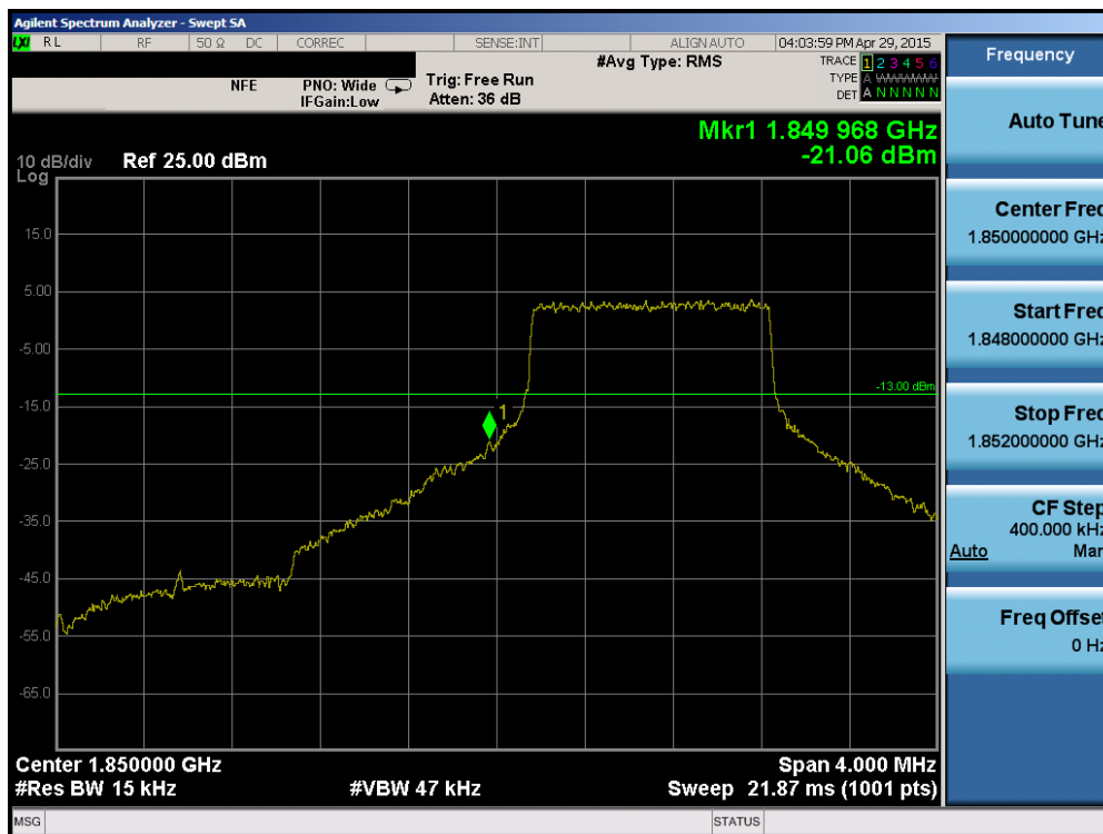
Plot 6-119. Lower Band Edge Plot (Band 2 – 1.4MHz QPSK – RB Size 6)
