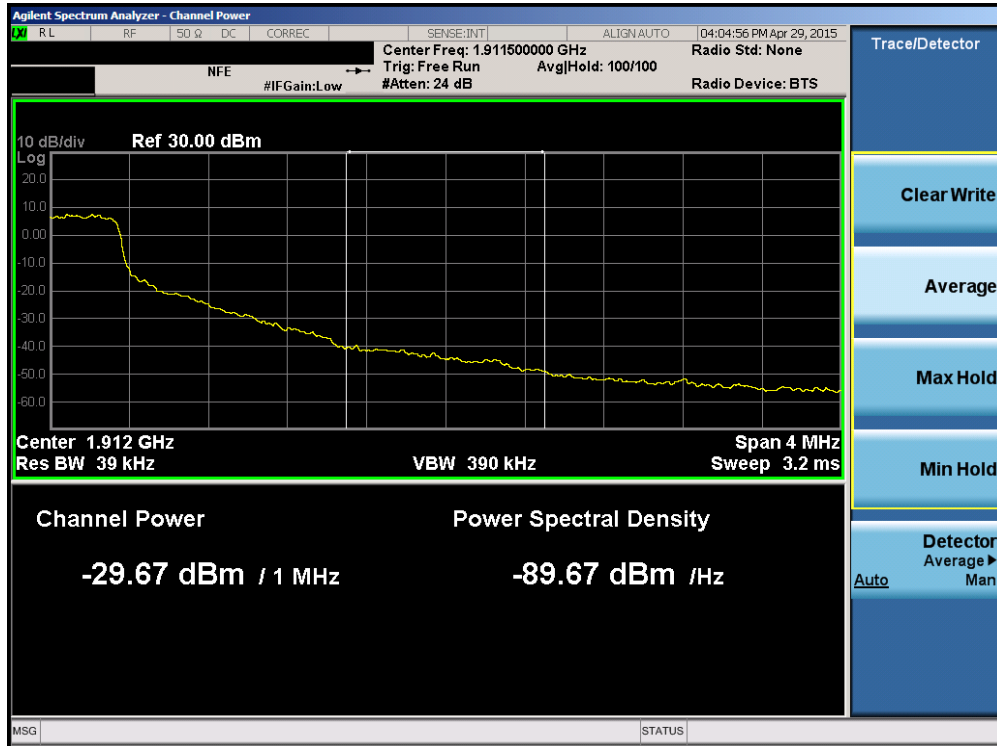
Plot 6-122. Upper Extended Band Edge Plot (Band 2 – 1.4MHz QPSK – RB Size 6)
