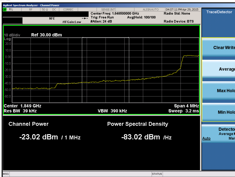
Plot 6-124. Lower Extended Band Edge Plot (Band 2 – 3.0MHz QPSK – RB Size 15)
