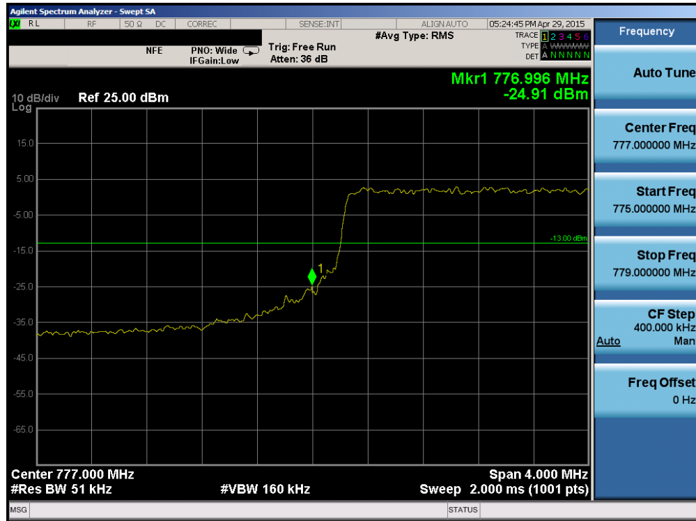
Plot 6-73. Lower Band Edge Plot (Band 13 – 5.0MHz QPSK – RB Size 25)
