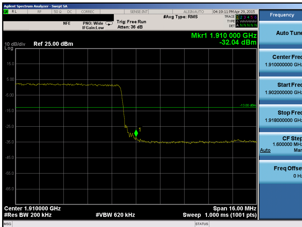
Plot 6-141. Upper Band Edge Plot (Band 2 – 20.0MHz QPSK – RB Size 100)
