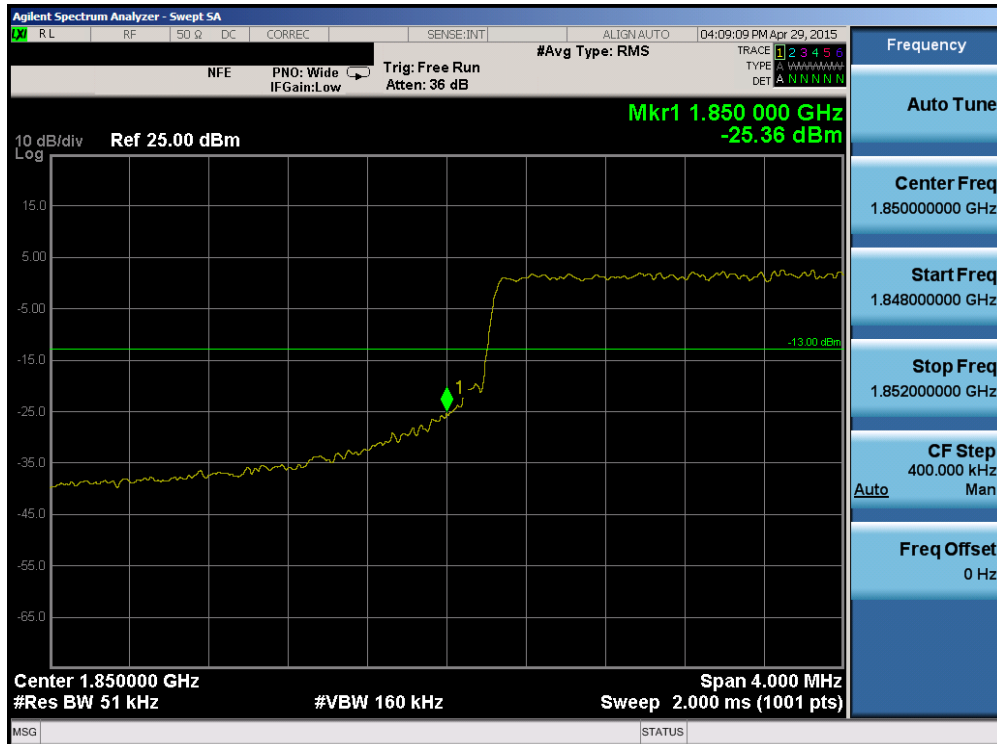
Plot 6-127. Lower Band Edge Plot (Band 2 – 5.0MHz QPSK – RB Size 25)
