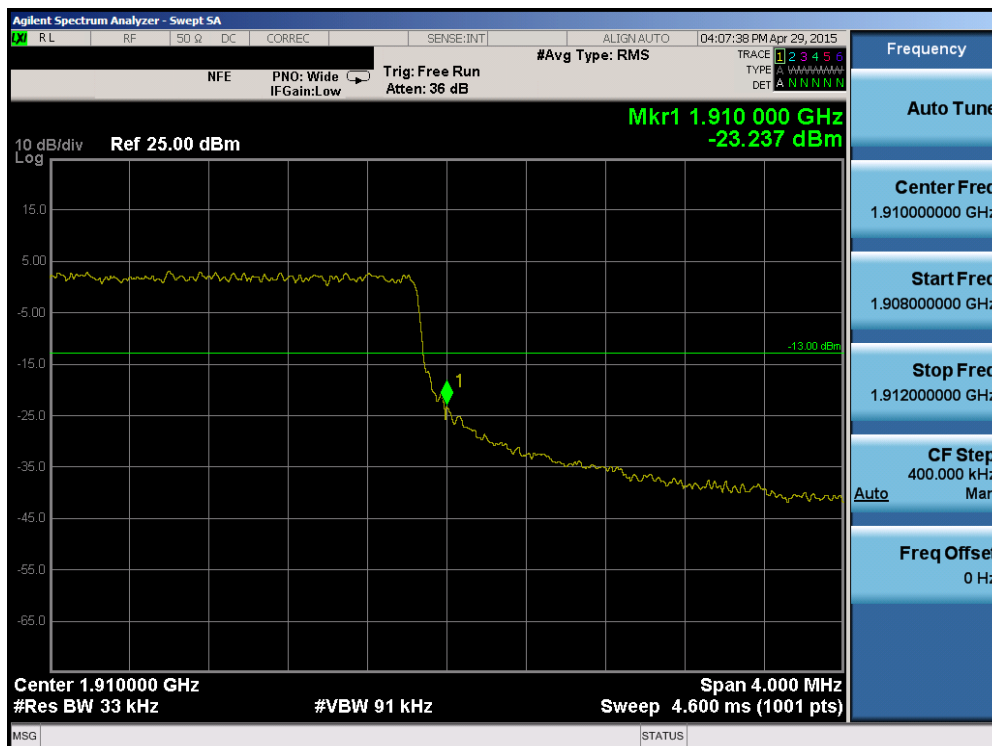
Plot 6-125. Upper Band Edge Plot (Band 2 – 3.0MHz QPSK – RB Size 15)
