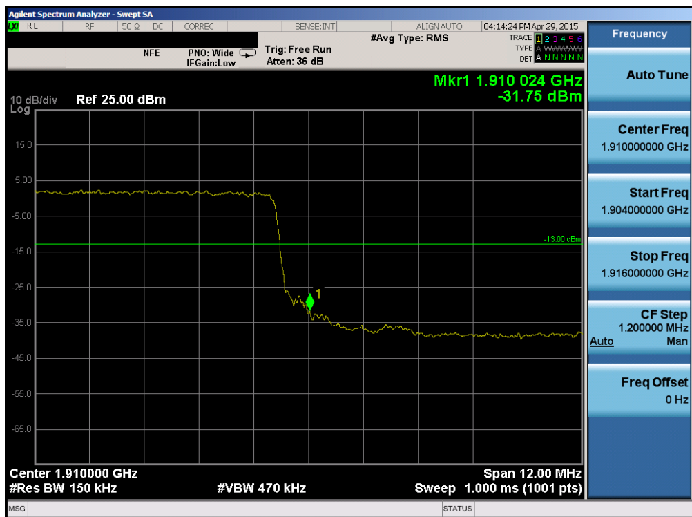
Plot 6-137. Upper Band Edge Plot (Band 2 – 15.0MHz QPSK – RB Size 75)
