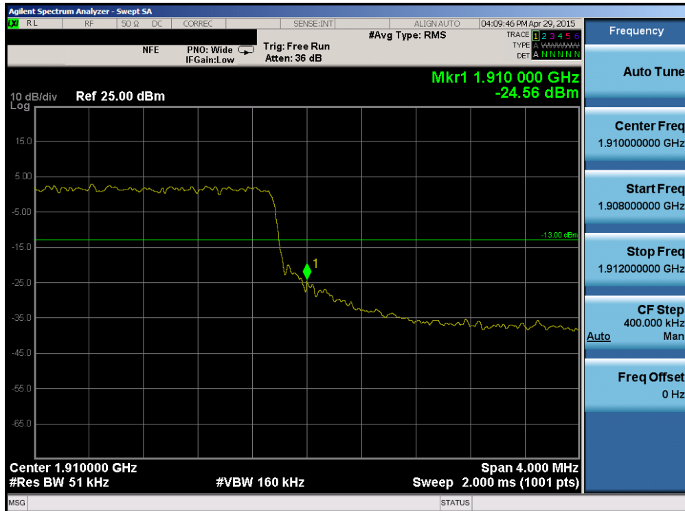
Plot 6-129. Upper Band Edge Plot (Band 2 – 5.0MHz QPSK – RB Size 25)
