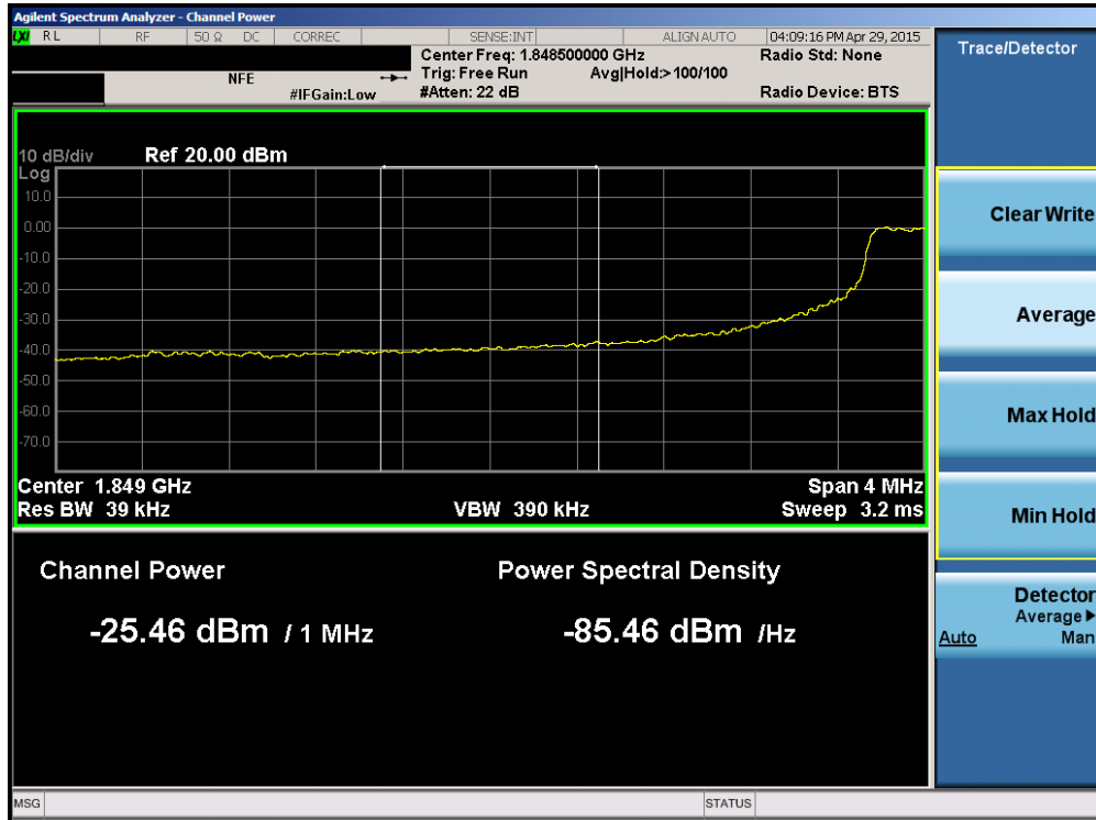
Plot 6-128. Lower Extended Band Edge Plot (Band 2 – 5.0MHz QPSK – RB Size 25)
