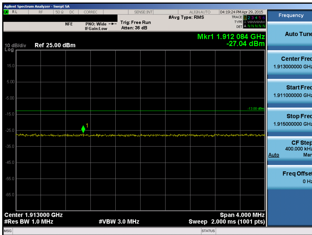
Plot 6-142. Upper Extended Band Edge Plot (Band 2 – 20.0MHz QPSK – RB Size 100)
