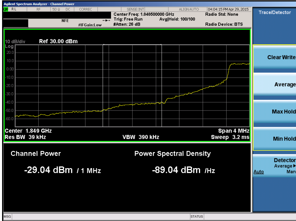
Plot 6-120. Lower Extended Band Edge Plot (Band 2 – 1.4MHz QPSK – RB Size 6)
