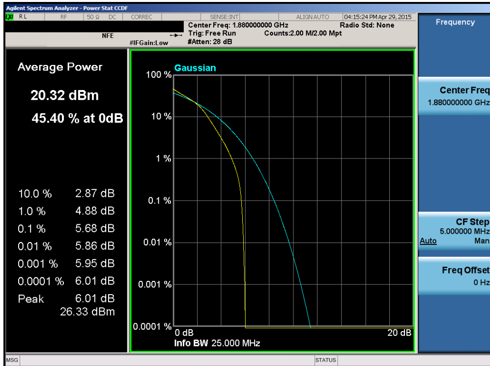
Plot 6-154. PAR Plot (Band 2 – 20.0MHz 16-QAM – RB Size 100)
