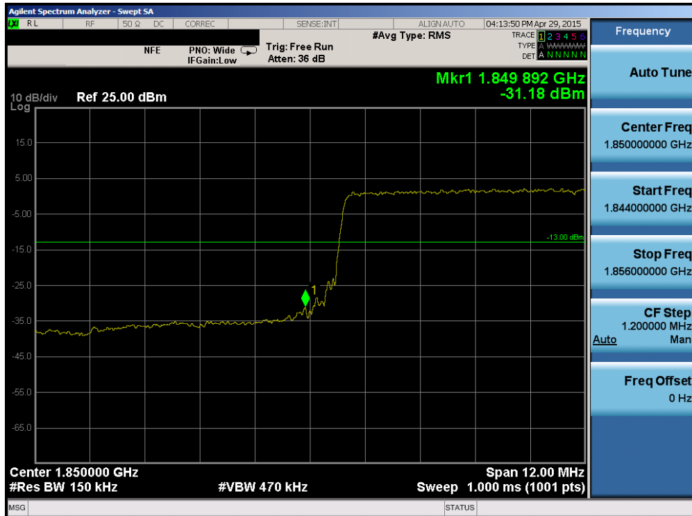
Plot 6-135. Lower Band Edge Plot (Band 2 – 15.0MHz QPSK – RB Size 75)
