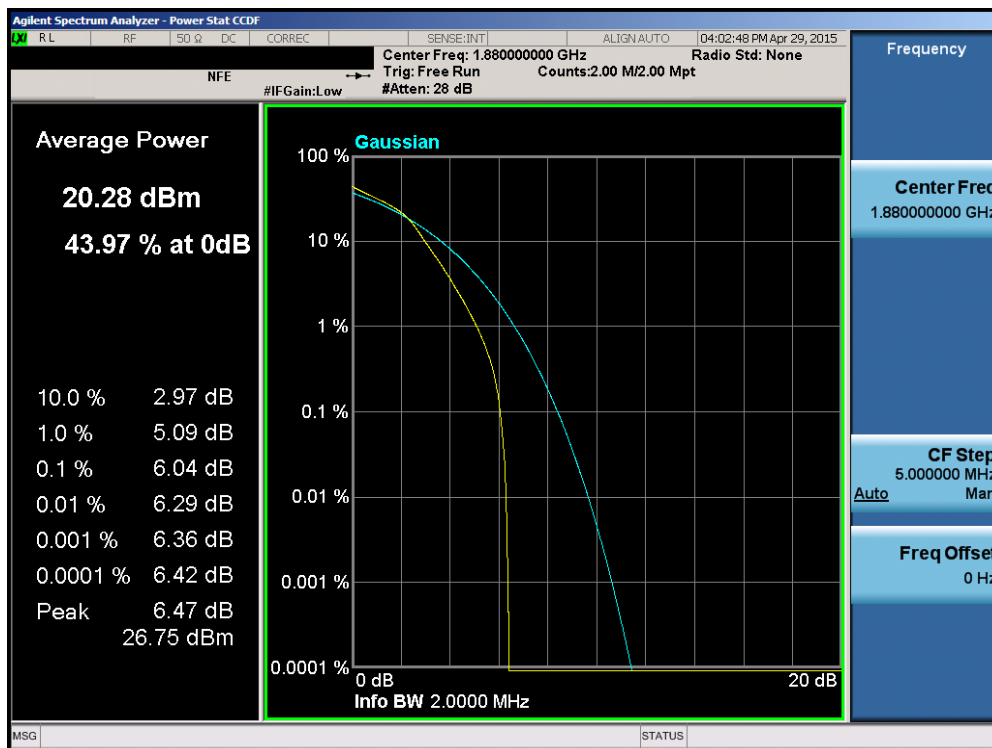
Plot 6-144. PAR Plot (Band 2 – 1.4MHz 16-QAM – RB Size 6)
