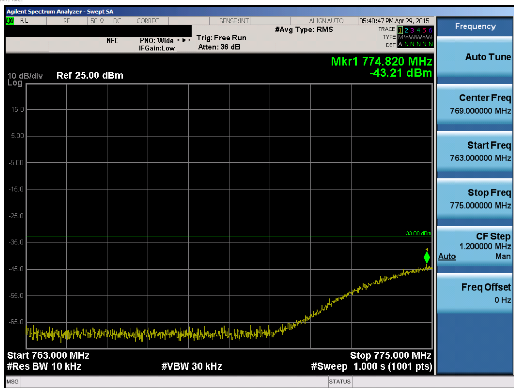
Plot 6-78. Lower Emission Mask Edge Plot (Band 13 – 10.0MHz QPSK – RB Size 50)
