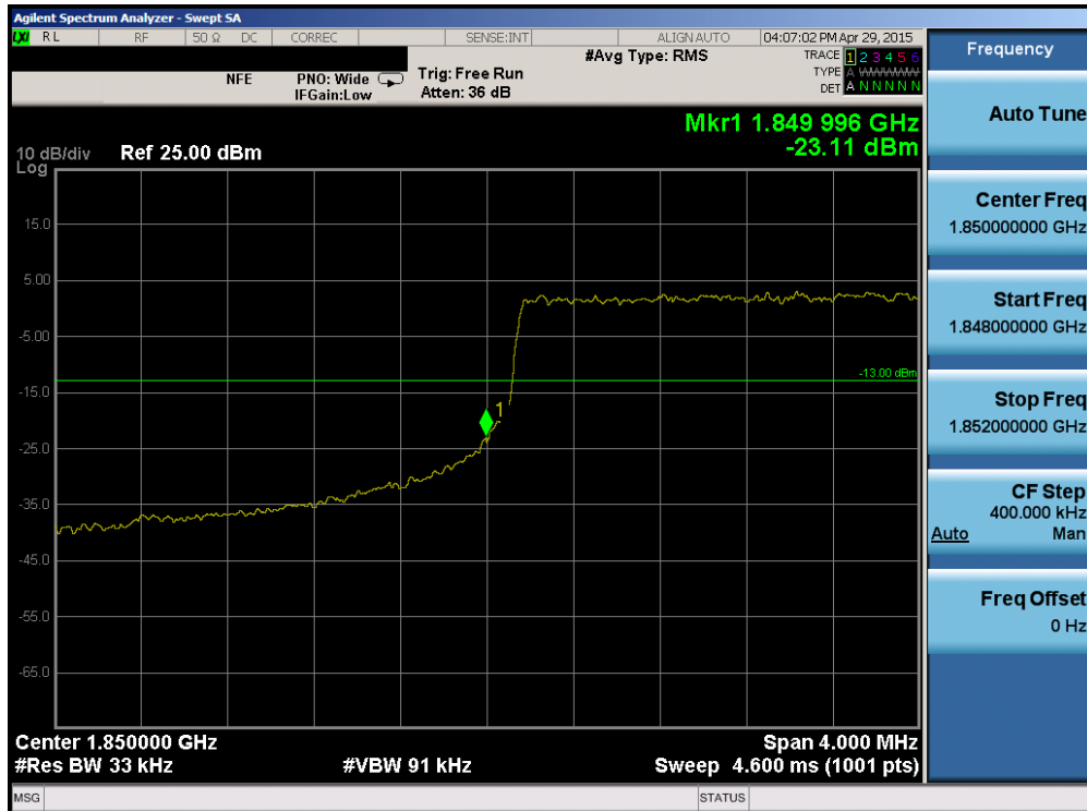
Plot 6-123. Lower Band Edge Plot (Band 2 – 3.0MHz QPSK – RB Size 15)
