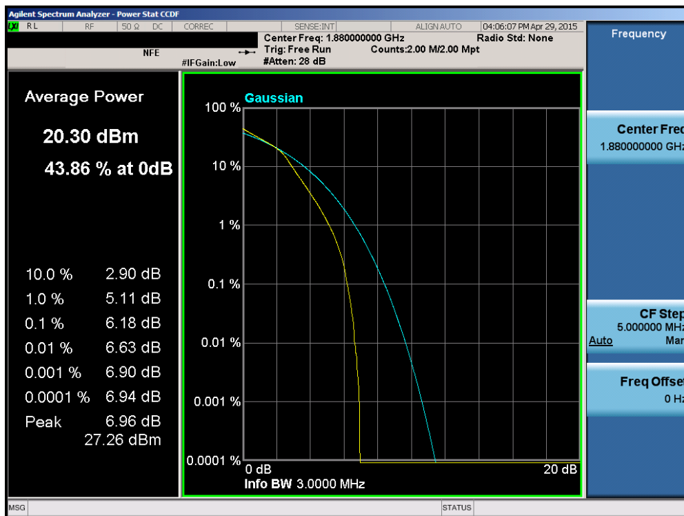
Plot 6-146. PAR Plot (Band 2 – 3.0MHz 16-QAM – RB Size 15)
