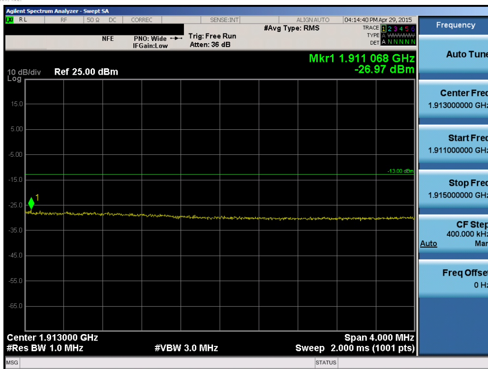
Plot 6-138. Upper Extended Band Edge Plot (Band 2 – 15.0MHz QPSK – RB Size 75)
