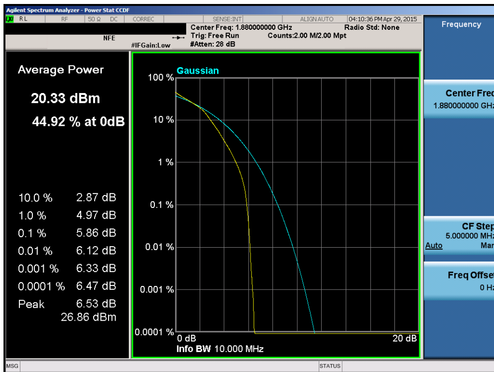
Plot 6-150. PAR Plot (Band 2 – 10.0MHz 16-QAM – RB Size 50)
