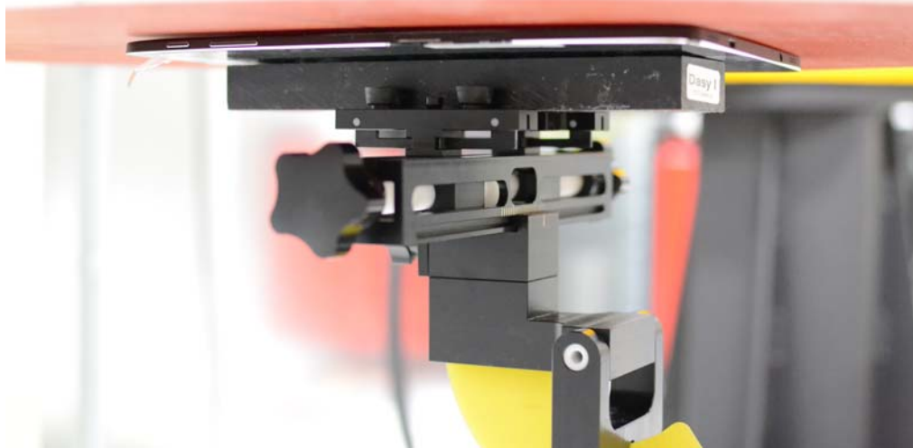
SAR Test Setup Photo 1: Back Side at 0.0 cm
