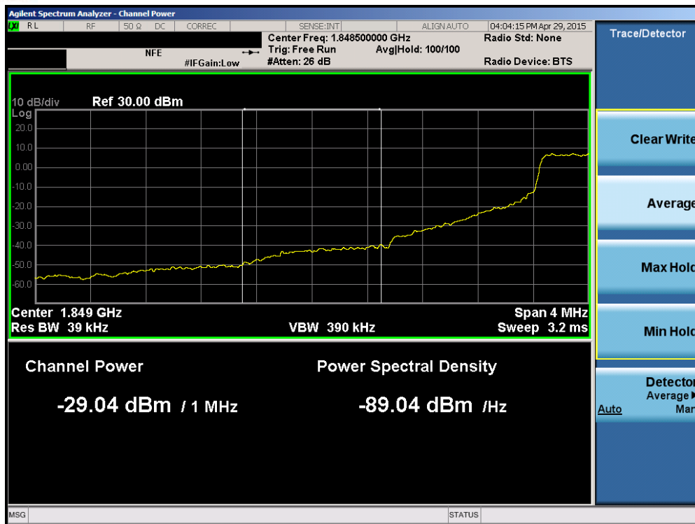
Plot 6-151. Lower Extended Band Edge Plot (Band 2 – 1.4MHz QPSK – RB Size 6)
