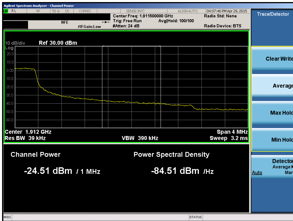
Plot 6-157. Upper Extended Band Edge Plot (Band 2 – 3.0MHz QPSK – RB Size 15)
