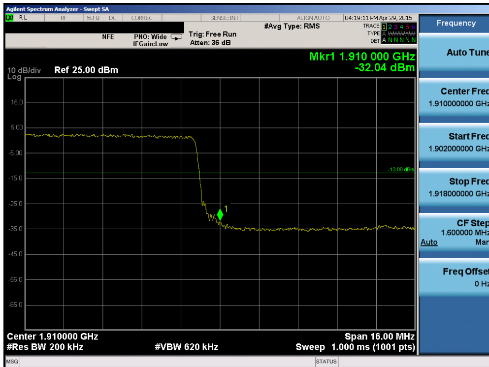
Plot 6-172. Upper Band Edge Plot (Band 2 – 20.0MHz QPSK – RB Size 100)
