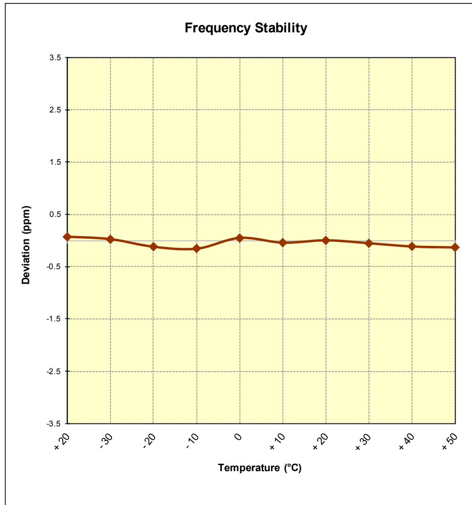
Figure 6-10. Frequency Stability Graph (Band 4)
