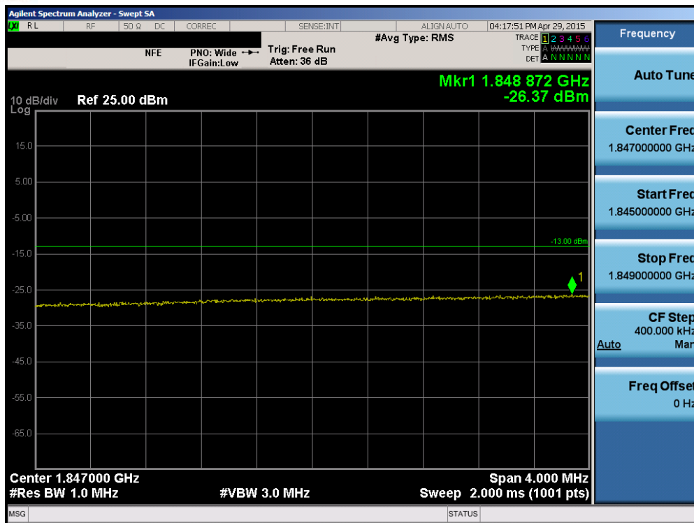
Plot 6-171. Lower Extended Band Edge Plot (Band 2 – 20.0MHz QPSK – RB Size 100)
