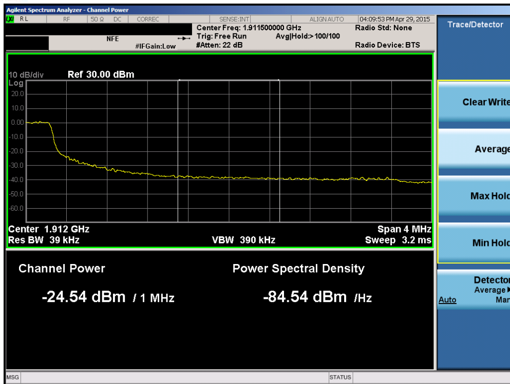
Plot 6-161. Upper Extended Band Edge Plot (Band 2 – 5.0MHz QPSK – RB Size 25)
