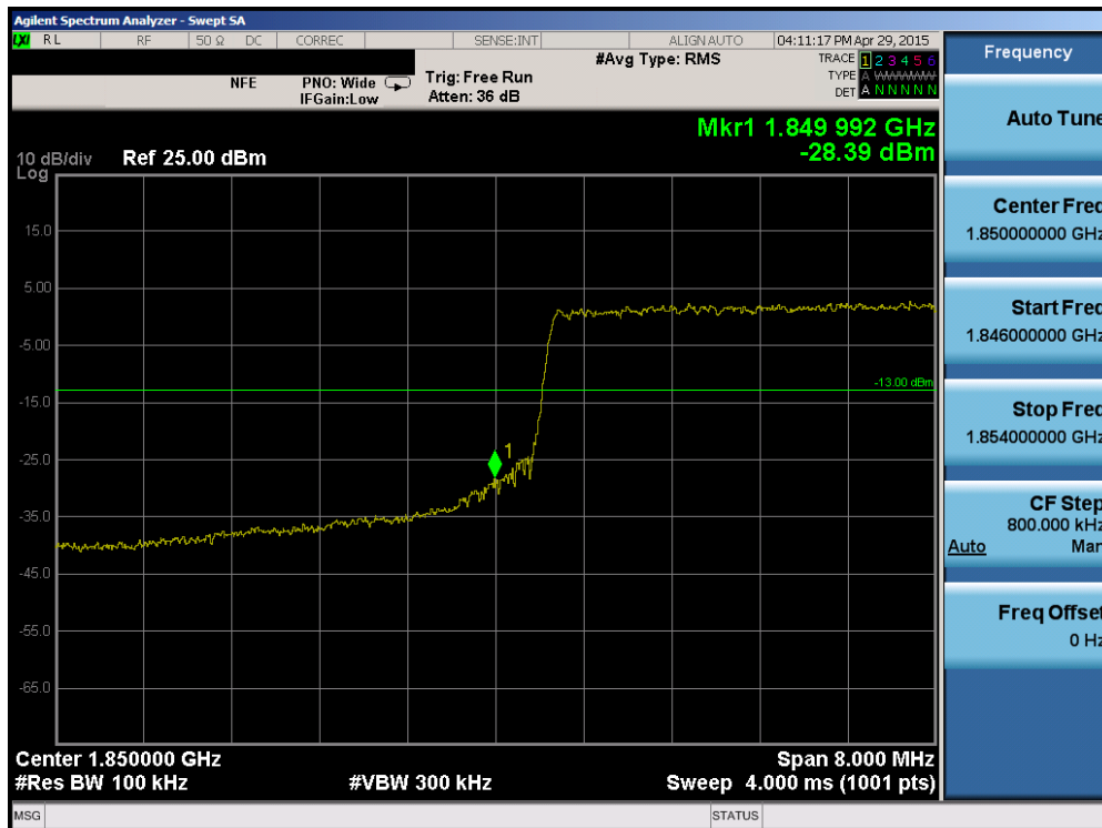
Plot 6-162. Lower Band Edge Plot (Band 2 – 10.0MHz QPSK – RB Size 50)
