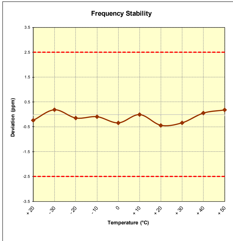
Figure 6-8. Frequency Stability Graph (Band 13)
