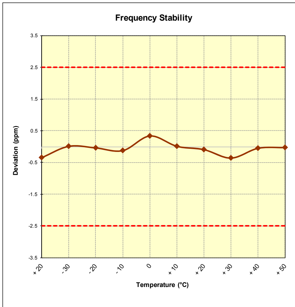
Figure 6-9. Frequency Stability Graph (Band 5)
