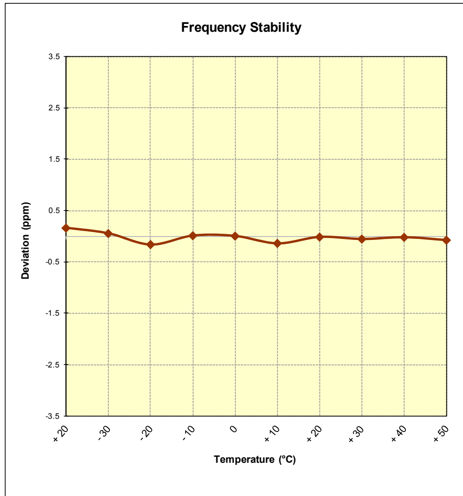
Figure 6-11. Frequency Stability Graph (Band 2)
