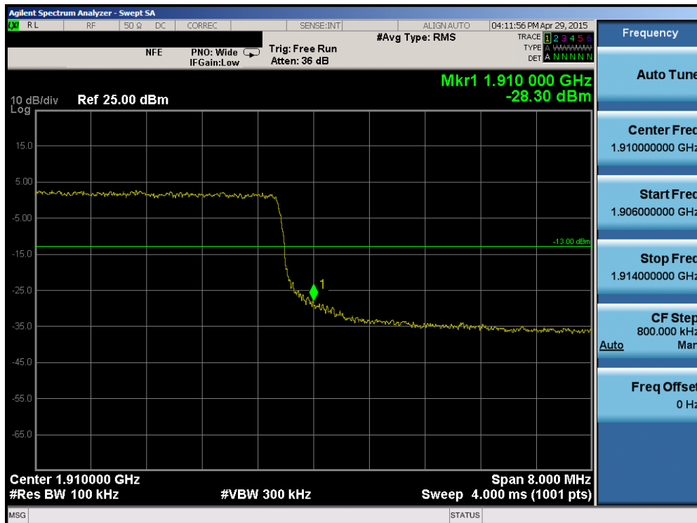
Plot 6-164. Upper Band Edge Plot (Band 2 – 10.0MHz QPSK – RB Size 50)
