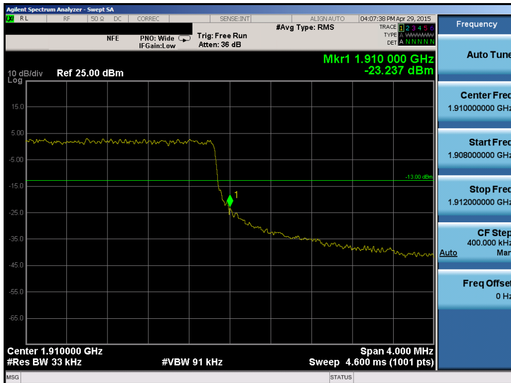
Plot 6-156. Upper Band Edge Plot (Band 2 – 3.0MHz QPSK – RB Size 15)
