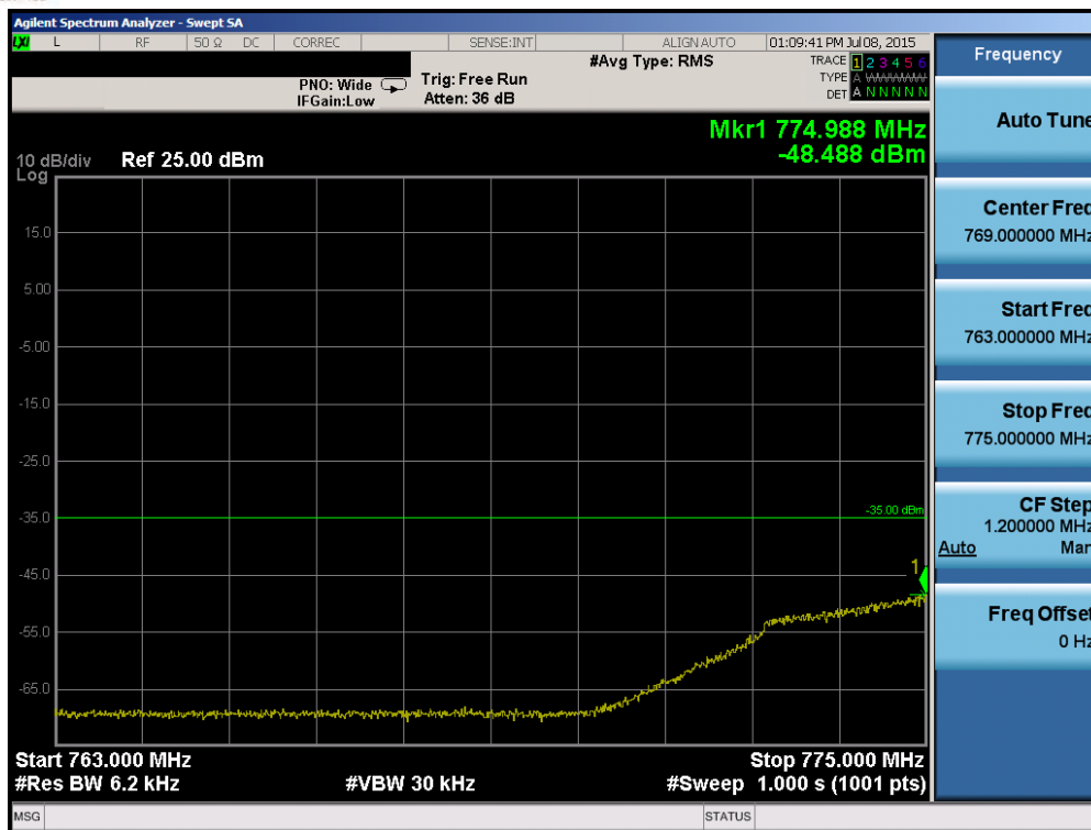
Plot 6-105. Lower Emission Mask Edge Plot (Band 13 - 5.0MHz QPSK - RB Size 25)
