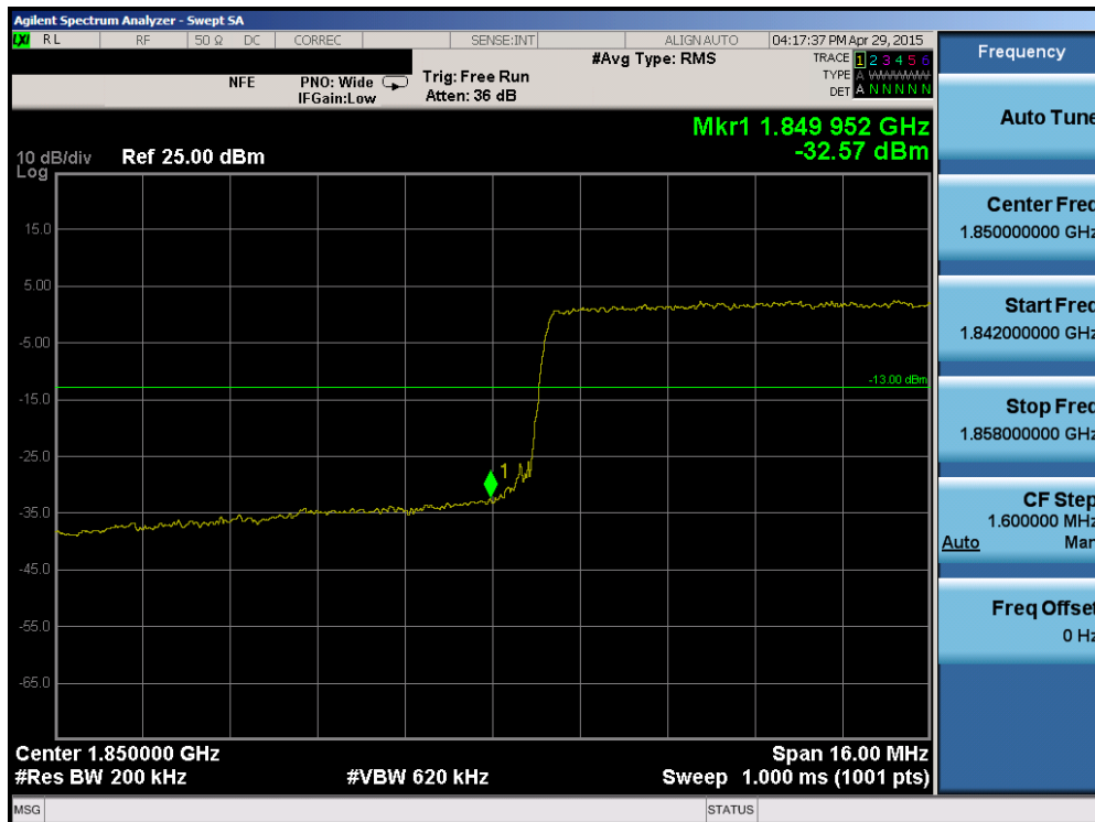
Plot 6-170. Lower Band Edge Plot (Band 2 – 20.0MHz QPSK – RB Size 100)
