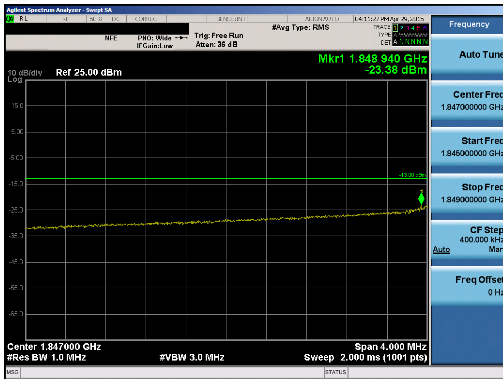
Plot 6-163. Lower Extended Band Edge Plot (Band 2 – 10.0MHz QPSK – RB Size 50)
