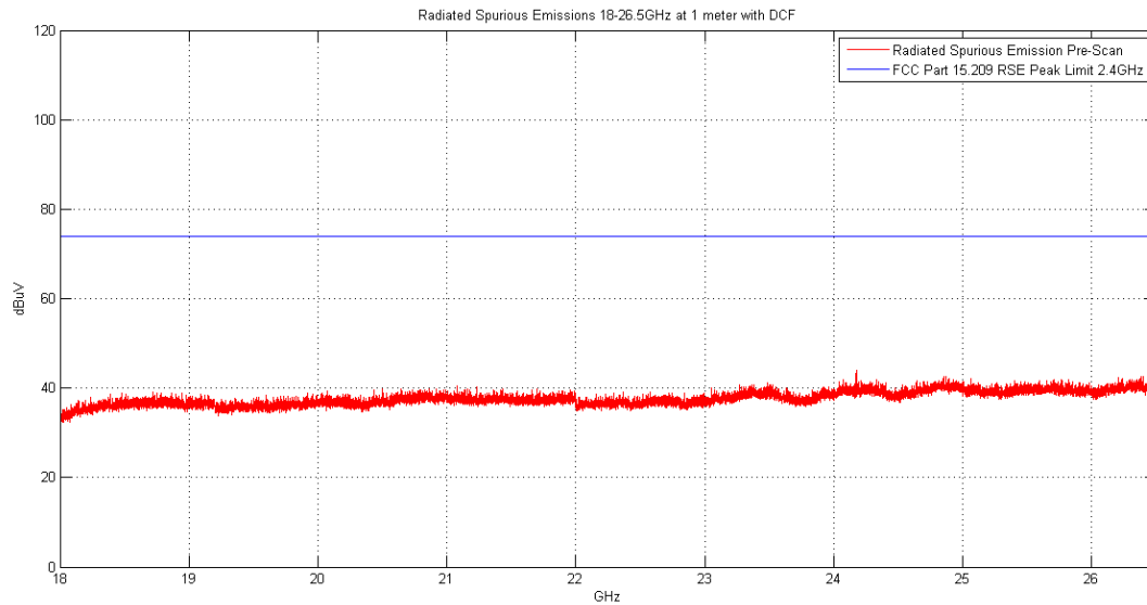
Plot 6-67. Radiated Spurious Plot above 18GHz (Pol. H)
