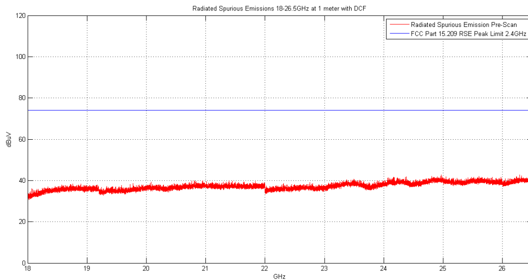
Plot 6-68. Radiated Spurious Plot above 18GHz (Pol. V)
