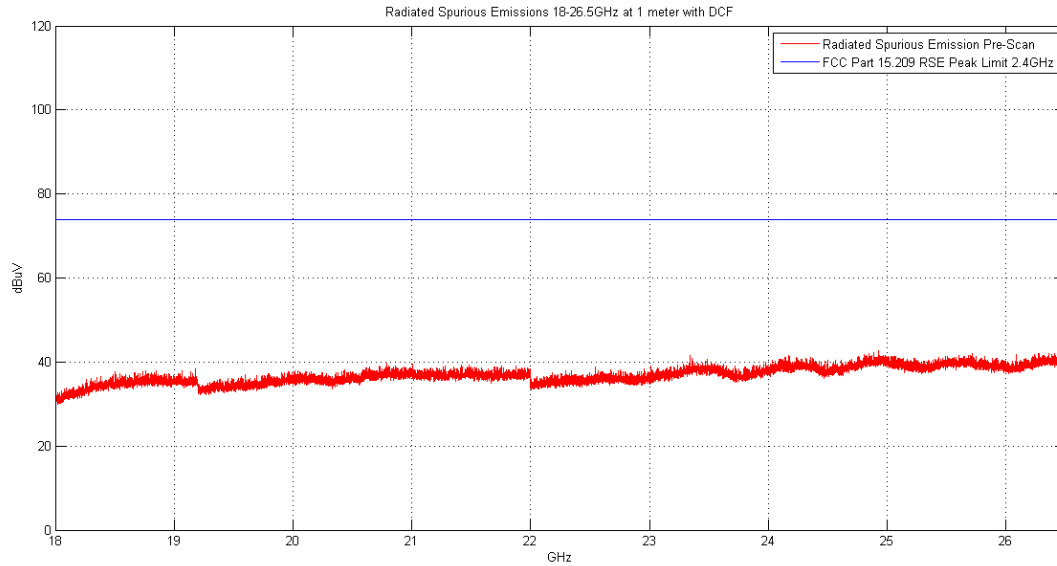
Plot 6-75. Radiated Spurious Plot above 18GHz (Pol. H)
