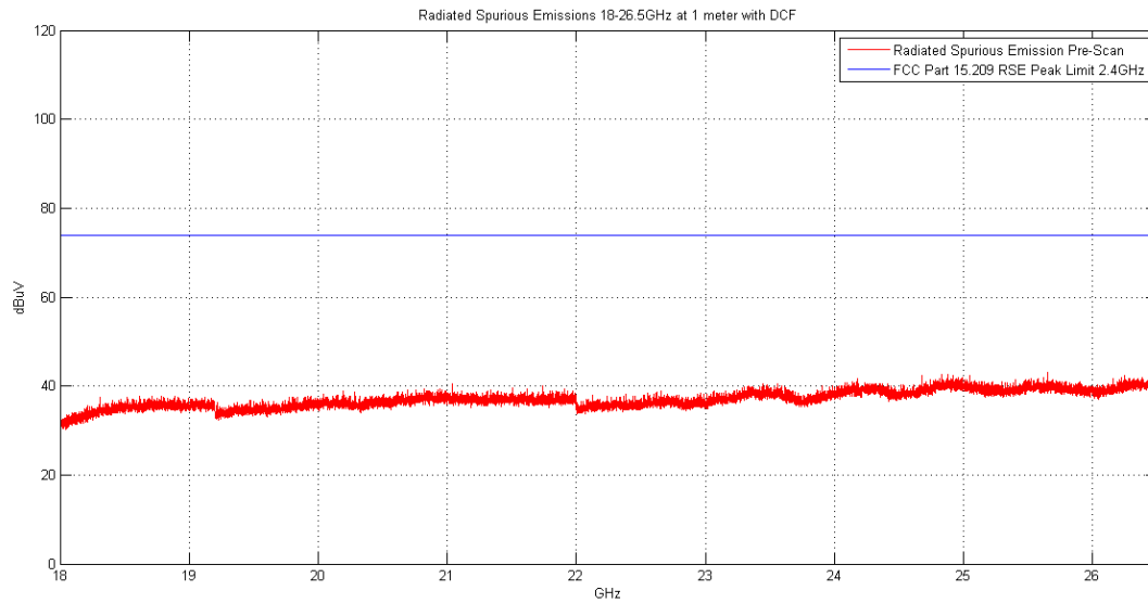
Plot 6-76. Radiated Spurious Plot above 18GHz (Pol. V)
