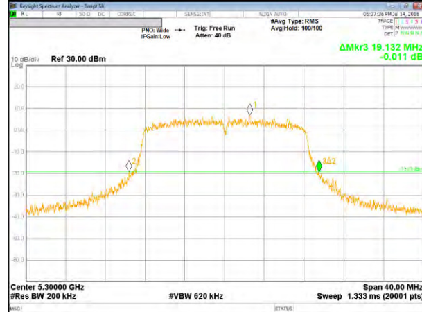
11a Mode High Channel Primary
