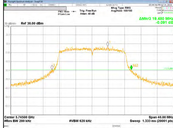
11a Mode Middle Channel Primary
