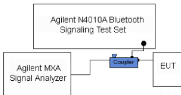
Figure 7-1 Power Measurement Setup
