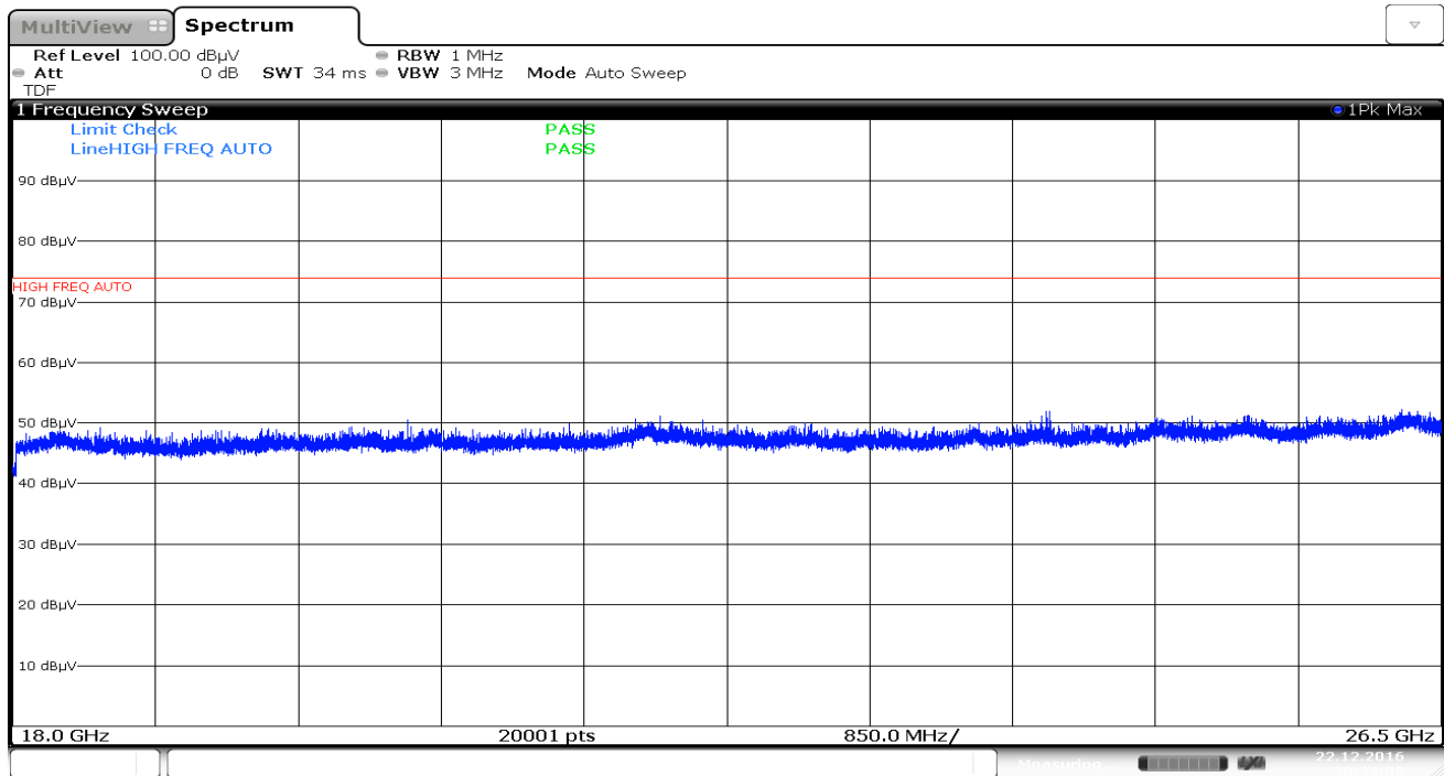
Plot 7-49. Radiated Spurious Plot above 18GHz (Pol. V)
