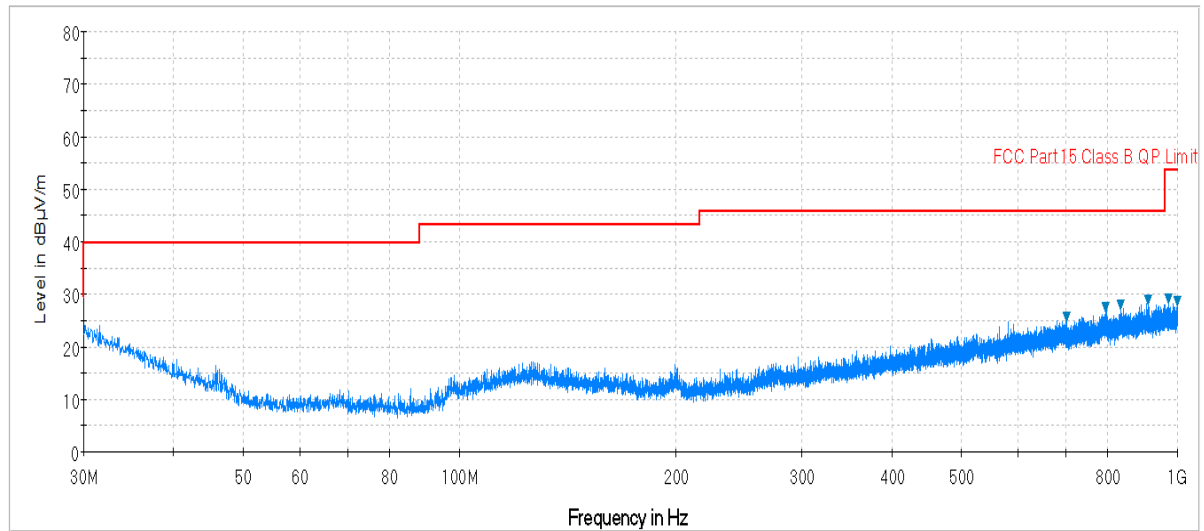
Plot 7-52. Radiated Spurious Plot below 1GHz (Pol. H)
