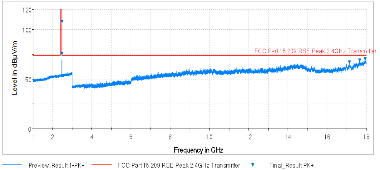
Plot 7-46. Radiated Spurious Plot above 1GHz (BT – Ch. 78, Ant. Pol. H)
