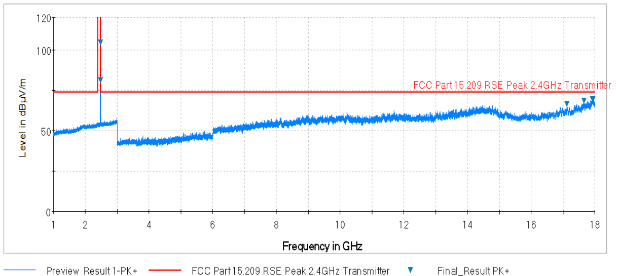
Plot 7-47. Radiated Spurious Plot above 1GHz (BT – Ch. 78, Ant. Pol. V)
