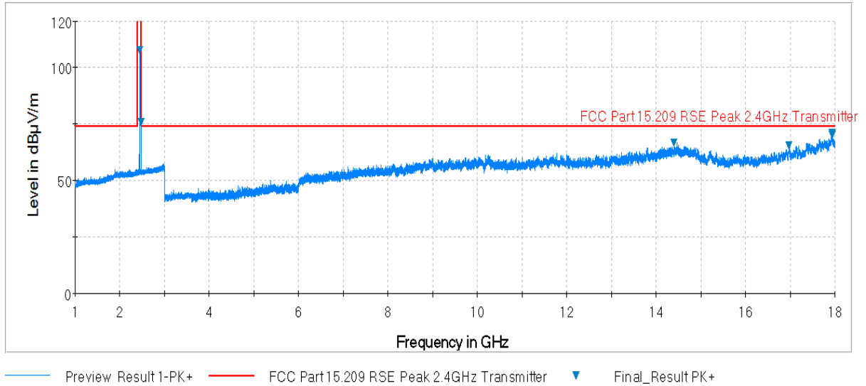
Plot 7-44. Radiated Spurious Plot above 1GHz (BT – Ch. 39, Ant. Pol. H)
