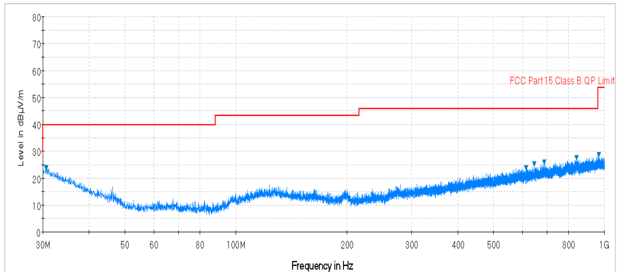
Plot 7-53. Radiated Spurious Plot below 1GHz (Pol. V)
