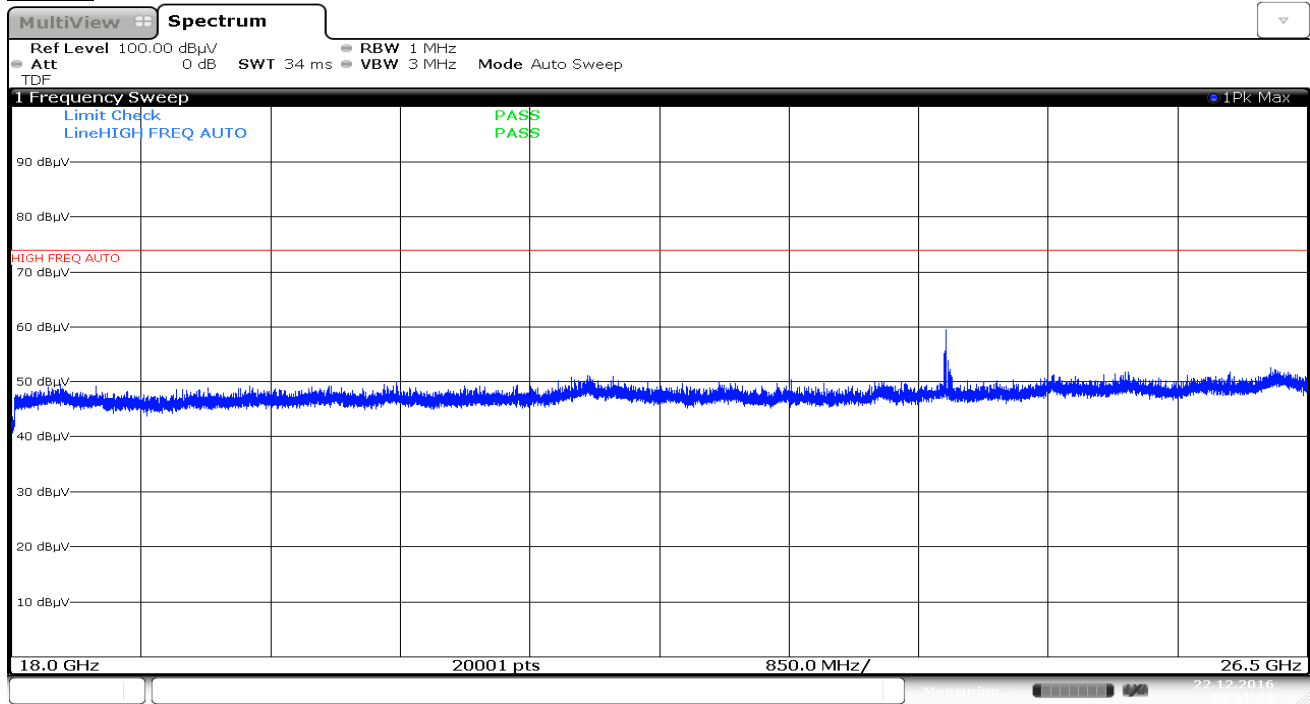
Plot 7-48. Radiated Spurious Plot above 18GHz (Pol. H)
