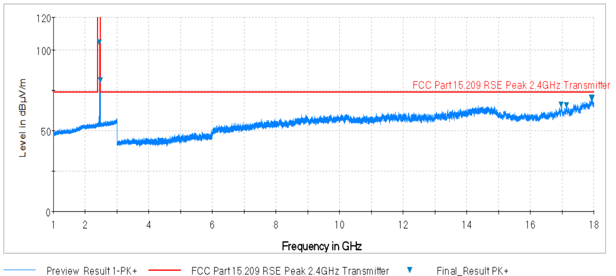
Plot 7-45. Radiated Spurious Plot above 1GHz (BT – Ch. 39, Ant. Pol. V)
