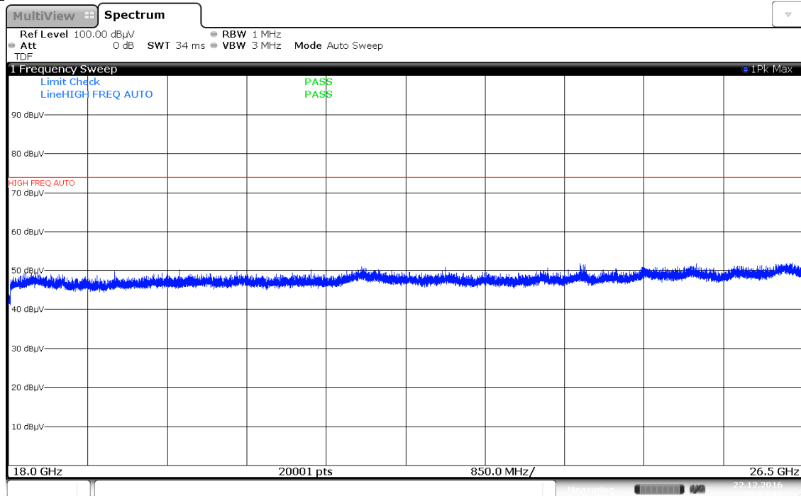
Plot 7-177. Radiated Spurious Plot above 18GHz (802.11a – Ant. Pol. H)
