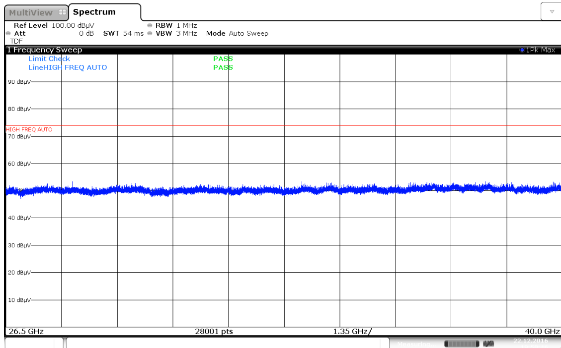
Plot 7-166. Radiated Spurious Plot above 26.5GHz (802.11a – Ant. Pol. H)
