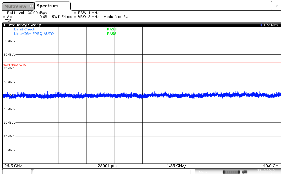
Plot 7-178. Radiated Spurious Plot above 26.5GHz (802.11a – Ant. Pol. H)
