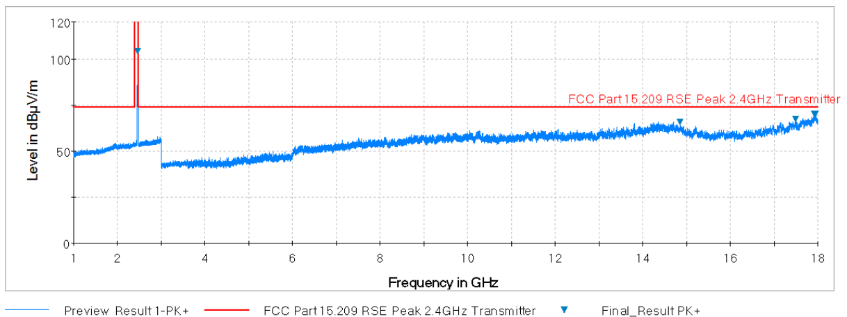
Plot 7-86. Radiated Spurious Plot above 1GHz (802.11b – Ch. 11, Ant. Pol. V)
