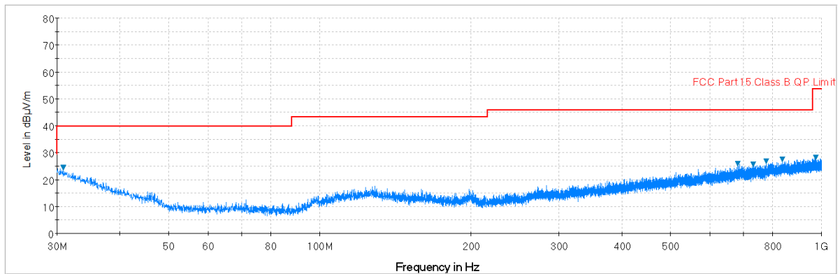
Plot 7-116. Radiated Spurious Plot below 1GHz (Pol. V)
