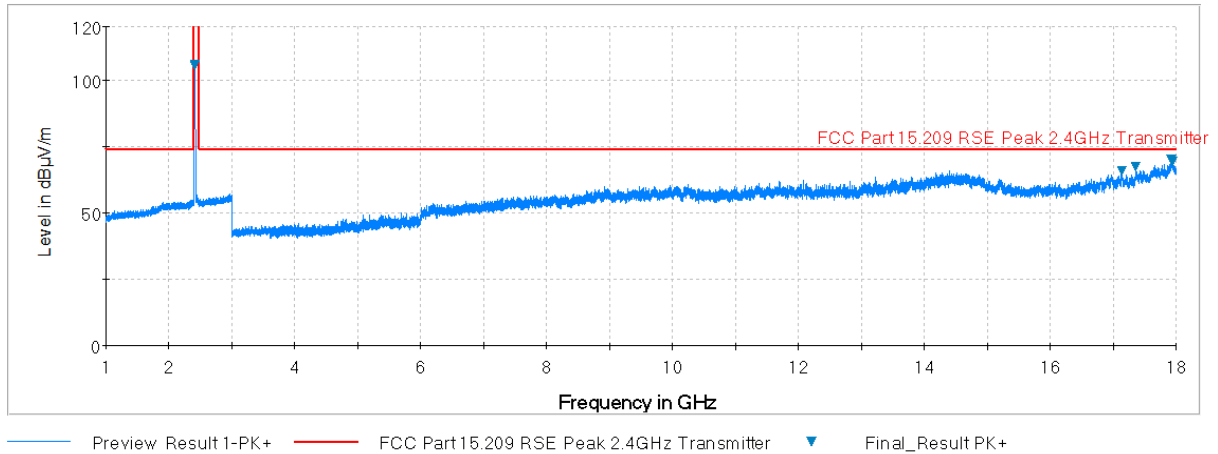
Plot 7-74. Radiated Spurious Plot above 1GHz (802.11b – Ch. 1, Ant. Pol. V)
