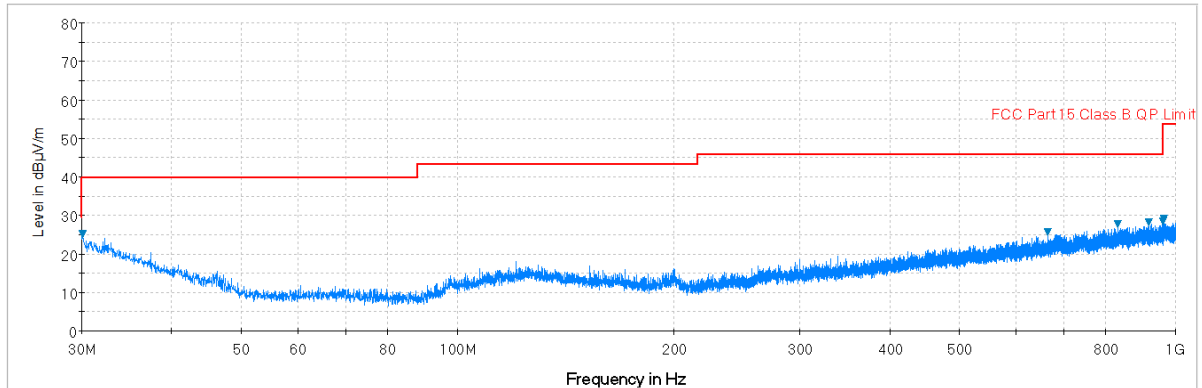
Plot 7-115. Radiated Spurious Plot below 1GHz (Pol. H)
