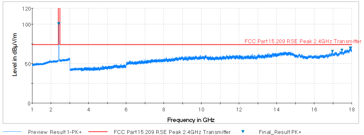
Plot 7-81. Radiated Spurious Plot above 1GHz (802.11b – Ch. 1, Ant. Pol. H)
