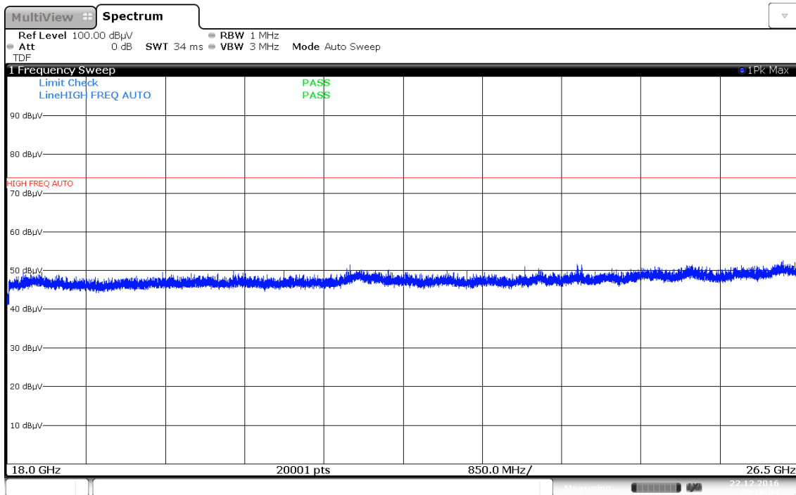
Plot 7-88. Radiated Spurious Plot above 18GHz (Pol. V)
