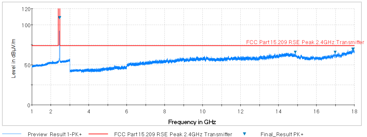
Plot 7-77. Radiated Spurious Plot above 1GHz (802.11b – Ch. 11, Ant. Pol. H)
