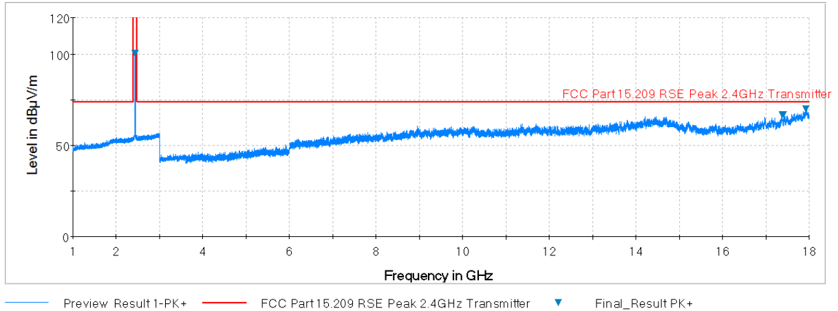
Plot 7-76. Radiated Spurious Plot above 1GHz (802.11b – Ch. 6, Ant. Pol. V)
