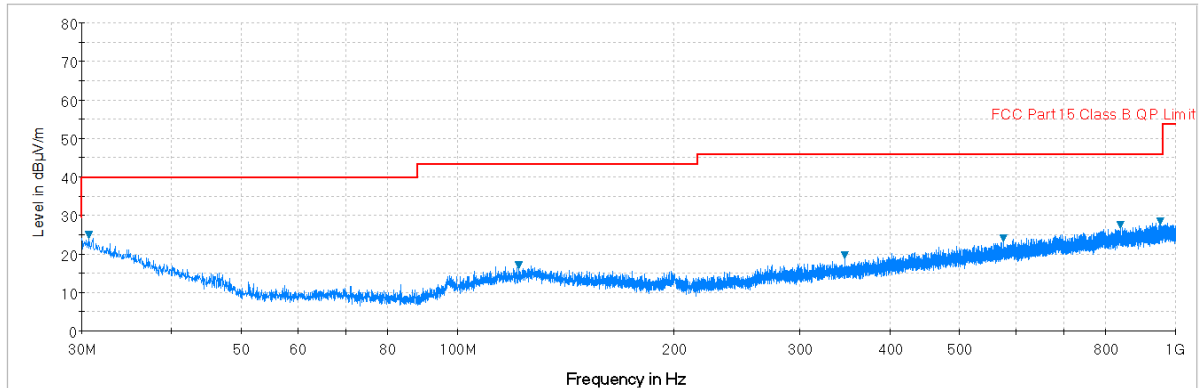
Plot 7-113. Radiated Spurious Plot below 1GHz (Pol. H)
