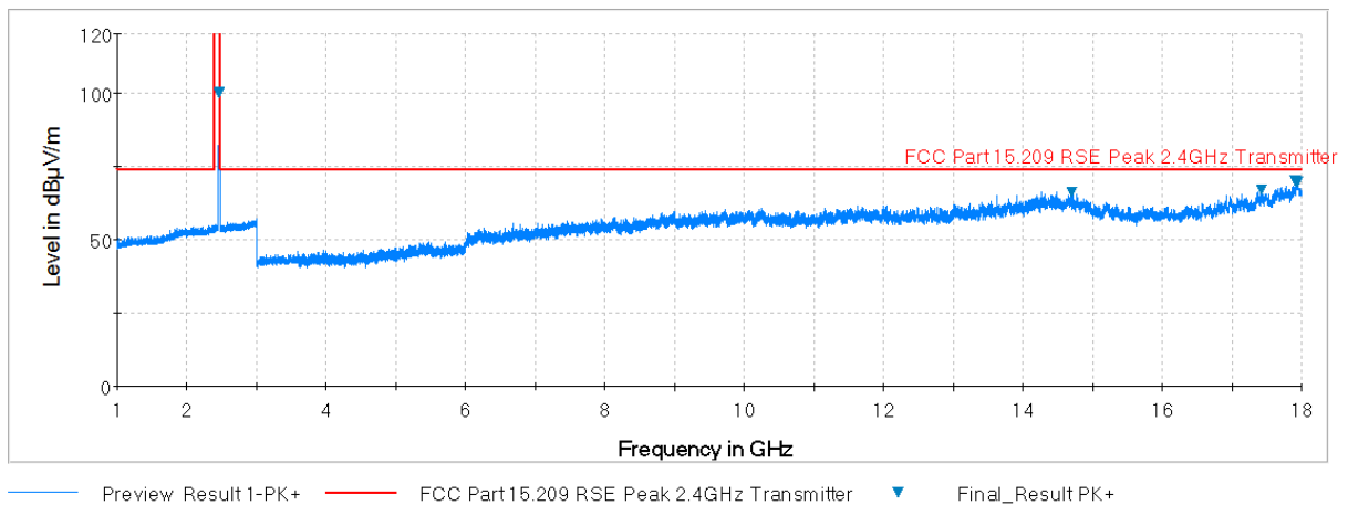
Plot 7-85. Radiated Spurious Plot above 1GHz (802.11b – Ch. 11, Ant. Pol. H)
