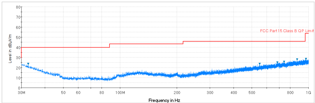
Plot 7-114. Radiated Spurious Plot below 1GHz (Pol. V)
