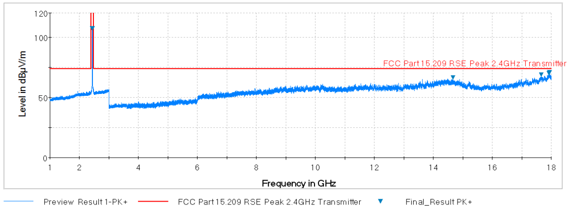
Plot 7-75. Radiated Spurious Plot above 1GHz (802.11b – Ch. 6, Ant. Pol. H)
