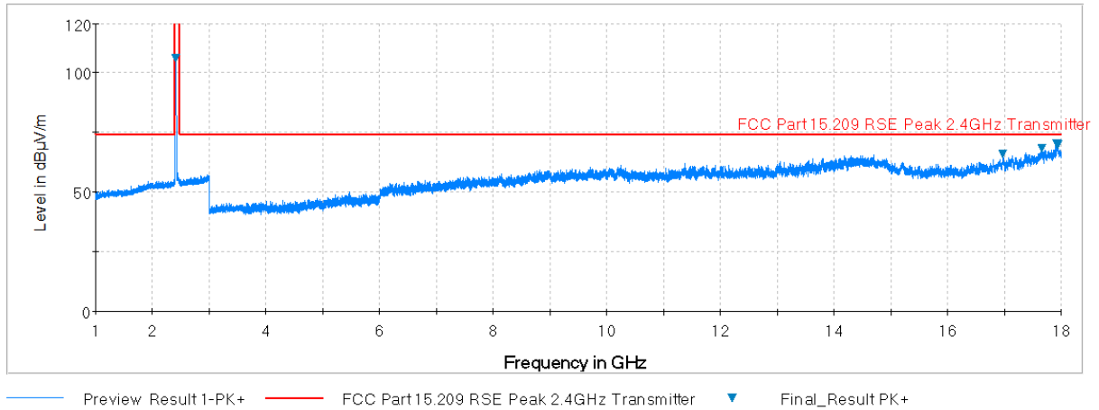
Plot 7-73. Radiated Spurious Plot above 1GHz (802.11b – Ch. 1, Ant. Pol. H)
