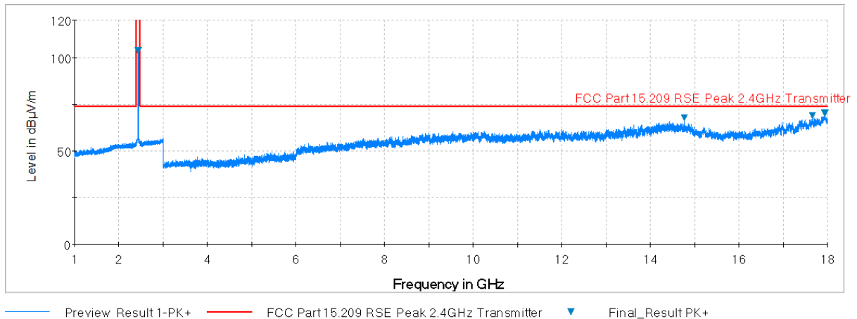
Plot 7-84. Radiated Spurious Plot above 1GHz (802.11b – Ch. 6, Ant. Pol. V)
