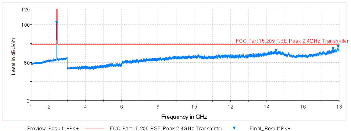
Plot 7-82. Radiated Spurious Plot above 1GHz (802.11b – Ch. 1, Ant. Pol. V)
