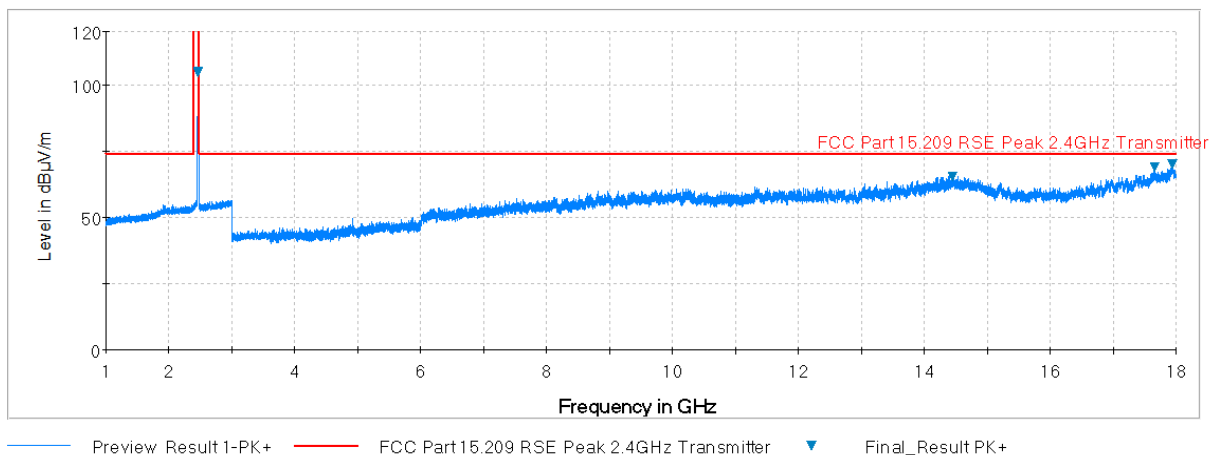
Plot 7-78. Radiated Spurious Plot above 1GHz (802.11b – Ch. 11, Ant. Pol. V)
