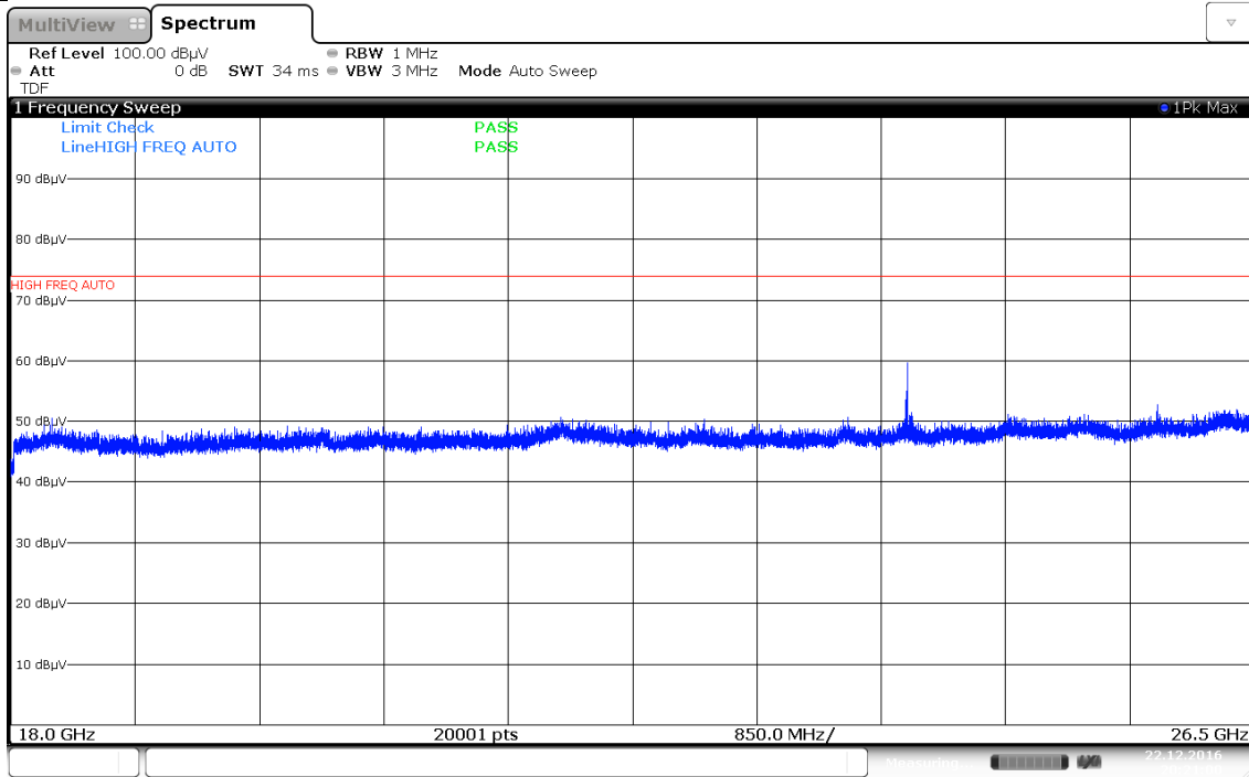
Plot 7-87. Radiated Spurious Plot above 18GHz (Pol. H)
