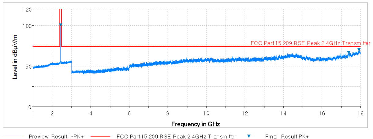
Plot 7-83. Radiated Spurious Plot above 1GHz (802.11b – Ch. 6, Ant. Pol. H)
