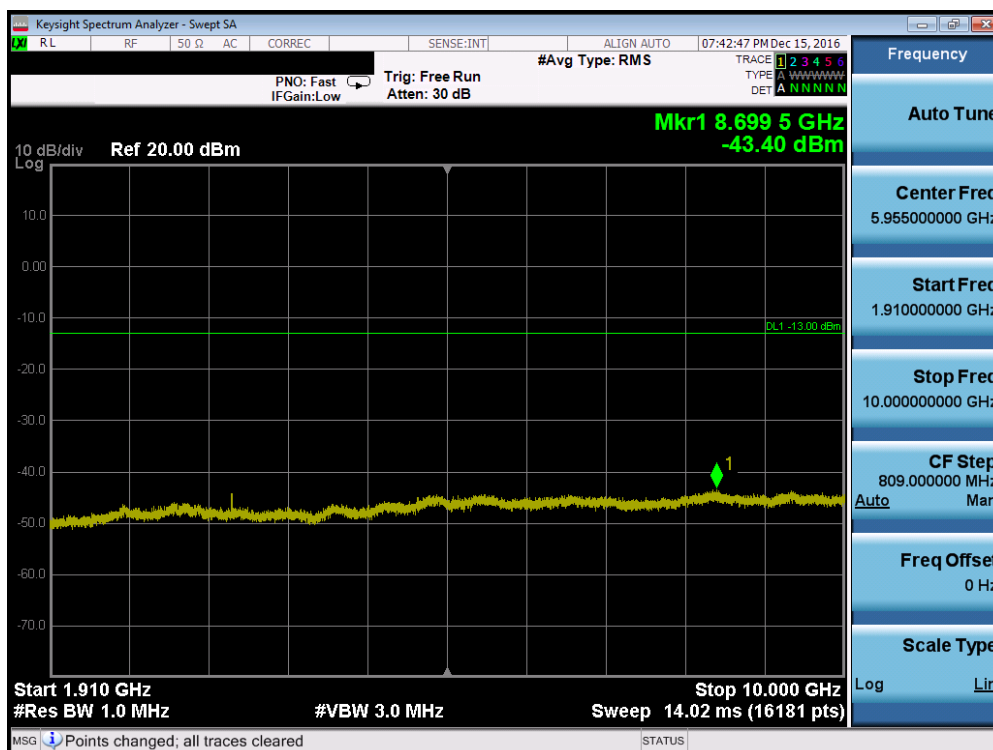
Plot 7-68. Conducted Spurious Plot (Band 2 – 3.0MHz QPSK – RB Size 1, RB Offset 0 – Mid Channel)
