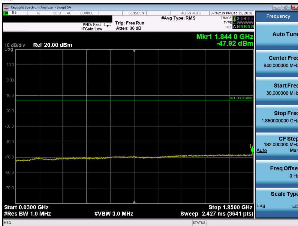
Plot 7-67. Conducted Spurious Plot (Band 2 – 3.0MHz QPSK – RB Size 1, RB Offset 0 – Mid Channel)
