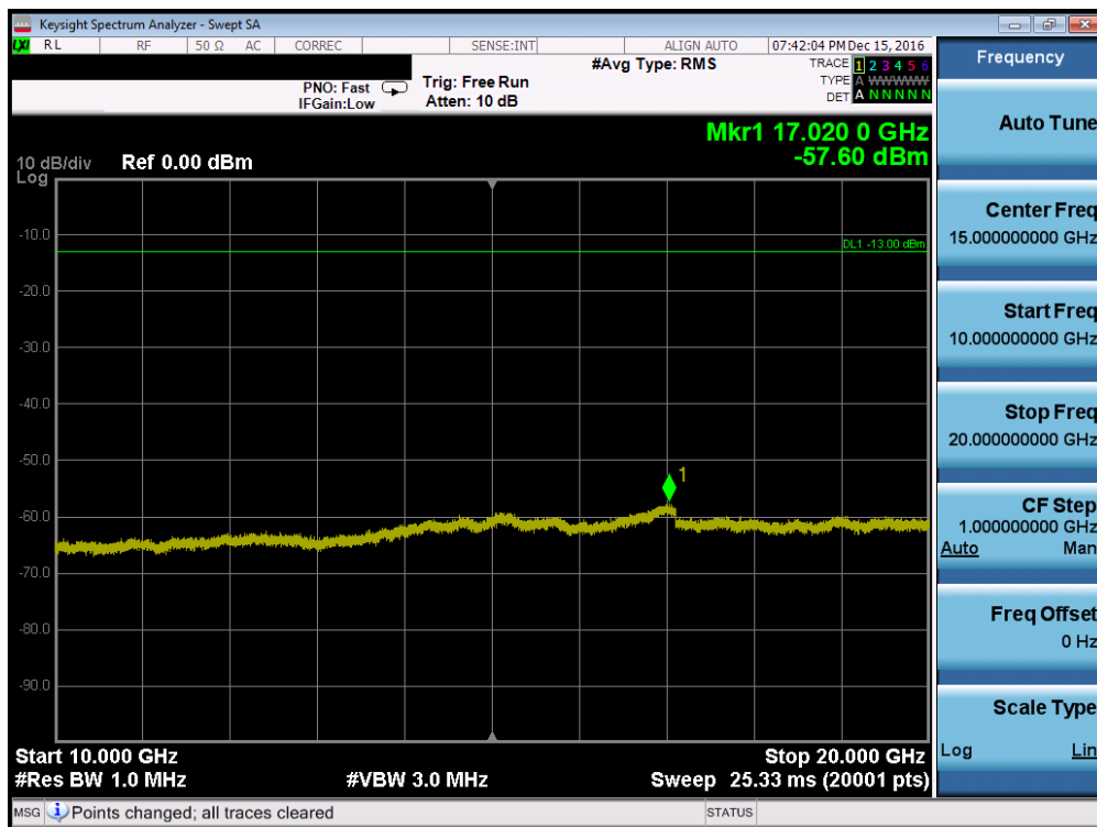
Plot 7-72. Conducted Spurious Plot (Band 2 – 3.0MHz QPSK – RB Size 1, RB Offset 0 – High Channel)
