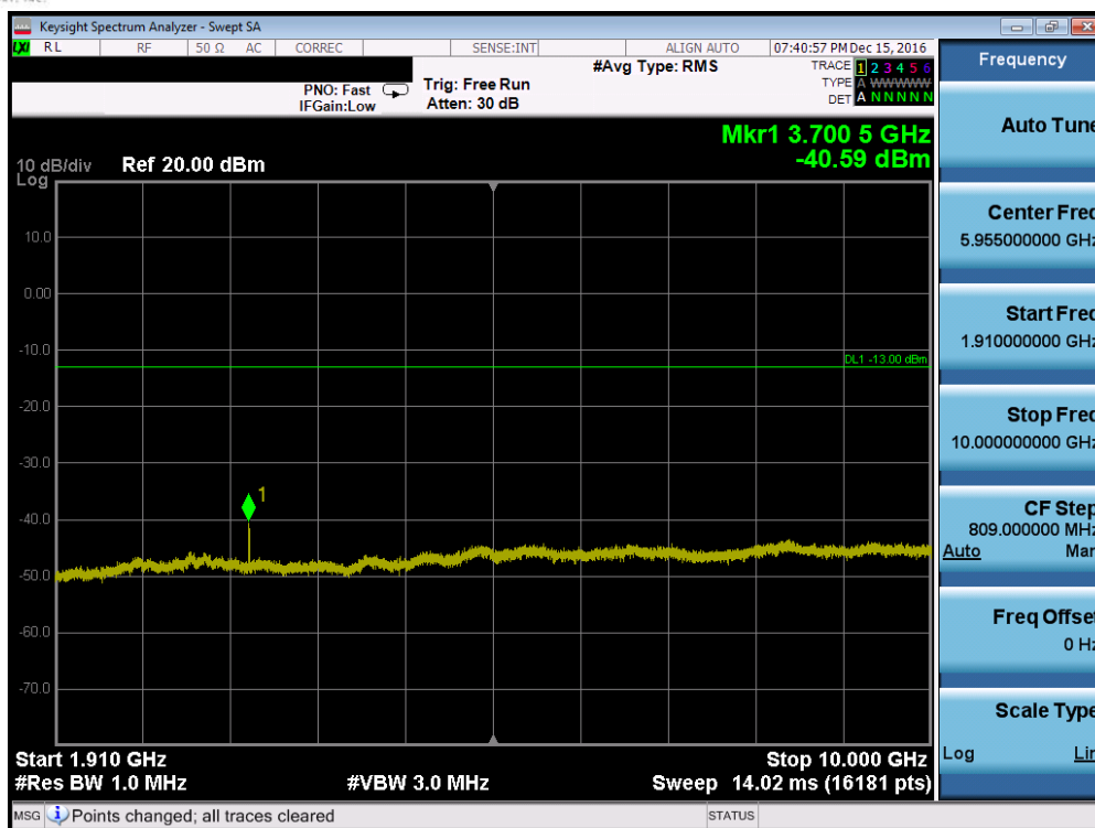
Plot 7-65. Conducted Spurious Plot (Band 2 – 3.0MHz QPSK – RB Size 1, RB Offset 0 – Low Channel)
