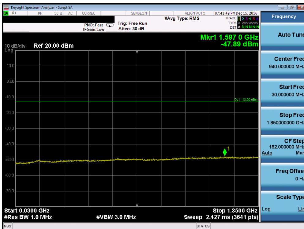
Plot 7-70. Conducted Spurious Plot (Band 2 – 3.0MHz QPSK – RB Size 1, RB Offset 0 – High Channel)
