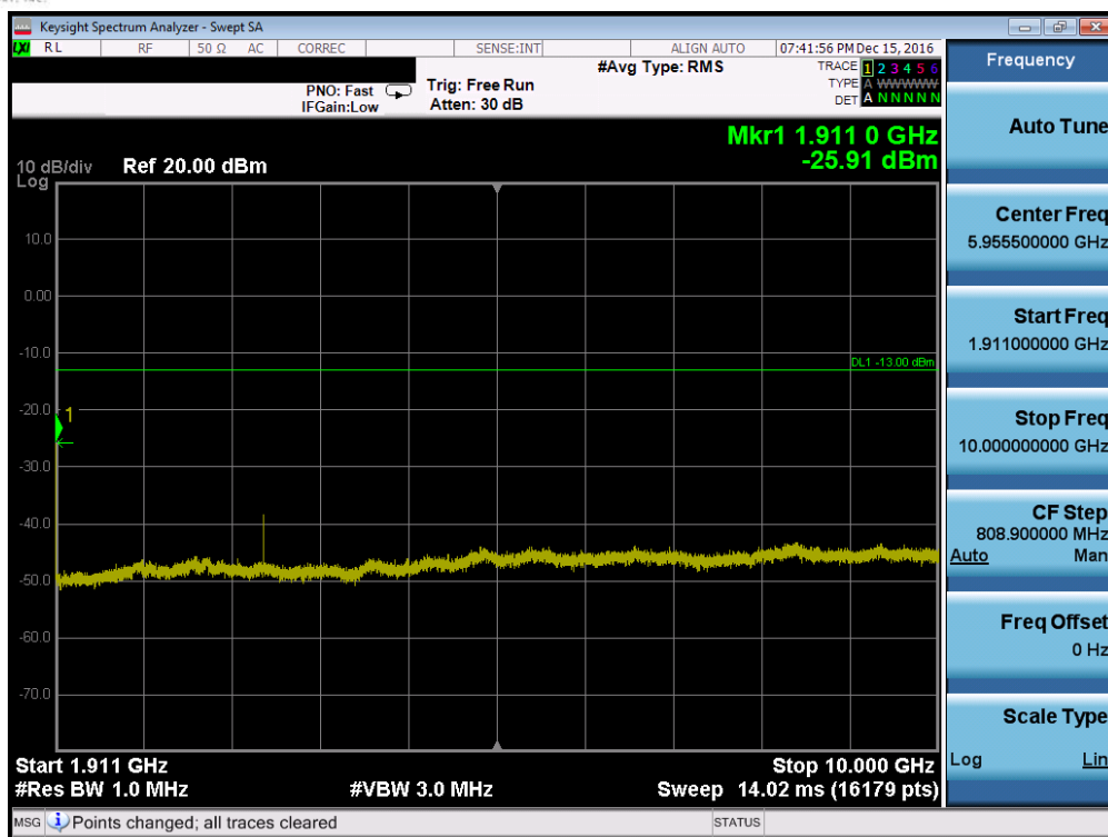
Plot 7-71. Conducted Spurious Plot (Band 2 – 3.0MHz QPSK – RB Size 1, RB Offset 0 – High Channel)
