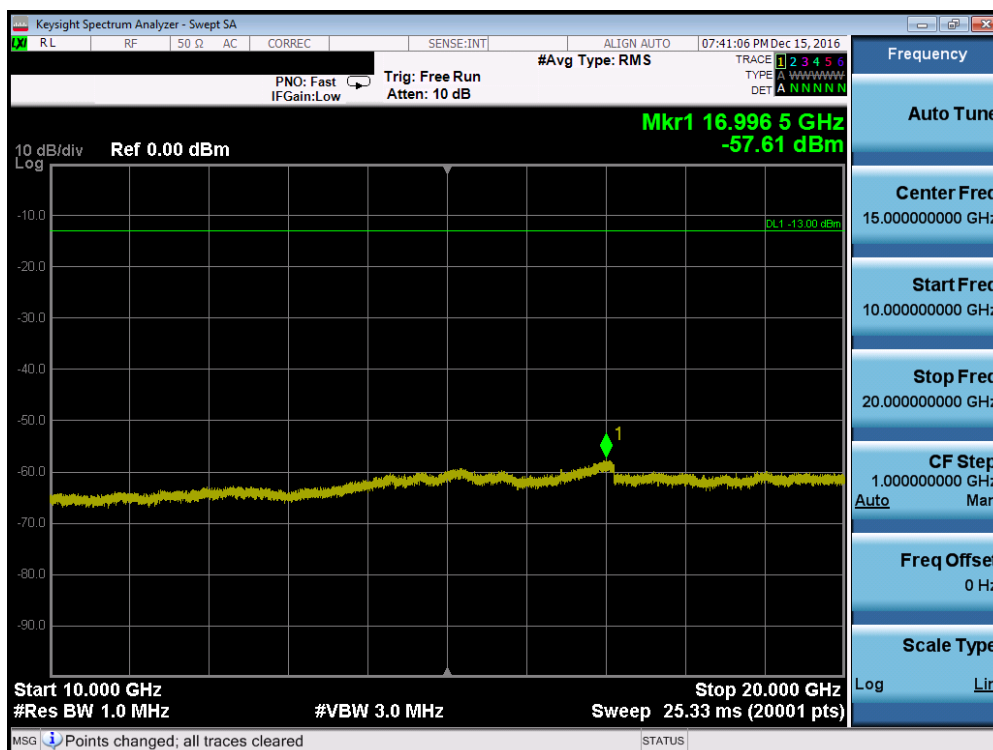
Plot 7-66. Conducted Spurious Plot (Band 2 – 3.0MHz QPSK – RB Size 1, RB Offset 0 – Low Channel)
