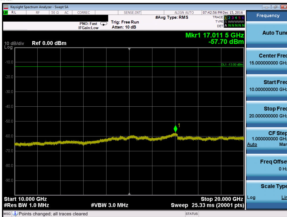
Plot 7-69. Conducted Spurious Plot (Band 2 – 3.0MHz QPSK – RB Size 1, RB Offset 0 – Mid Channel)
