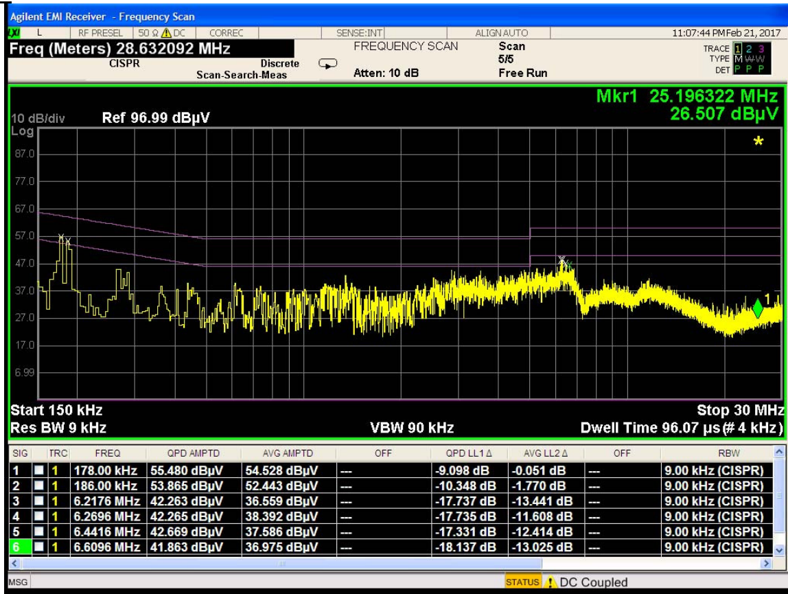
Plot 7-2. Line Conducted Plot (N)
