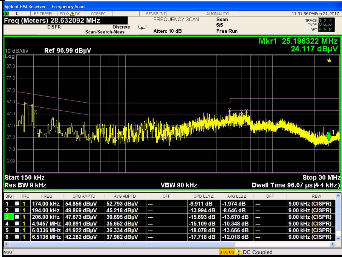
Plot 7-1. Line Conducted Plot (L1)
