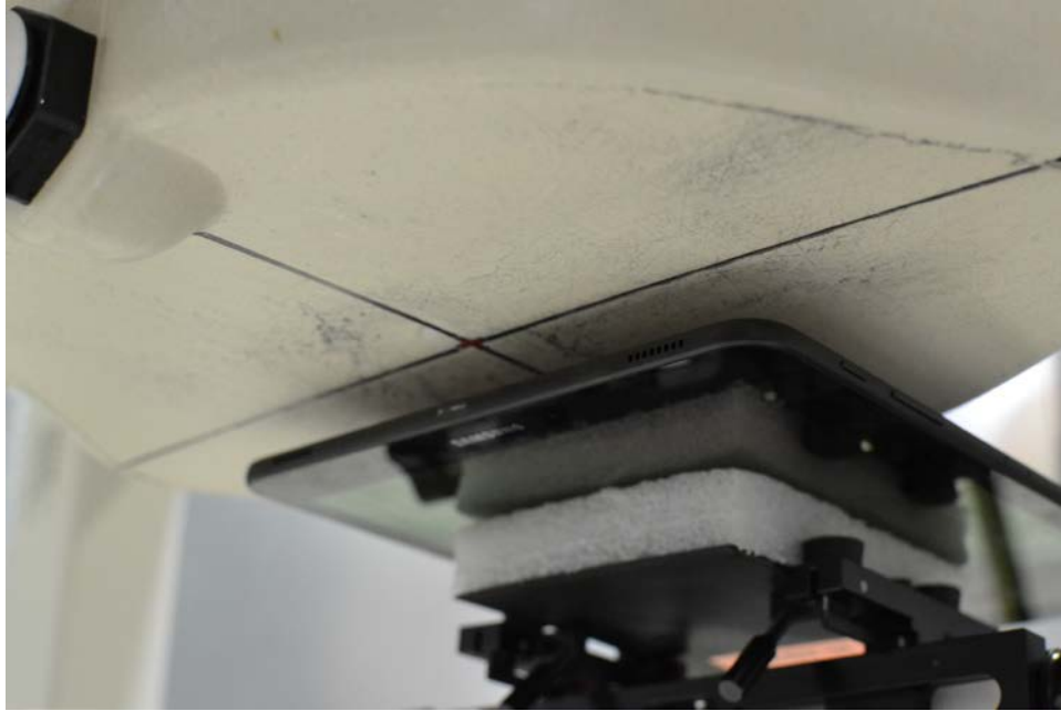
SAR Test Setup Photo 1: Back Side at 1.3 cm
