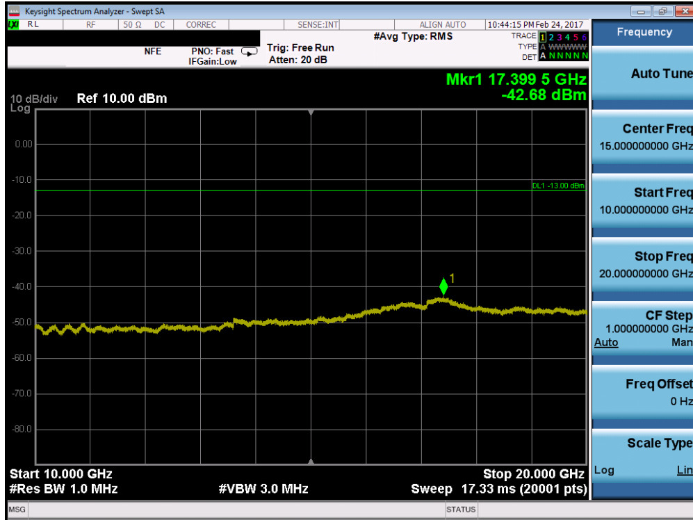
Plot 7-19. Conducted Spurious Plot (PCS CDMA Mode – Ch. 600)
