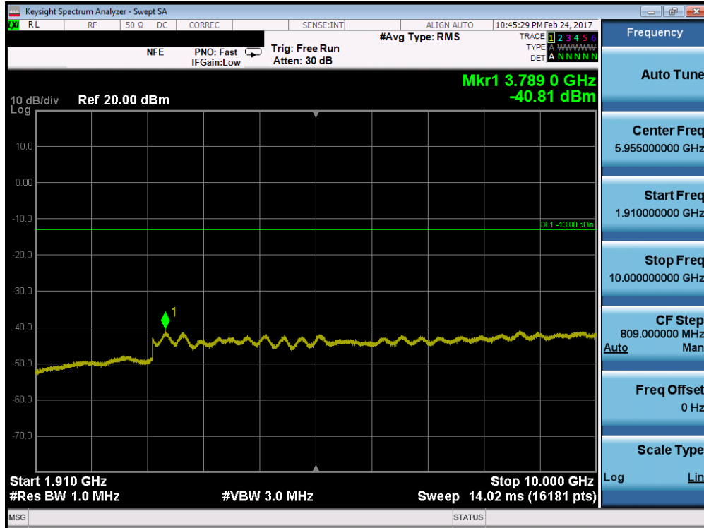
Plot 7-15. Conducted Spurious Plot (PCS CDMA Mode – Ch. 25)
