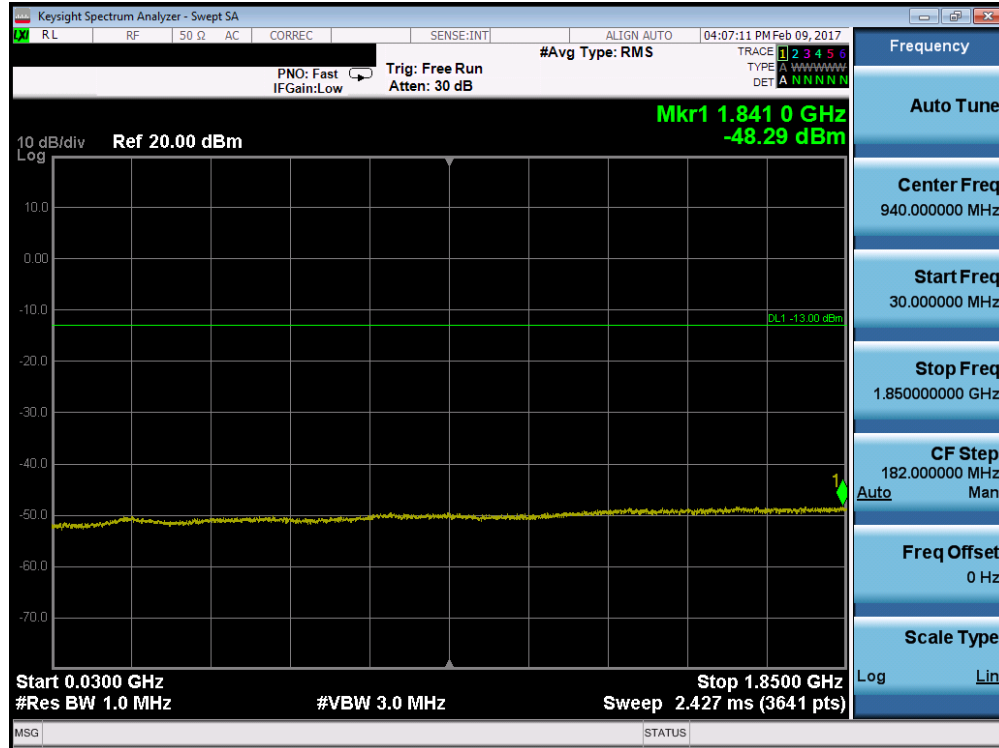
Plot 7-35. Conducted Spurious Plot (PCS WCDMA Mode – Ch. 9400)
