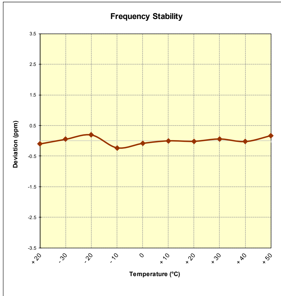
Figure 7-10. Frequency Stability Graph (PCS CDMA Mode – Ch. 600)
