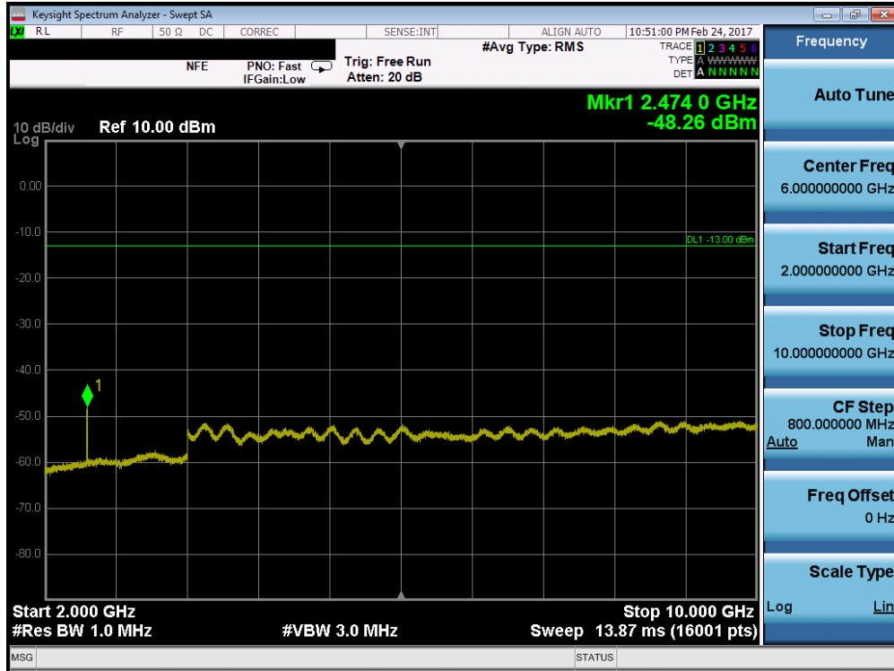
Plot 7-7. Conducted Spurious Plot (Cellular CDMA Mode – Ch. 1013)
