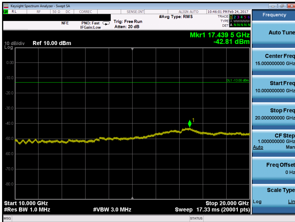
Plot 7-16. Conducted Spurious Plot (PCS CDMA Mode – Ch. 25)
