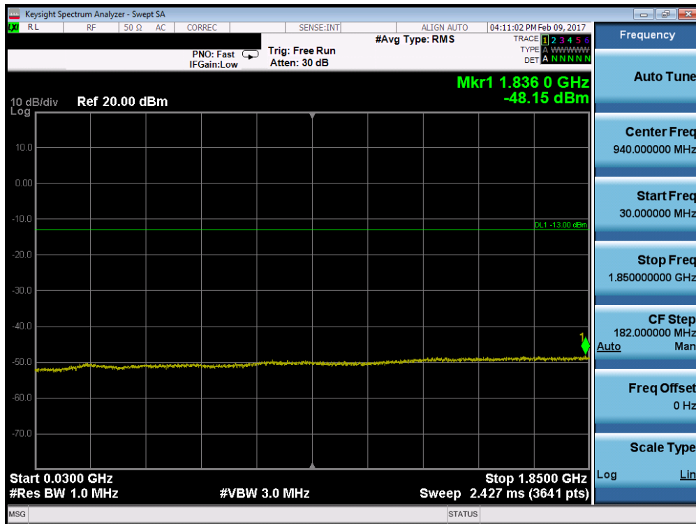
Plot 7-38. Conducted Spurious Plot (PCS WCDMA Mode – Ch. 9538)
