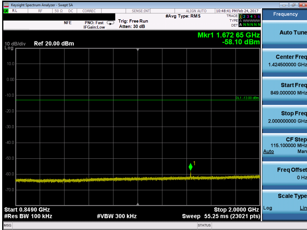
Plot 7-9. Conducted Spurious Plot (Cellular CDMA Mode – Ch. 384)
