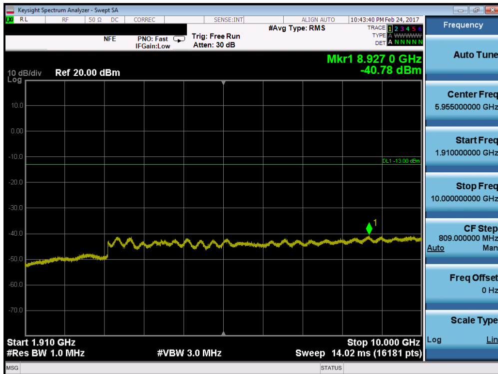
Plot 7-18. Conducted Spurious Plot (PCS CDMA Mode – Ch. 600)
