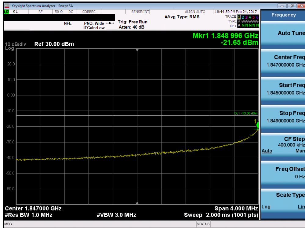
Plot 7-46. 4MHz Span Plot (PCS CDMA Mode – Ch. 25)
