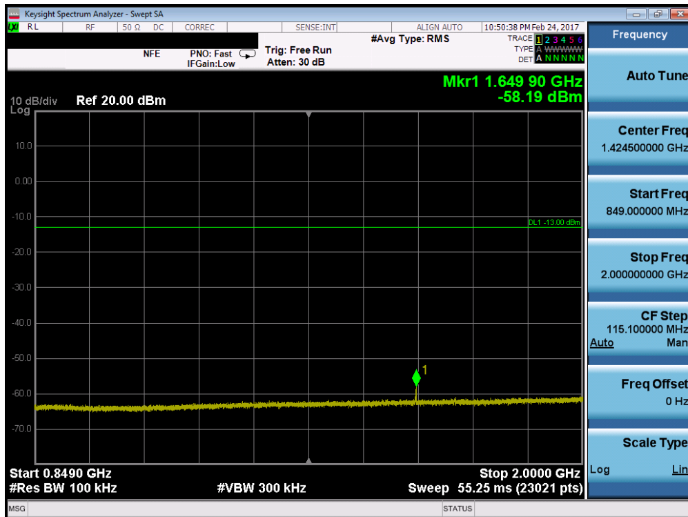
Plot 7-6. Conducted Spurious Plot (Cellular CDMA Mode – Ch. 1013)
