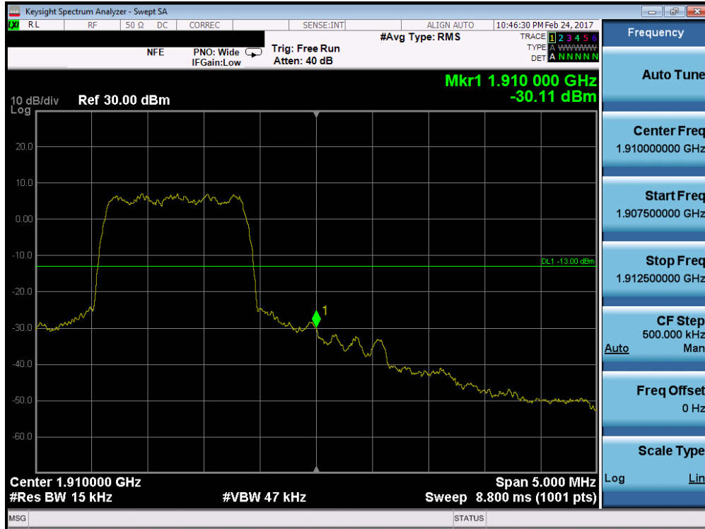
Plot 7-47. Band Edge Plot (PCS CDMA Mode – Ch. 1175)
