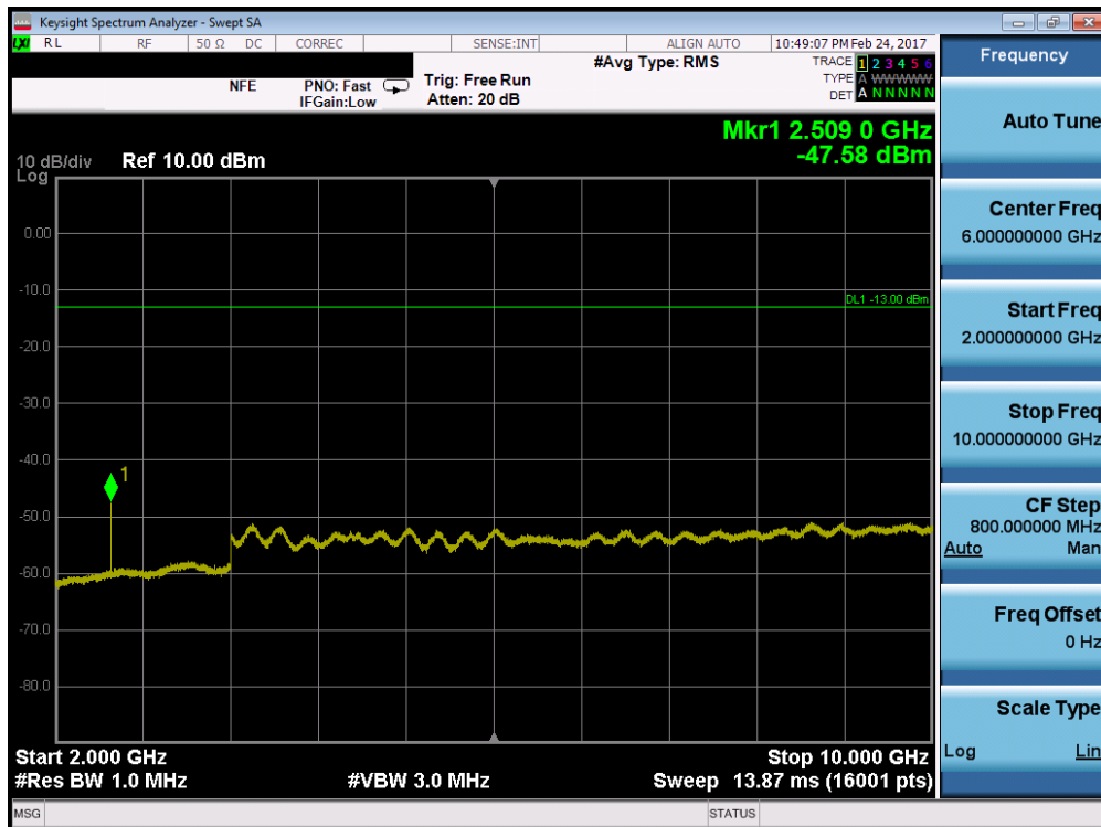
Plot 7-10. Conducted Spurious Plot (Cellular CDMA Mode – Ch. 384)
