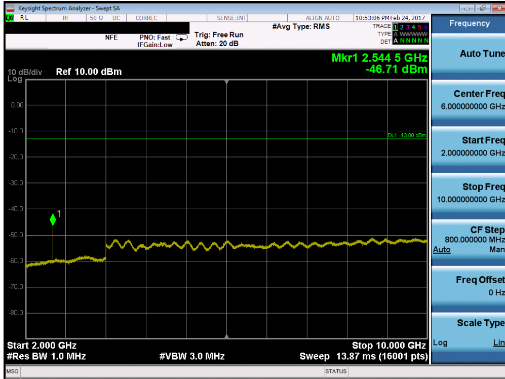
Plot 7-13. Conducted Spurious Plot (Cellular CDMA Mode – Ch. 777)
