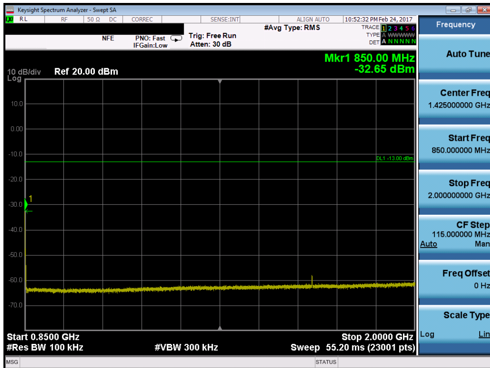
Plot 7-12. Conducted Spurious Plot (Cellular CDMA Mode – Ch. 777)
