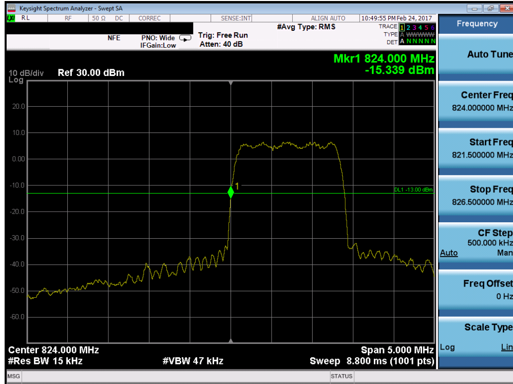
Plot 7-41. Band Edge Plot (Cellular CDMA Mode – Ch. 1013)
