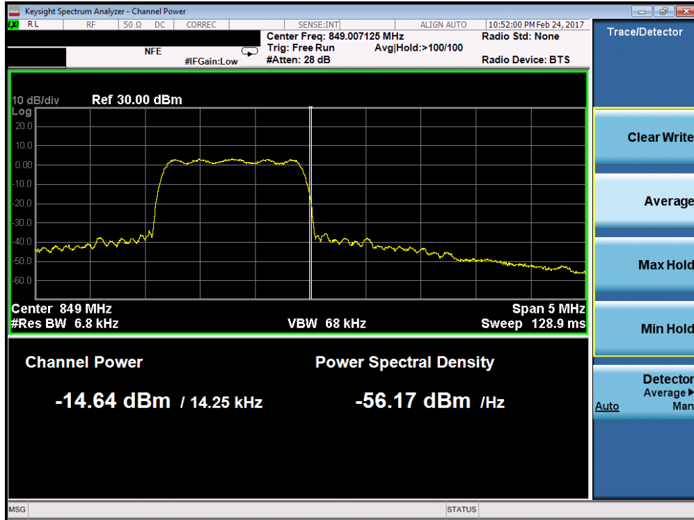
Plot 7-43. Band Edge Plot (Cellular CDMA Mode – Ch. 777)
