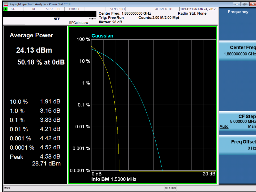
Plot 7-55. Peak-Average Ratio Plot (PCS CDMA Mode – Ch. 600)
