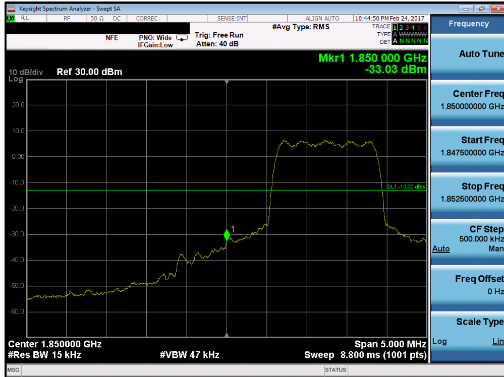
Plot 7-45. Band Edge Plot (PCS CDMA Mode – Ch. 25)
