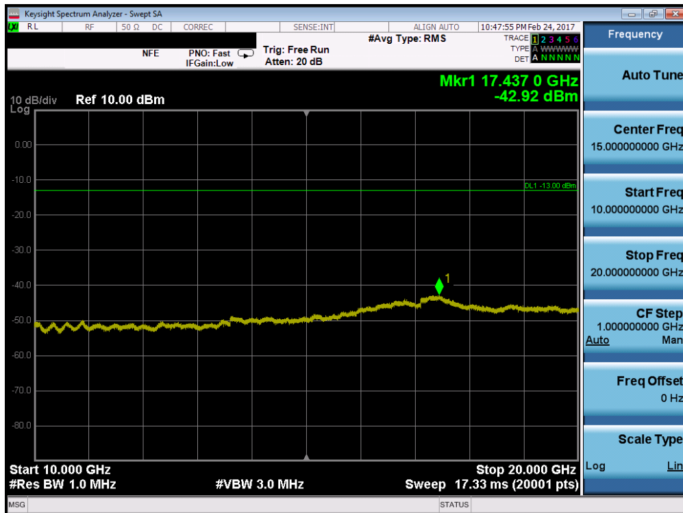
Plot 7-22. Conducted Spurious Plot (PCS CDMA Mode – Ch. 1175)
