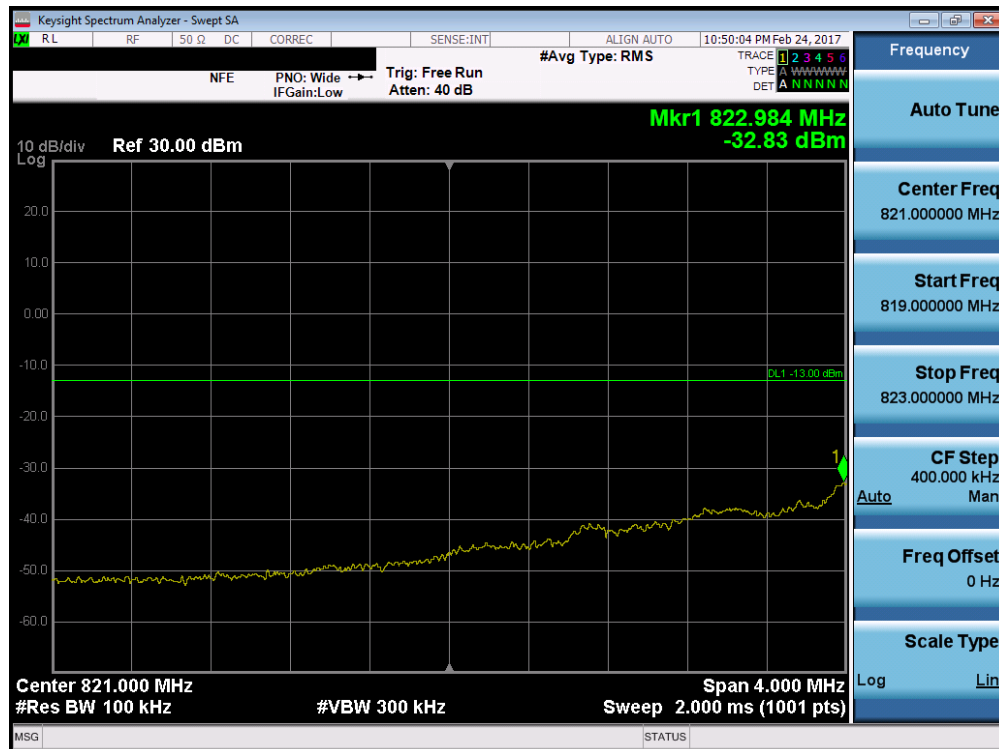
Plot 7-42. 4MHz Span Plot (Cellular CDMA Mode – Ch. 1013)
