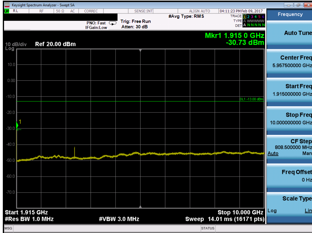
Plot 7-39. Conducted Spurious Plot (PCS WCDMA Mode – Ch. 9538)
