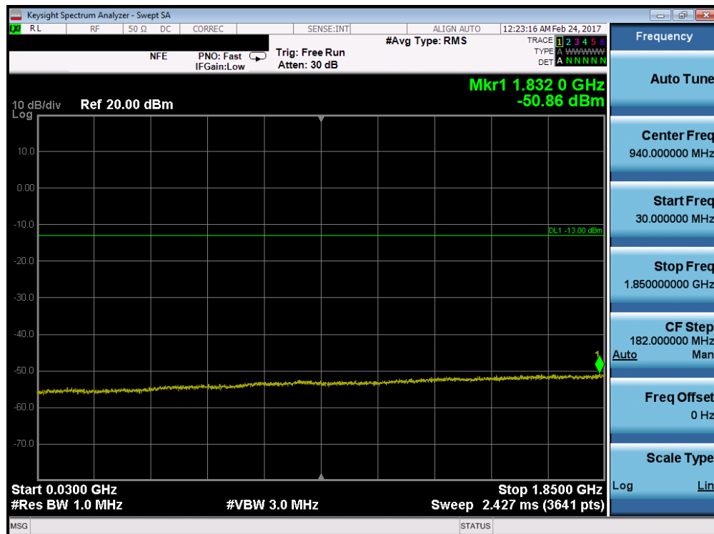
Plot 7-84. Conducted Spurious Plot (Band 25/2 – 3.0MHz QPSK – RB Size 1, RB Offset 0 – Mid Channel)
