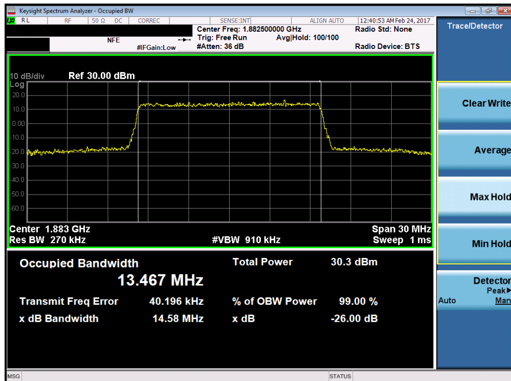
Plot 7-42. Occupied Bandwidth Plot (Band 25/2 – 15.0MHz 16-QAM – RB Size 75)
