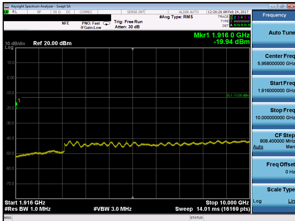
Plot 7-88. Conducted Spurious Plot (Band 25/2 – 3.0MHz QPSK – RB Size 1, RB Offset 0 – High Channel)
