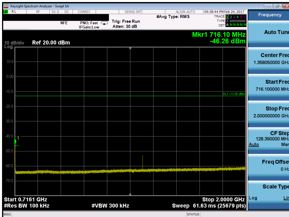
Plot 7-52. Conducted Spurious Plot (Band 12 – 3.0MHz QPSK – RB Size 1, RB Offset 0 – High Channel)
