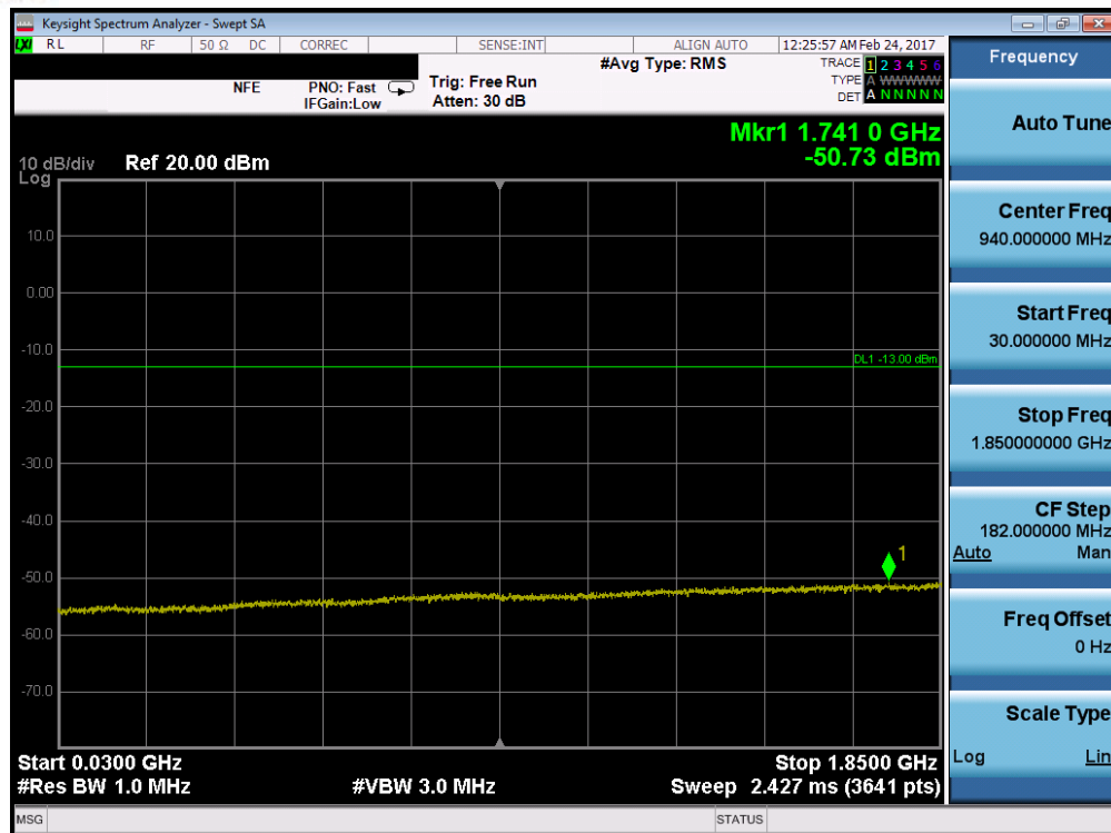
Plot 7-87. Conducted Spurious Plot (Band 25/2 – 3.0MHz QPSK – RB Size 1, RB Offset 0 – High Channel)
