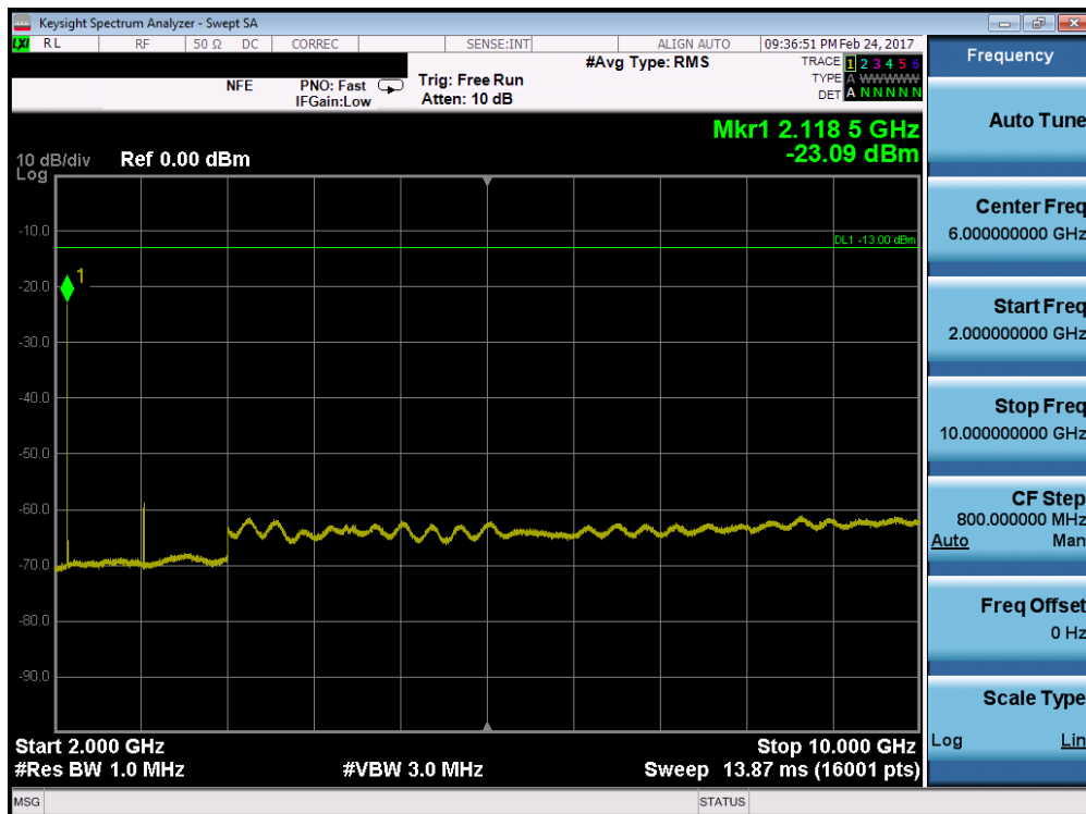
Plot 7-50. Conducted Spurious Plot (Band 12 – 3.0MHz QPSK – RB Size 1, RB Offset 0 – Mid Channel)
