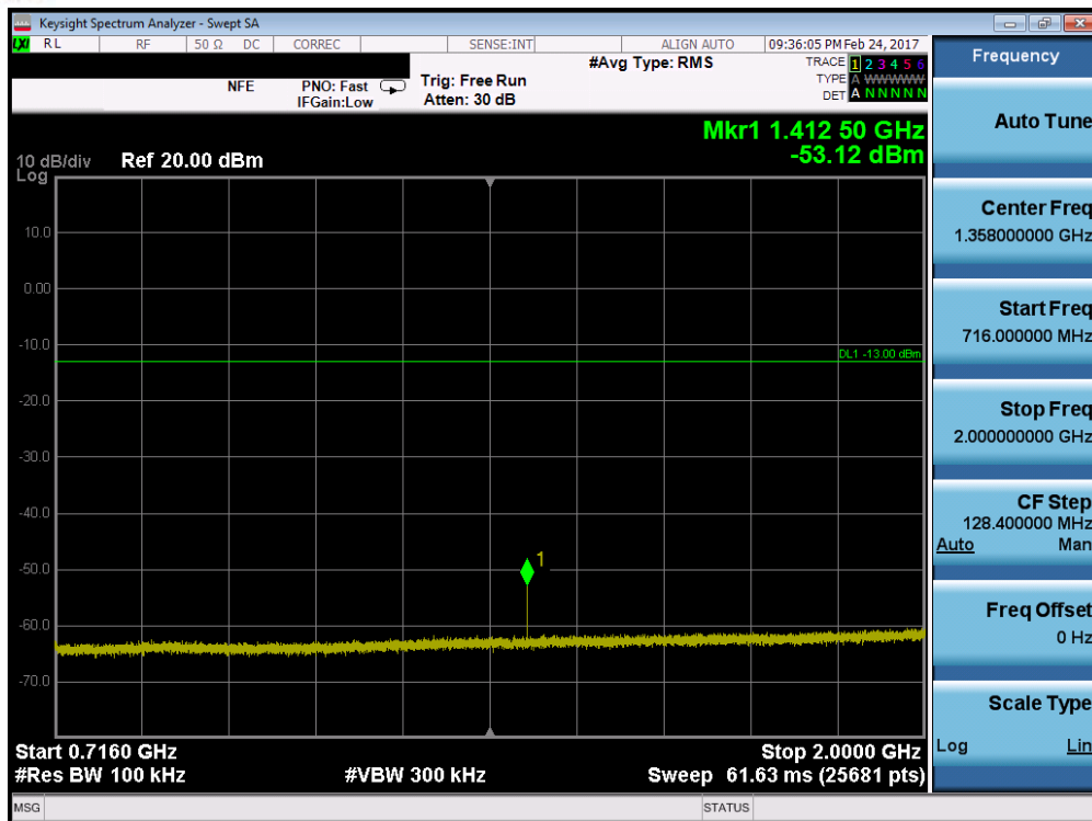
Plot 7-49. Conducted Spurious Plot (Band 12 – 3.0MHz QPSK – RB Size 1, RB Offset 0 – Mid Channel)
