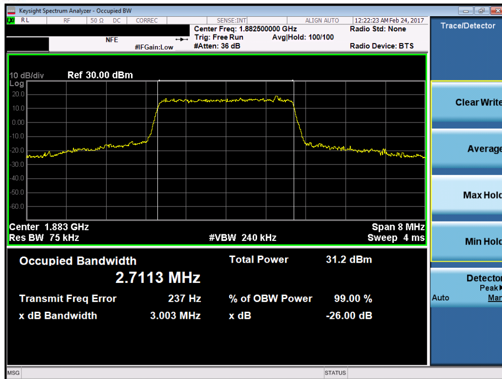
Plot 7-35. Occupied Bandwidth Plot (Band 25/2 - 3.0MHz QPSK - RB Size 15)
