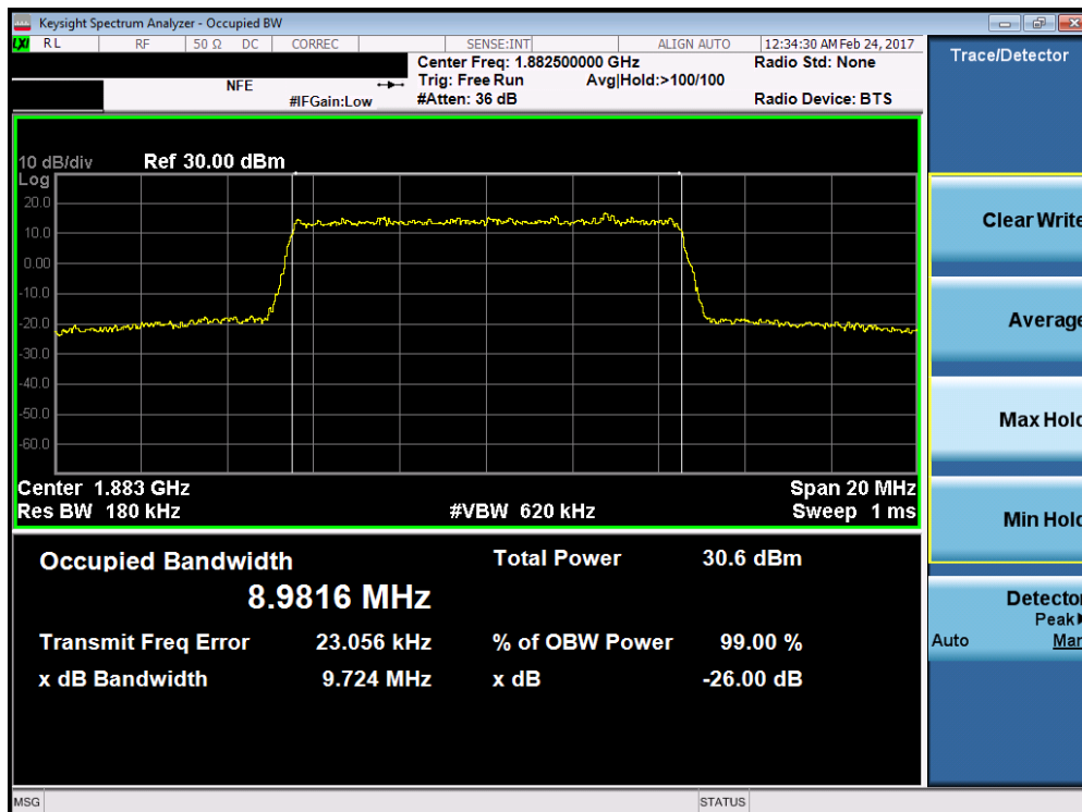
Plot 7-40. Occupied Bandwidth Plot (Band 25/2 – 10.0MHz 16-QAM – RB Size 50)
