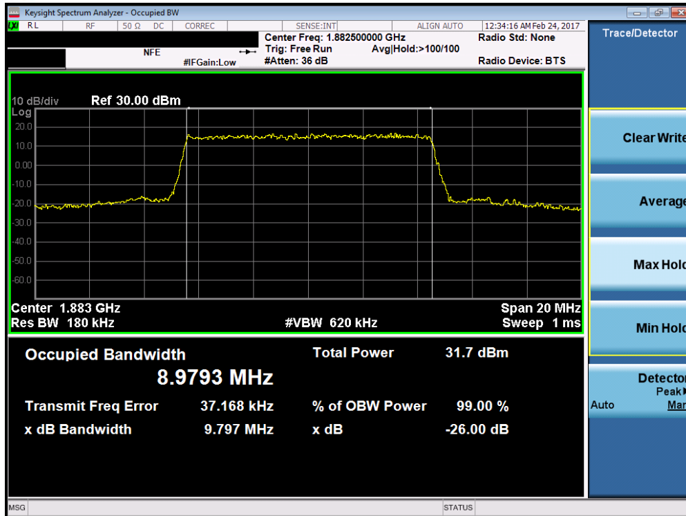
Plot 7-39. Occupied Bandwidth Plot (Band 25/2 – 10.0MHz QPSK – RB Size 50)
