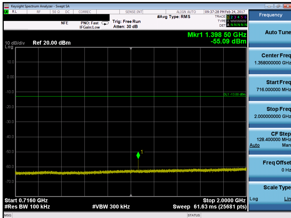
Plot 7-46. Conducted Spurious Plot (Band 12 – 3.0MHz QPSK – RB Size 1, RB Offset 0 – Low Channel)
