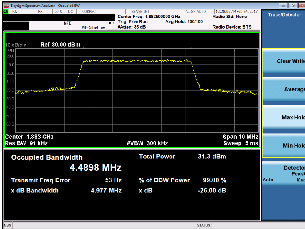
Plot 7-37. Occupied Bandwidth Plot (Band 25/2 – 5.0MHz QPSK – RB Size 25)
