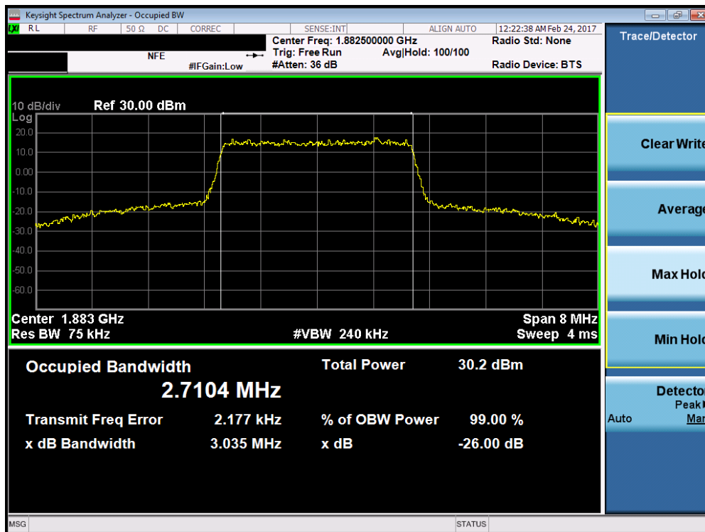
Plot 7-36. Occupied Bandwidth Plot (Band 25/2 - 3.0MHz 16-QAM - RB Size 15)
