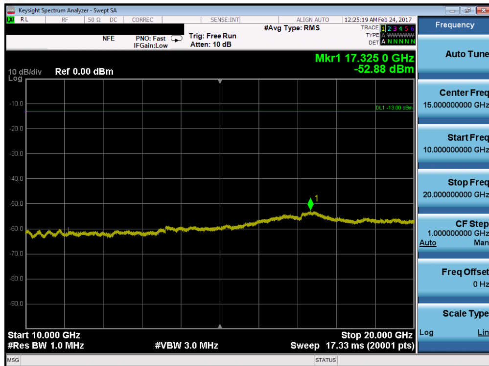
Plot 7-83. Conducted Spurious Plot (Band 25/2 – 3.0MHz QPSK – RB Size 1, RB Offset 0 – Low Channel)
