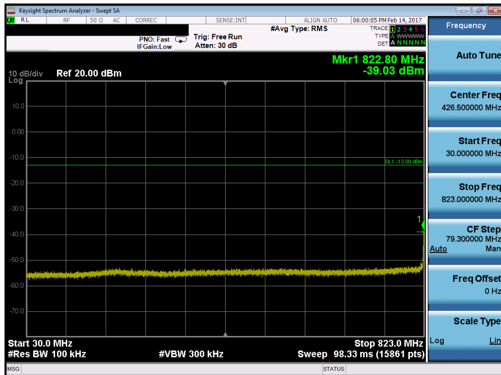
Plot 7-63. Conducted Spurious Plot (Band 5 – 5.0MHz QPSK – RB Size 1, RB Offset 0 – Low Channel)
