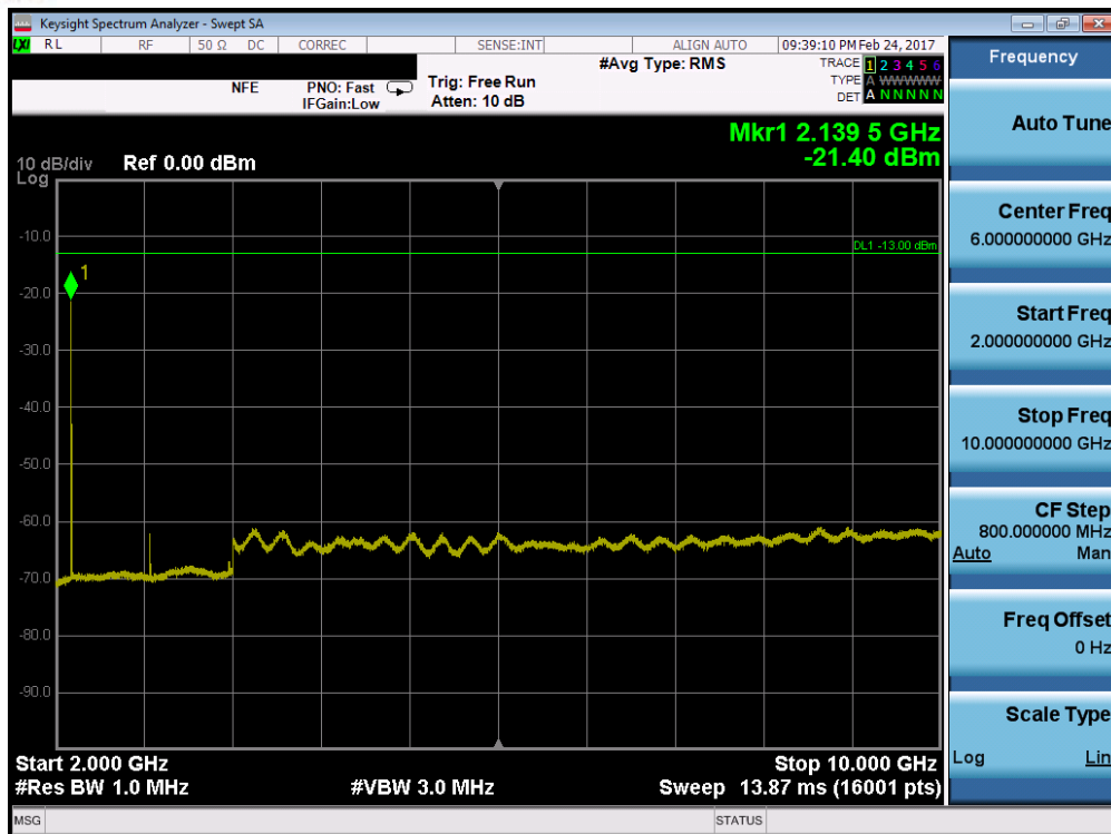
Plot 7-53. Conducted Spurious Plot (Band 12 – 3.0MHz QPSK – RB Size 1, RB Offset 0 – High Channel)
