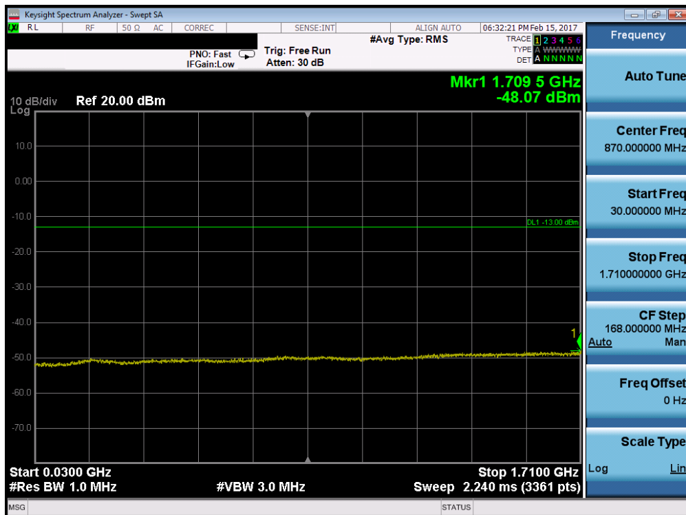
Plot 7-78. Conducted Spurious Plot (Band 4 – 15.0MHz QPSK – RB Size 1, RB Offset 0 – High Channel)
