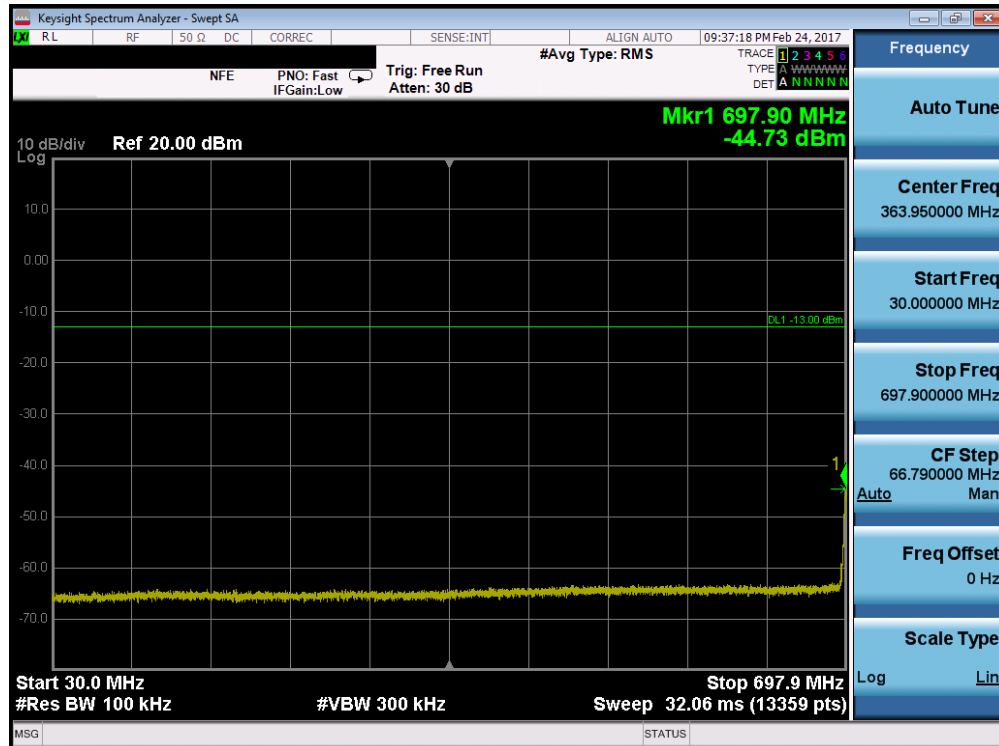
Plot 7-45. Conducted Spurious Plot (Band 12 – 3.0MHz QPSK – RB Size 1, RB Offset 0 – Low Channel)
