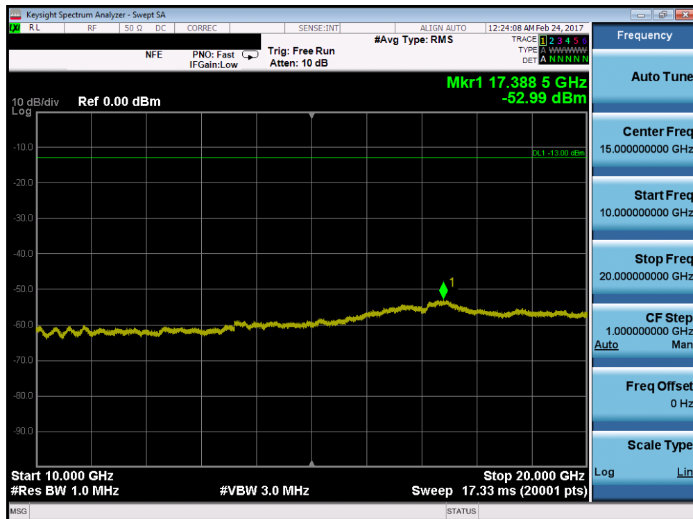
Plot 7-86. Conducted Spurious Plot (Band 25/2 – 3.0MHz QPSK – RB Size 1, RB Offset 0 – Mid Channel)
