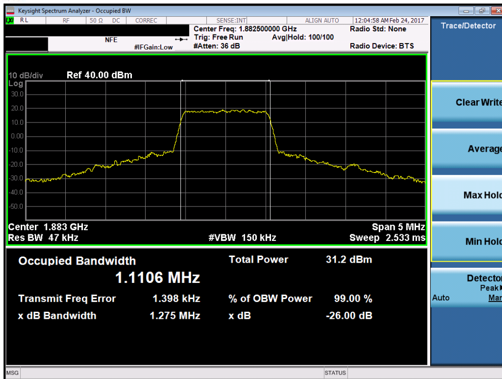
Plot 7-33. Occupied Bandwidth Plot (Band 25/2 – 1.4MHz QPSK – RB Size 6)
