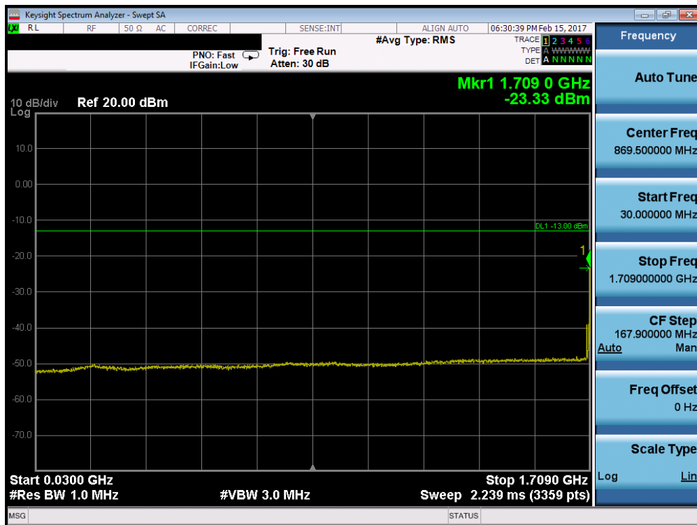
Plot 7-72. Conducted Spurious Plot (Band 4 – 15.0MHz QPSK – RB Size 1, RB Offset 0 – Low Channel)
