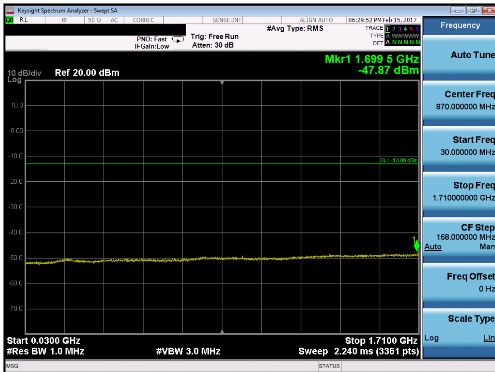
Plot 7-75. Conducted Spurious Plot (Band 4 – 15.0MHz QPSK – RB Size 1, RB Offset 0 – Mid Channel)
