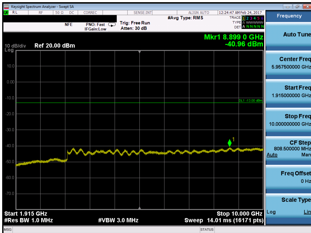
Plot 7-82. Conducted Spurious Plot (Band 25/2 – 3.0MHz QPSK – RB Size 1, RB Offset 0 – Low Channel)
