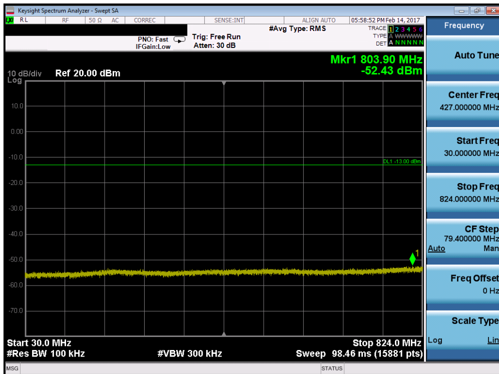
Plot 7-66. Conducted Spurious Plot (Band 5 – 5.0MHz QPSK – RB Size 1, RB Offset 0 – Mid Channel)
