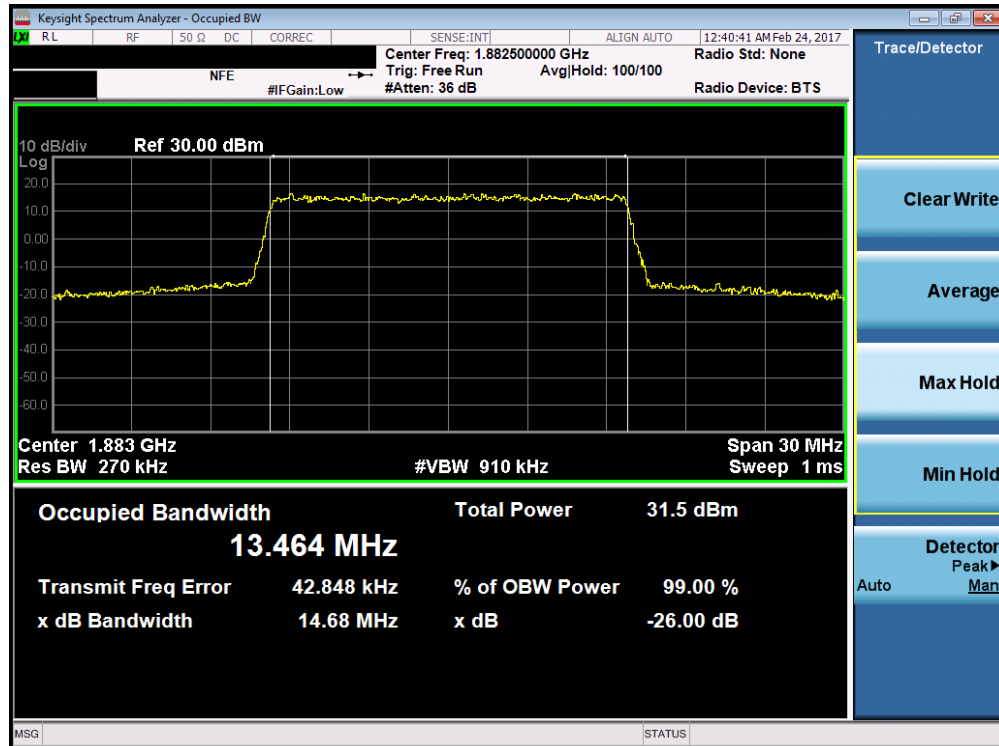
Plot 7-41. Occupied Bandwidth Plot (Band 25/2 – 15.0MHz QPSK – RB Size 75)
