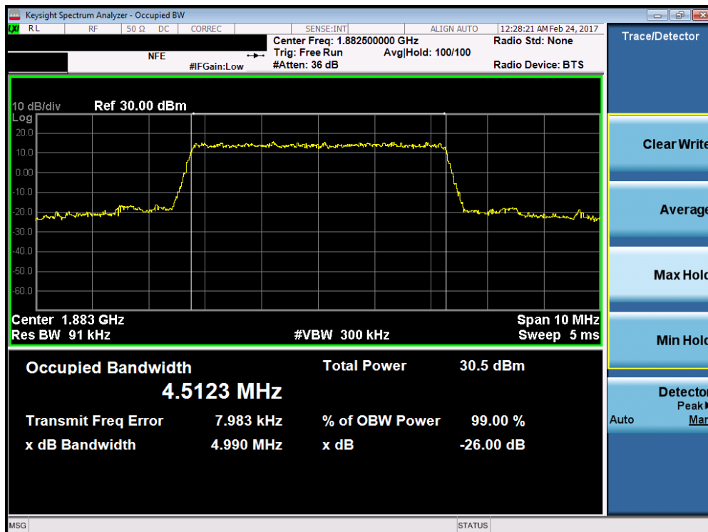
Plot 7-38. Occupied Bandwidth Plot (Band 25/2 – 5.0MHz 16-QAM – RB Size 25)
