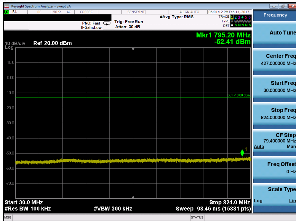
Plot 7-69. Conducted Spurious Plot (Band 5 – 5.0MHz QPSK – RB Size 1, RB Offset 0 – High Channel)
