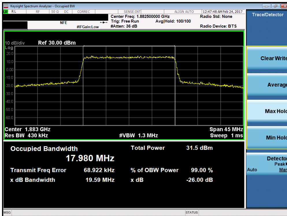
Plot 7-43. Occupied Bandwidth Plot (Band 25/2 – 20.0MHz QPSK – RB Size 100)
