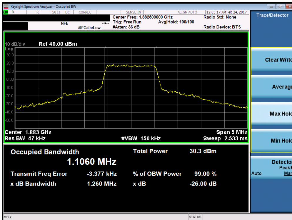
Plot 7-34. Occupied Bandwidth Plot (Band 25/2 – 1.4MHz 16-QAM – RB Size 6)
