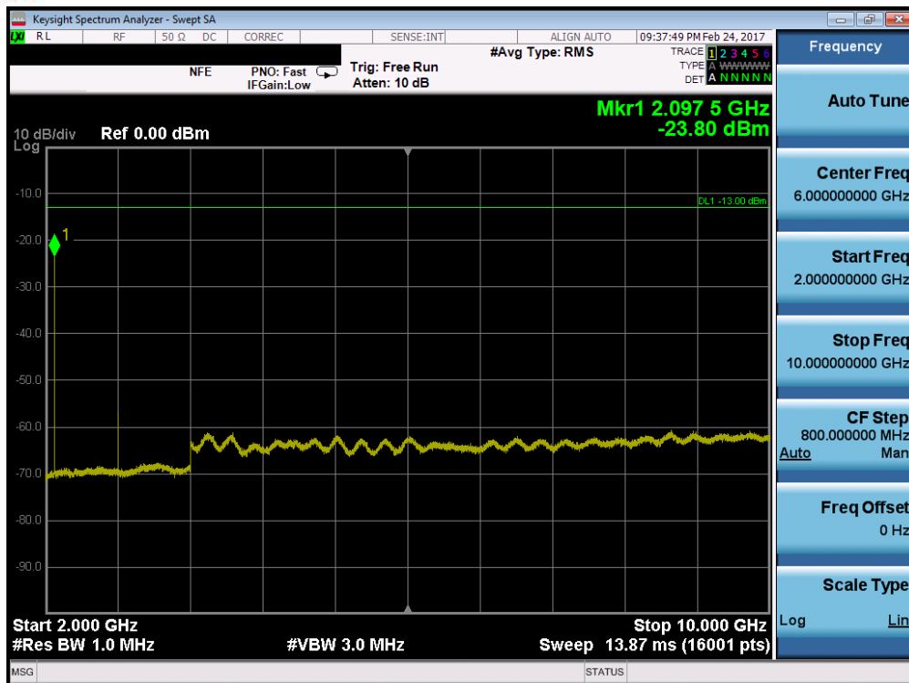
Plot 7-47. Conducted Spurious Plot (Band 12 – 3.0MHz QPSK – RB Size 1, RB Offset 0 – Low Channel)
