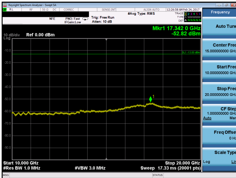
Plot 7-89. Conducted Spurious Plot (Band 25/2 – 3.0MHz QPSK – RB Size 1, RB Offset 0 – High Channel)
