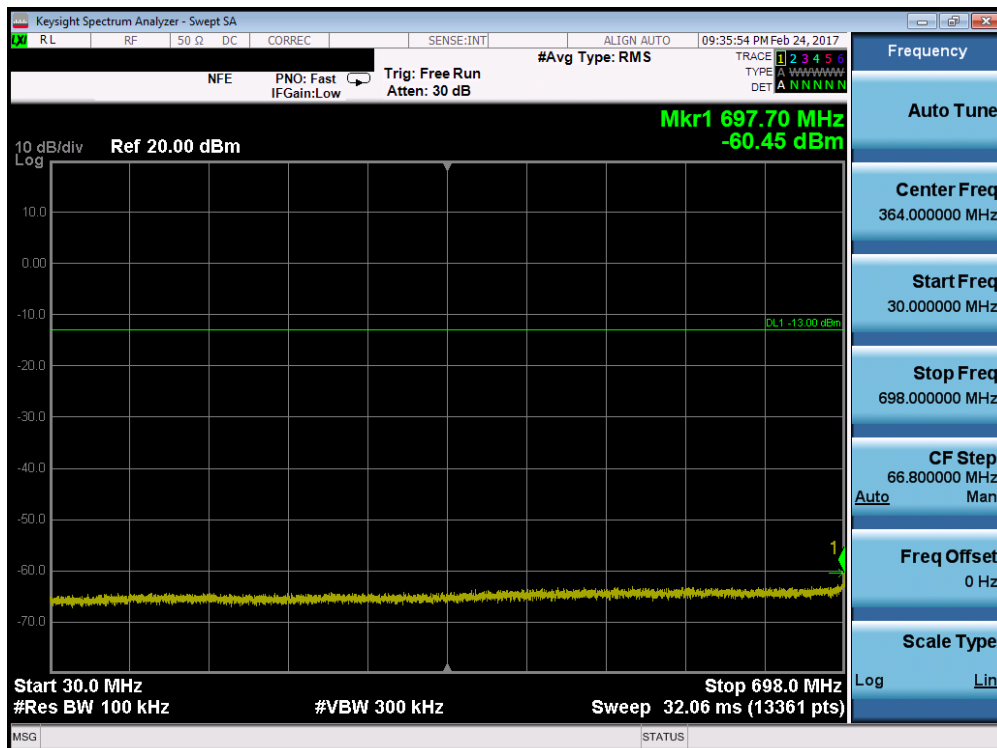
Plot 7-48. Conducted Spurious Plot (Band 12 – 3.0MHz QPSK – RB Size 1, RB Offset 0 – Mid Channel)
