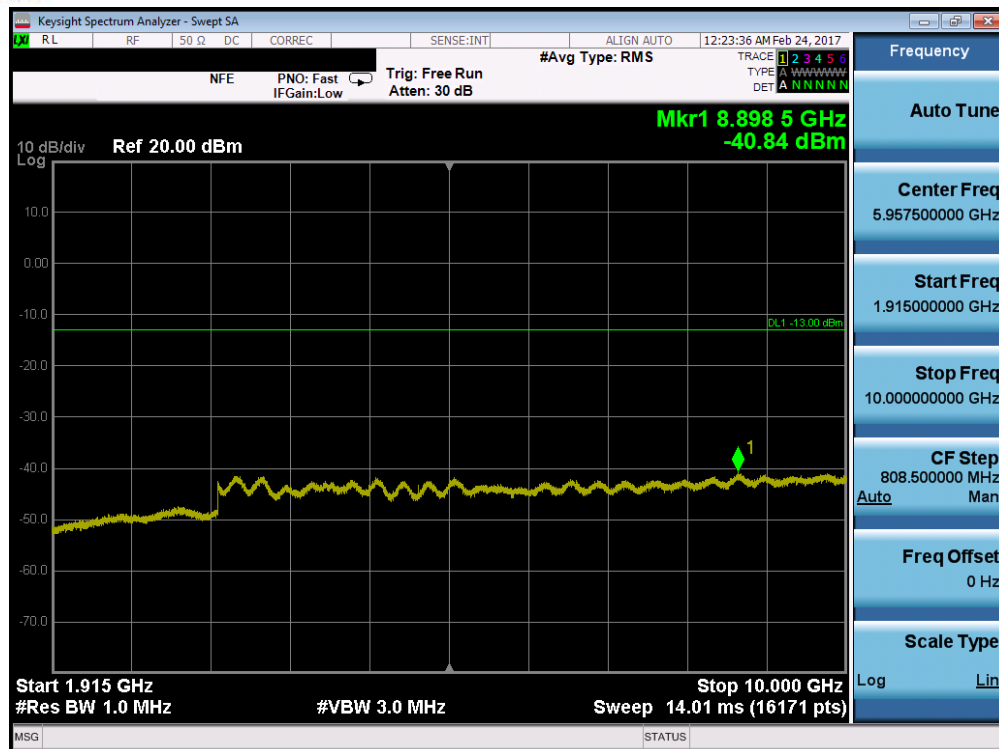
Plot 7-85. Conducted Spurious Plot (Band 25/2 – 3.0MHz QPSK – RB Size 1, RB Offset 0 – Mid Channel)
