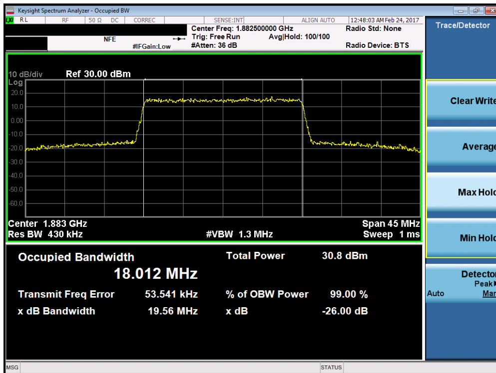
Plot 7-44. Occupied Bandwidth Plot (Band 25/2 – 20.0MHz 16-QAM – RB Size 100)
