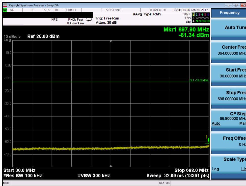
Plot 7-51. Conducted Spurious Plot (Band 12 – 3.0MHz QPSK – RB Size 1, RB Offset 0 – High Channel)
