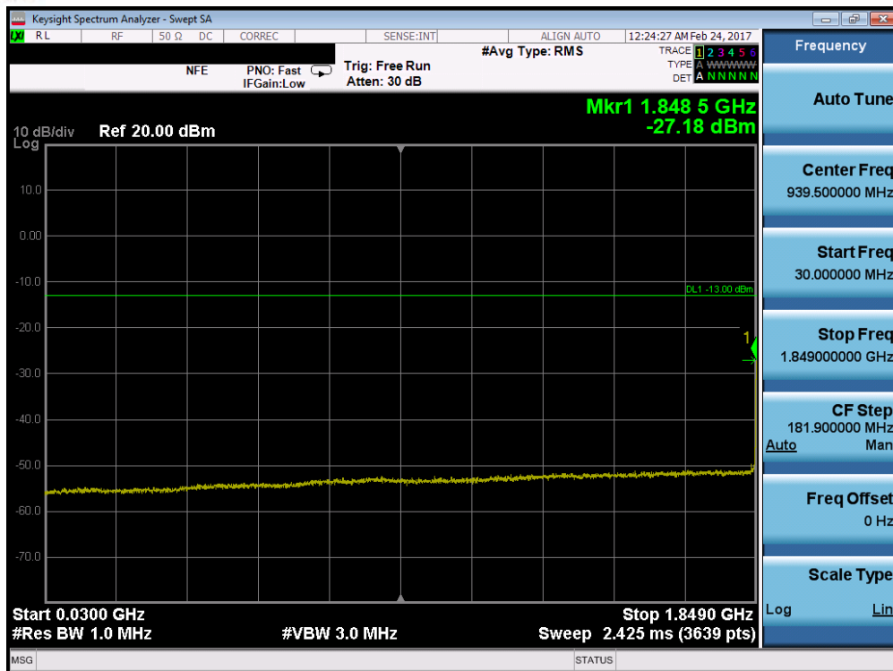
Plot 7-81. Conducted Spurious Plot (Band 25/2 – 3.0MHz QPSK – RB Size 1, RB Offset 0 – Low Channel)
