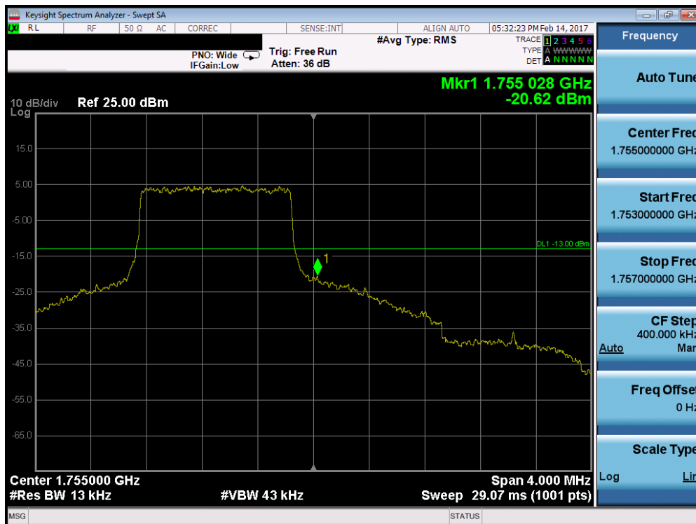
Plot 7-116. Upper Band Edge Plot (Band 4 – 1.4MHz QPSK – RB Size 6)
