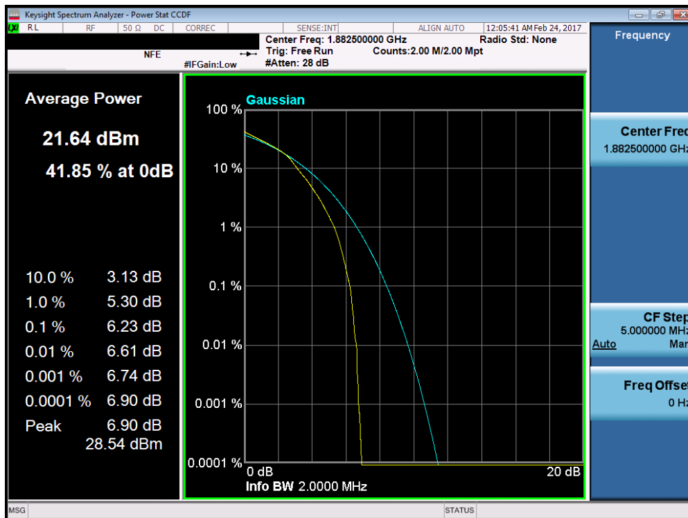
Plot 7-163. PAR Plot (Band 25/2 – 1.4MHz 16-QAM – RB Size 6)
