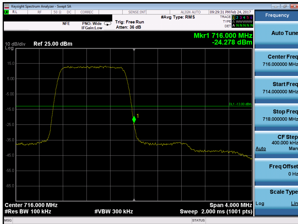
Plot 7-91. Upper Band Edge Plot (Band 12 – 1.4MHz QPSK – RB Size 6)
