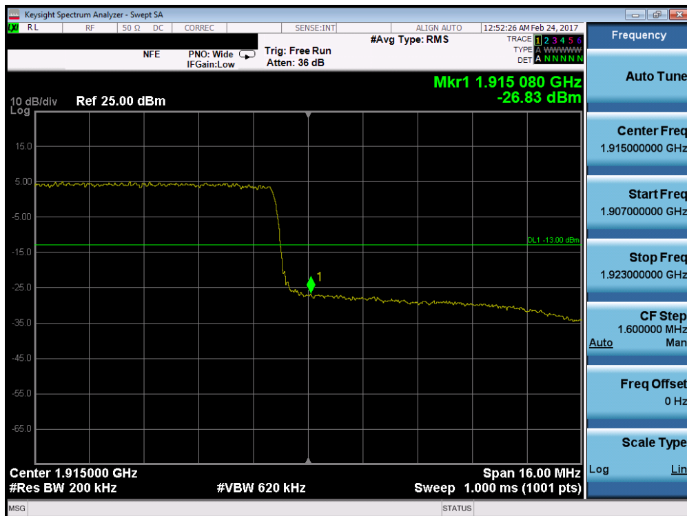
Plot 7-160. Upper Band Edge Plot (Band 25/2 - 20.0MHz QPSK - RB Size 100)
