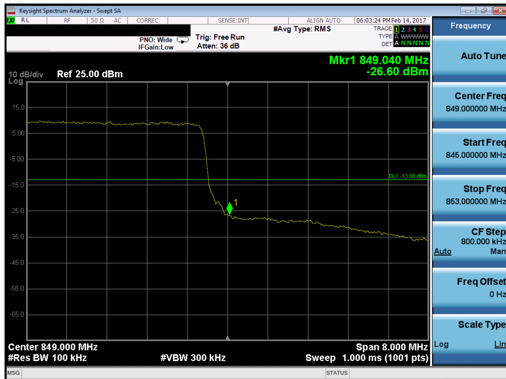
Plot 7-113. Upper Band Edge Plot (Band 5 – 10.0MHz QPSK – RB Size 50)
