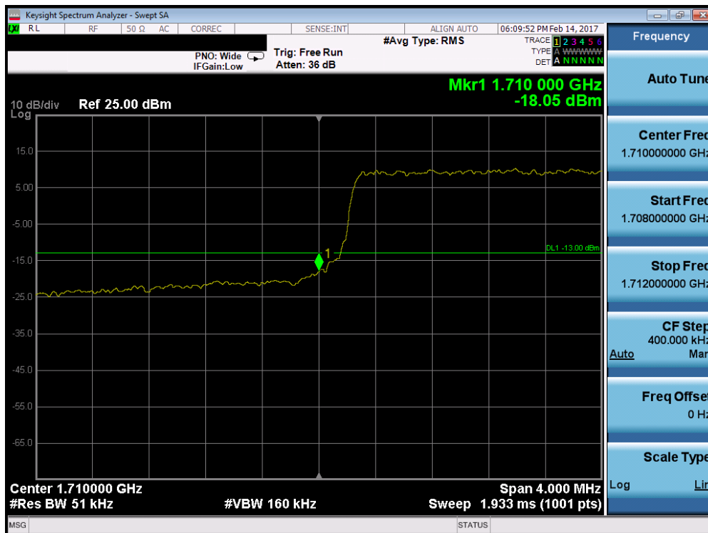
Plot 7-122. Lower Band Edge Plot (Band 4 – 5.0MHz QPSK – RB Size 25)
