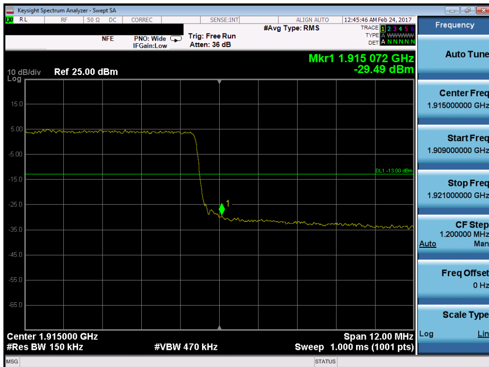
Plot 7-156. Upper Band Edge Plot (Band 25/2 – 15.0MHz QPSK – RB Size 75)
