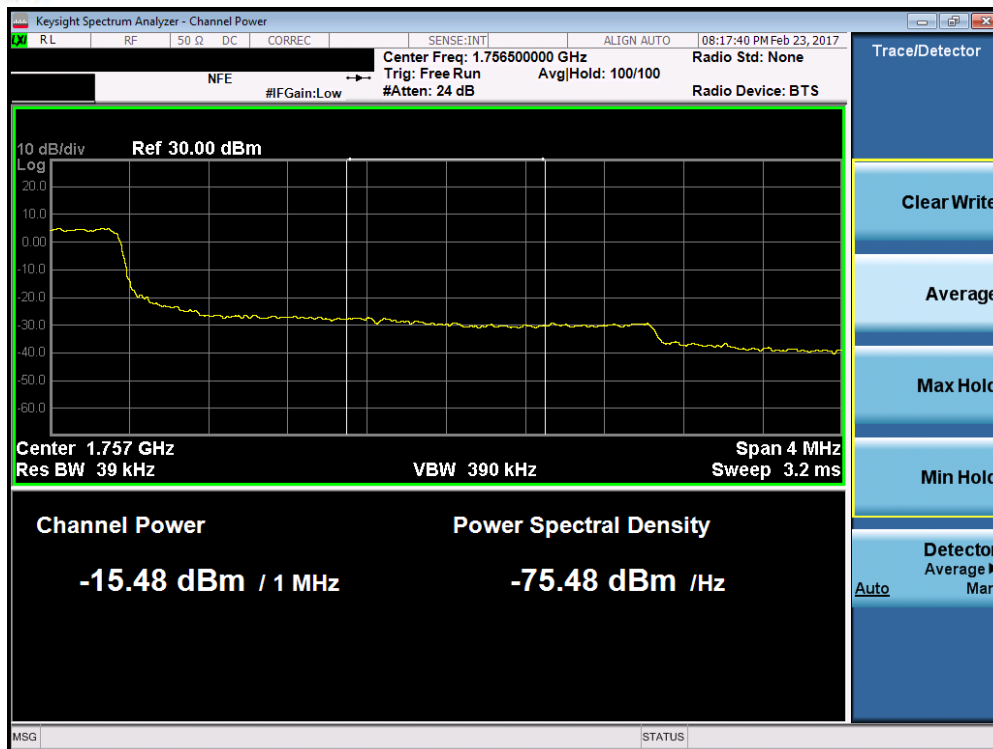
Plot 7-121. Upper Extended Band Edge Plot (Band 4 – 3.0MHz QPSK – RB Size 15)
