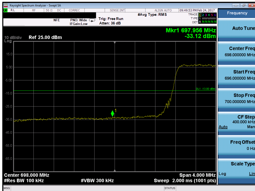
Plot 7-94. Lower Band Edge Plot (Band 12/17 – 5.0MHz QPSK – RB Size 25)
