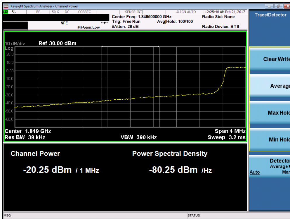
Plot 7-143. Lower Extended Band Edge Plot (Band 25/2 – 3.0MHz QPSK – RB Size 15)
