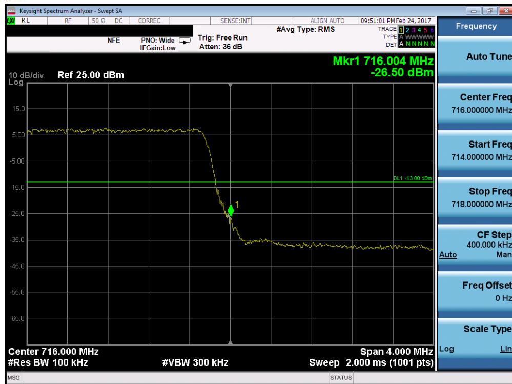
Plot 7-95. Upper Band Edge Plot (Band 12/17 – 5.0MHz QPSK – RB Size 25)
