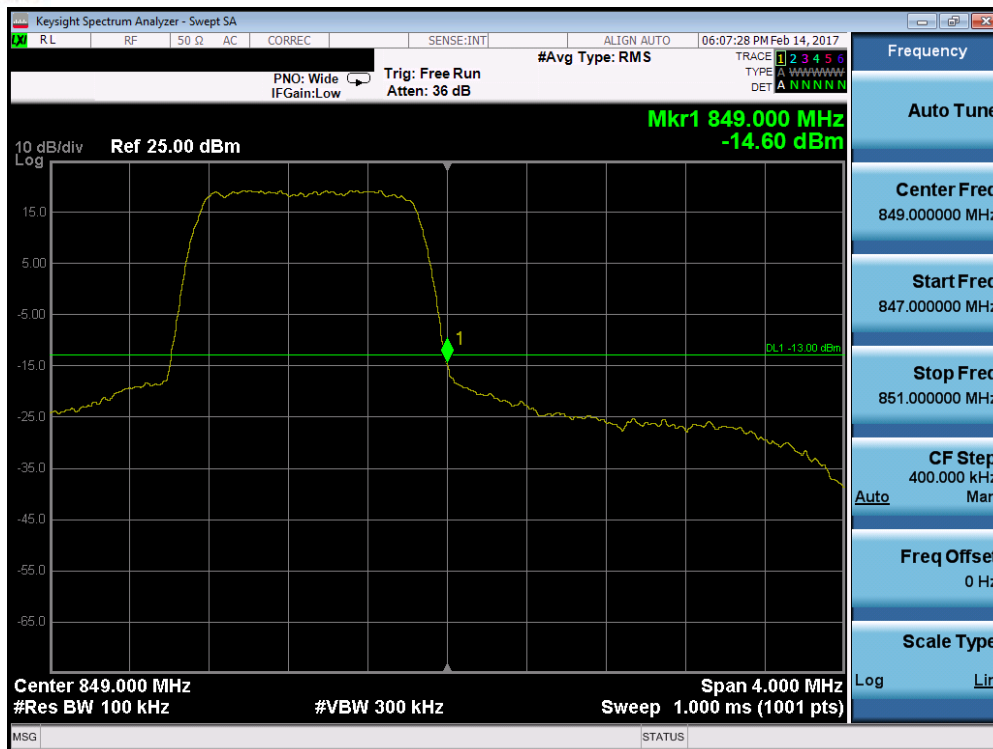
Plot 7-107. Upper Band Edge Plot (Band 5 – 1.4MHz QPSK – RB Size 6)
