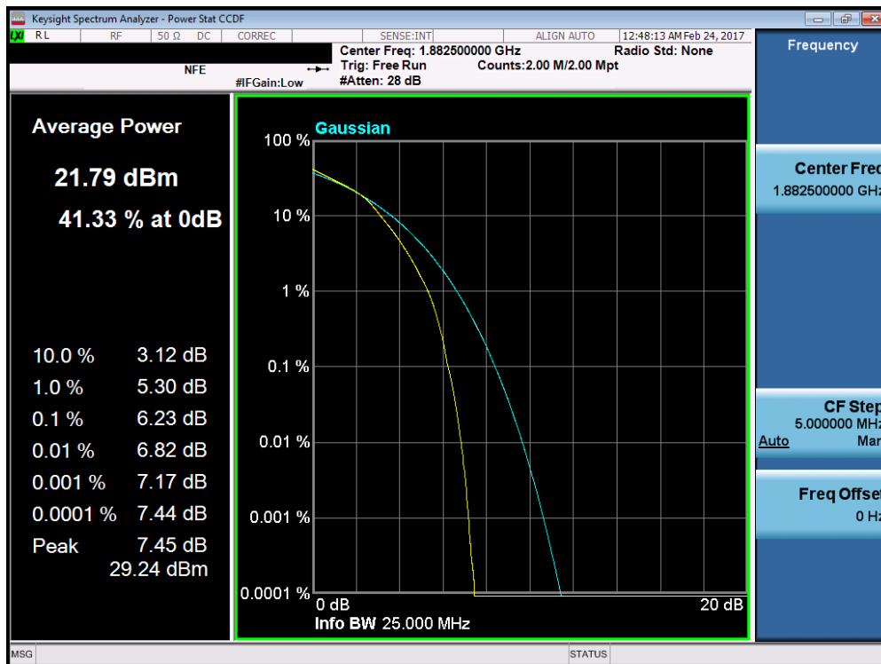
Plot 7-173. PAR Plot (Band 25/2 – 20.0MHz 16-QAM – RB Size 100)
