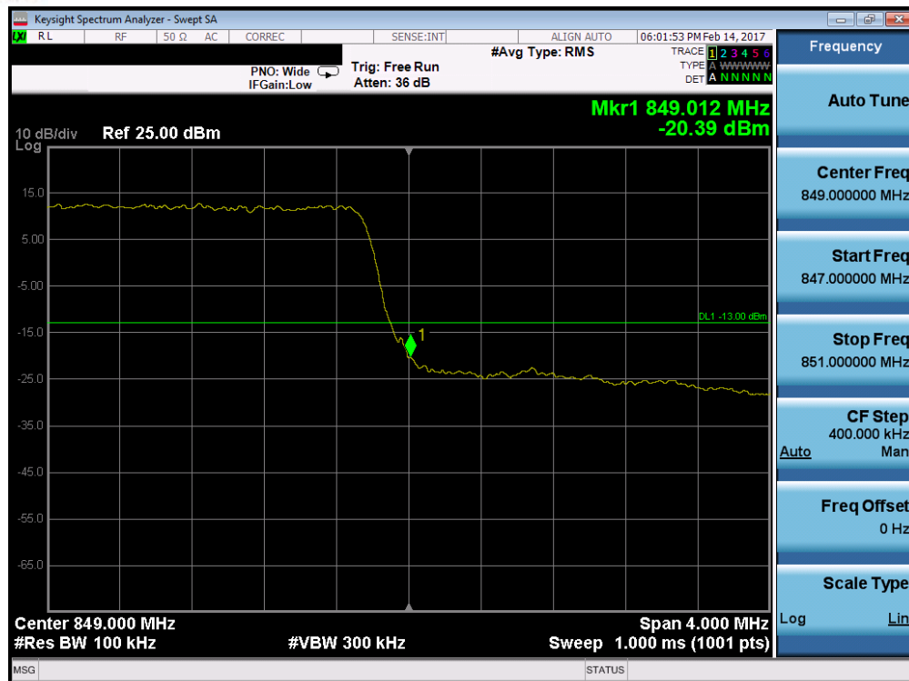
Plot 7-111. Upper Band Edge Plot (Band 5 – 5.0MHz QPSK – RB Size 25)
