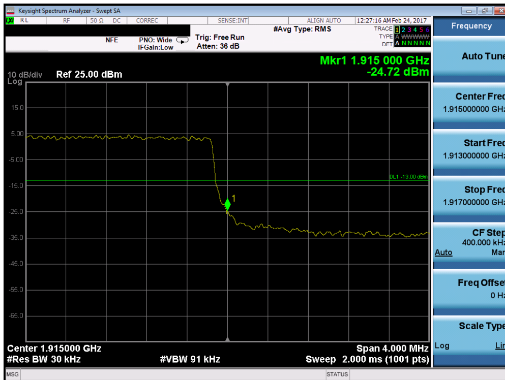
Plot 7-144. Upper Band Edge Plot (Band 25/2 – 3.0MHz QPSK – RB Size 15)
