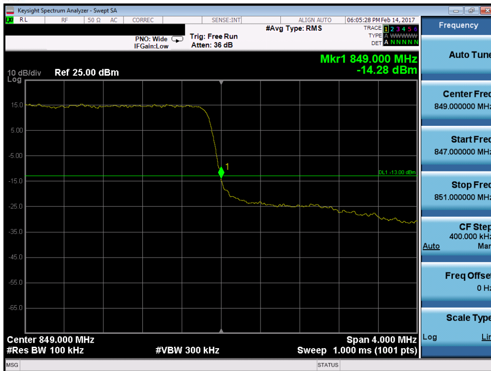
Plot 7-109. Upper Band Edge Plot (Band 5 – 3.0MHz QPSK – RB Size 15)
