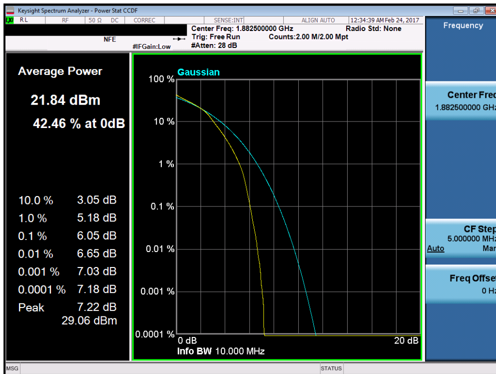
Plot 7-169. PAR Plot (Band 25/2 – 10.0MHz 16-QAM – RB Size 50)
