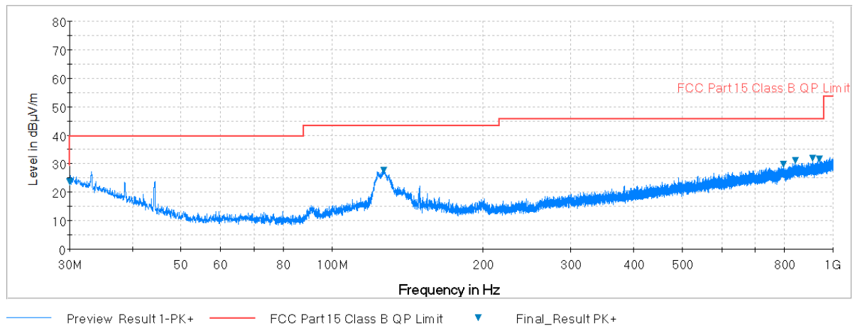
Plot 7-53. Radiated Spurious Plot below 1GHz (Pol. V)
