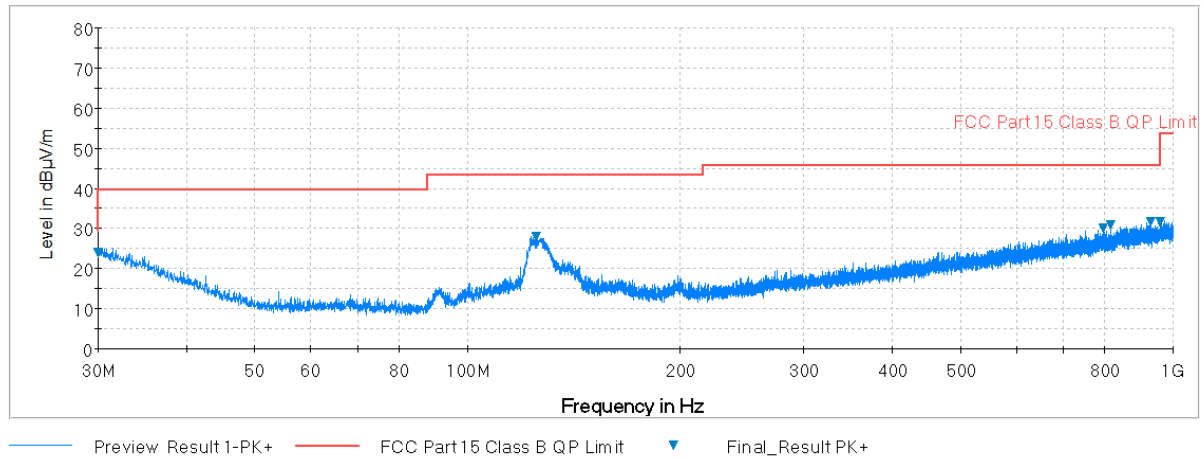
Plot 7-52. Radiated Spurious Plot below 1GHz (Pol. H)
