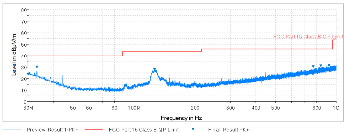
Plot 7-247. Radiated Spurious Plot below 1GHz (802.11a – U3 Ch. 157, Ant. Pol. V)
