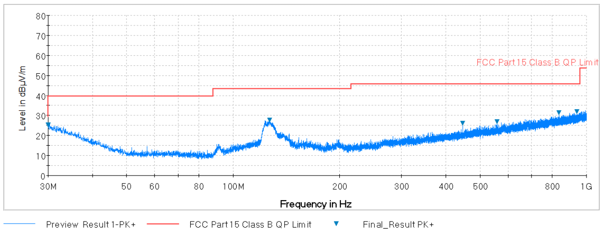
Plot 7-244. Radiated Spurious Plot below 1GHz (802.11a – U3 Ch. 157, Ant. Pol. H)
