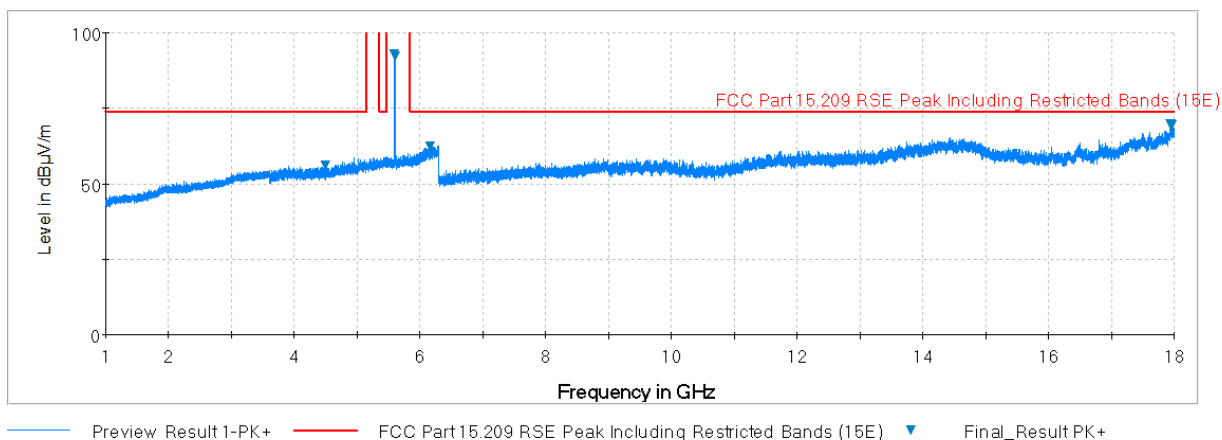
Plot 7-174. Radiated Spurious Plot above 1GHz (802.11a – U2C Ch. 120, Ant. Pol. V)
