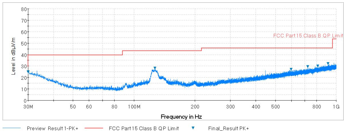
Plot 7-246. Radiated Spurious Plot below 1GHz (802.11a – U3 Ch. 157, Ant. Pol. H)
