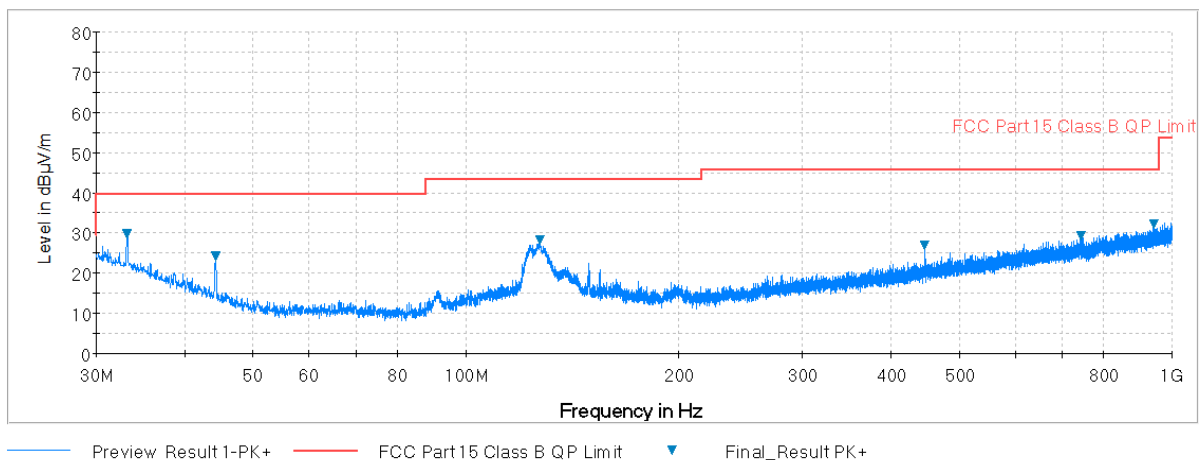
Plot 7-245. Radiated Spurious Plot below 1GHz (802.11a – U3 Ch. 157, Ant. Pol. V)
