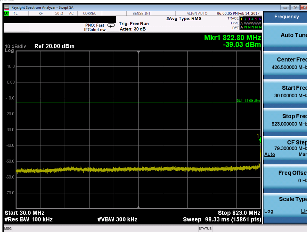
Plot 7-49. Conducted Spurious Plot (Band 5 – 5.0MHz QPSK – RB Size 1, RB Offset 0 – Low Channel)
