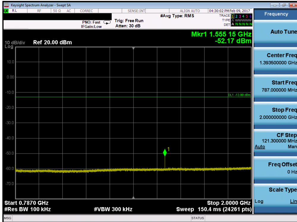
Plot 7-47. Conducted Spurious Plot (Band 13 – 10.0MHz QPSK – RB Size 1, RB Offset 0)
