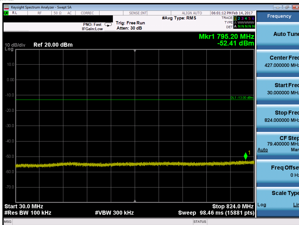
Plot 7-55. Conducted Spurious Plot (Band 5 – 5.0MHz QPSK – RB Size 1, RB Offset 0 – High Channel)
