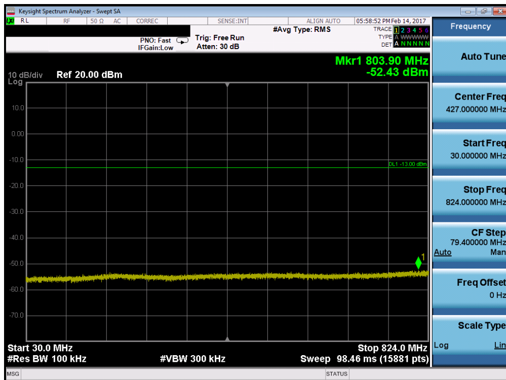
Plot 7-52. Conducted Spurious Plot (Band 5 – 5.0MHz QPSK – RB Size 1, RB Offset 0 – Mid Channel)
