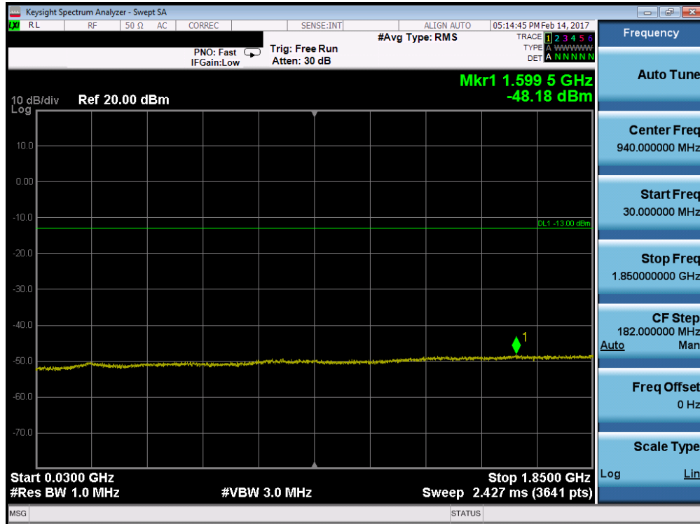
Plot 7-73. Conducted Spurious Plot (Band 2 – 15.0MHz QPSK – RB Size 1, RB Offset 0 – High Channel)
