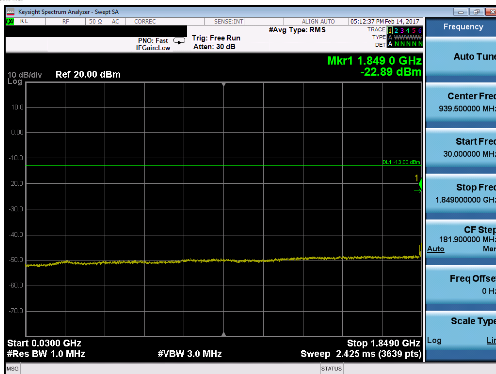
Plot 7-67. Conducted Spurious Plot (Band 2 – 15.0MHz QPSK – RB Size 1, RB Offset 0 – Low Channel)
