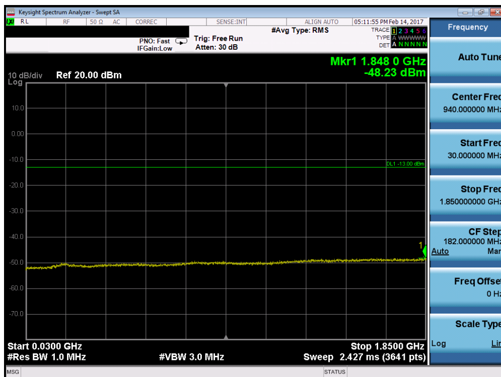
Plot 7-70. Conducted Spurious Plot (Band 2 – 15.0MHz QPSK – RB Size 1, RB Offset 0 – Mid Channel)
