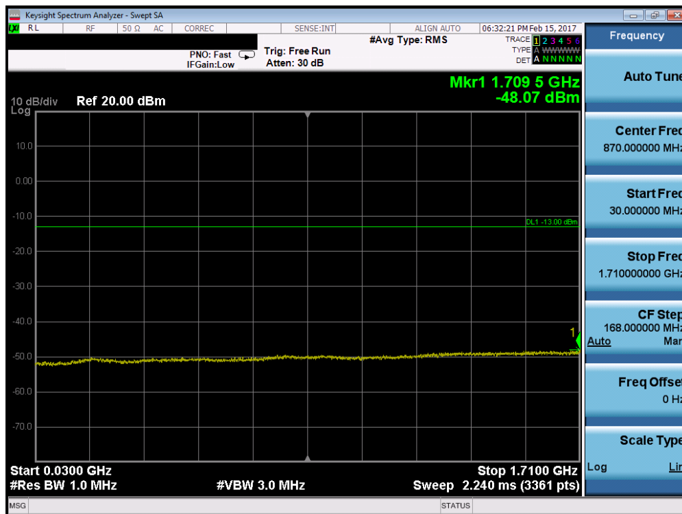
Plot 7-64. Conducted Spurious Plot (Band 4 – 15.0MHz QPSK – RB Size 1, RB Offset 0 – High Channel)
