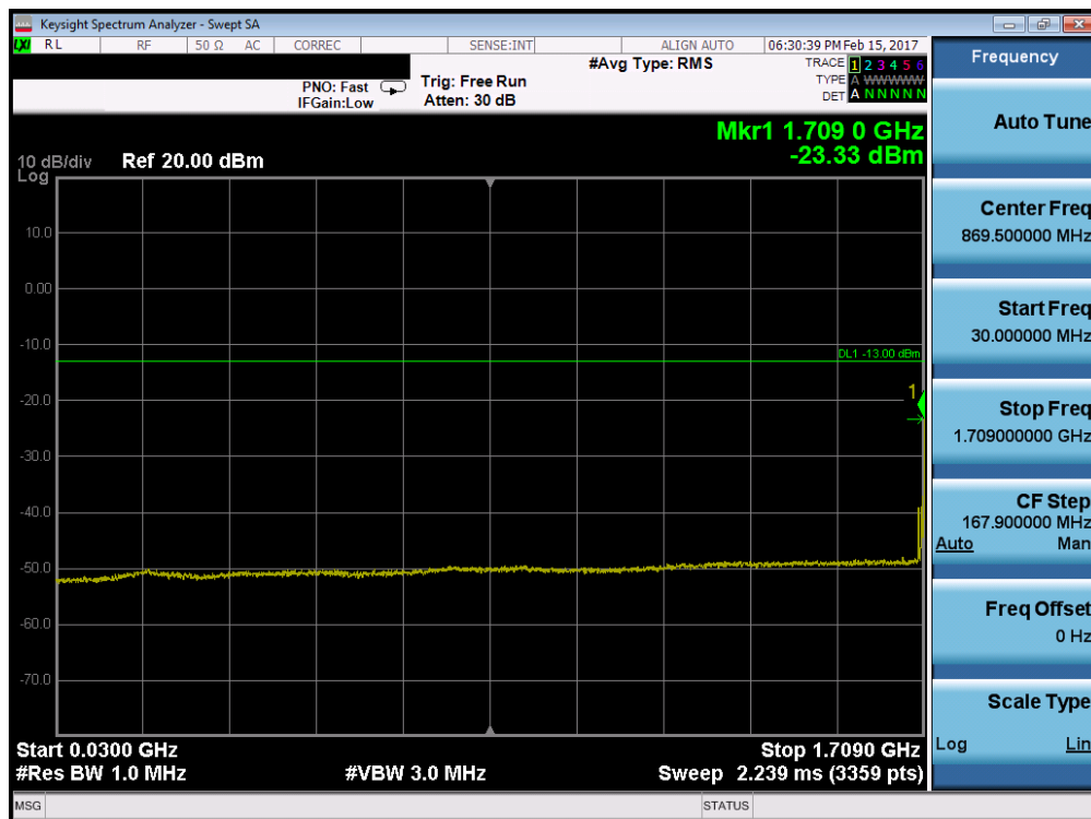
Plot 7-58. Conducted Spurious Plot (Band 4 – 15.0MHz QPSK – RB Size 1, RB Offset 0 – Low Channel)
