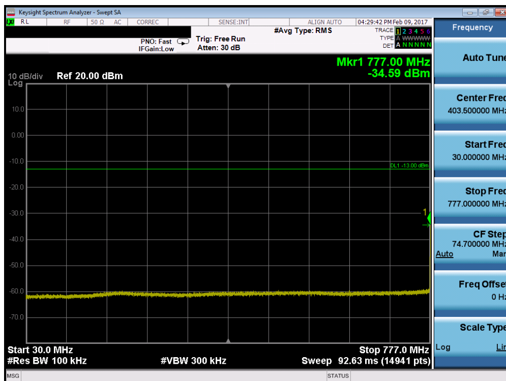
Plot 7-46. Conducted Spurious Plot (Band 13 – 10.0MHz QPSK – RB Size 1, RB Offset 0)
