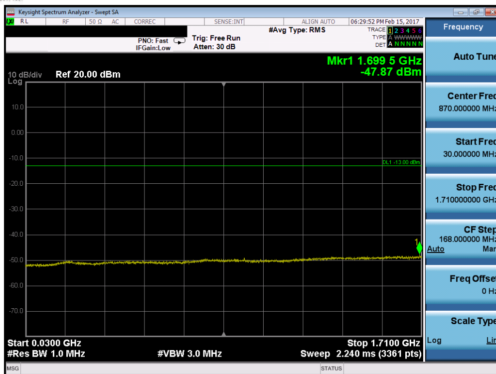
Plot 7-61. Conducted Spurious Plot (Band 4 – 15.0MHz QPSK – RB Size 1, RB Offset 0 – Mid Channel)
