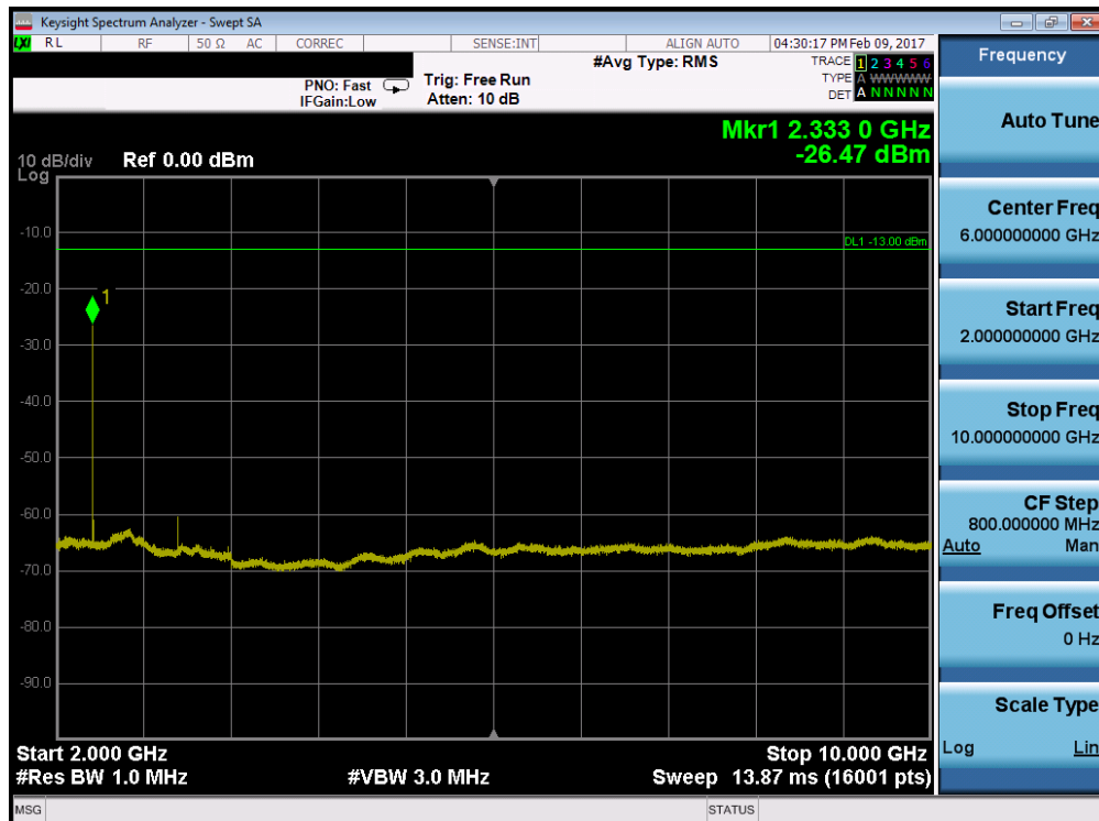
Plot 7-48. Conducted Spurious Plot (Band 13 – 10.0MHz QPSK – RB Size 1, RB Offset 0)
