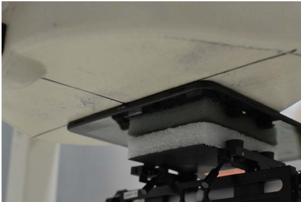
SAR Test Setup Photo 2: Back Side at 0.0 cm (Licensed Modes)
