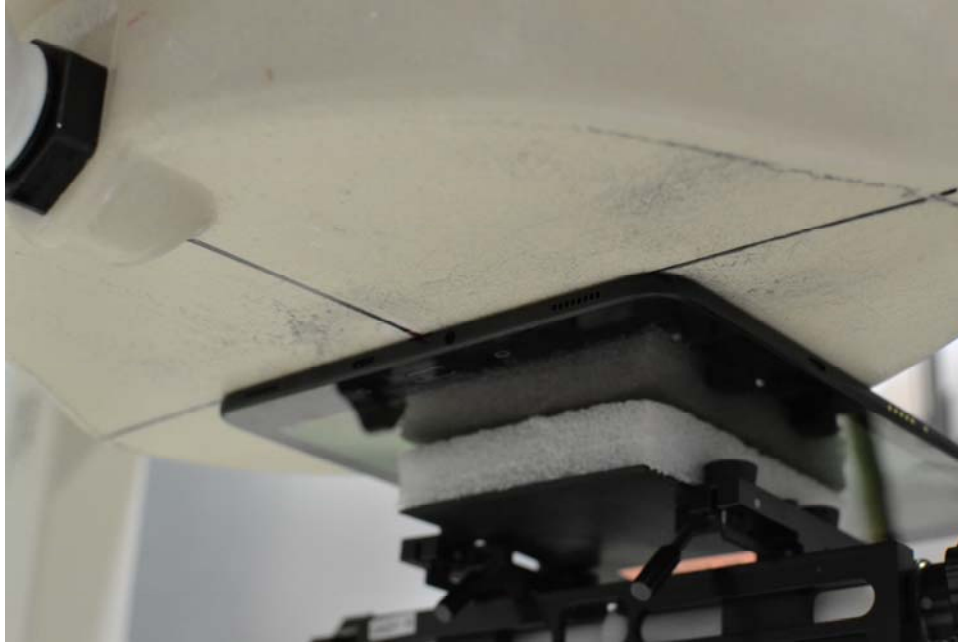
SAR Test Setup Photo 3: Back Side at 0.0 cm (Unlicensed Modes)
