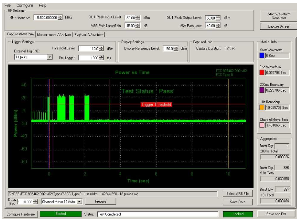
Figure 5-4. Band 2C Move Time and Aggregate Time
