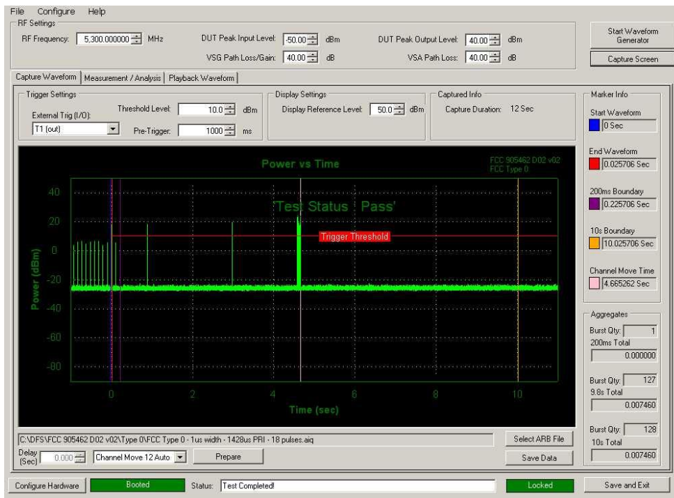
Figure 5-3. Band 2A Move Time and Aggregate Time
