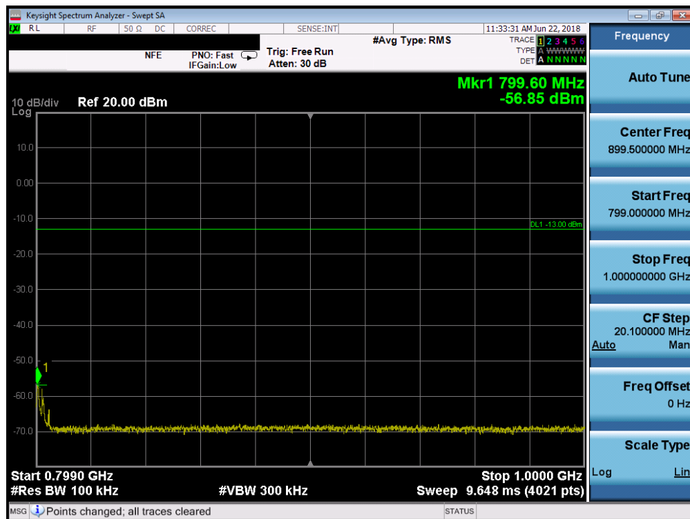
Plot 7-14. Conducted Spurious Plot (LTE Band 14, 5MHz QPSK – RB Size 1, RB Offset 0 – High Channel)
