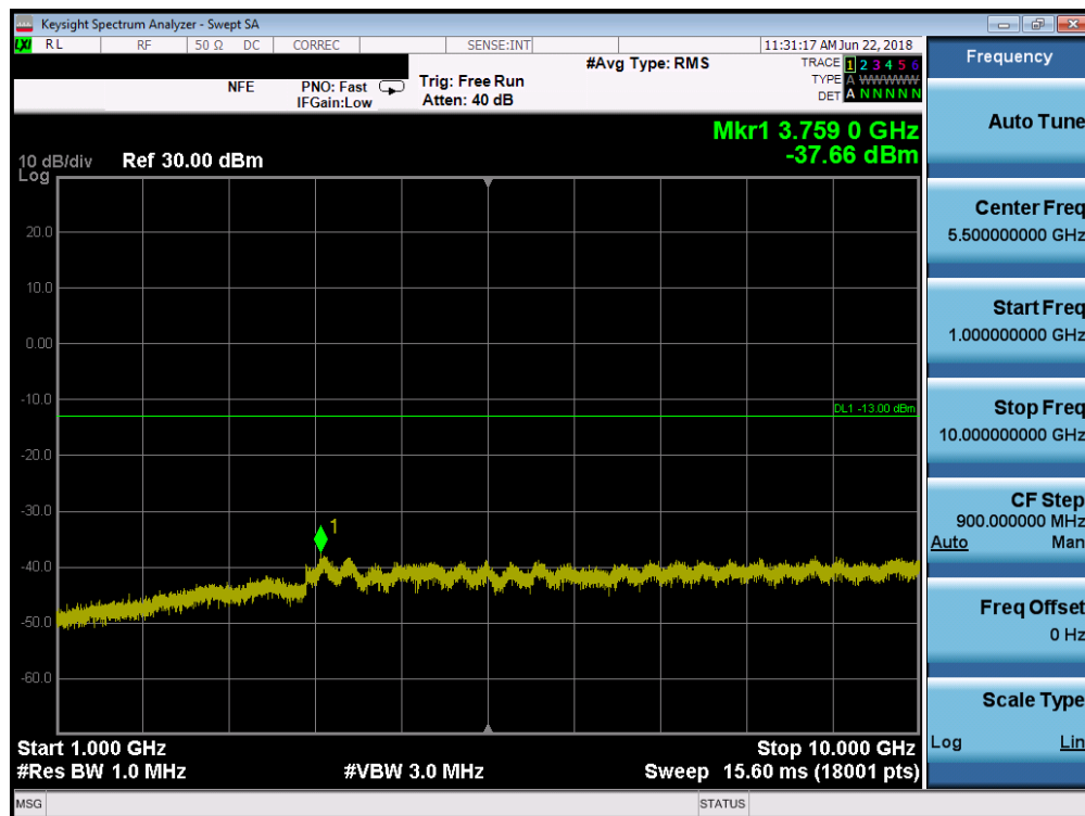
Plot 7-12. Conducted Spurious Plot (LTE Band 14, 5MHz QPSK – RB Size 1, RB Offset 0 – Mid Channel)
