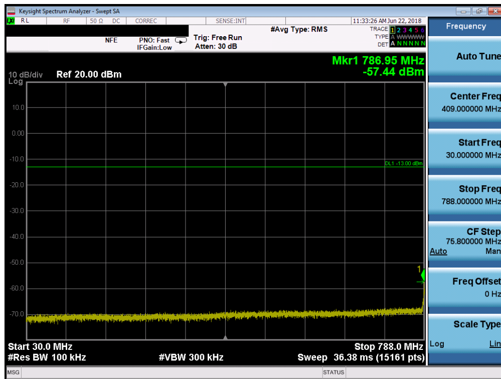
Plot 7-13. Conducted Spurious Plot (LTE Band 14, 5MHz QPSK – RB Size 1, RB Offset 0 – High Channel)
