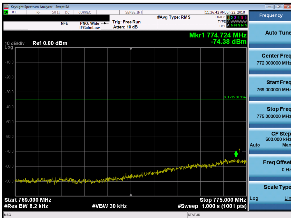
Plot 7-21. Lower Emission Mask Plot (LTE Band 14, 10MHz QPSK – RB Size 50)
