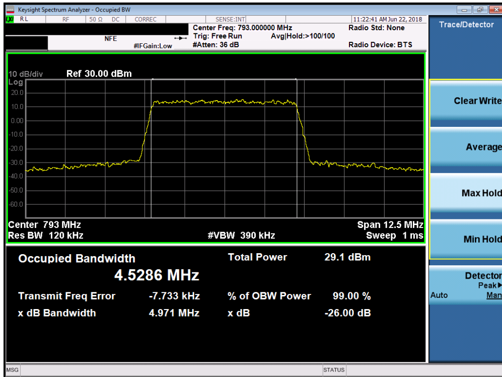
Plot 7-3. Occupied Bandwidth Plot (LTE Band 14, 5MHz 64-QAM – RB Size 25)
