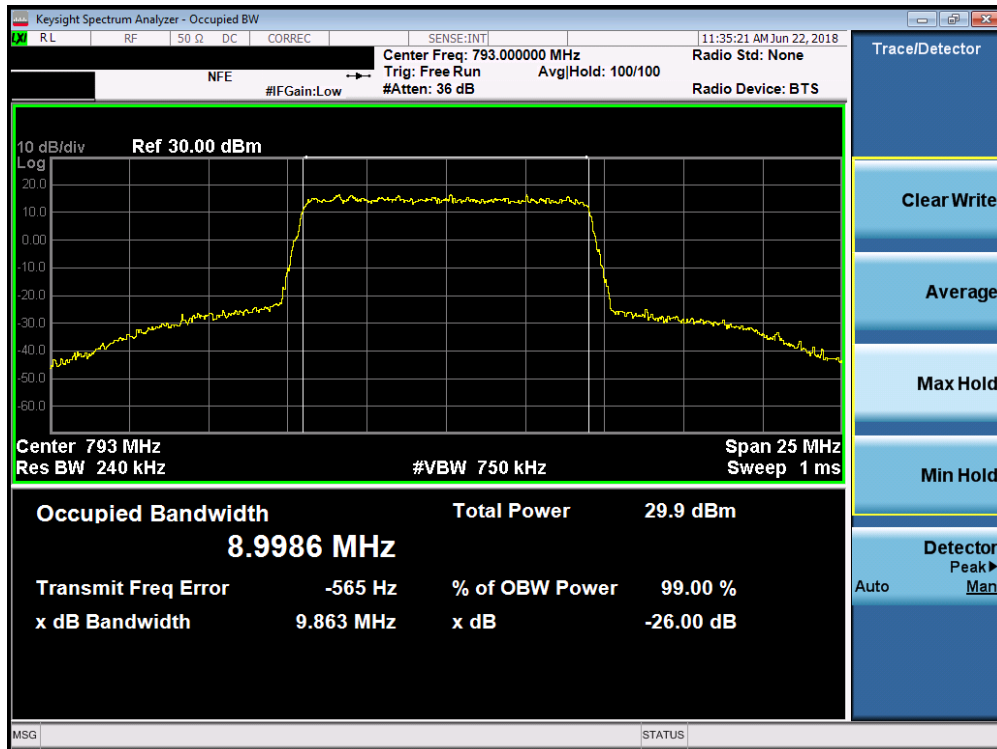
Plot 7-5. Occupied Bandwidth Plot (LTE Band 14, 10MHz 16-QAM – RB Size 50)
