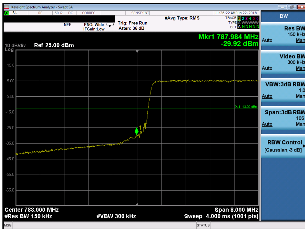
Plot 7-20. Lower Band Edge Plot (LTE Band 14, 10MHz QPSK – RB Size 50)
