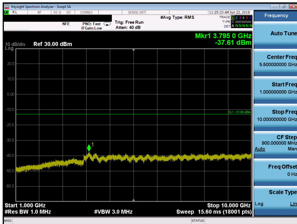
Plot 7-9. Conducted Spurious Plot (LTE Band 14, 5MHz QPSK – RB Size 1, RB Offset 0 – Low Channel)
