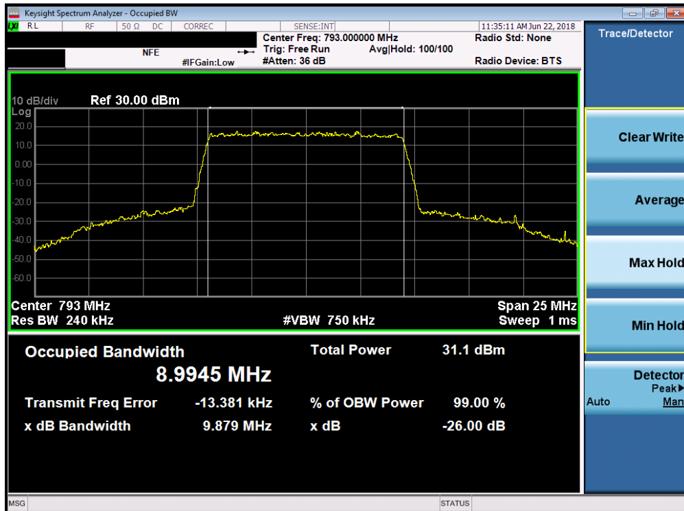
Plot 7-4. Occupied Bandwidth Plot (LTE Band 14, 10MHz QPSK – RB Size 50)
