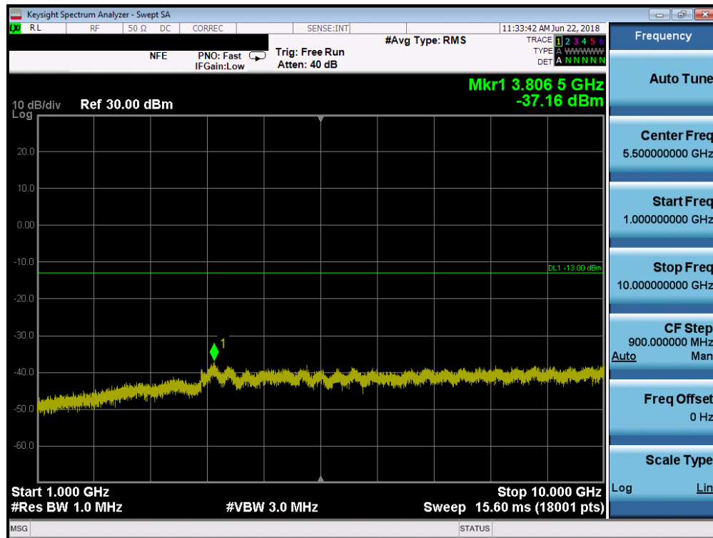
Plot 7-15. Conducted Spurious Plot (LTE Band 14, 5MHz QPSK – RB Size 1, RB Offset 0 – High Channel)
