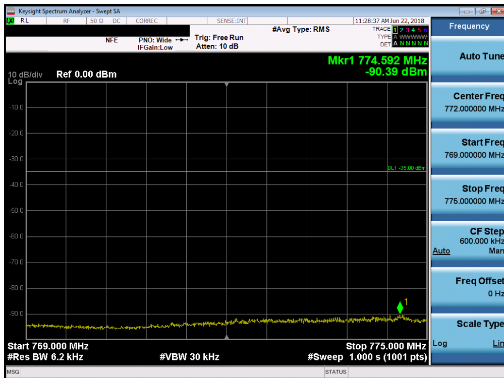
Plot 7-17. Lower Emission Mask Plot (LTE Band 14, 5MHz QPSK – RB Size 25)
