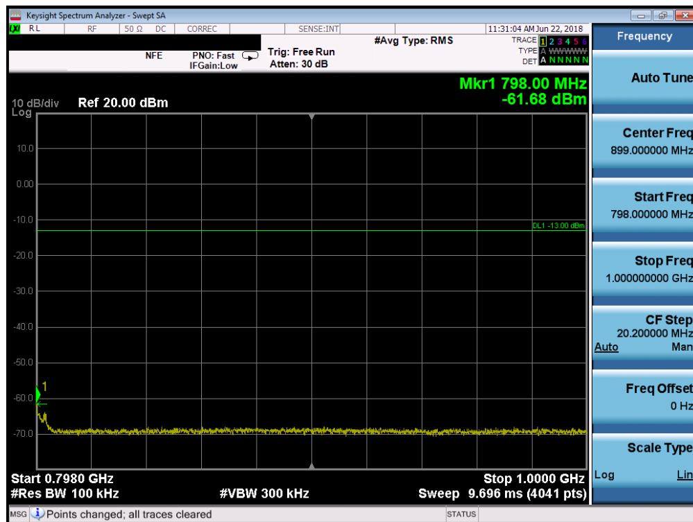
Plot 7-11. Conducted Spurious Plot (LTE Band 14, 5MHz QPSK – RB Size 1, RB Offset 0 – Mid Channel)
