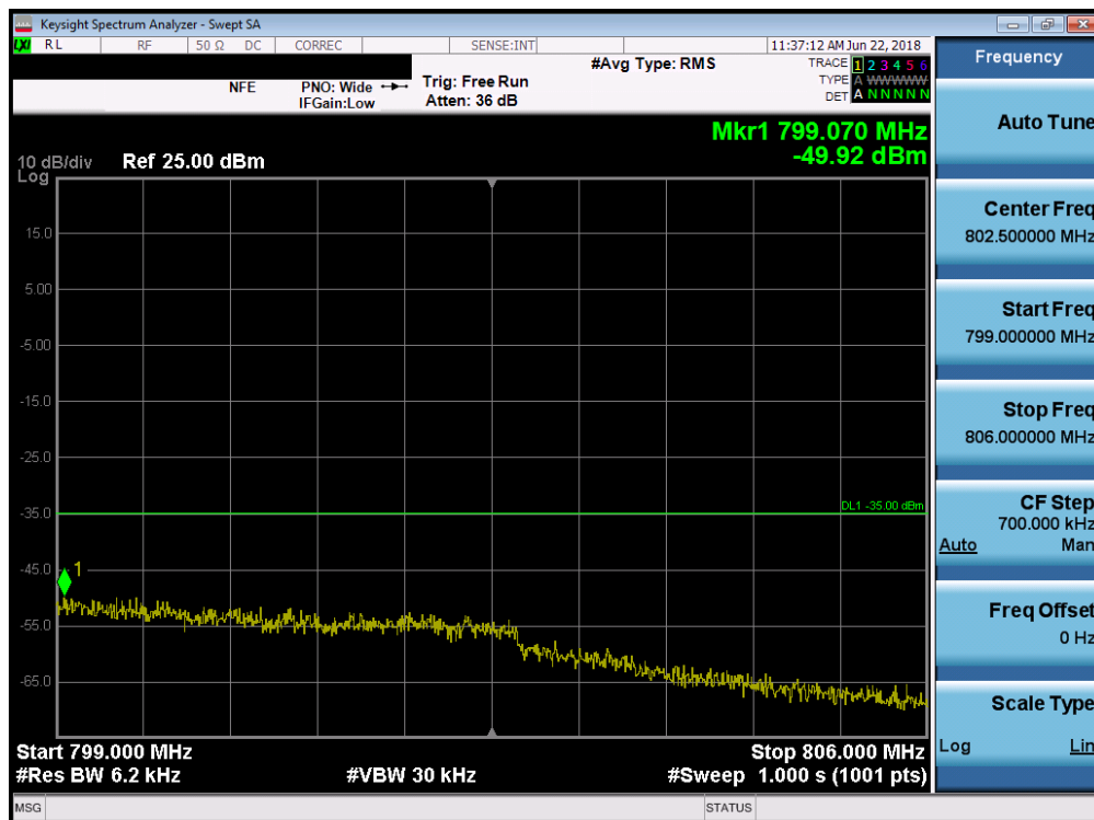
Plot 7-23. Upper Emission Mask Plot (LTE Band 14, 10MHz QPSK - RB Size 50)
