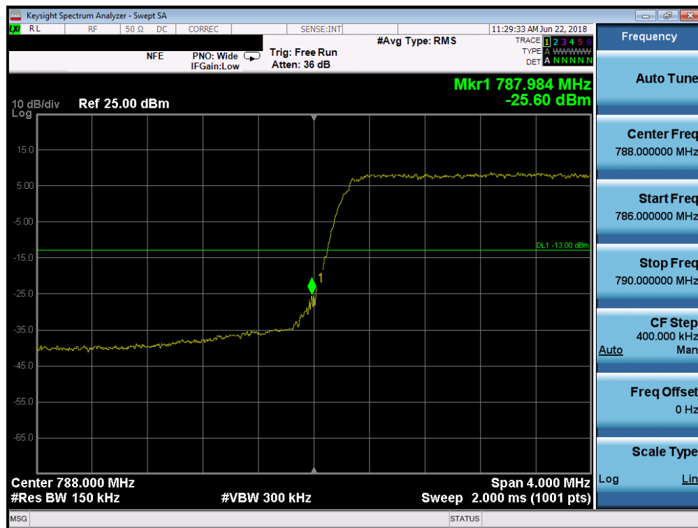
Plot 7-16. Lower Band Edge Plot (LTE Band 14, 5MHz QPSK – RB Size 25)
