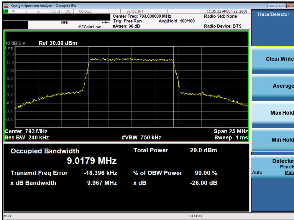
Plot 7-6. Occupied Bandwidth Plot (LTE Band 14, 10MHz 64-QAM – RB Size 50)
