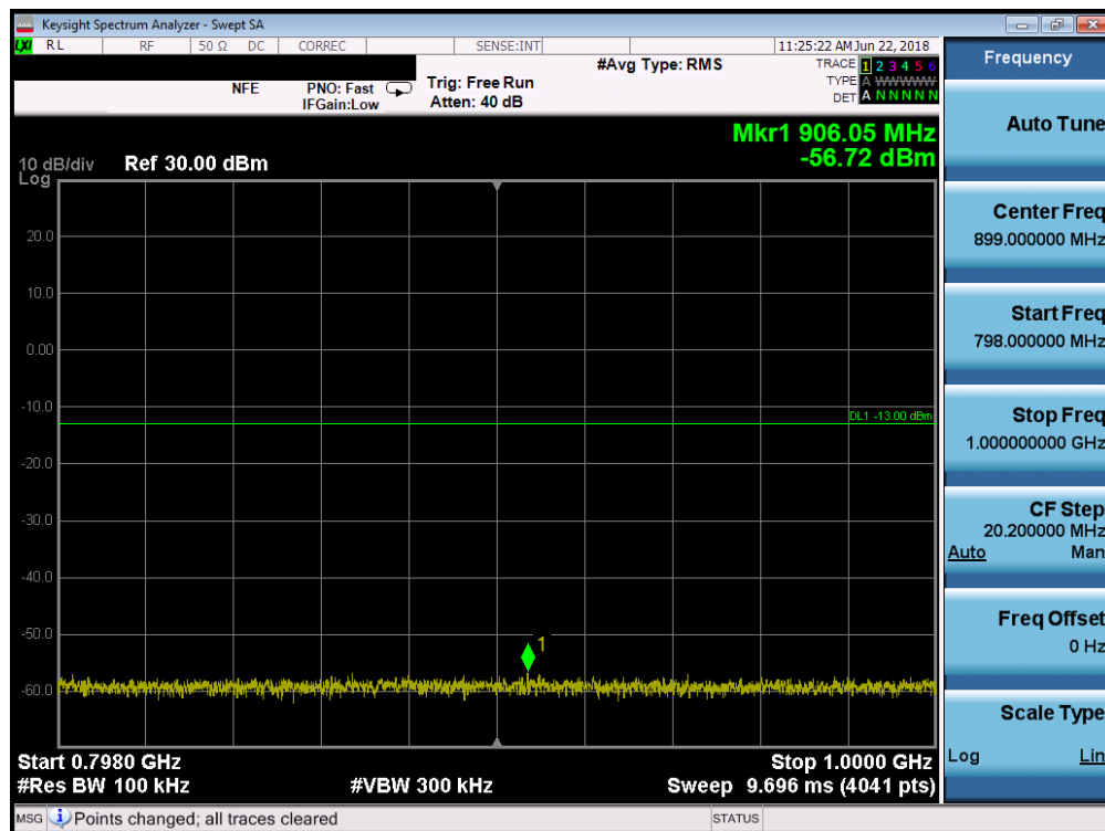
Plot 7-8. Conducted Spurious Plot (LTE Band 14, 5MHz QPSK – RB Size 1, RB Offset 0 – Low Channel)
